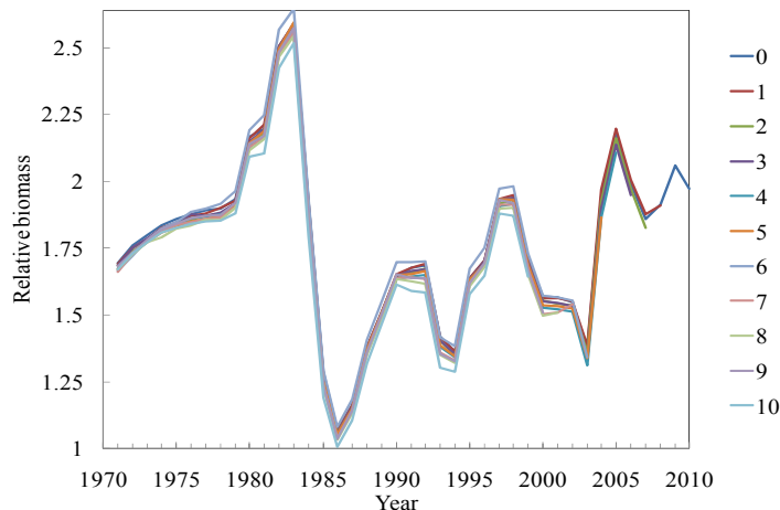
Fig. 6.18. Shrimp in ICES SA I and II: Retrospective plot of median relative biomass ( B/B_{msy} ). Relative biomass series are estimated by consecutively leaving out from 0 to 10 years of data.
