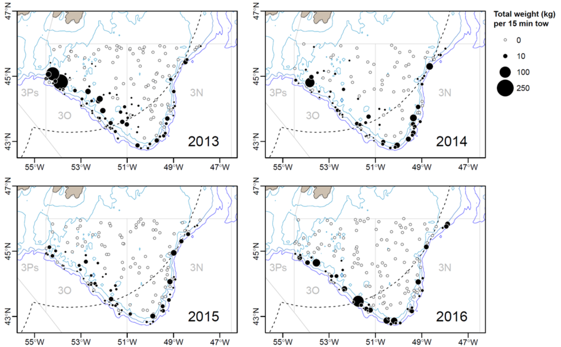
Fig. 9. Distribution of witch flounder (weight (kg) per tow) from Canadian spring surveys in NAFO Divs. 3NO during 2013 to 2016.
