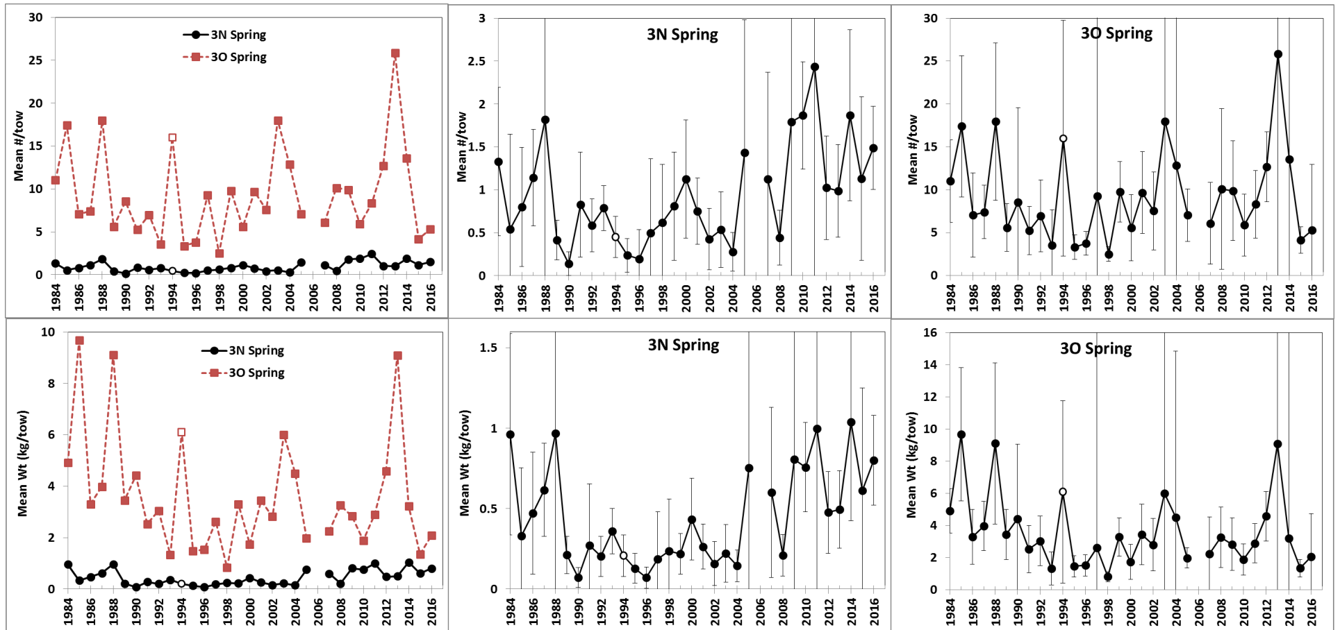
Fig. 4. Mean numbers and weights (kg) per tow for witch flounder from Canadian spring rv surveys in NAFO Divs. 3N and 3O during 1984-2016. Vertical lines represent 95% confidence intervals. White markers represent years where >50% of deep-water strata were surveyed. No data was available for spring 2006.
