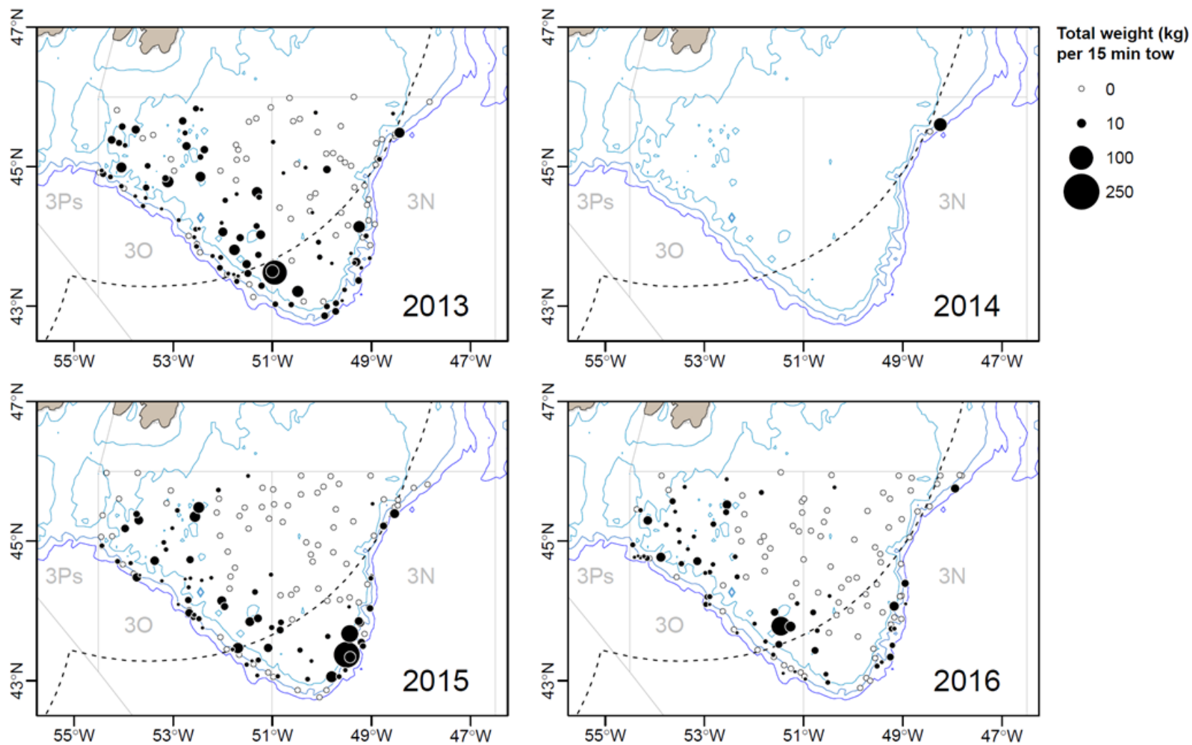
Fig. 10. Distribution of witch flounder (weight (kg) per tow) from Canadian fall surveys in NAFO Divs. 3NO during 2013 to 2016 (note there was no fall survey in 2014).
