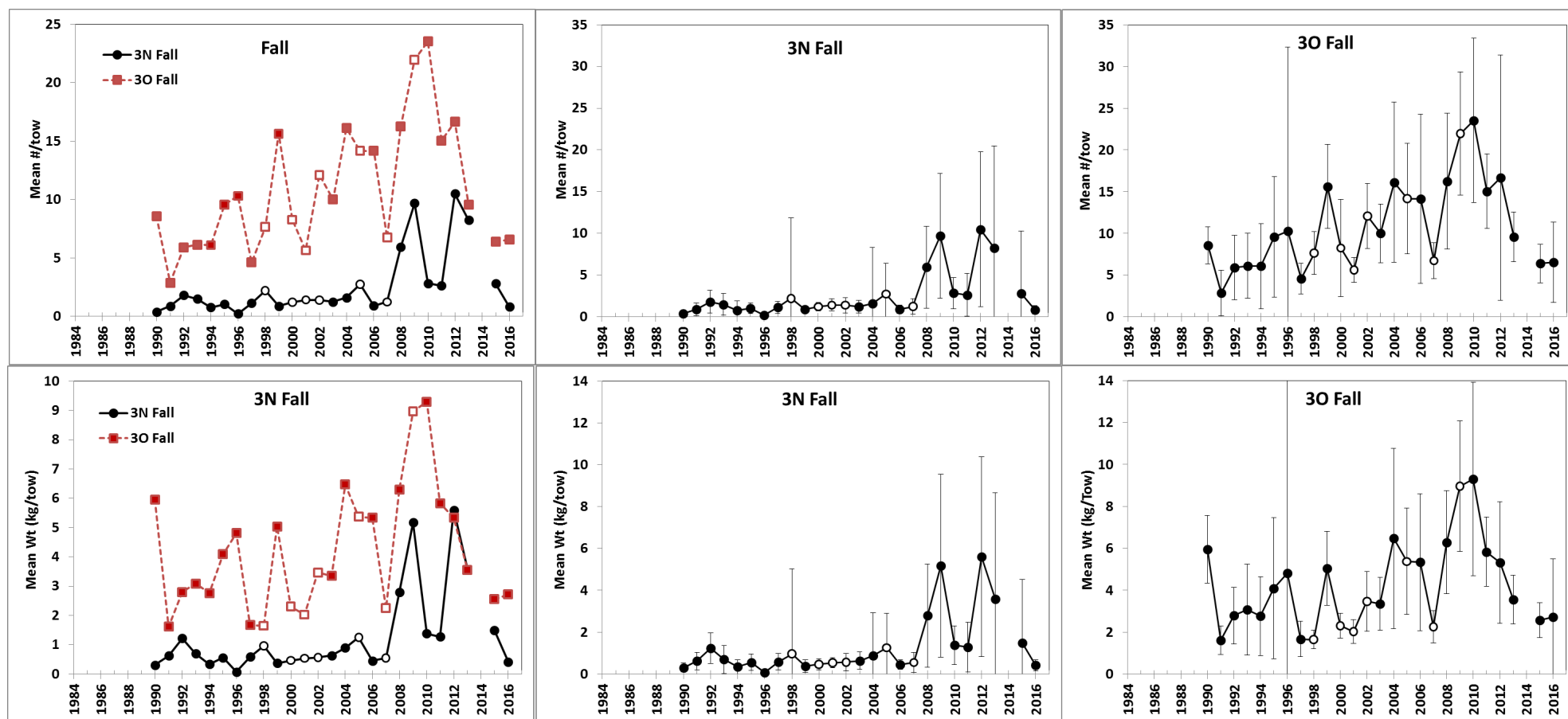
Fig. 6. Mean number per tow and mean weight (kg) per tow for witch flounder from Canadian fall surveys in NAFO Divs. 3N and 3O during 1990-2016 (no data was available for fall 2014). Vertical lines represent 95% confidence intervals. White markers represent years where >50% of deep-water strata were surveyed.
