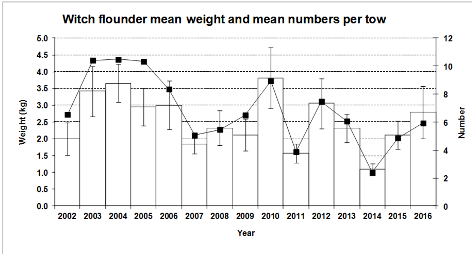
Fig. 14. Witch flounder stratified mean catches (kg) and mean number by year. Spanish spring surveys in NAFO Divs. 3NO: 2002-2016.
