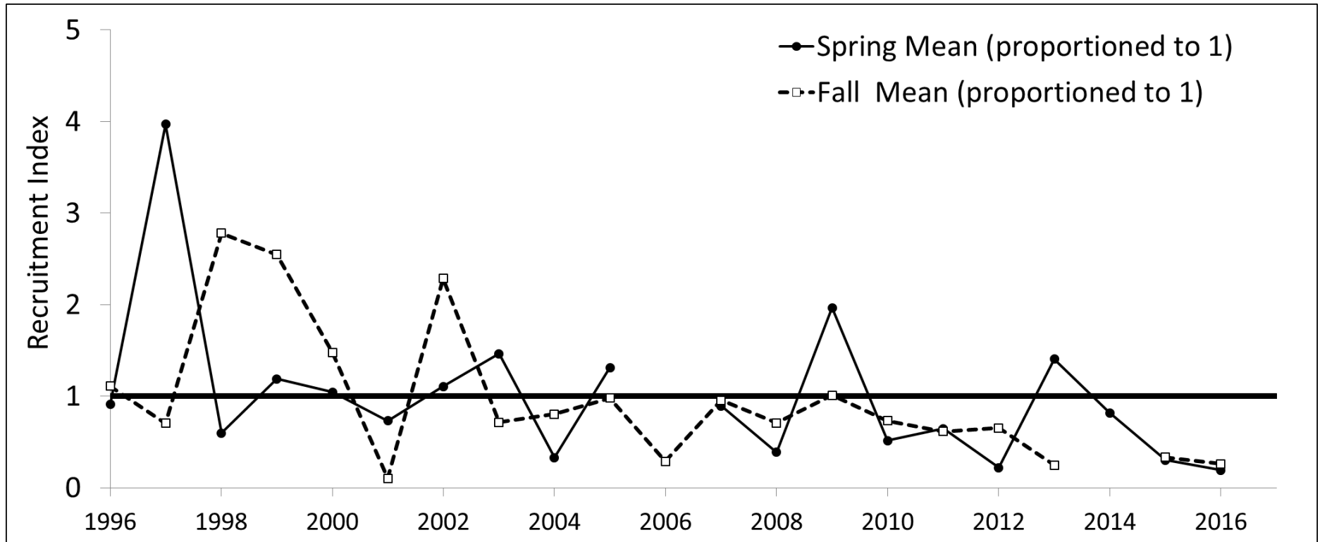
Fig.13. Recruitment index means proportioned to 1 of witch flounder <21cm in length from spring and fall Canadian rv surveys in NAFO Divs. 3NO 1995-2016. Note there was no fall survey in 2014 or spring survey in 2006.
