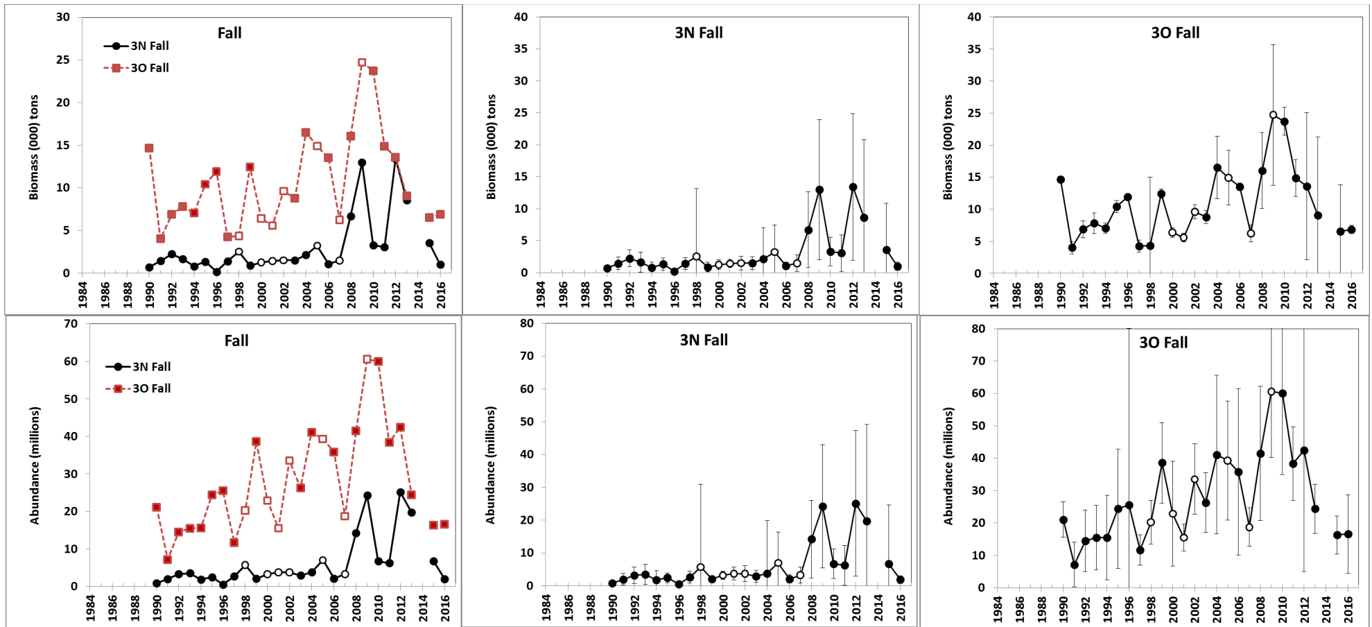
Fig. 5. Biomass (tons), abundance (millions) for witch flounder from Canadian fall surveys in NAFO Divs. 3N and 30 during 1990-2016 (no data was available for fall 2014). Vertical lines represent 95% confidence intervals. White markers represent years where >50% of deep-water strata were surveyed.
