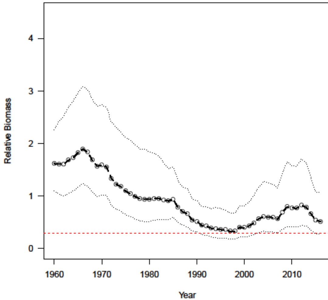
Fig. 17. Relative biomass (biomass divided by BMSY) for Div. 3NO witch flounder. The median with its 80 th percent credible intervals are shown. The horizontal red dashed line is Blim (30% BMSY).
