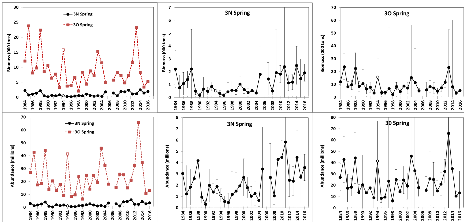
Fig. 3. Biomass (tons), abundance (millions) for witch flounder from Canadian spring rv surveys in NAFO Divs. 3N and 3O during 1984-2016. Vertical lines represent 95% confidence intervals. White markers represent years where >50% of deep-water strata were surveyed. No data was available for spring 2006.
