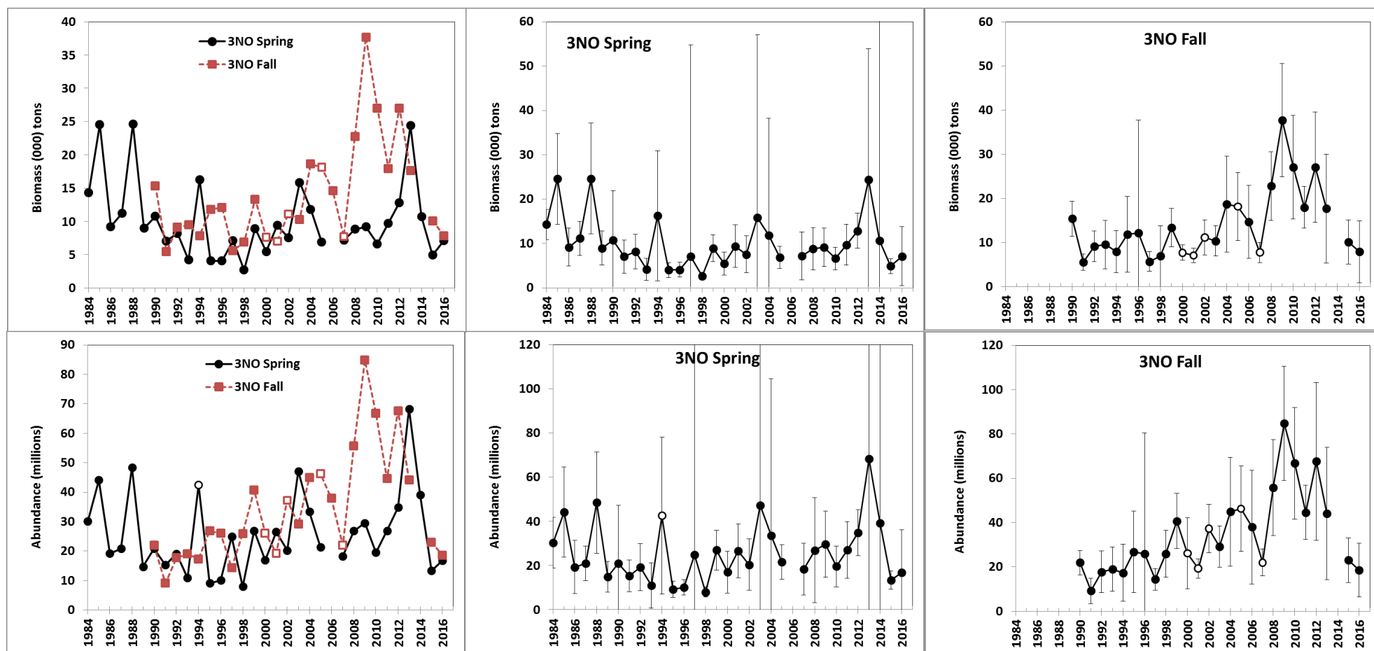
Fig. 7. Biomass (tons), abundance (millions) for witch flounder from Canadian spring and fall surveys in NAFO Divs. 3NO combined during 1984-2016 (no data was available for fall 2014 or spring 2016). Vertical lines represent 95% confidence intervals. White markers represent years where >50% of deep-water strata were surveyed.
