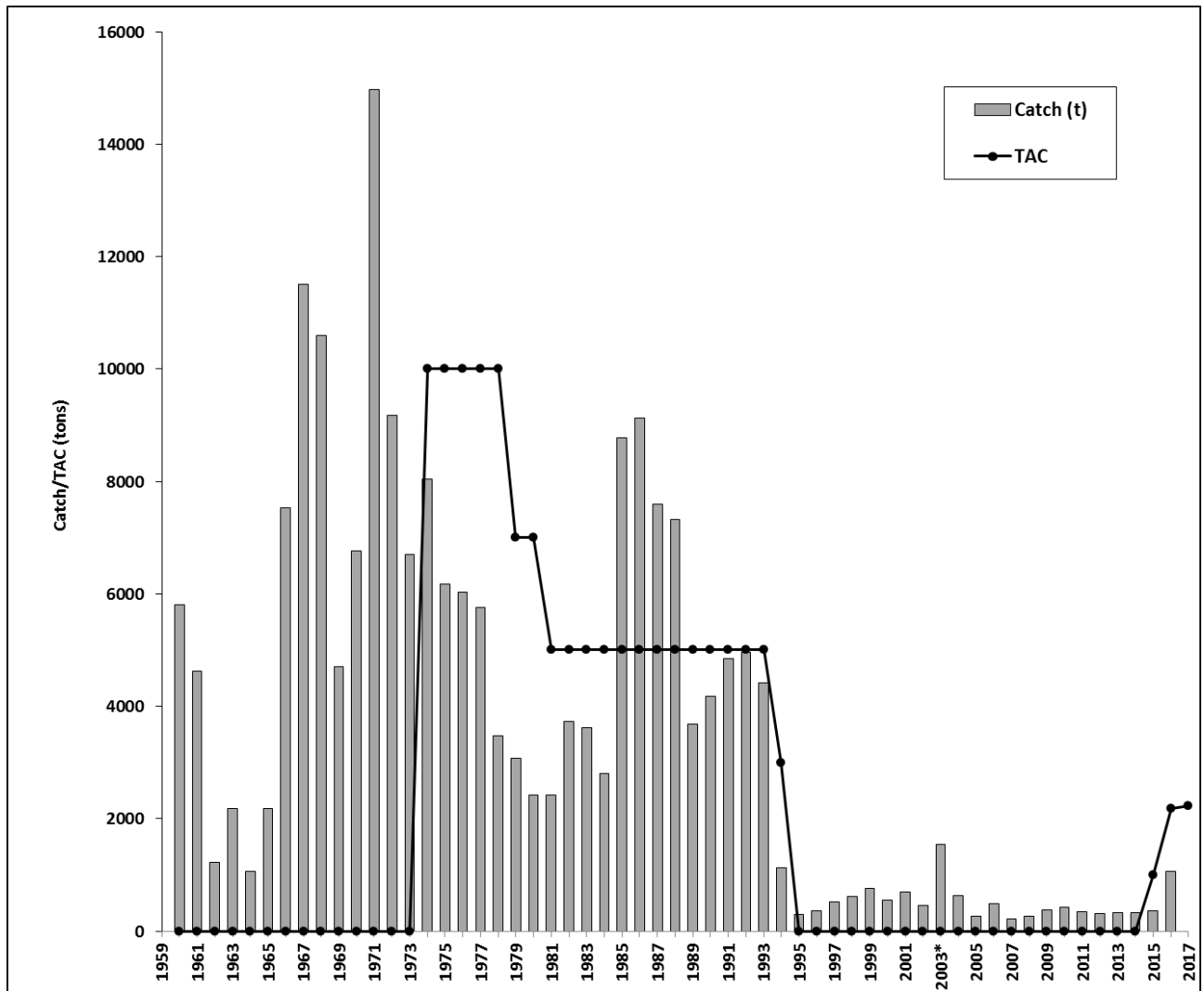
Fig. 1. Commercial catch of witch flounder in NAFO Divs. 3NO from 1960-2016 and total allowable catch (TACs).
