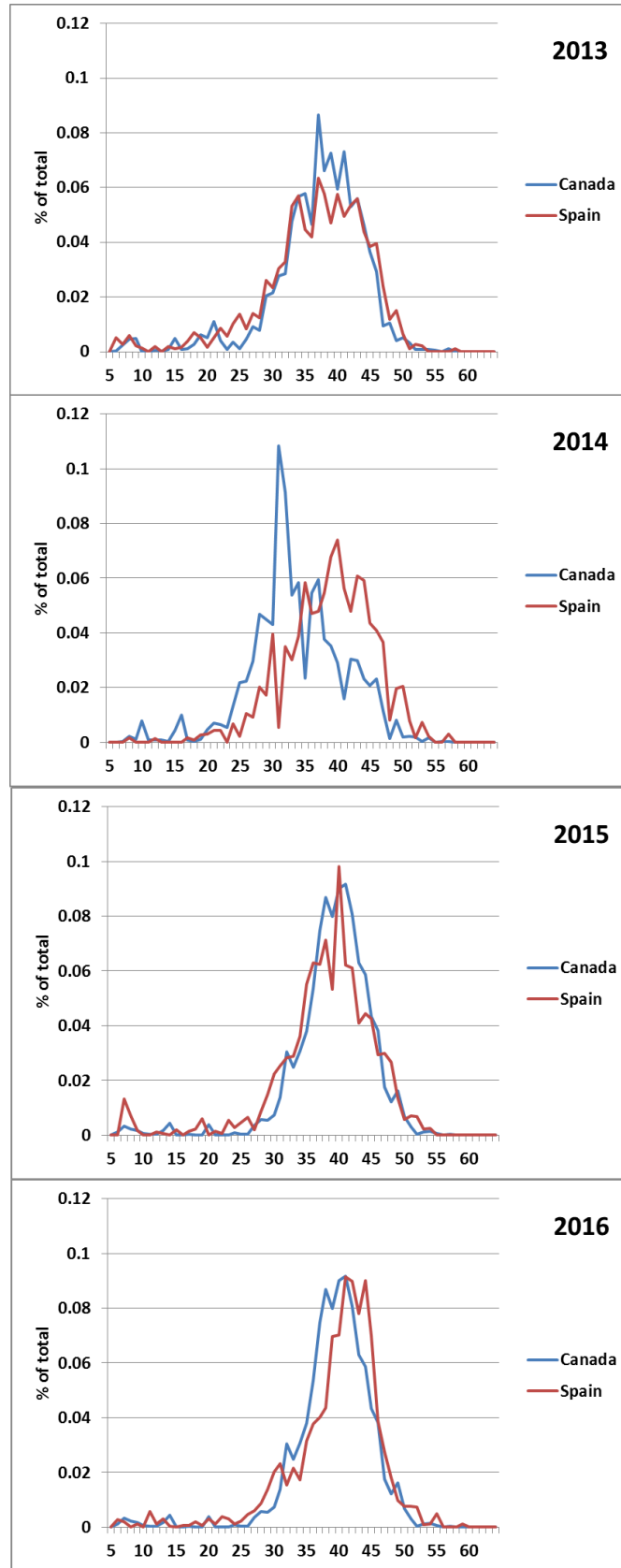
Fig. 16. Witch flounder length-frequencies (cm) for Canadian and Spanish spring rv surveys in NAFO Divs. 3NO: 2013-2016.
