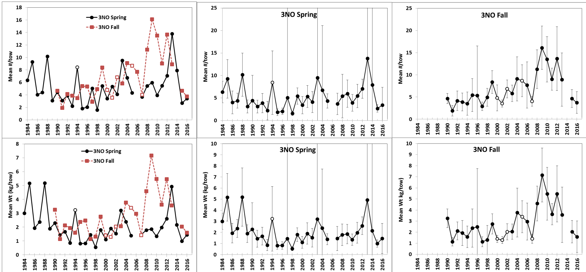
Fig. 8. Mean number per tow and mean weight (kg) per tow for witch flounder from Canadian spring and fall surveys in NAFO Divs. 3NO combined during 1984-2016 (no data was available for fall 2014 or spring 2016). Vertical lines represent 95% confidence intervals. White markers represent years where >50% of deep-water strata were surveyed.
