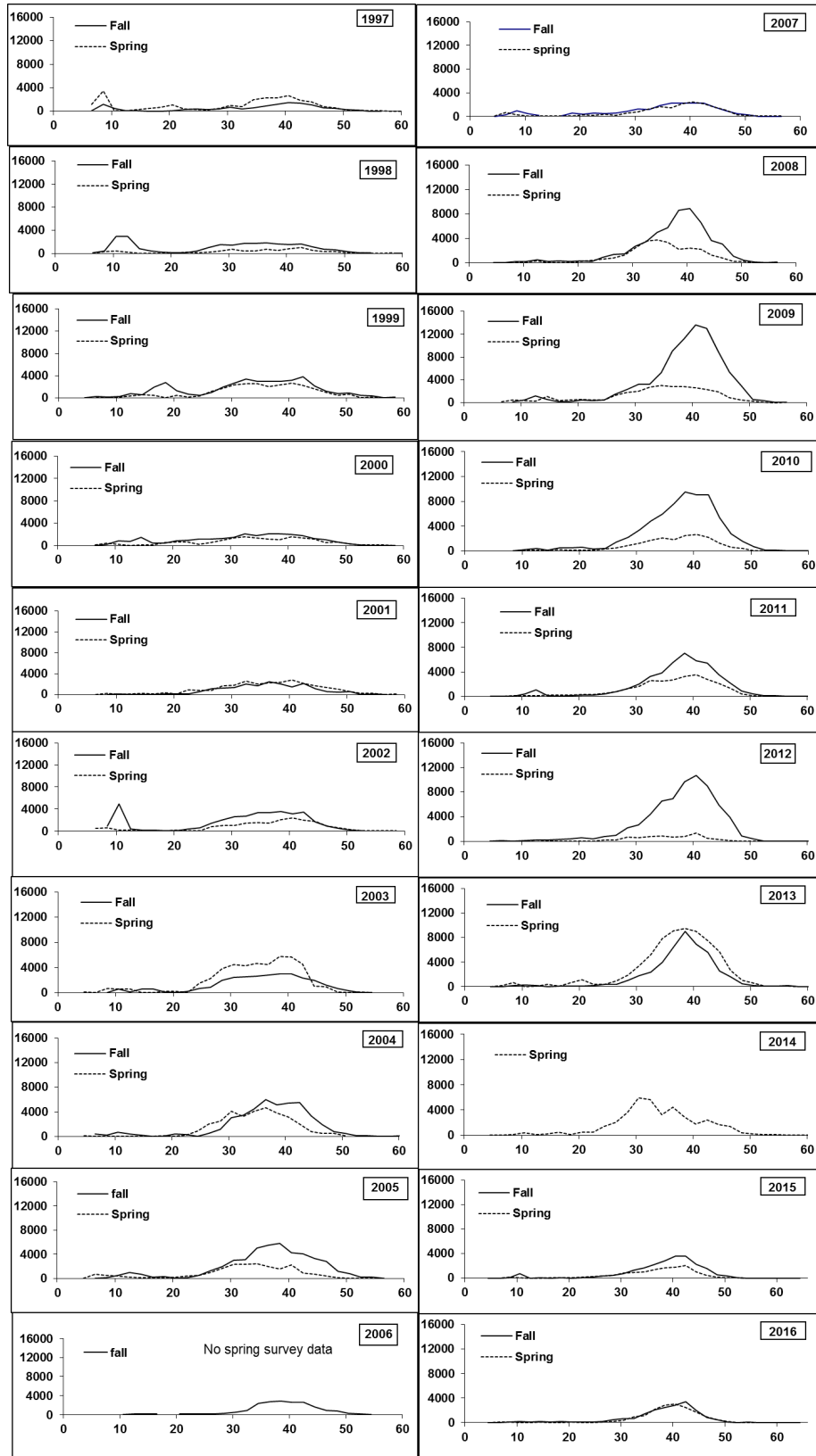
Fig. 11. Length frequency distributions of witch flounder from Canadian spring and fall surveys (1997-2016) using the Campelen 1800 shrimp trawl. Estimates represent abundance at length (cm) of the surveyed area. All distributions are for NAFO Divs. 3NO.
