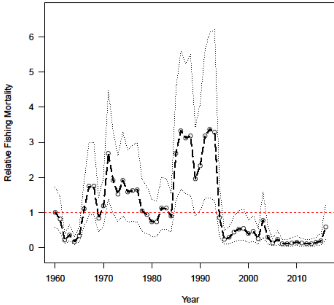
Fig. 18. Relative fishing mortality (fishing mortality divided by FMSY) for Div. 3NO witch flounder. The median with its 80th percent credible intervals are shown. The horizontal red dashed line is Flim (FMSY)
