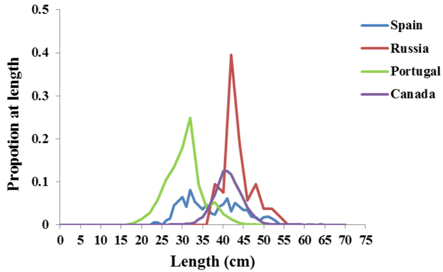
Fig. 2. Witch flounder length frequency (cm) distributions for Spain, Russia, and Portugal, and Canada commercial fisheries in NAFO Divs. 3NO in 2016.
