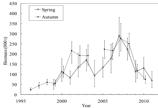
Fig. 2.2. Northern Shrimp in Div. 3LNO: biomass index estimates from Canadian spring and autumn multi-species surveys (with 95% confidence intervals).
