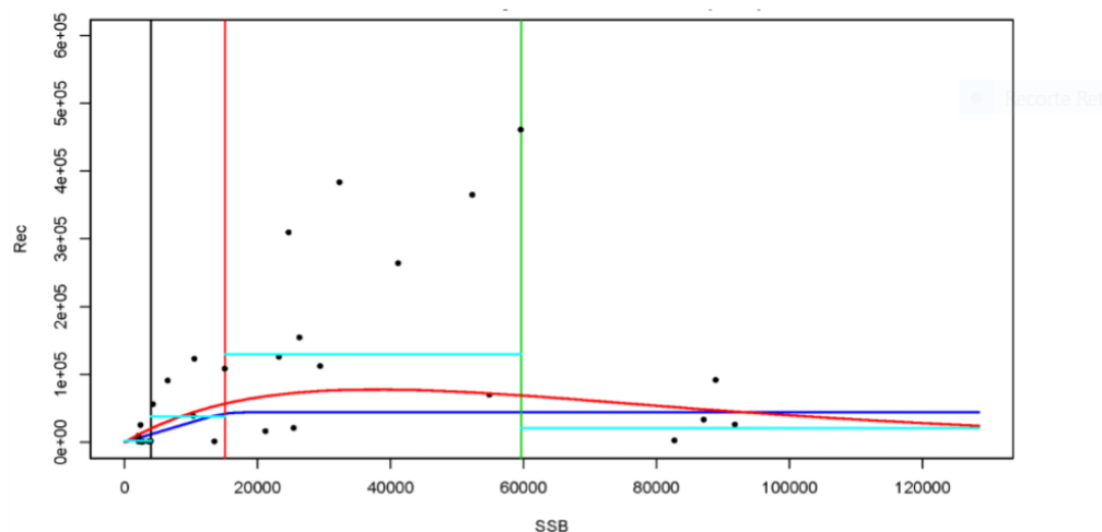
Figure 5. Historical SSB/recruit pairs (posterior medians) for the base case OM, with the SSB divided into bins with cut-offs at SSB 1997 (black line), SSB 2007 (red) and SSB 2010 (green). A segmented regression with a break point at SSB 2007 and a Ricker curve fitted to years with SSB > SSB 1997 are shown by the dark blue and red fitted lines respectively. The sky blue lines represent the geometric mean of historical recruitment within each SSB bin.
