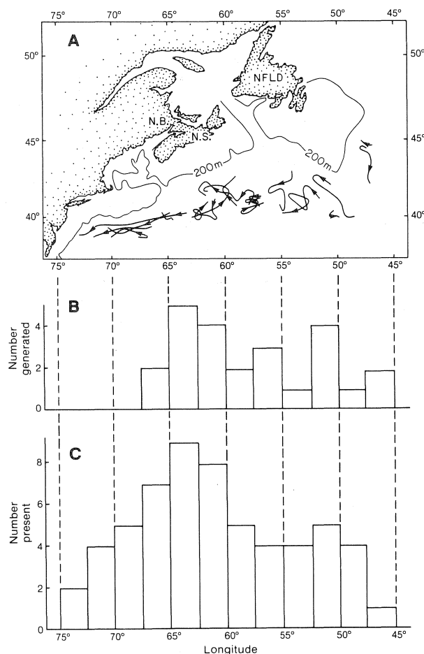
Fig. 10. Warm-core Gulf Stream rings in the region between 45° W and 75° W during 1988: (A) tracks of rings with a lifespan longer than 2 months; (B) number of rings generated in each 2.5° zone of longitude; and (C) number of rings present in each 2.5° zone during some part of the year.
