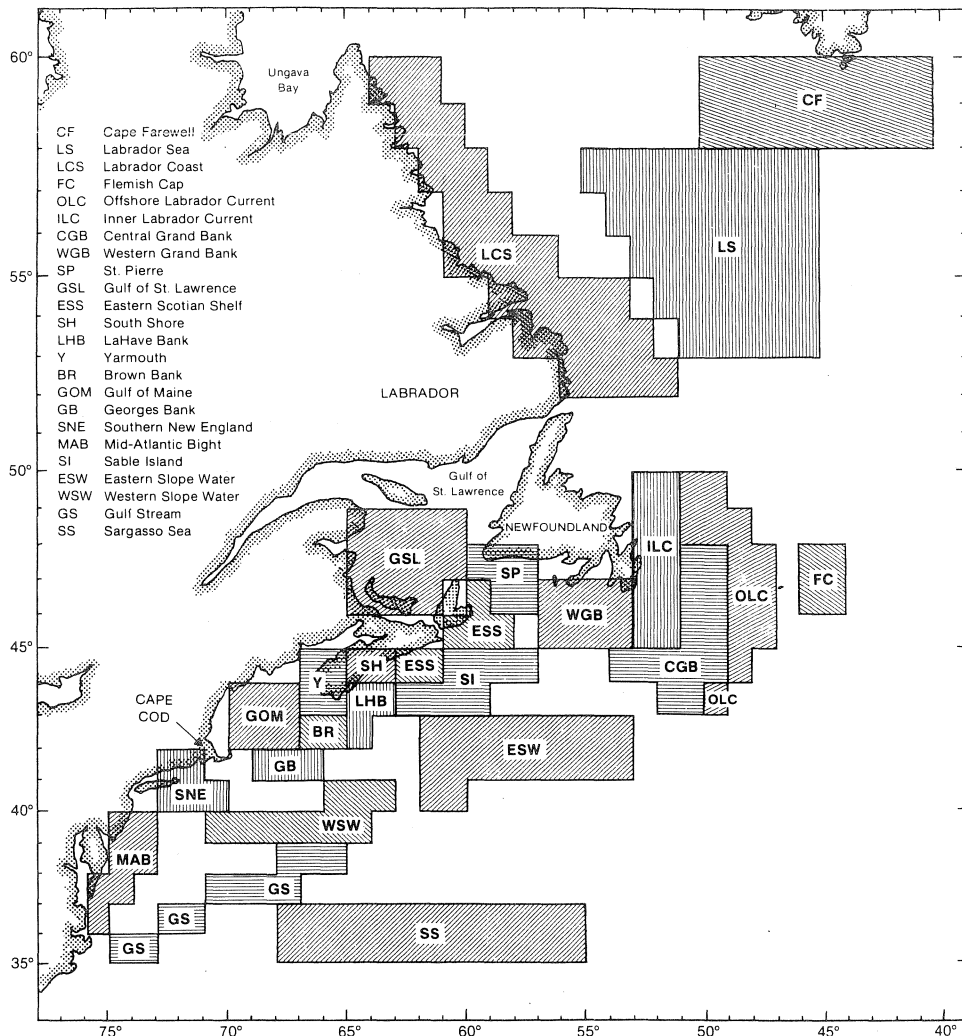
Fig. 6. Geographic boundaries of 24 subregions (Cape Hatteras to Cape Farewell) for which sea-surface temperatures were analyzed on a monthly basis.
