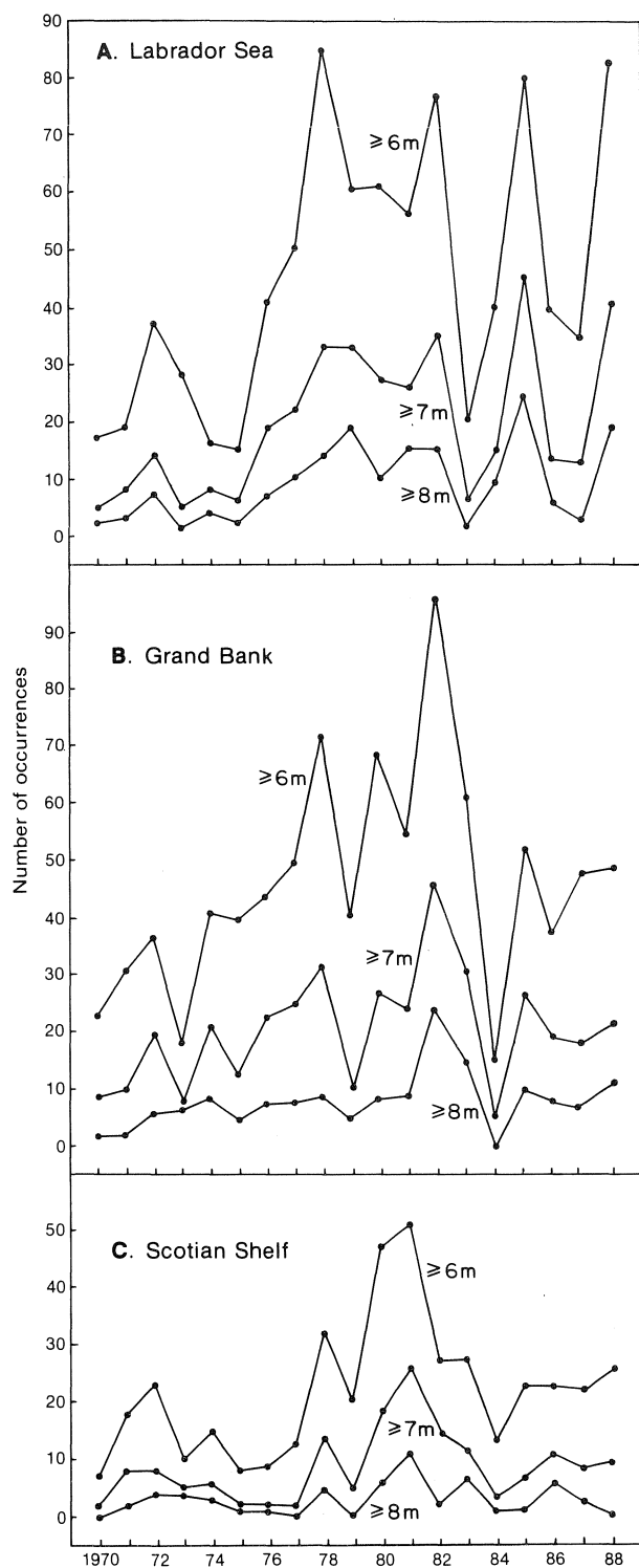
Fig. 12. Annual occurrences of storms during which wave heights exceeded 6, 7, and 8 m in three regions of the Northwest Atlantic during 1970-88.
