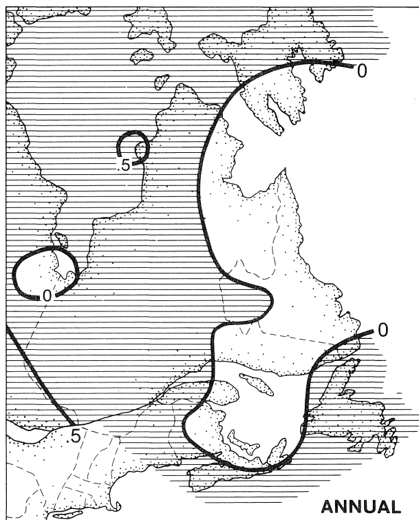
Fig. 16. Annual air temperature anomalies ( ^{\circ}\text{C} ) over eastern Canada in 1988 relative to the 1951-80 means. (Positive anomalies are shaded.)
