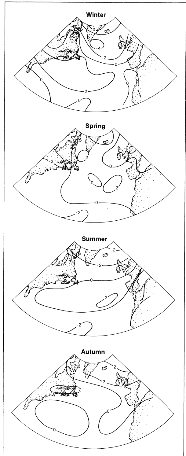
Fig. 17. Seasonal sea-surface air-pressure anomalies (mb) over the North Atlantic in 1988 relative to the 1951-80 means.
