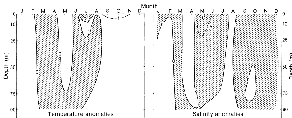
Fig. 9. Monthly temperature and salinity anomalies at Prince 5 near the entrance to the Bay of Fundy during 1988 relative to the 1951-80 means (Shaded areas represent positive anomalies).
