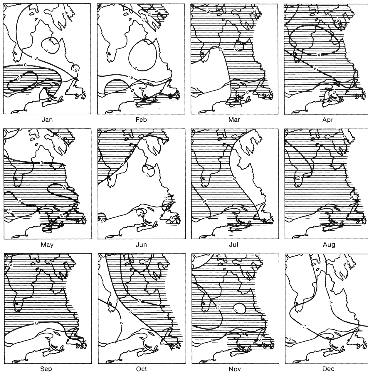
Fig. 15. Monthly air temperature anomalies ( ^{\circ}\text{C} ) over eastern Canada in 1988 relative to the 1951-80 means. (Positive anomalies are shaded.)
