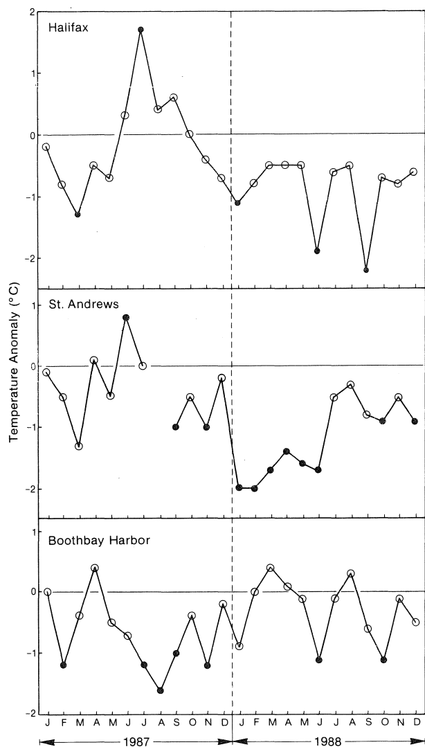
Fig. 2. Monthly sea-surface temperature anomalies at Halifax, St. Andrews and Boothbay Harbor in 1987 and 1988 relative to the 1951-80 means. (Solid dots indicate months when the anomalies equaled or exceeded one standard deviation. The missing data for St. Andrews during August, 1987, was due to an instrument malfunction.)
