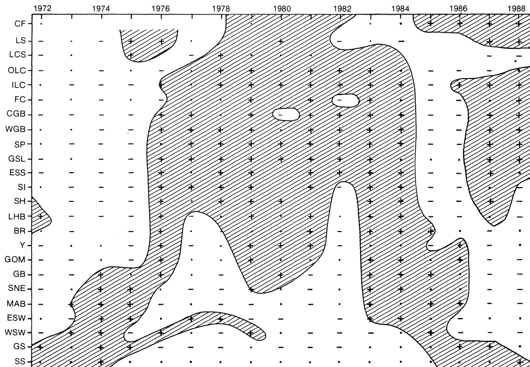
Fig. 7. Distribution of positive (+) and negative (-) annual sea-surface temperature anomalies in 1972-88 by subregion (Fig. 6) relative to the 1972-80 means. (Only anomalies less than -0.15^{\circ}\text{C} and greater than +0.15^{\circ}\text{C} were used in drawing the contours.)
