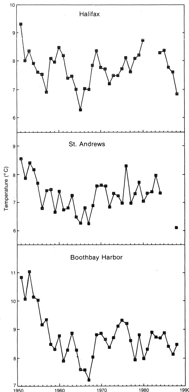
Fig. 3. Annual sea-surface temperatures at Halifax, St. Andrews and Boothbay Harbor during 1951-88.
