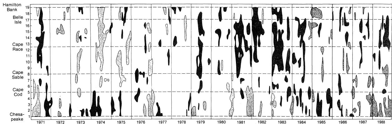
Fig. 5. Contoured monthly sea-surface temperature anomalies (relative to the 1971–80 means) for the 1971–88 period by area (Fig. 4). (Only anomalies exceeding 1.0^{\circ}\text{C} (black) and less than -1.0^{\circ}\text{C} (dotted) which extended in space through at least two neighbouring areas or in time for at least two consecutive months have been contoured.)
