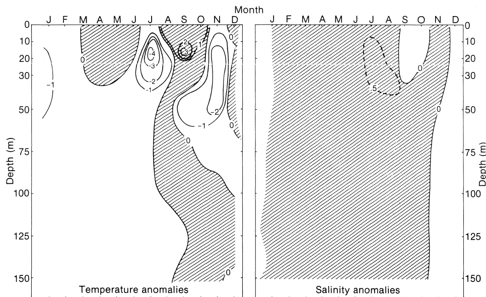
Fig. 8. Monthly temperature and salinity anomalies at Station 27 off St. John's during 1988 relative to the 1946-77 means (Keeley, 1981). (Shaded areas represent positive anomalies).
