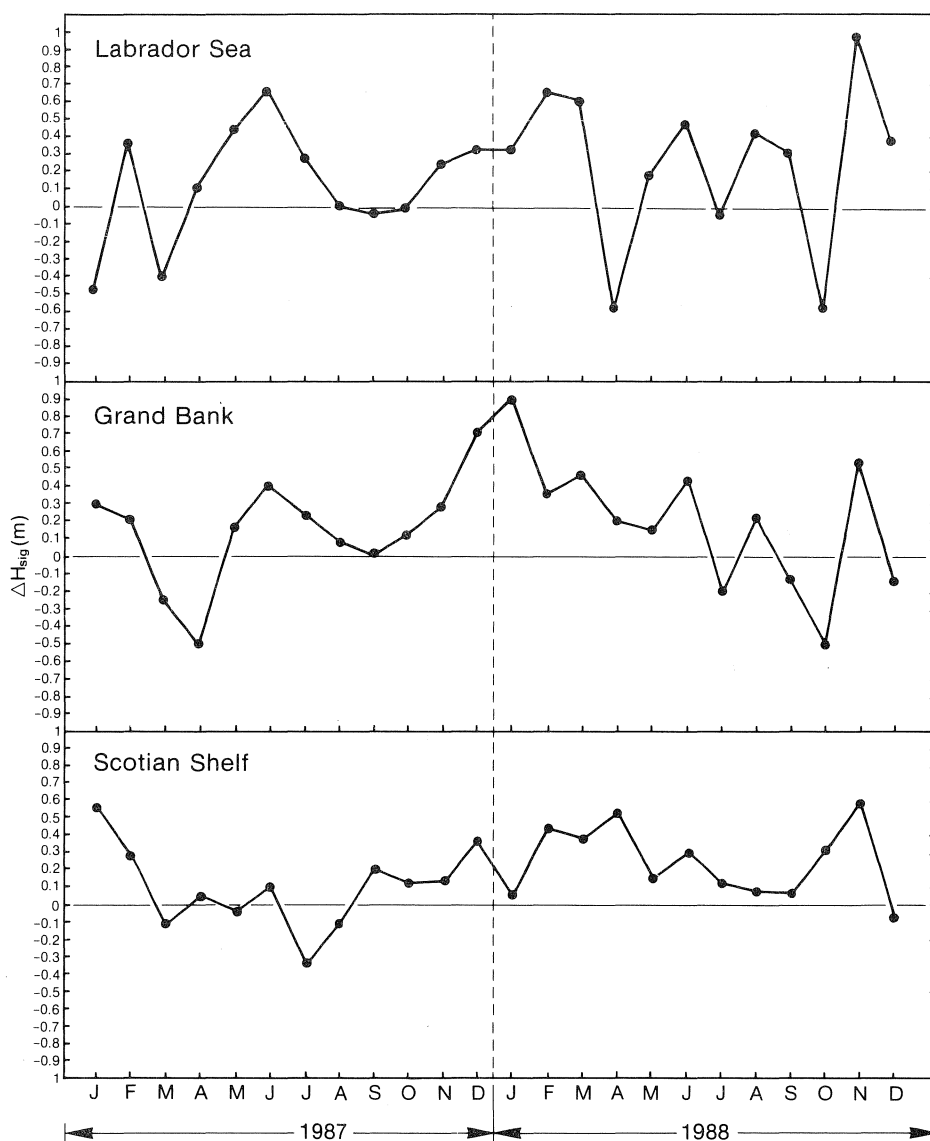
Fig. 11. Monthly significant wave heights ( \Delta H_{sig} ) in three regions of the Northwest Atlantic during 1987 and 1988 relative to the 1970-80 means.
