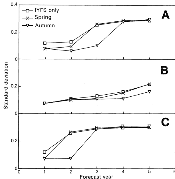
Fig. 2. Standard deviation of forecast quantity plotted against forecast year, for three possible scenarios of recruitment survey availability ( A — Log yield; B — Log spawning stock biomass; C — Log total stock biomass). The standard deviation is approximately equal to the coefficient of variation.
