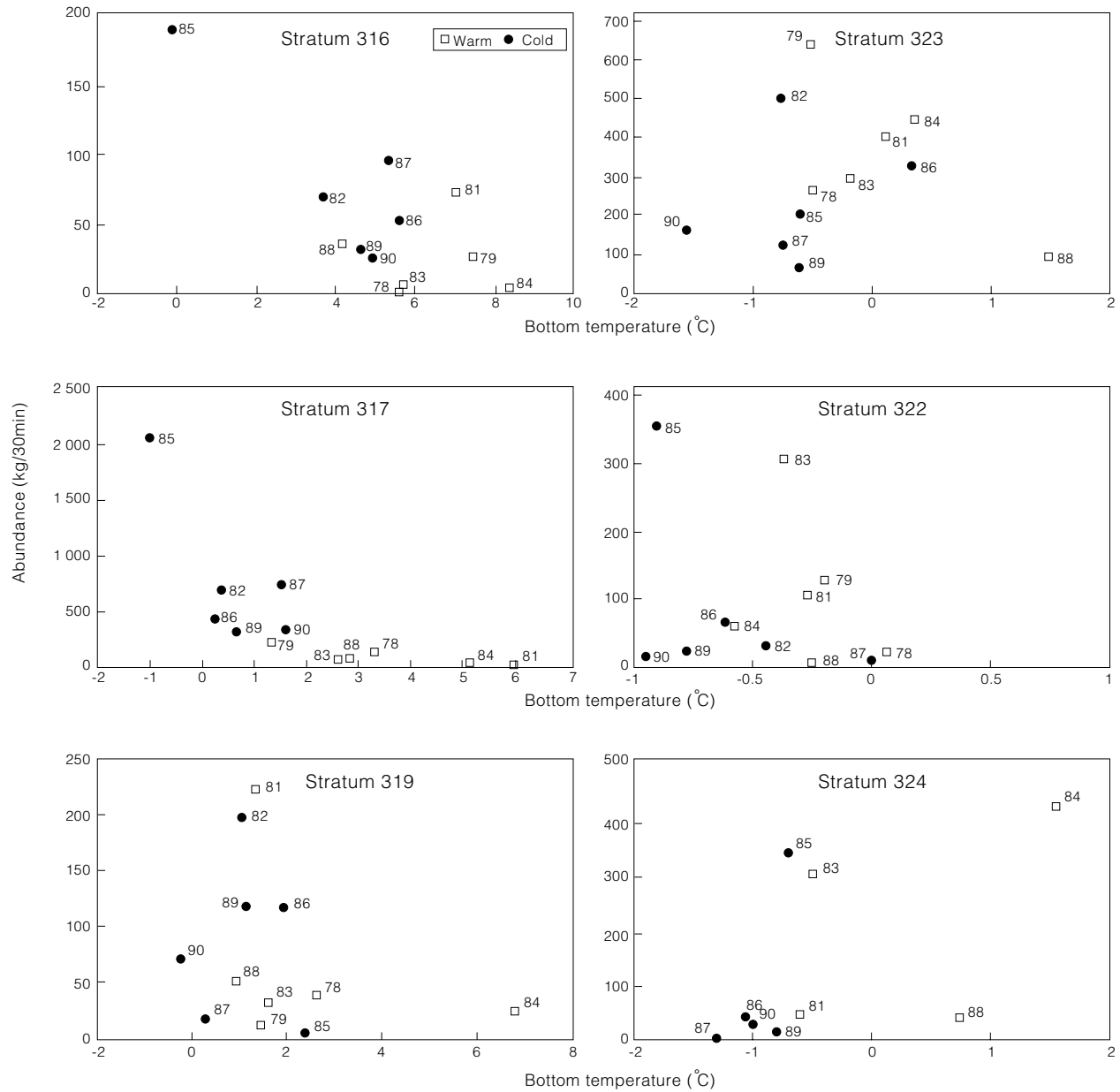
Fig. 5. Relationships between bottom temperature (average for the stratum) and average catch per tow (kg/30 min) for American plaice in strata 316, 317, 319, 323, 322 and 324 from 1978 to 1990 (1980 excluded).
