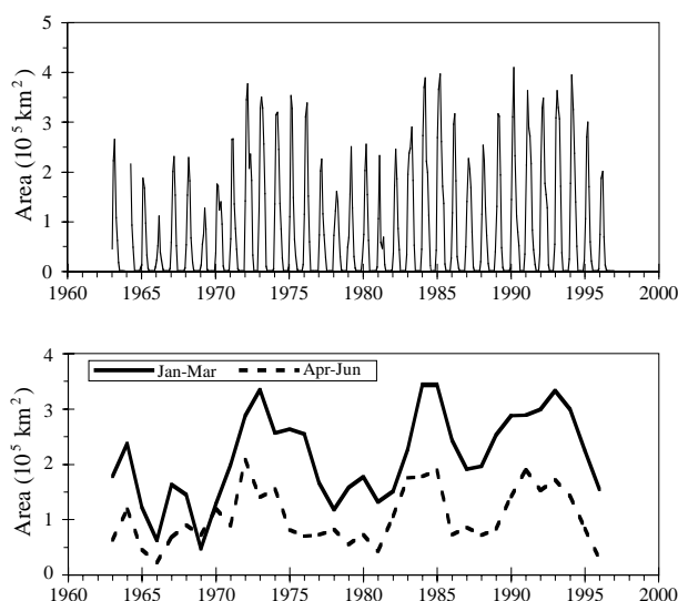
Fig. 14. The time series of the mean ice area by month (top panel) and during ice advance (Jan–Mar) and ice retreat (Apr–June) on the southern Labrador and Newfoundland shelves.
