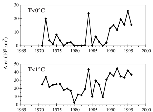
Fig. 31. Area of the Magdalen Shallows with bottom temperatures <0^{\circ}\text{C} and <1^{\circ}\text{C} during September.
