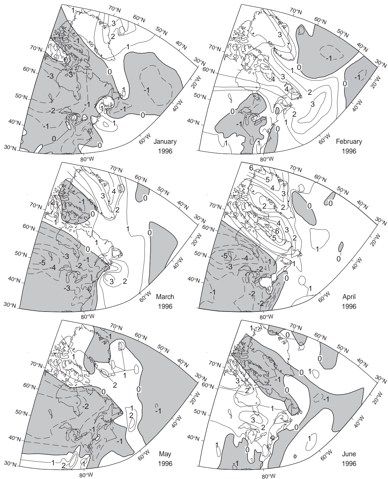
Fig. 2. Monthly air temperature anomalies (in °C) over the northwest Atlantic in 1996 relative to the 1961–90 means (from Grosswetterlagen Europas ). The shaded anomalies indicate areas of below normal temperatures.
