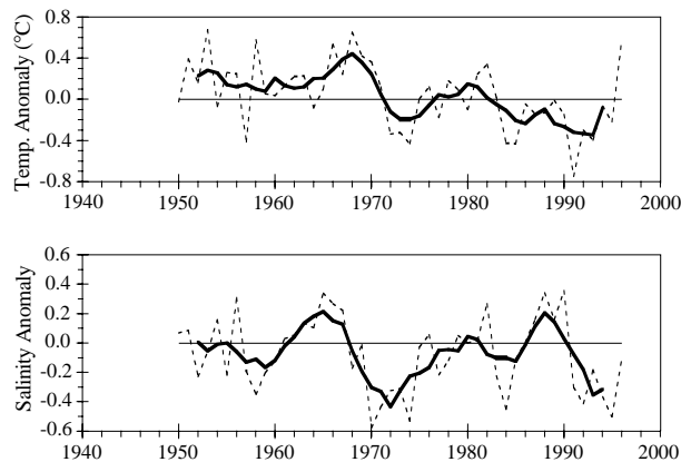
Fig. 21. Vertically-averaged temperature (0–176 m) and salinity (0–50) anomalies from Station 27. The annual values are designated by the lighter dashed line and the 5-yr running means by the heavy solid line.
