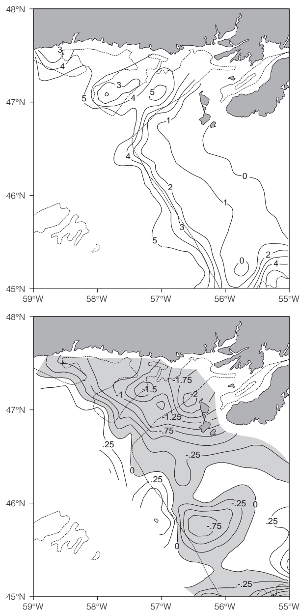
Fig. 27. The horizontal distribution of bottom temperature off southern Newfoundland during April. Temperatures are in the top panel and their anomalies are on the bottom panel. Negative anomalies, indicating cooler-than-normal temperatures, are shaded.
