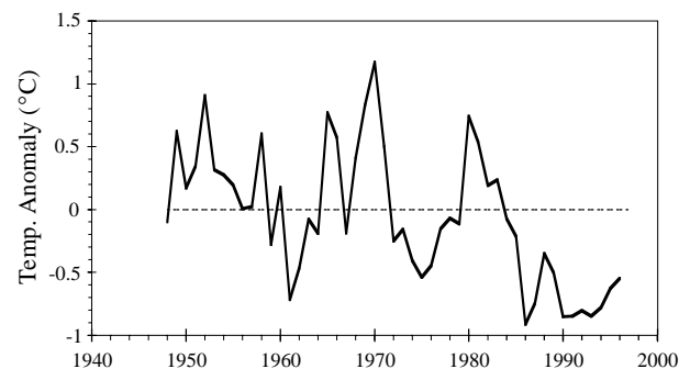
Fig. 29. Anomalies of the CIL core temperatures (extrapolated to July 15) for the Gulf of St. Lawrence relative to the 1948–94 mean (of 0.08^{\circ}\text{C} ).
