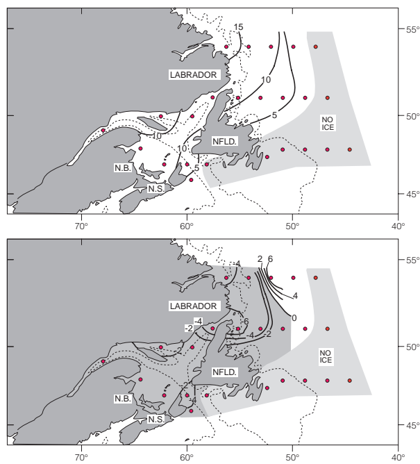
Fig. 13. The duration of sea ice during the winter of 1996 (top panel) and their anomalies from the long-term mean in weeks (bottom panel). The shaded negative anomaly indicates ice duration was less-than-normal which is generally associated with a warmer year.
