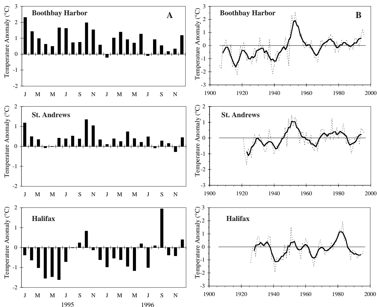
Fig. 33. Monthly sea surface temperature anomalies during 1995 and 1996 (left) and the annual temperature anomalies (right, dashed line) and their 5 year running means (solid line) for Boothbay Harbor, St. Andrews and Halifax.
