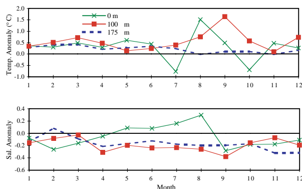
Fig. 19. Monthly temperature (top panel) and salinity (bottom panel) anomalies at 0, 100 and 175 m at Station 27 during 1996.
