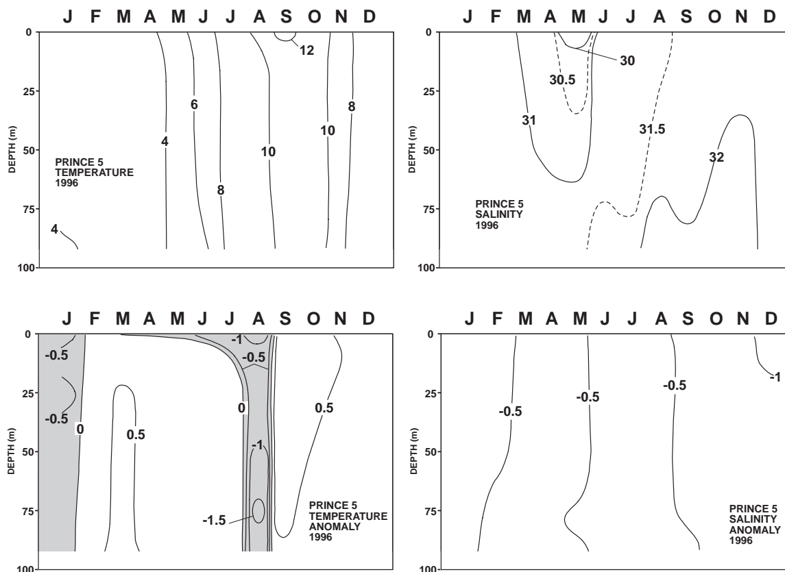
Fig. 34. Monthly mean temperatures and salinities and their anomalies at Prince 5 as a function of depth during 1996. Negative anomalies (cooler, fresher) are shaded.
