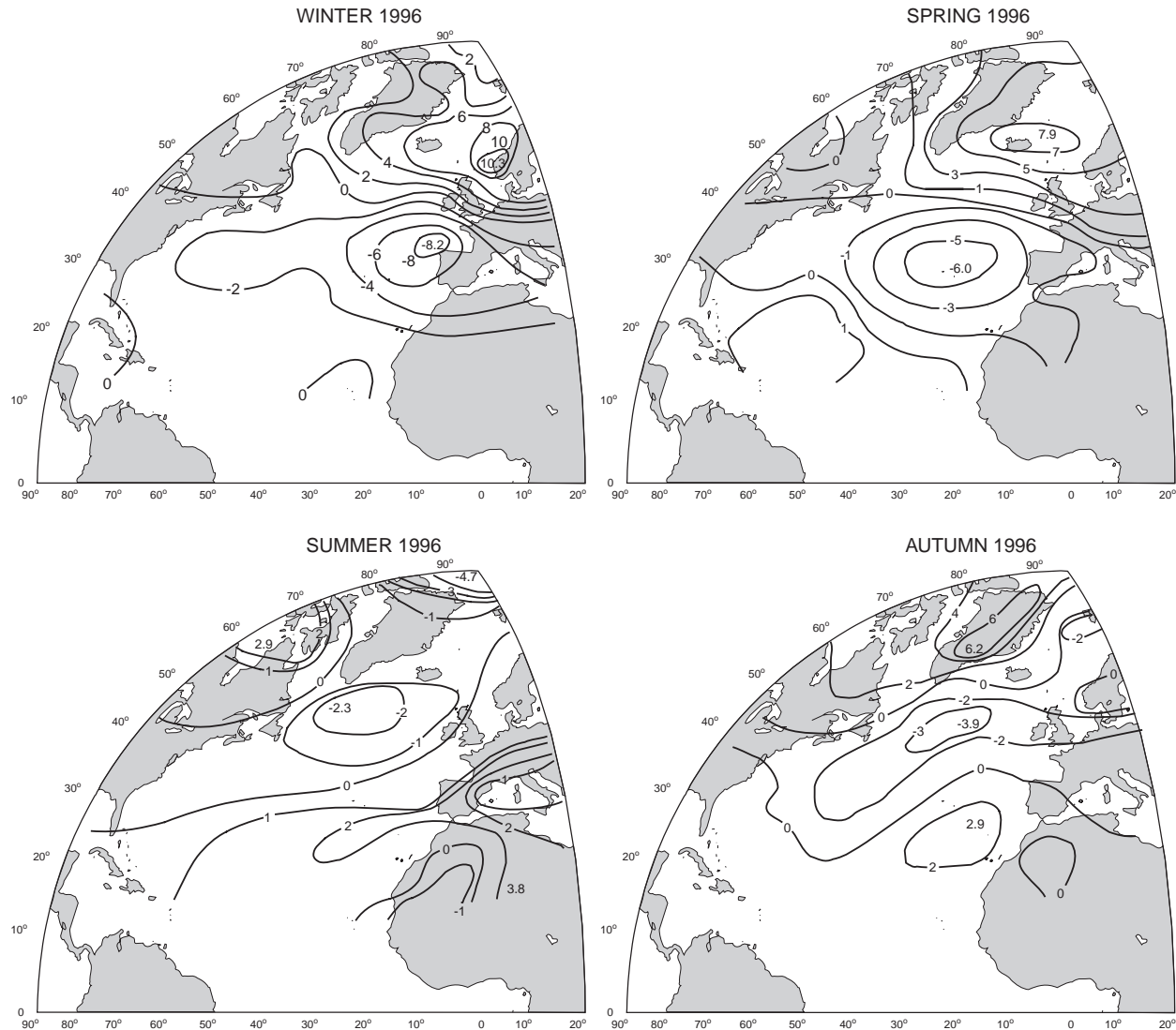
Fig. 7. Seasonal sea-surface air pressure anomalies (mb) over the North Atlantic in 1996.
