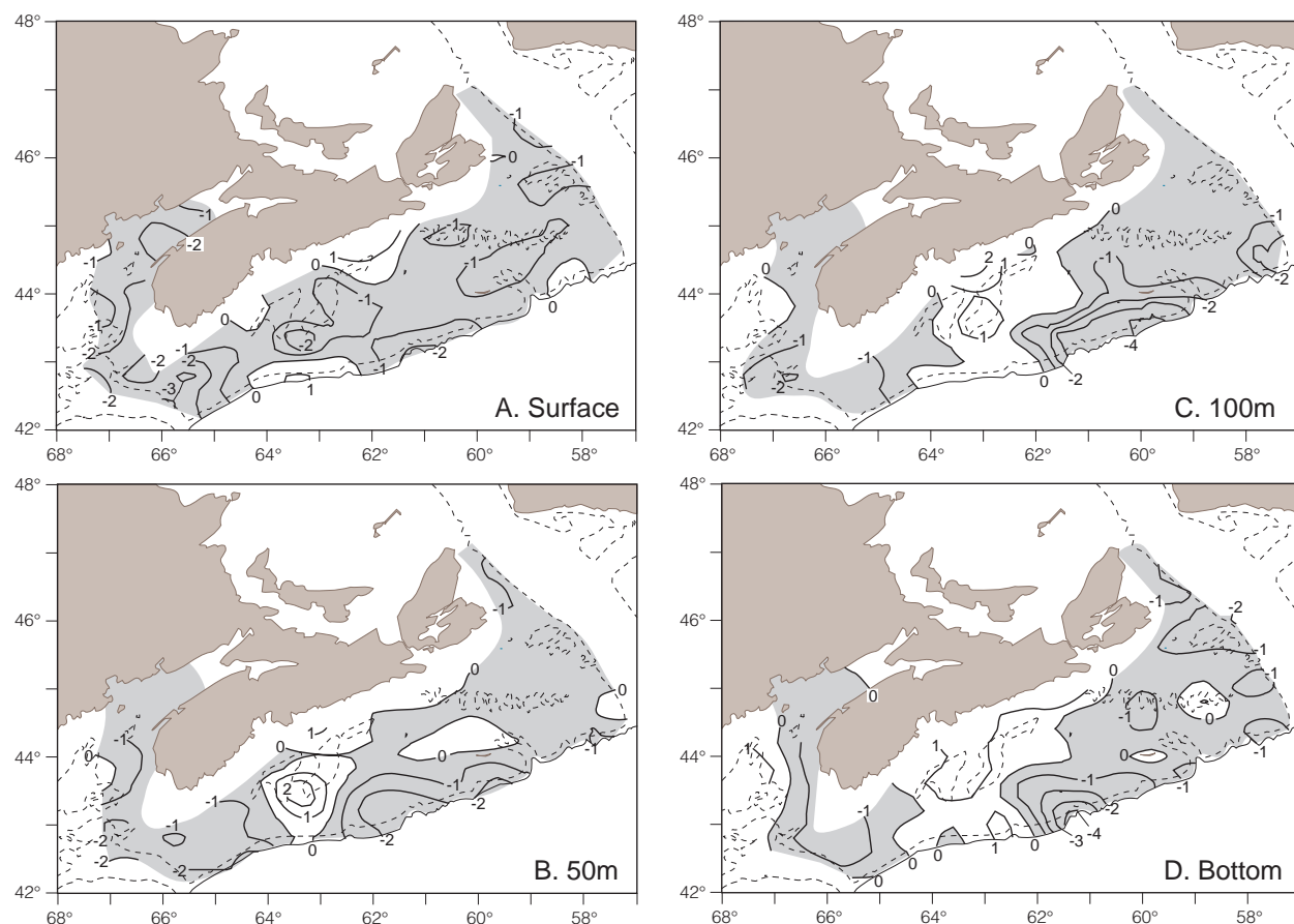
Fig. 44. Contours of temperature anomaly at different depths calculated from data taken during the 1996 Canadian July groundfish survey. Negative anomalies are shaded.
