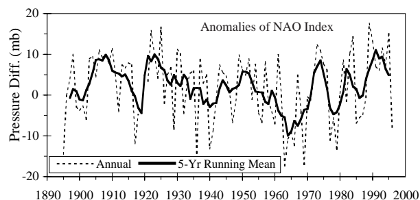
Fig. 8. Anomalies of the North Atlantic Oscillation Index.
