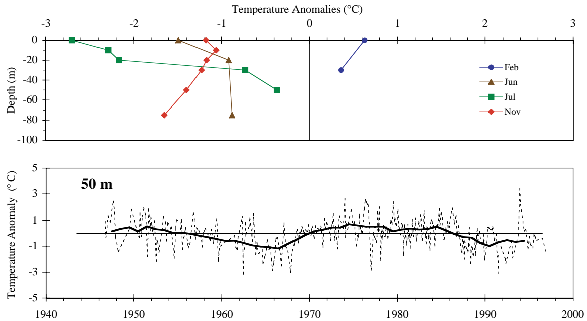
Fig. 42. The 1996 monthly temperature anomaly profiles (top panel) and temperature anomaly time series at 50 m (bottom panel) for Lurcher Shoals (area 24 in Fig. 39).
