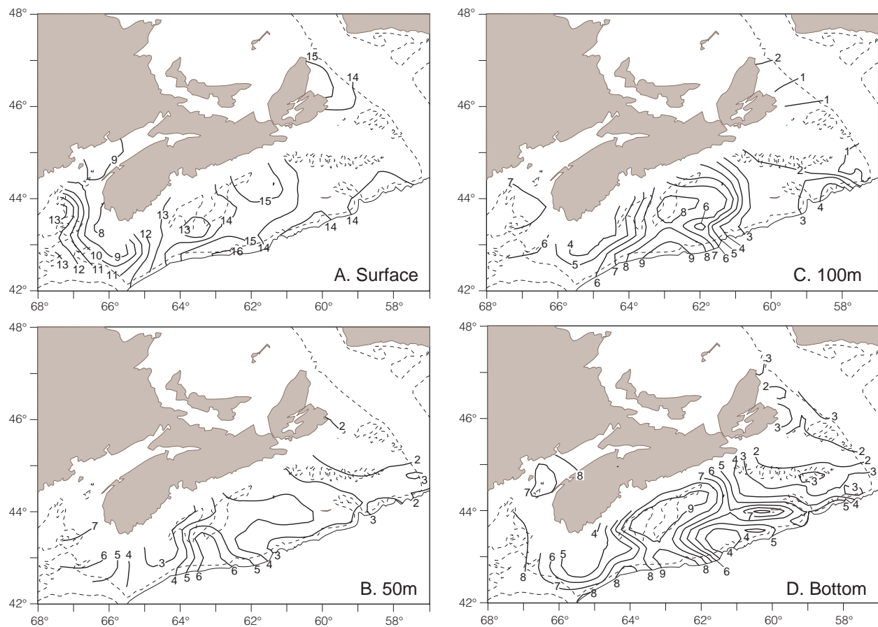
Fig. 43. Contours of temperature at different depths calculated from data collected during the 1996 Canadian July groundfish survey.
