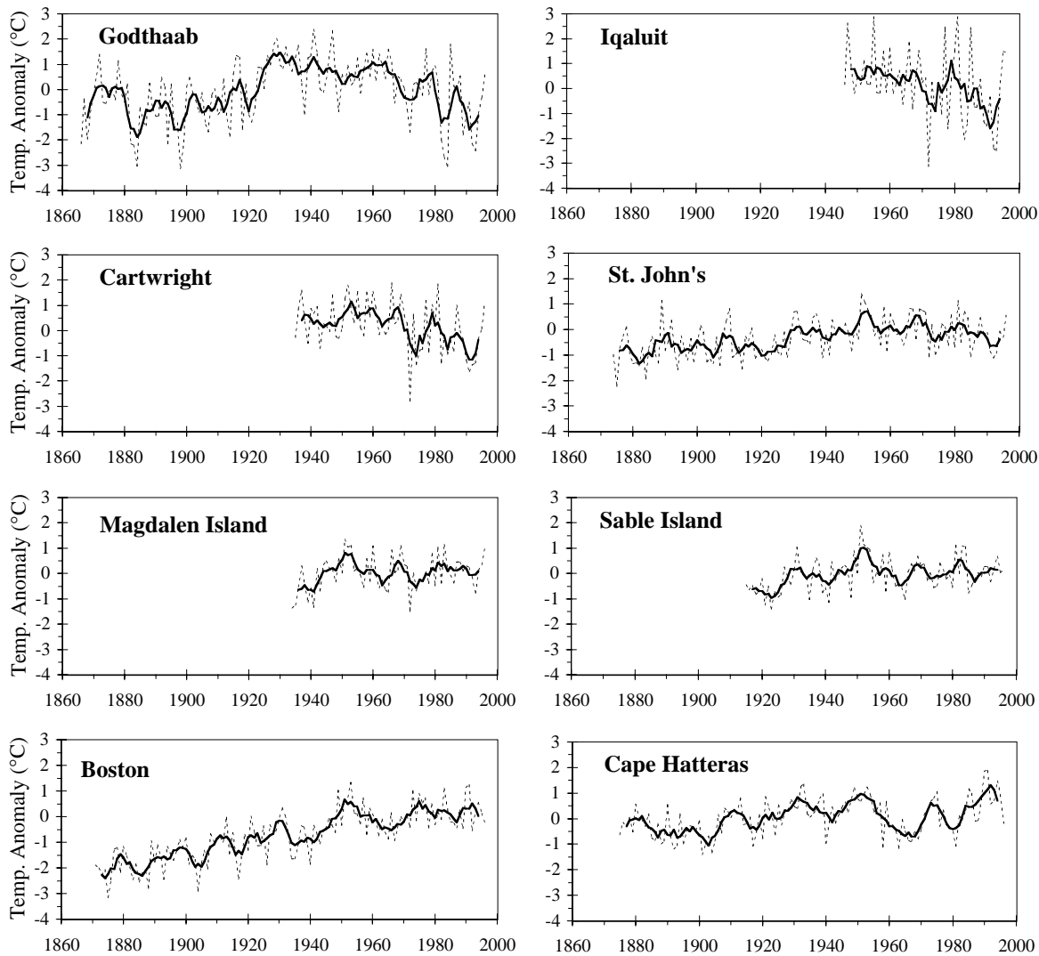
Fig. 5. Annual (dashed) and 5-year running (solid) means of the air temperature anomalies at selected sites.
