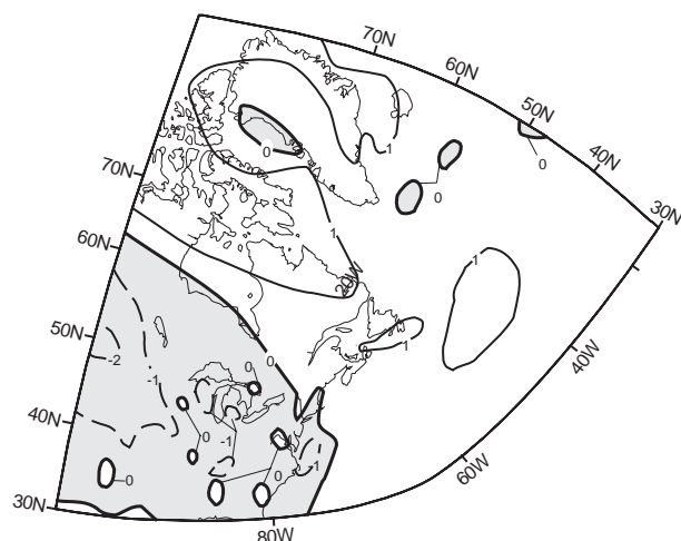
Fig. 1. The annual air temperature anomalies ( ^{\circ}\text{C} ) over the northwest Atlantic in 1996 relative to the 1961–90 means (taken from Grosswetterlagen Europas ). The shaded anomalies indicate areas of below normal temperatures.
