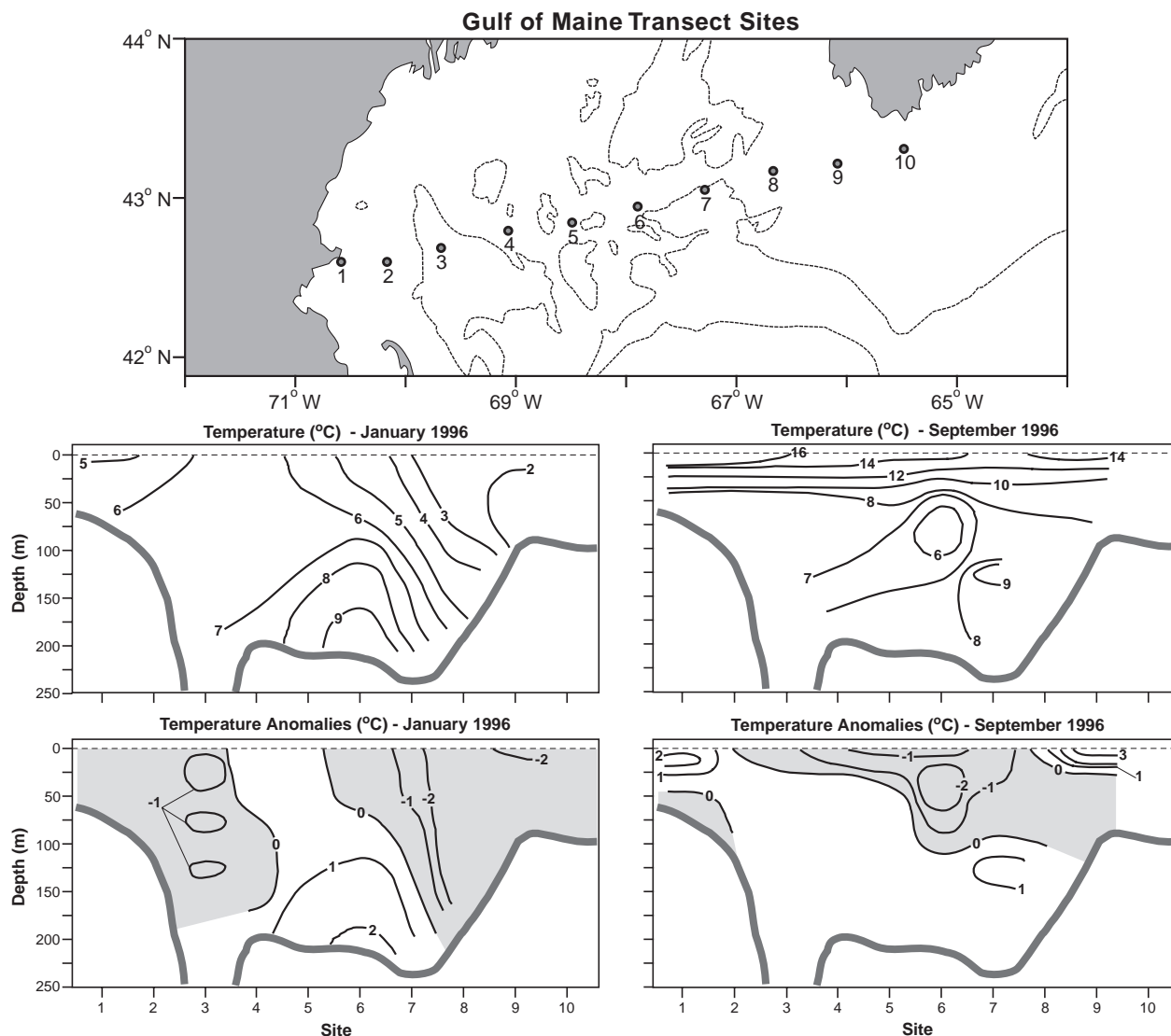
Fig. 37. The temperature (middle panels) and temperature anomalies (bottom panels) in °C along a XBT transect (top panel) across the Gulf of Maine during January and September 1996.
