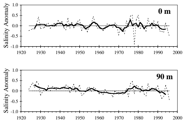
Fig. 36. Annual and 5 yr running means of salinity anomalies at Prince 5, 0 and 90 m.
