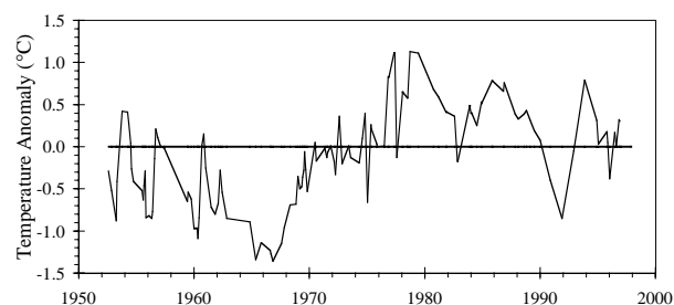
Fig. 28. Anomalies in the average temperature in the 200–300 m layer in Cabot Strait.
