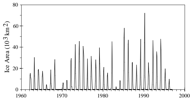
Fig. 17. Time series of the monthly mean area of sea ice seaward of Cabot Strait.
