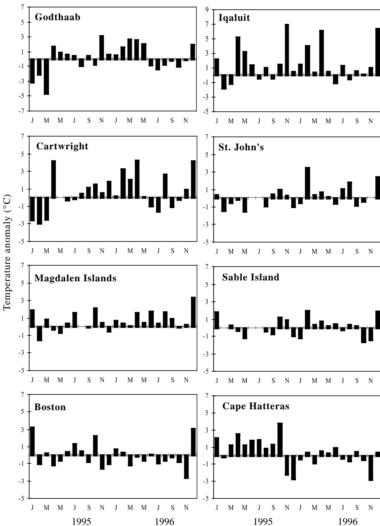
Fig. 4. Monthly air temperature anomalies in 1995 and 1996 at selected coastal sites (see Fig. 3 for locations).
