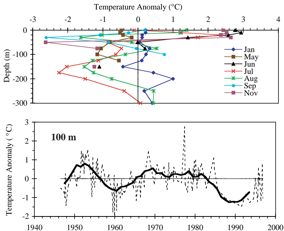
Fig. 40. The 1996 monthly temperature anomaly profiles (top panel) and temperature anomaly time series at 100 m (bottom panel) for Sydney Bight (area 1 in Fig. 39).
