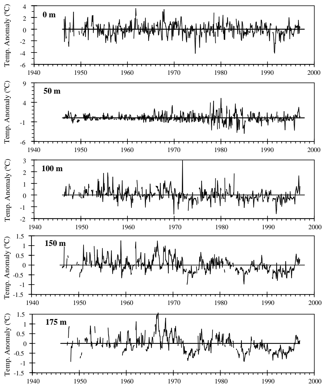
Fig. 20. Monthly mean temperature anomalies at selected depths from Station 27.
