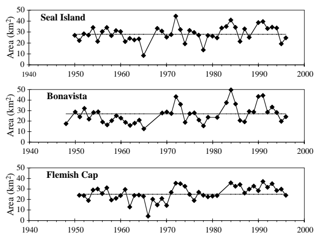
Fig. 22. The CIL cross-sectional area (in km 2 ) during the summer along transects off the Seal Island (southern Labrador), Bonavista Bay (northern Newfoundland) and Flemish Cap (Grand Banks).
