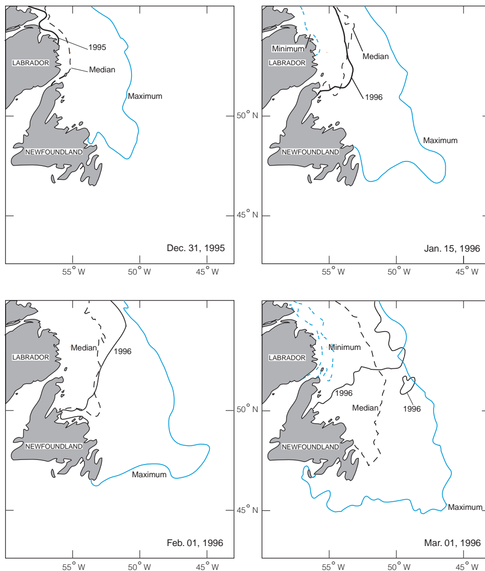
Fig. 9a. The location of the ice edge (>10% concentration) together with the historical (1962–87) minimum, median and maximum positions off Newfoundland and Labrador at selected dates between December 1995 and March 1996.
