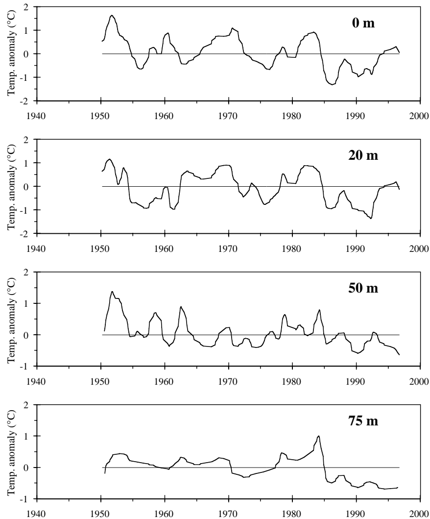
Fig. 26. Smoothed time series of temperature anomalies at standard depths over St. Pierre Bank. The apparent vertical lines in the plots are surveys conducted over a day or two and thus reflect both spatial and temporal variability over the Bank.
