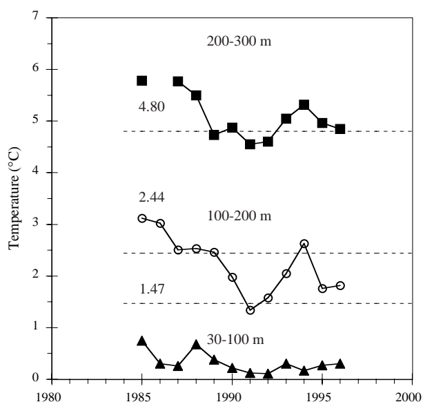
Fig. 32. Temperatures in the 30–100 m, the 100–200 m and the 200–300 m layers in the Gulf of St. Lawrence during August–September. The dashed lines indicate the long-term averages based on Petrie et al. (1996a).
