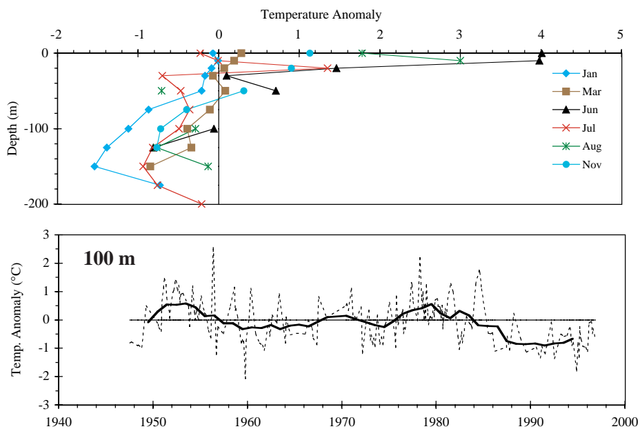
Fig. 41. The 1996 monthly temperature anomaly profiles (top panel) and temperature anomaly time series at 100 m (bottom panel) for Misaine Bank (area 5 in Fig. 39).
