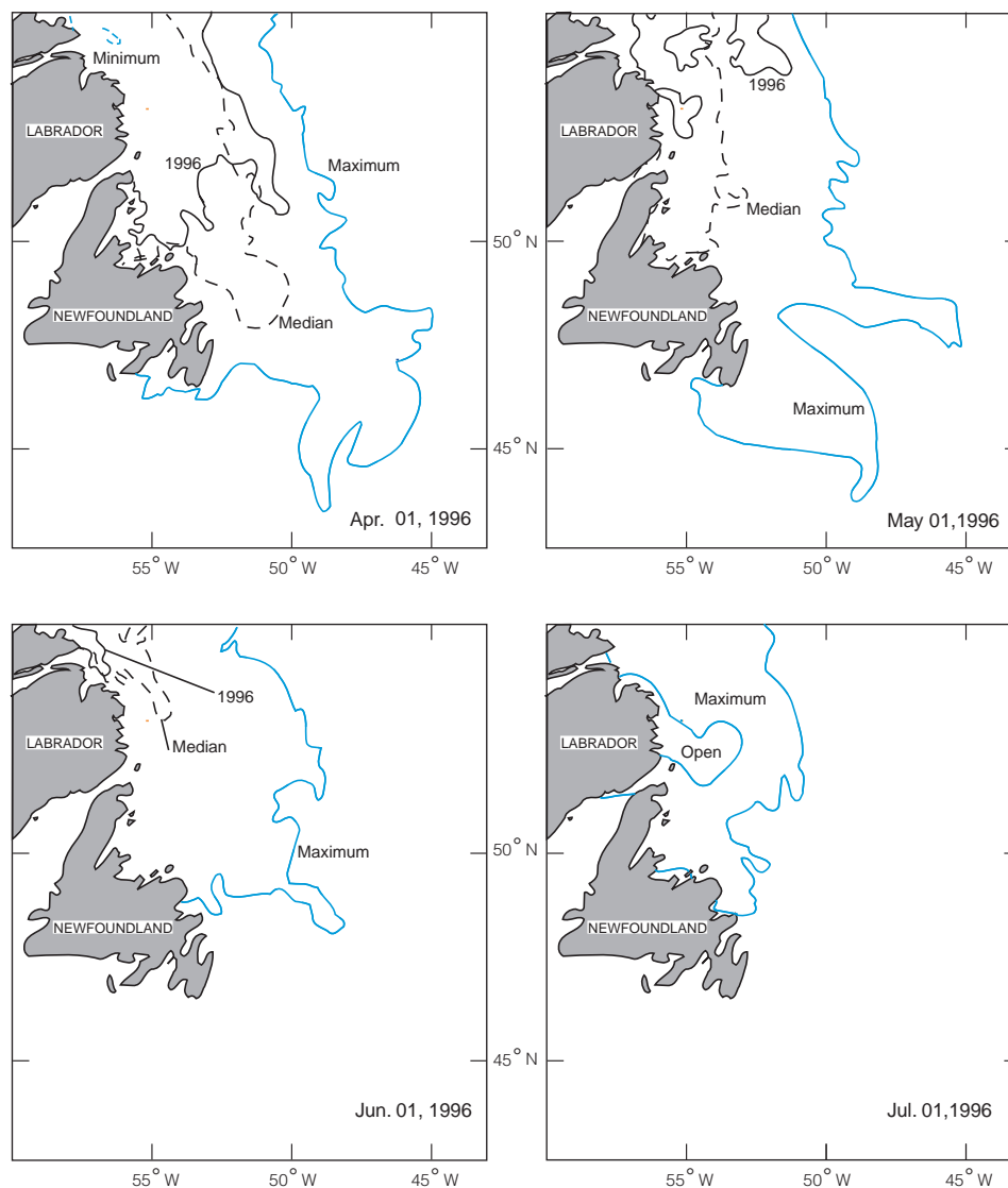
Fig. 9b. The location of the ice edge (>10% concentration) together with the historical (1962–87) minimum, median and maximum positions off Newfoundland and Labrador at selected dates between April and July 1996.
