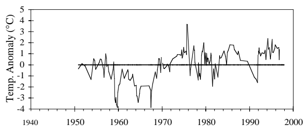
Fig. 38. Temperature anomalies in Emerald Basin at 250 m. The mean temperature is 8.5°C.
