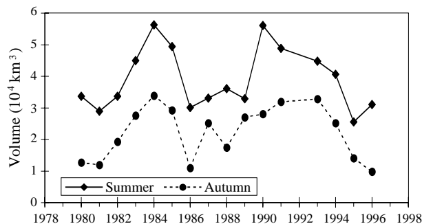
Fig. 23. The CIL volume in the summer and autumn within Div. 2J and 3KL.
