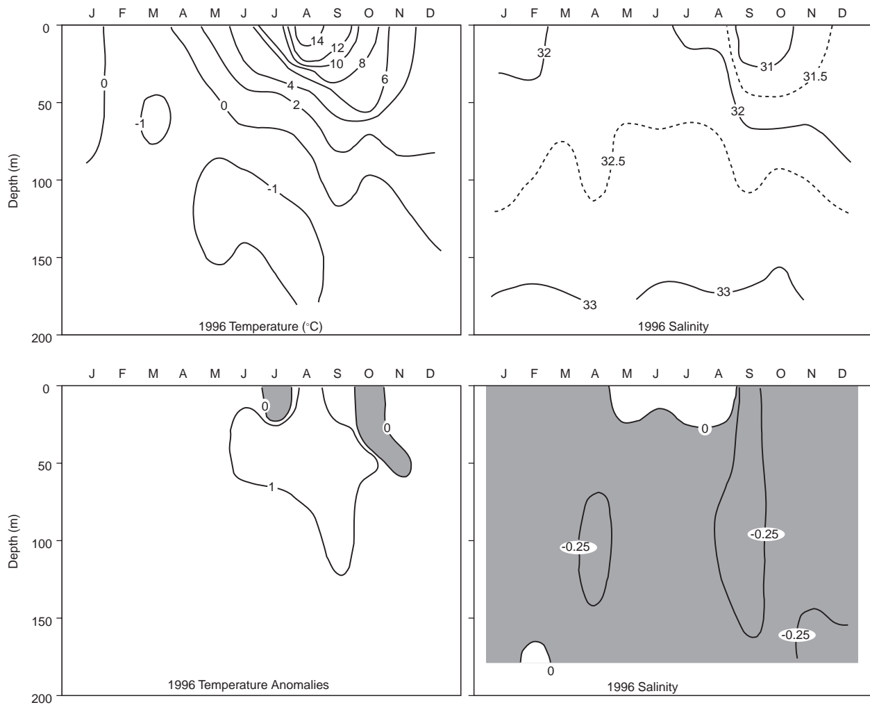
Fig. 18. The monthly mean and anomalies of temperature and salinity at Station 27. The negative (cold, fresher) anomalies are shaded.
