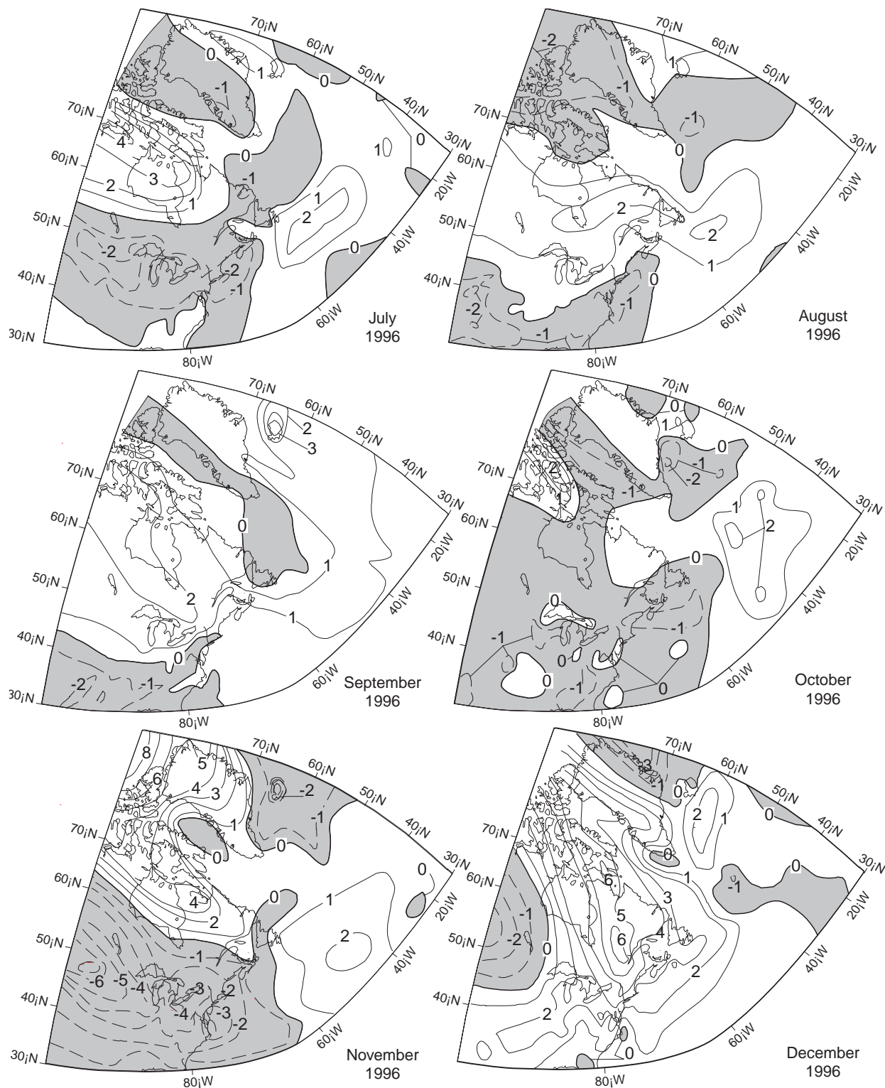
Fig. 2. (Continued). Monthly air temperature anomalies (in °C) over the northwest Atlantic in 1996 relative to the 1961–90 means (from Grosswetterlagen Europas ). The shaded anomalies indicate areas of below normal temperatures.
