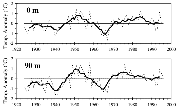
Fig. 35. Annual and 5 yr running means of temperature anomalies at Prince 5, 0 and 90 m.
