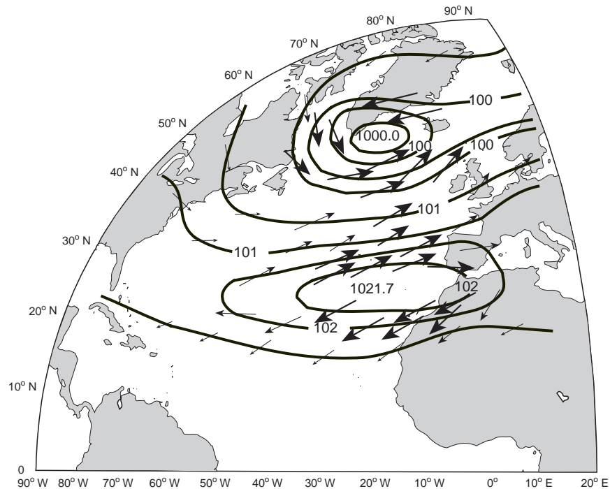
Fig. 6. The long-term (1961–90) mean sea surface pressures during winter (average of December, January and February). A schematic of the wind field associated with the mean pressure is also shown.
