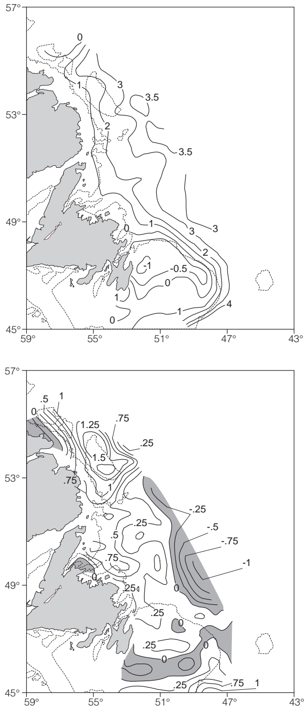
Fig. 24. Horizontal distribution of bottom temperature off Labrador and Newfoundland in autumn. Temperatures are in the top panel and their anomalies are in the bottom panel. Negative anomalies, indicating colder-than-normal temperatures, are shaded.
