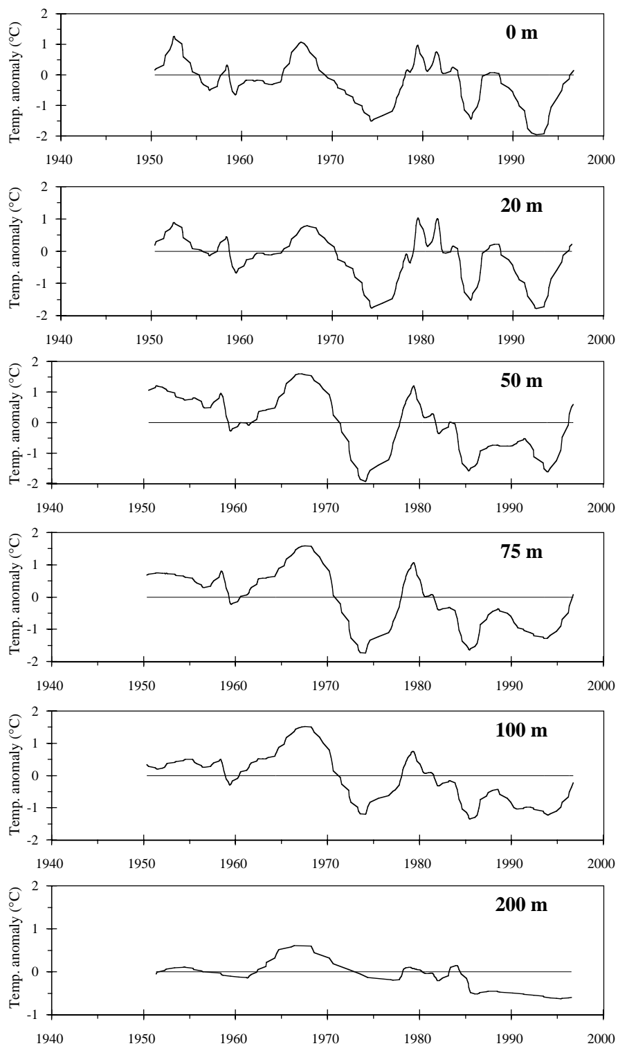
Fig. 25. Smoothed time series of temperature anomalies at standard depths over Flemish Cap.
