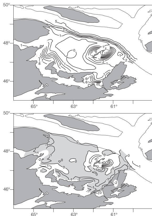
Fig. 30. Temperature (top panel) and temperature anomalies (bottom panel) in the southern Gulf of St. Lawrence in September 1996. Contours are in ^{\circ}\text{C} and negative anomalies are shaded.
