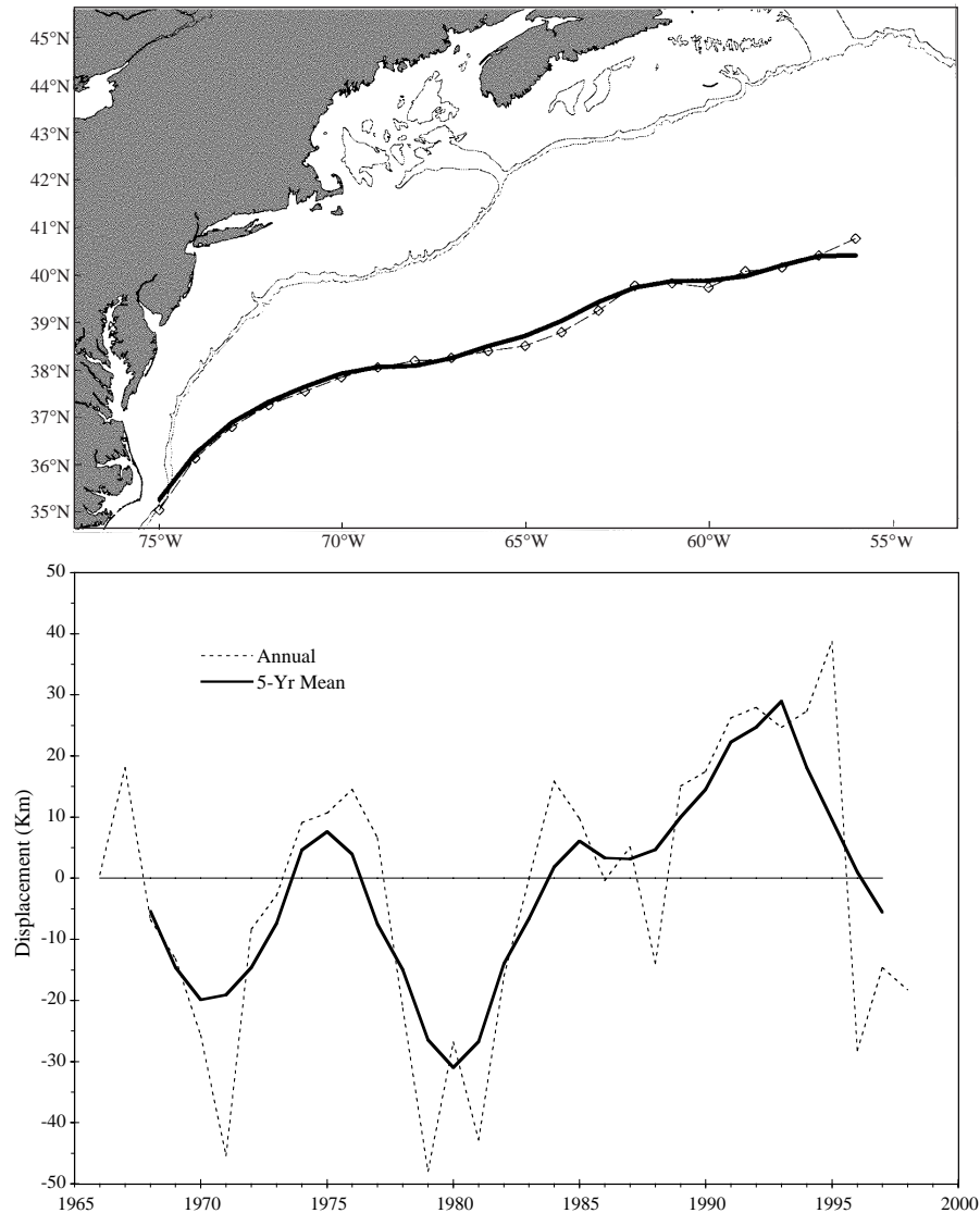
Fig. 50. The 1998 (dashed line) and long-term (1973–97; solid line) mean positions of the northern edge of the Gulf Stream (top panel) and the annual mean anomaly of the average (55°–75°W) position of the Gulf Stream front (bottom panel).
