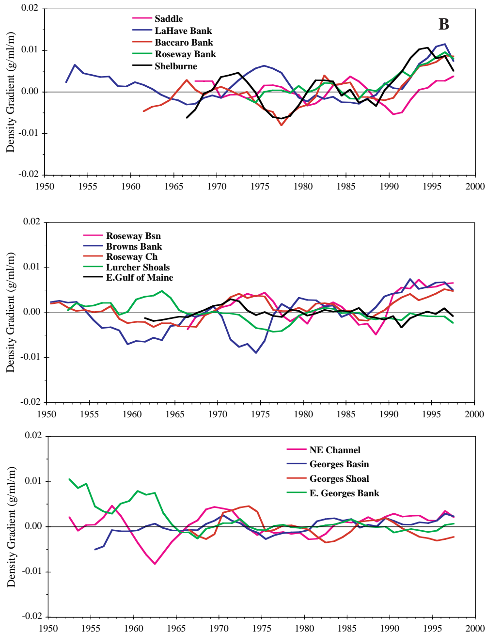
Fig. 48b. Five-year running means of the annual anomalies of the density gradient between the surface and 50 m calculated for the areas 16–29 in Fig. 41.
