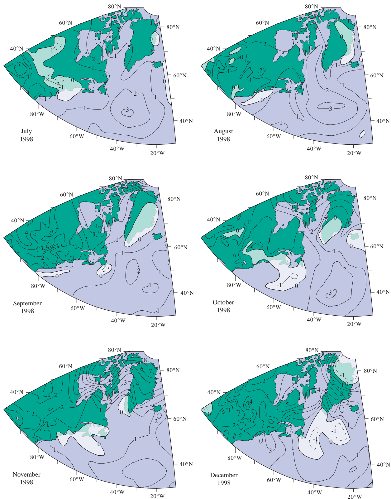
Fig. 2. (Continued). Monthly air temperature anomalies (°C) over the Northwest Atlantic and eastern Canada in 1998 relative to the 1961–90 means (from Grosswetterlagen Europas). Lighter coloured areas (dashed lines) are colder-than-normal.
