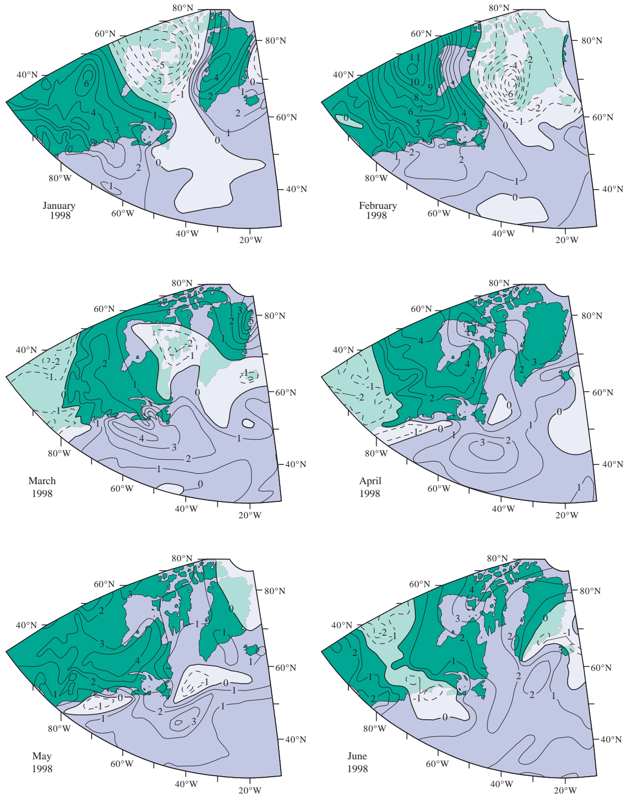
Fig. 2. Monthly air temperature anomalies ( ^{\circ}\text{C} ) over the Northwest Atlantic and eastern Canada in 1998 relative to the 1961–90 means (from Grosswetterlagen Europas). Lighter coloured areas (dashed lines) are colder-than-normal.
