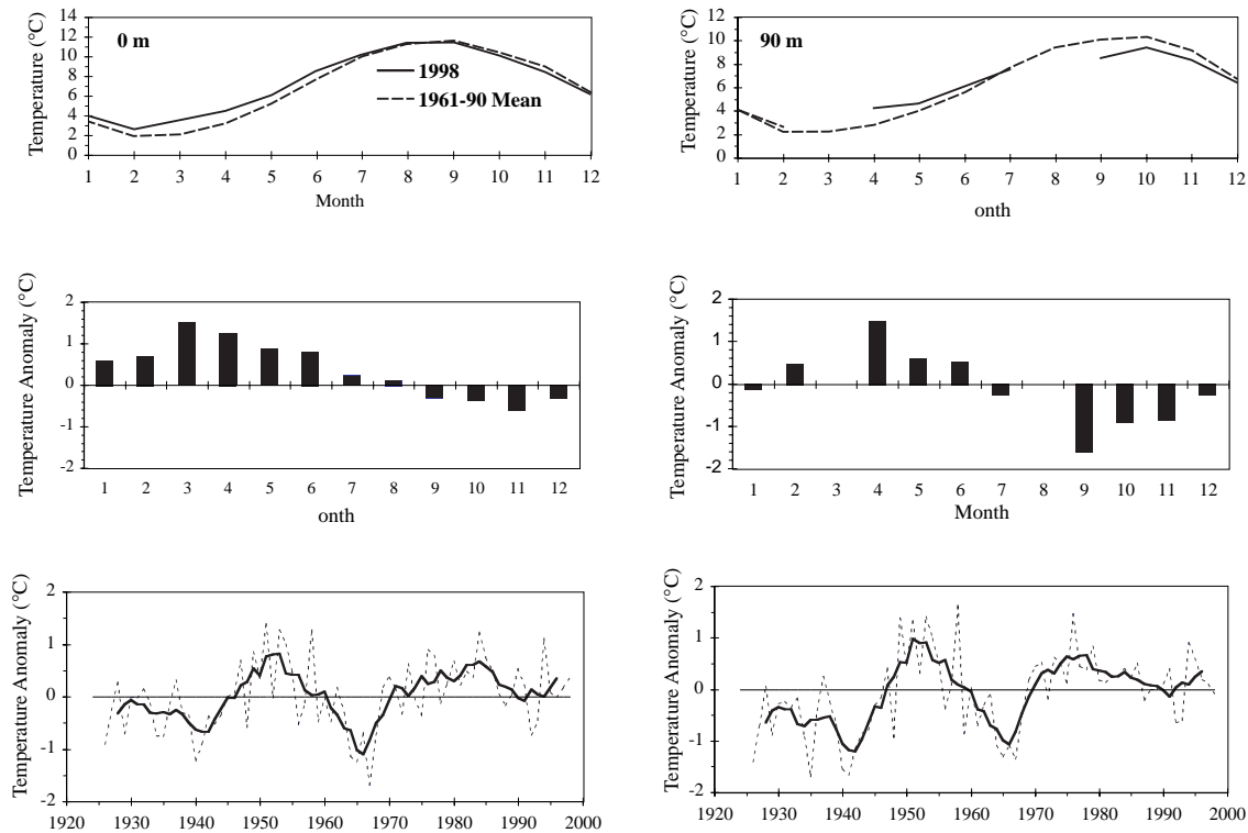
Fig. 37. The long-term (1961–90) and 1998 monthly mean temperatures (top panels), the 1998 monthly anomalies (middle panels) and in the bottom panels the time series of the annual mean anomalies (dashed line) and their 5-year running means (solid line) for Prince 5, 0 m (left) and 90 m (right).
