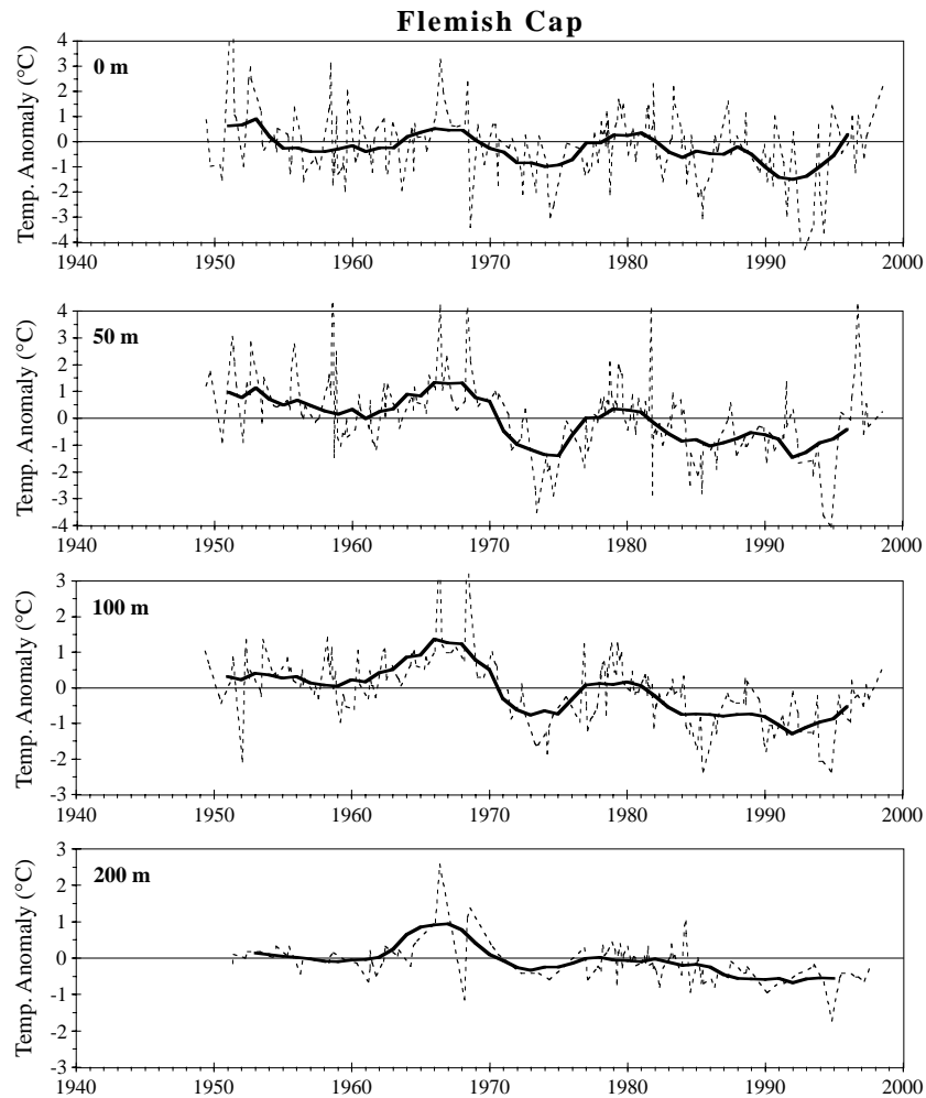
Fig. 26. Monthly (dashed) and 5-year running means (solid line) of temperature anomalies for different depths on Flemish Cap in Div. 3M.
