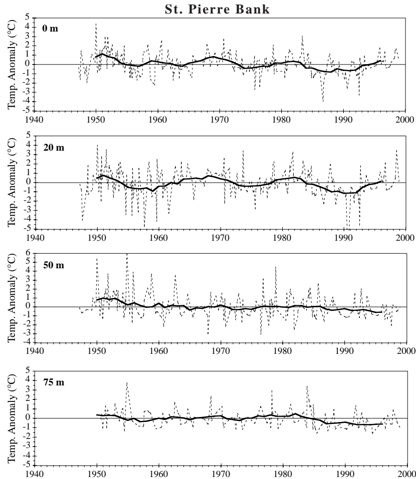
Fig. 28. Monthly (dashed) and 5-year running means (solid line) of temperature anomalies for different depths on St. Pierre Bank.
