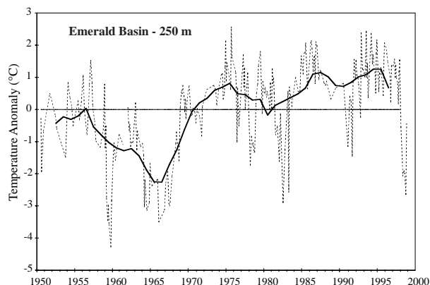
Fig. 40. Temperature anomalies (relative to 1961–90) in Emerald Basin at 250 m.
