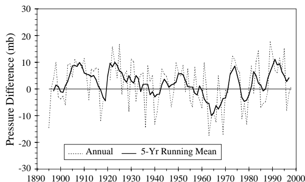
Fig. 8. Annual and 5-year running means of the anomalies of the North Atlantic Oscillation Index.
