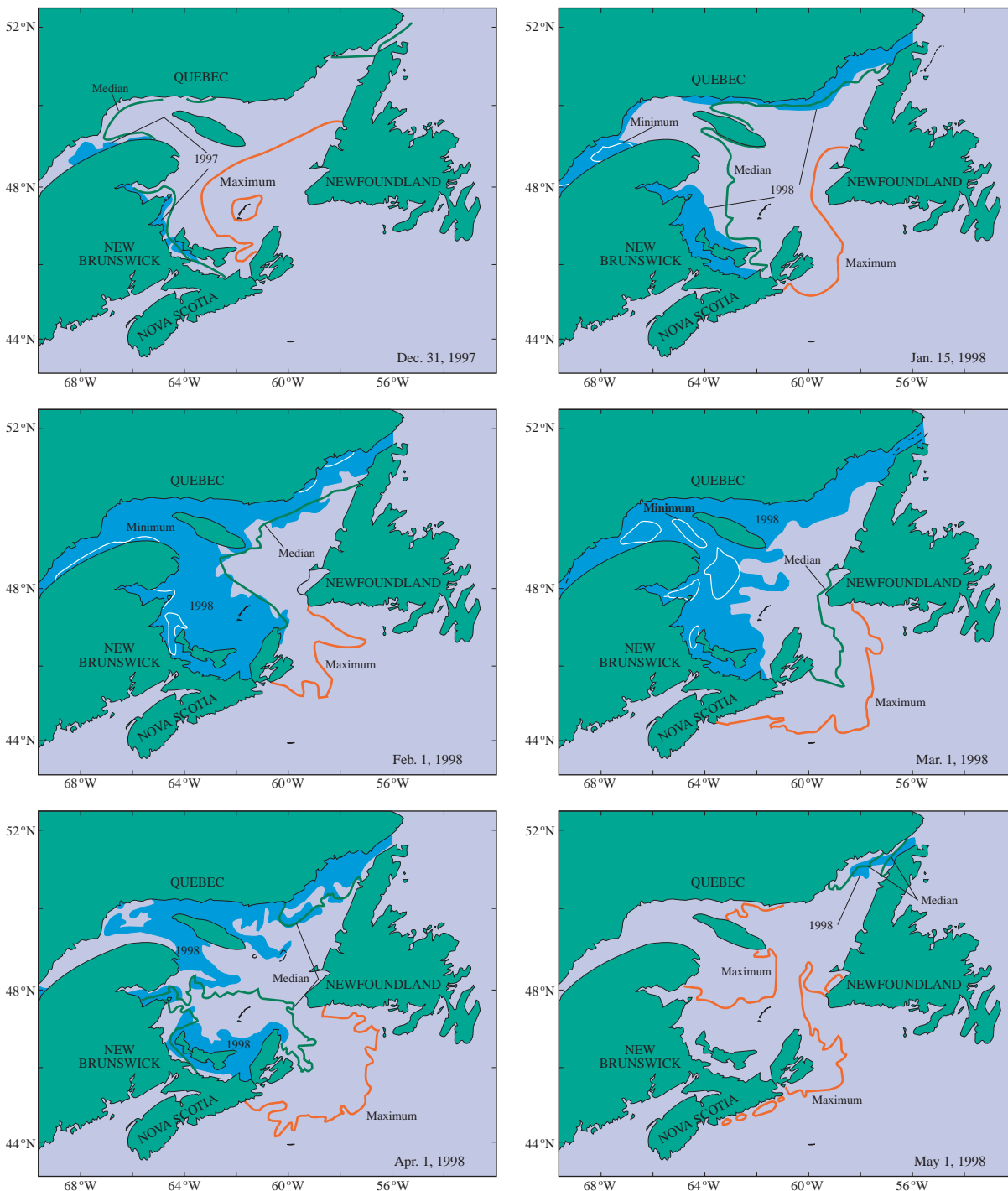
Fig. 15. The area of sea ice (>10% concentration) together with the historical (1962–87) minimum, median and maximum positions of the ice edge in the Gulf of St. Lawrence between December 1997 and May 1998.
