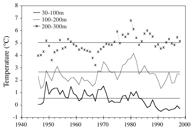
Fig. 34. Areal-weighted mean temperatures in the 30–100 m, 100–200 m, and 200–300 m layers in the Gulf of St. Lawrence during August–September. The horizontal lines indicate the 1961–90 means.
