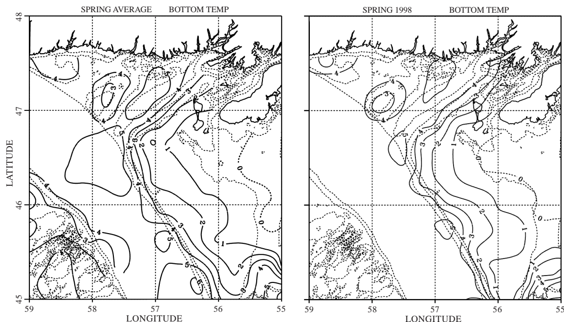
Fig. 29. Contours of the long-term (1961–90) mean and the 1998 spring bottom temperatures in Subdiv. 3Ps and 3Pn.
