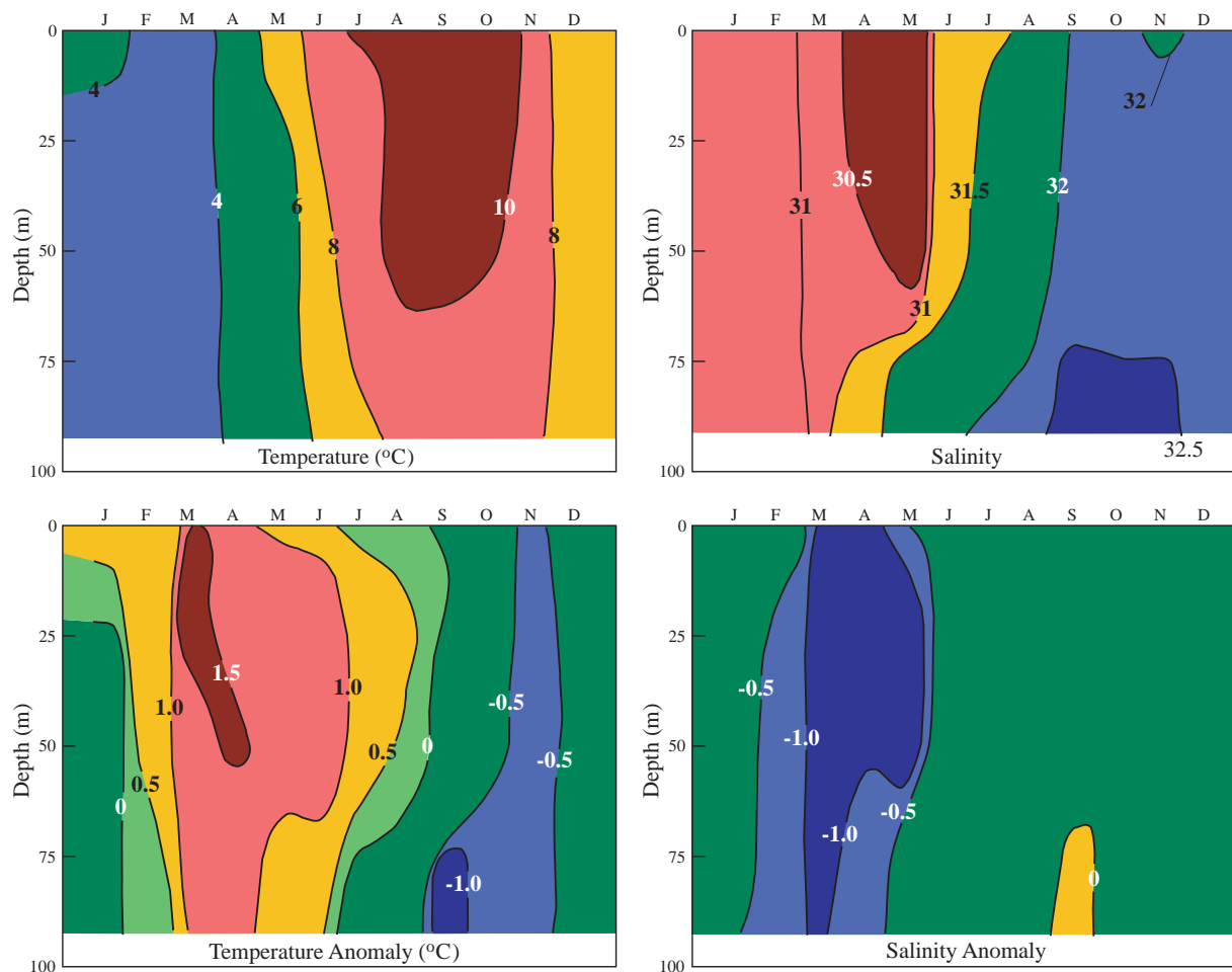
Fig. 36. Monthly mean (top panel) and anomalies relative to the 1961–90 average (bottom panel) of temperature (in °C) and salinity at Prince 5 as a function of depth during 1998.
