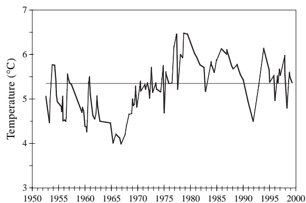
Fig. 30. The average temperature in the 200–300 m layer in Cabot Strait. The horizontal line indicates the 1961–90 mean.
