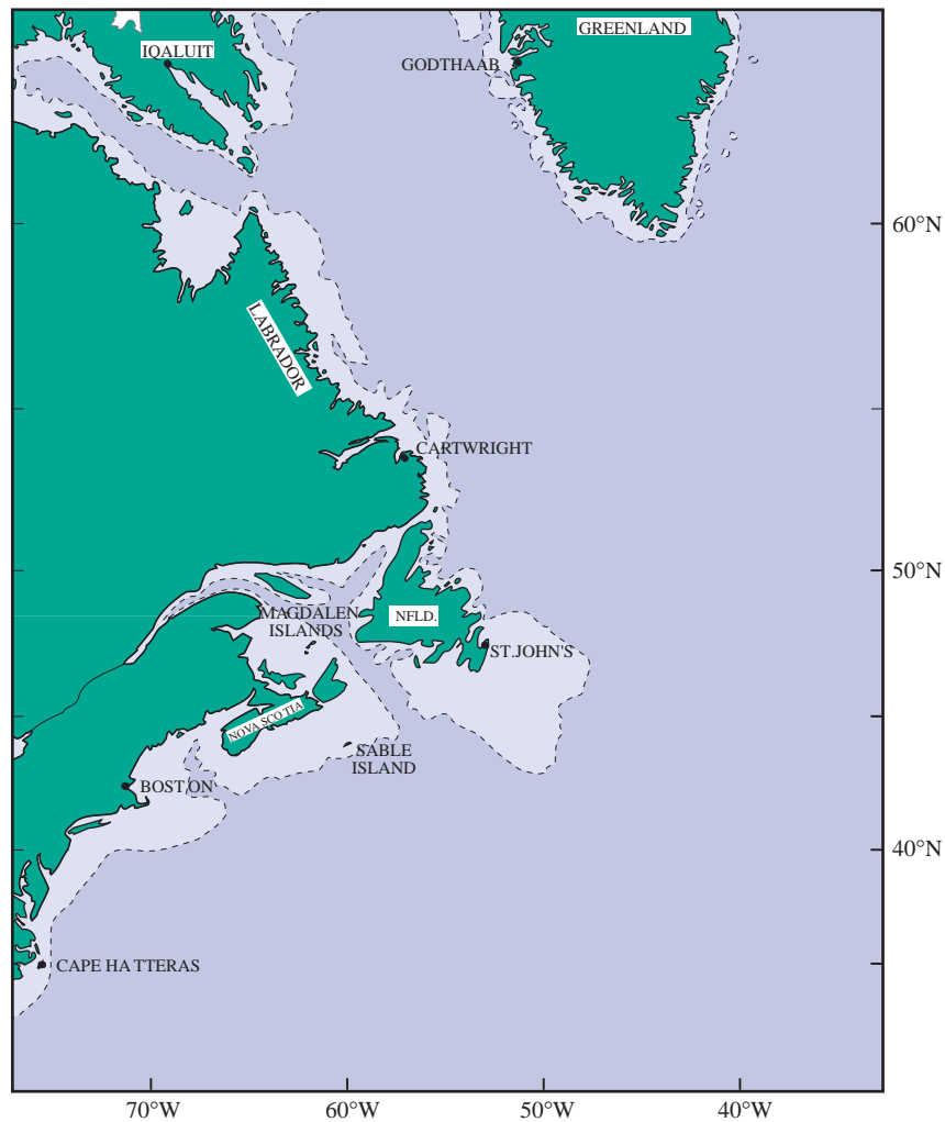
Fig. 3. Northwest Atlantic showing coastal air temperature stations. The dashed line denotes the 200 m isobath.
