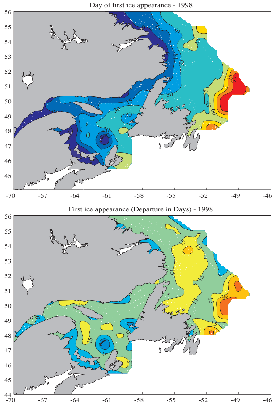
Fig. 11. The time of first presence of sea ice during 1998 measured in days from the end of 1997 (top panel) and their anomalies relative to the long term mean in days (bottom panel). White dashed lines indicate topography (200 m isobaths). Ice arriving earlier-than-normal are shaded in blue; all other colours indicate later-than-normal first presence of ice (bottom panel).
