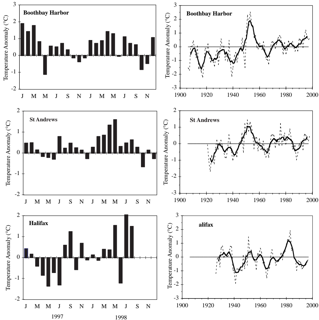
Fig. 35. The monthly sea surface temperature anomalies during 1997 and 1998 (left) and the annual temperature anomalies and their 5-year running means (right) for Boothbay Harbor, St. Andrews and Halifax. Anomalies are relative to 1961–90 means. Note no annual mean was calculated for Halifax in 1998 because of the missing data during September to December.
