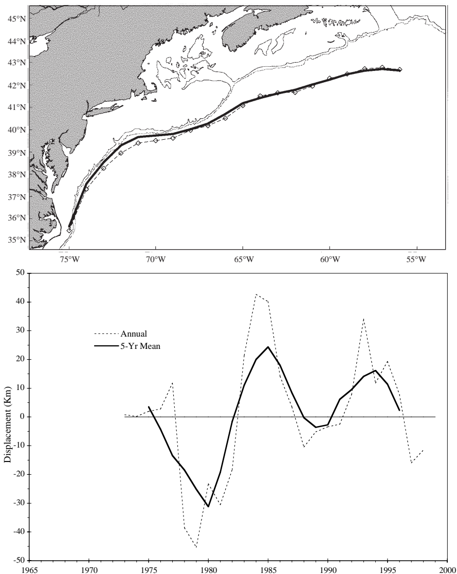
Fig. 49. The 1998 (dashed line) and long-term (1973–97; solid line) mean positions of the shelf/slope front (top panel) and the annual mean anomaly of the average (55°–75°W) position of the shelf/slope front (bottom panel).
