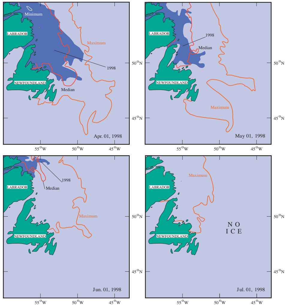
Fig. 9b. The area of sea ice (>10% concentration) together with the historical (1962–87) minimum, median and maximum positions of the ice edge off Newfoundland and Labrador between April and July 1998.
