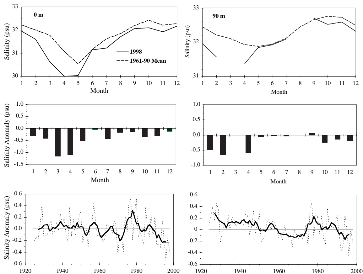
Fig. 38. The long-term (1961-90) and 1998 monthly mean salinities (top panels), the 1998 monthly anomalies (middle panels) and in the bottom panels the time series of the annual mean anomalies (dashed line) and their 5-year running means (solid line) for Prince 5, 0 m (left) and 90 m (right).
