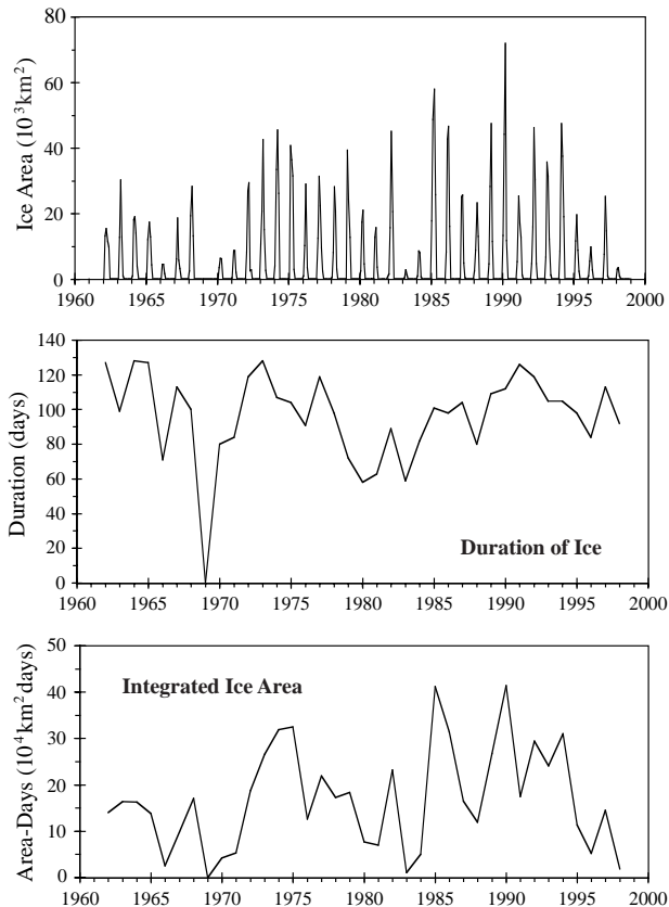
Fig. 16. The time series of the monthly mean area of sea ice (top panel), the duration of ice (middle panel) and the annual integrated ice area (summation of the area times the number of days, bottom panel) seaward of Cabot Strait.
