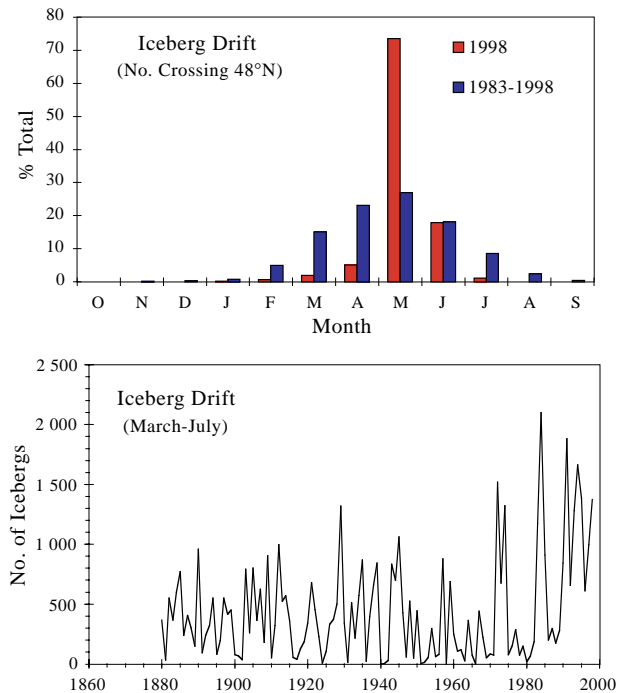
Fig. 14. The percentage of the total number of icebergs crossing south of 48°N by month during the iceberg season 1997/98 (top panel) and the number of icebergs during March to July from 1880 to 1998 (bottom panel).
