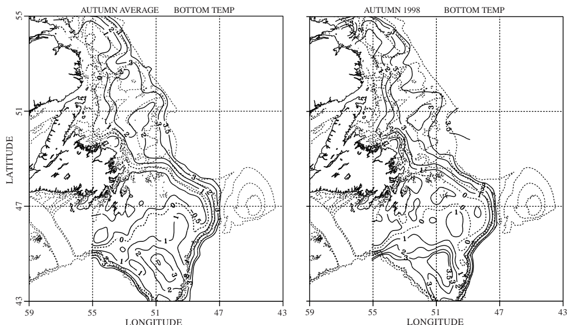
Fig. 23. Contours of the long-term mean (1961–90) (top panel) and 1998 autumn bottom temperatures (bottom panel) for the Newfoundland Shelf.
