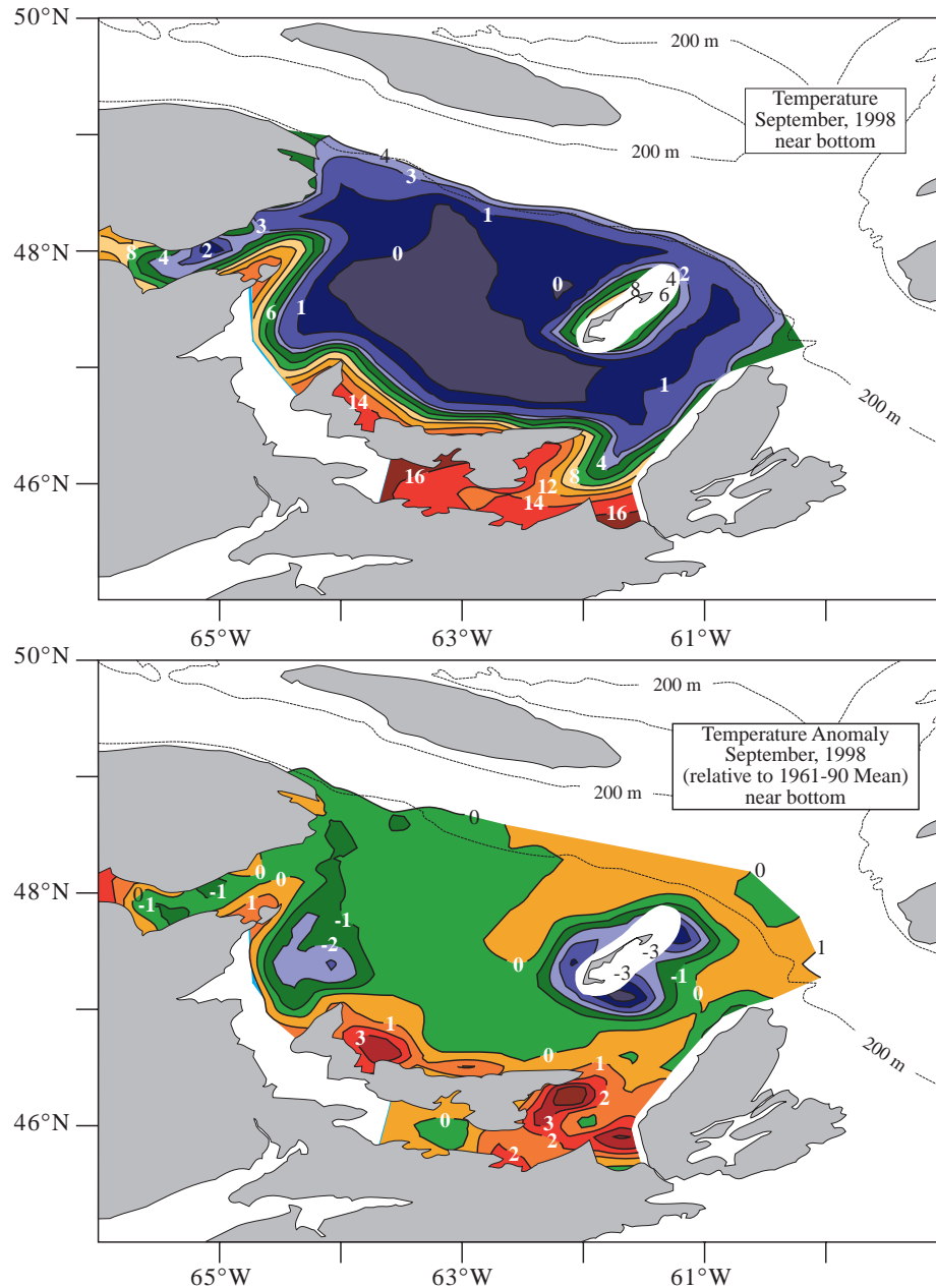
Fig. 32. Temperature (top panel) and temperature anomalies (bottom panel) in °C over the southern Gulf of St. Lawrence during September 1998. The dotted line represents the 200 m isobath.
