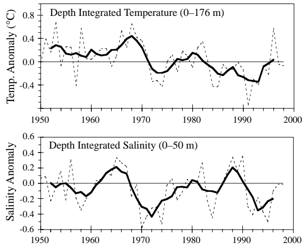
Fig. 20. Vertically-averaged (0–176 m) temperature and (0–50 m) salinity anomalies from Station 27. The annual values are designated by the lighter dashed lines and the 5-year running means by the heavy solid line.
