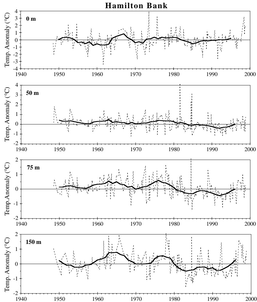
Fig. 24. Monthly (dashed) and 5-year running means (solid line) of temperature anomalies at selected depths on Hamilton Bank in Div. 2J.
