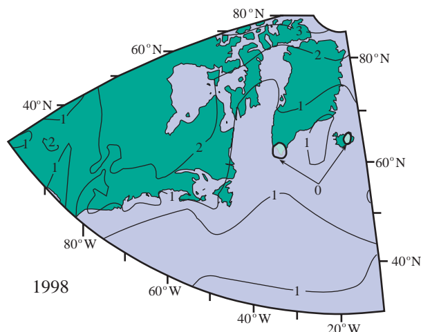
Fig. 1. Annual air temperature anomalies (in ^{\circ}\text{C} ) over the Northwest Atlantic in 1998 relative to the 1961–90 means (taken from Grosswetterlagen Europas ). The lighter coloured areas indicate colder-than-normal temperatures.
