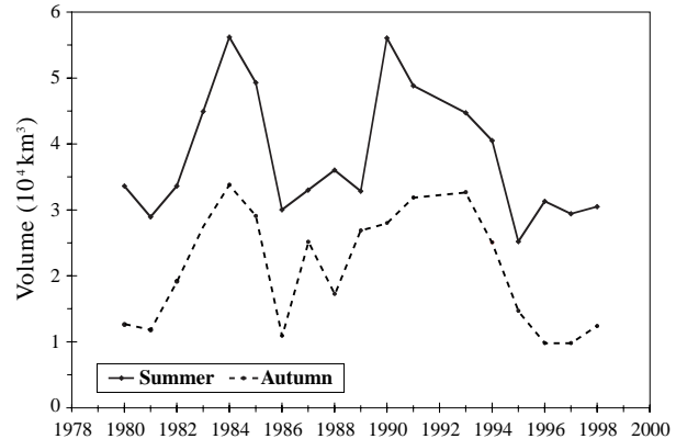
Fig. 22. The CIL volume in the summer and autumn within Div. 2J and 3KL.
