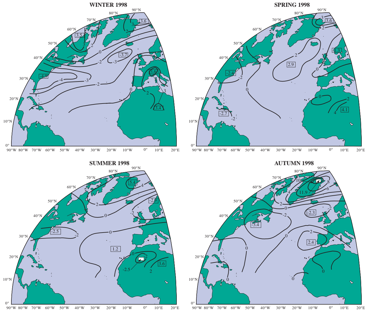
Fig. 7. Seasonal sea-surface air pressure anomalies (mb) over the North Atlantic in 1998 relative to the 1961–90 means.
