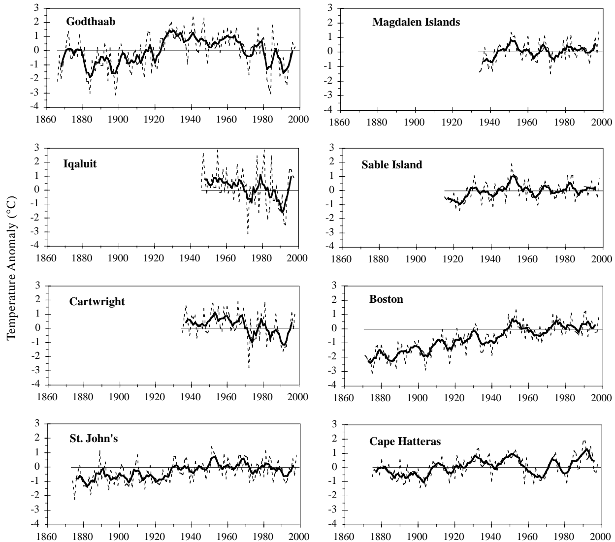
Fig. 5. Annual (dashed) and 5-year running (solid) means of the air temperature anomalies at selected sites.
