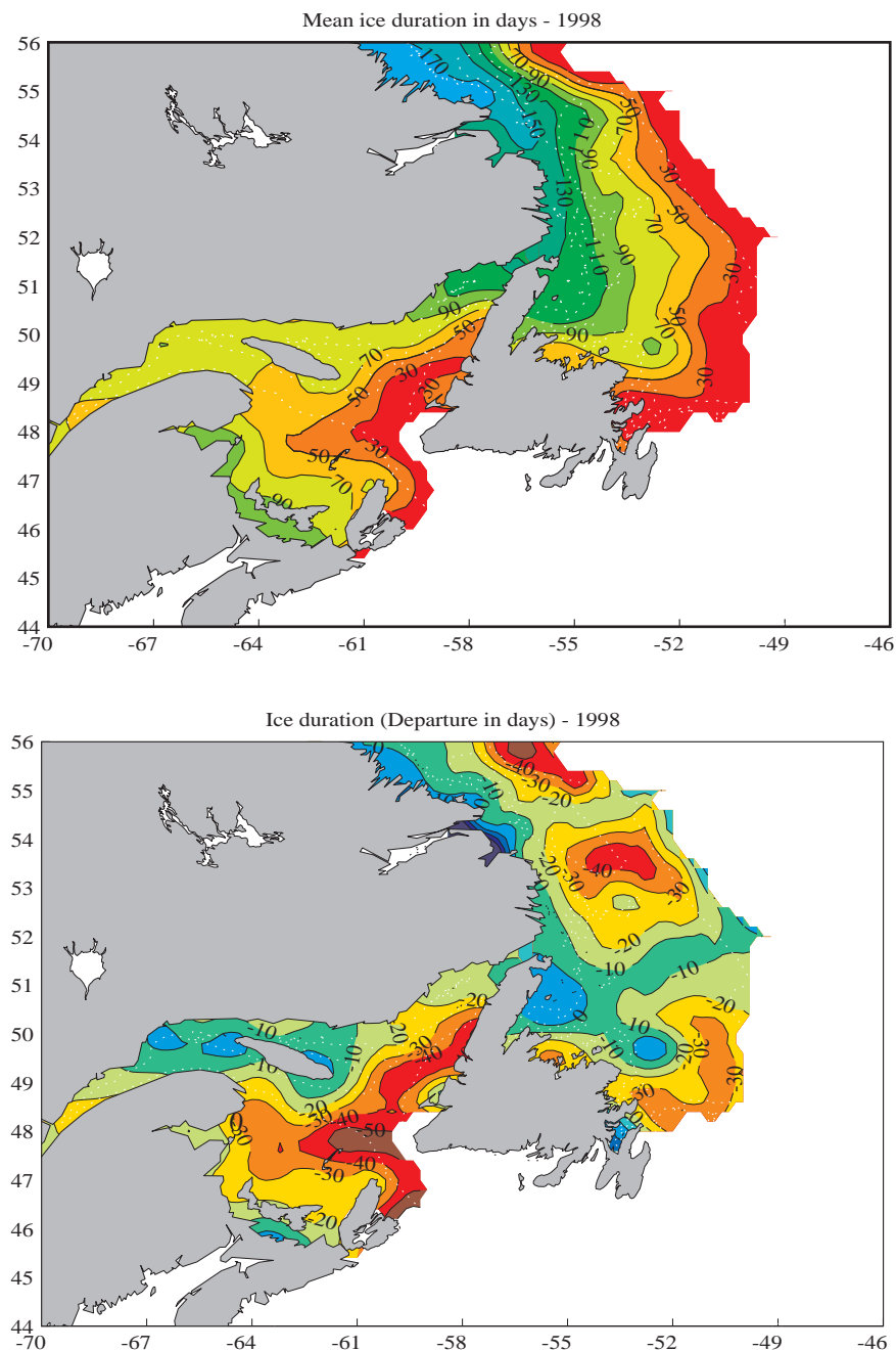
Fig. 13. The duration of sea ice in days during 1998 (top panel) and their anomalies relative to the long-term mean (bottom panel). Blue shaded anomalies indicate longer-than-normal duration; other colours indicate shorter-than-normal duration (bottom panel).
