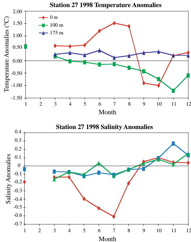
Fig. 18. Monthly temperature (top panel) and salinity (bottom panel) anomalies at 0, 100 and 175 m at Station 27 during 1998.
