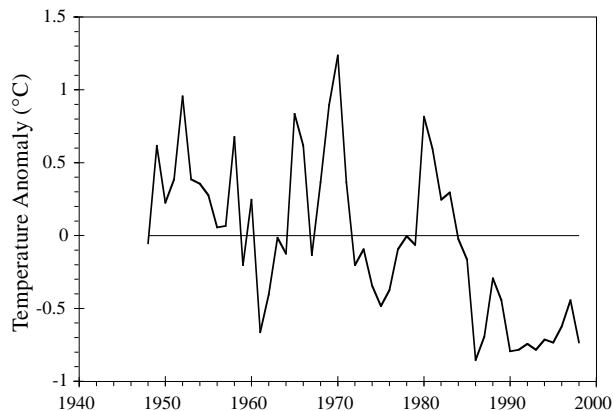
Fig. 31. Anomalies of the CIL core temperatures (extrapolated to 15 July) for the Gulf of St. Lawrence relative to the 1961–90 mean.
