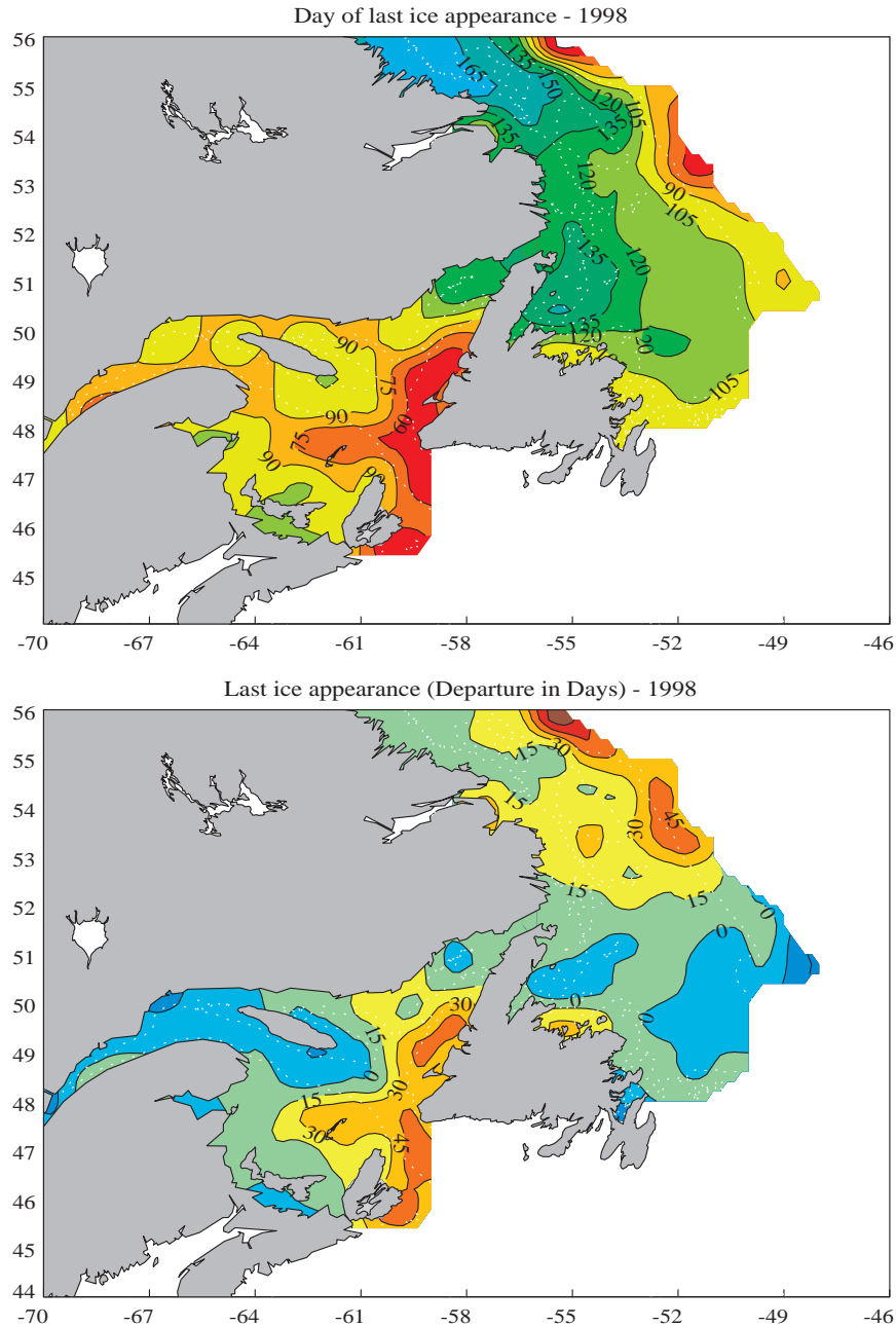
Fig. 12. The time of last presence of sea ice in 1998 measured in days from the end of 1997 (top panel) and their anomalies relative to the long-term mean in days (bottom panel). Blue shaded anomalies indicate later-than-normal departure; other colours indicate earlier-than-normal departure (bottom panel).
