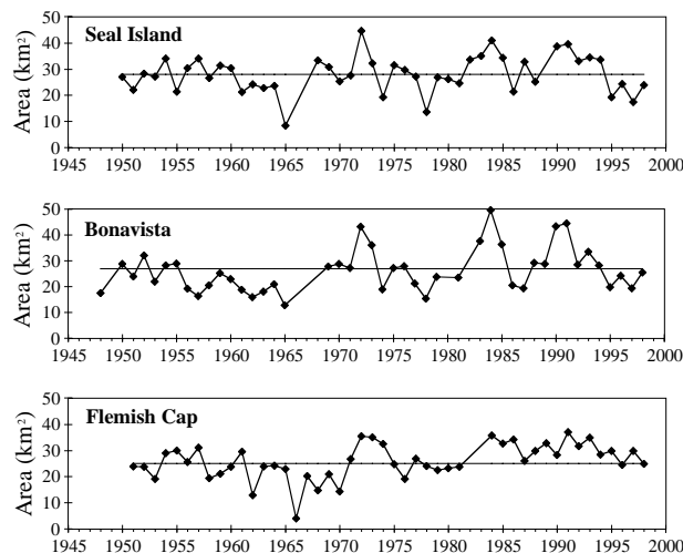
Fig. 21. The CIL cross-sectional area (in \text{km}^2 ) during the summer along transects off Seal Island (southern Labrador), Bonavista Bay (northern Newfoundland), and Flemish Cap (Grand Banks).
