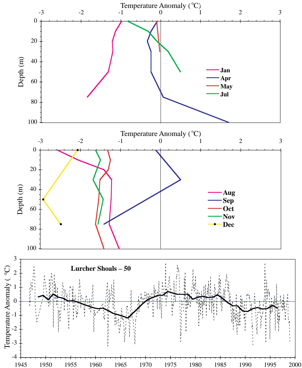
Fig. 44. The 1998 monthly temperature anomaly profiles (top 2 panels) plus the monthly mean temperature anomalies (dashed line) and the 5-year running means of the estimated annual anomalies (solid line) at 50 m for Lurcher Shoals (area 24 – Fig. 41).
