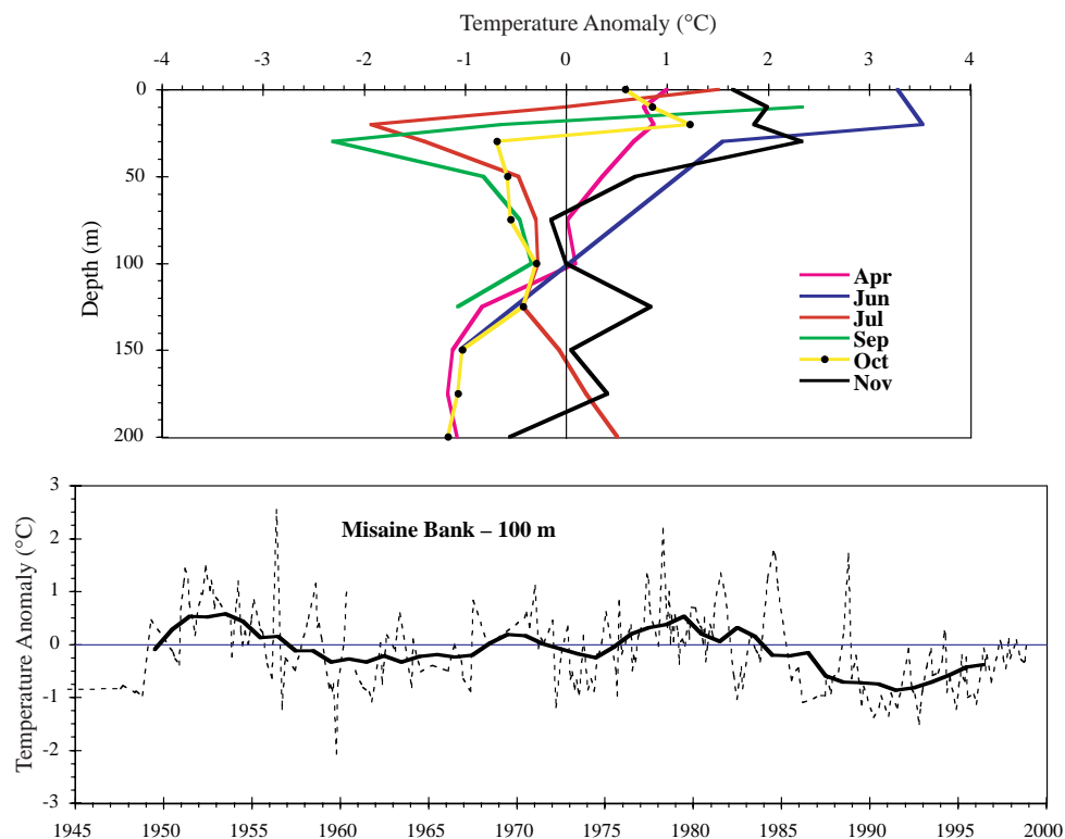
Fig. 43. The 1998 monthly temperature anomaly profiles (top panel) plus the monthly mean temperature anomalies (dashed line) and the 5-year running means of the estimated annual anomalies (solid line) at 100 m for Misaine Bank (area 5 – Fig. 41).
