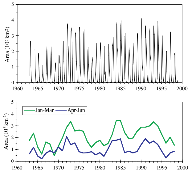
Fig. 10. Time series of the monthly mean ice area (top panel) and the average ice area during ice advance (January–March) and retreat (April–June) (bottom panel) on the southern Labrador and Newfoundland shelves between 45°N–55°N.
