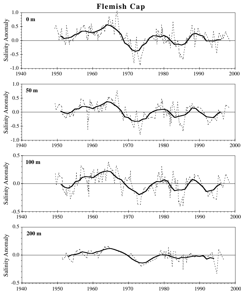
Fig. 27. Monthly (dashed) and 5-year running means (solid line) of salinity anomalies for different depths on Flemish Cap in Div. 3M.
