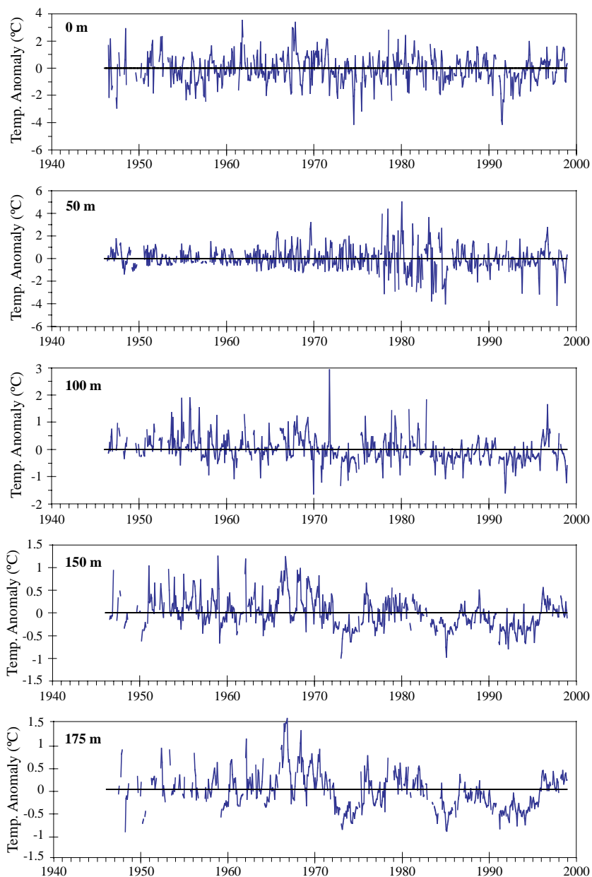
Fig. 19. Monthly mean temperature anomalies at selected depths from Station 27.
