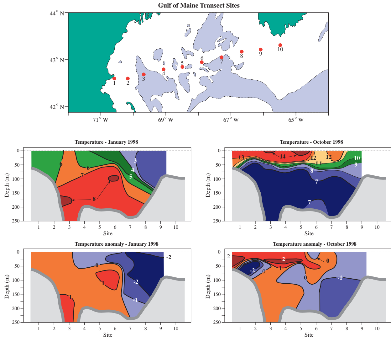
Fig. 39. The temperature (middle panels) and temperature anomalies (bottom panels) in °C along a XBT transect (top panel) across the Gulf of Maine during January and October 1998.
