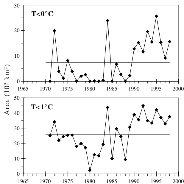
Fig. 33. Area of the Magdalen Shallows with bottom temperatures <0^{\circ}\text{C} (top panel) and <1^{\circ}\text{C} (bottom panel) during September.
