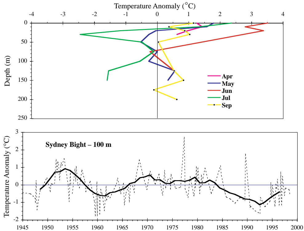
Fig. 42. The 1998 monthly temperature anomaly profiles (top panel) plus the monthly mean temperature anomalies (dashed line) and the 5-year running means of the estimated annual anomalies (solid line) at 100 m for Sydney Bight (area 1 – Fig. 41).
