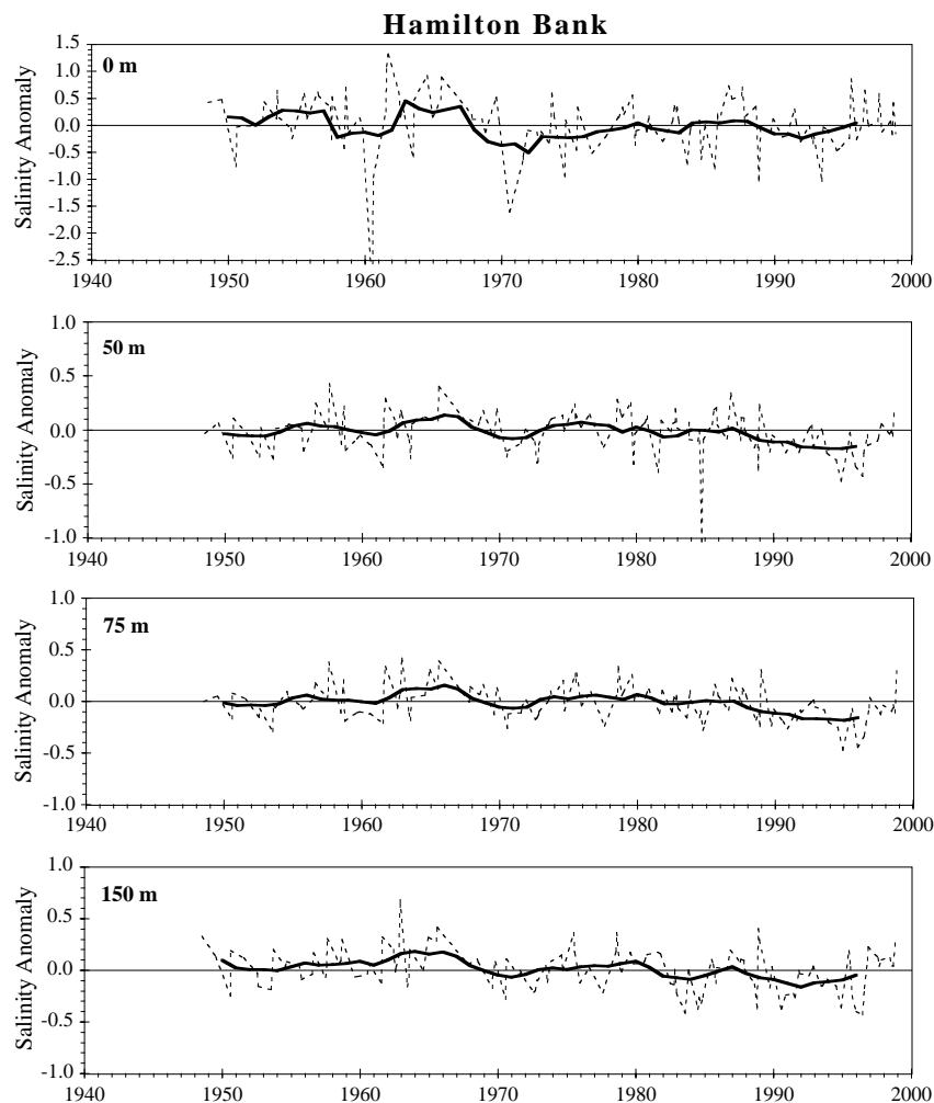
Fig. 25. Monthly (dashed) and 5-year running means (solid line) of salinity anomalies at selected depths on Hamilton Bank in Div. 2J.
