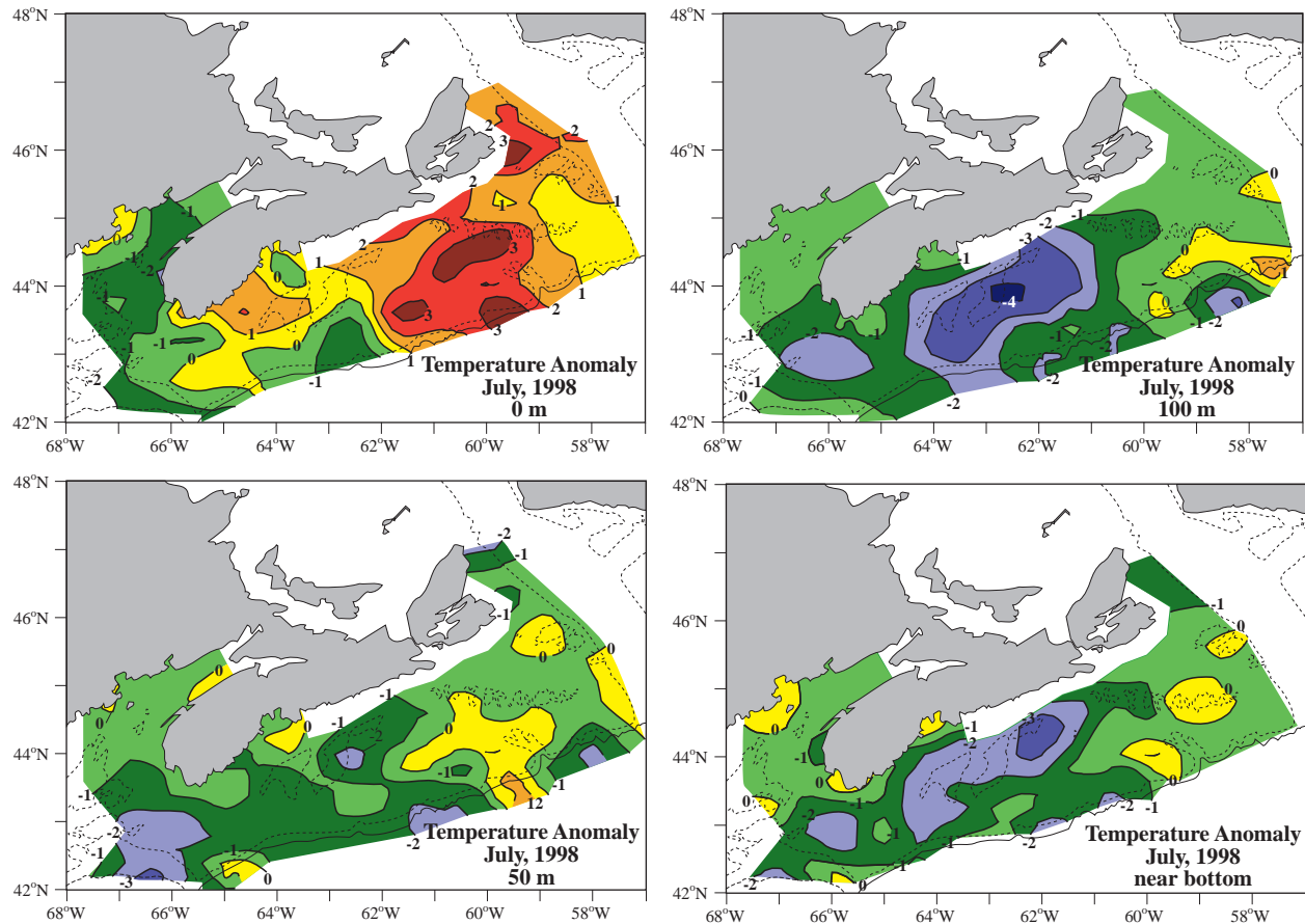
Fig. 47. Contours of optimally estimated temperature anomalies at the surface, 50 m, 100 m and near bottom during the 1998 July groundfish surveys.
