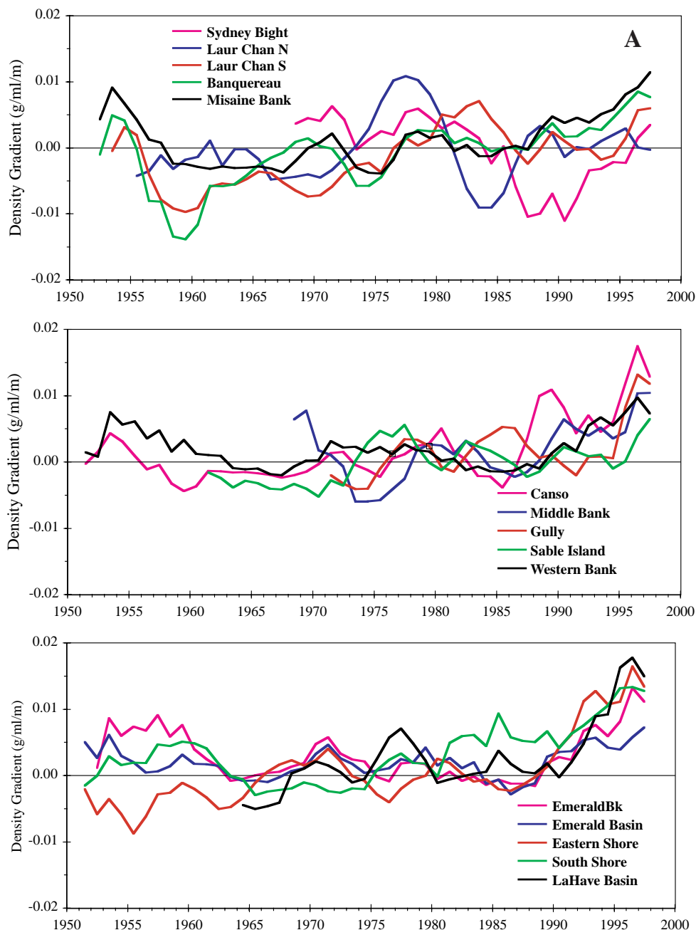
Fig. 48a. Five-year running means of the annual anomalies of the density gradient between surface and 50 m calculated for the areas 1–15 in Fig. 41.
