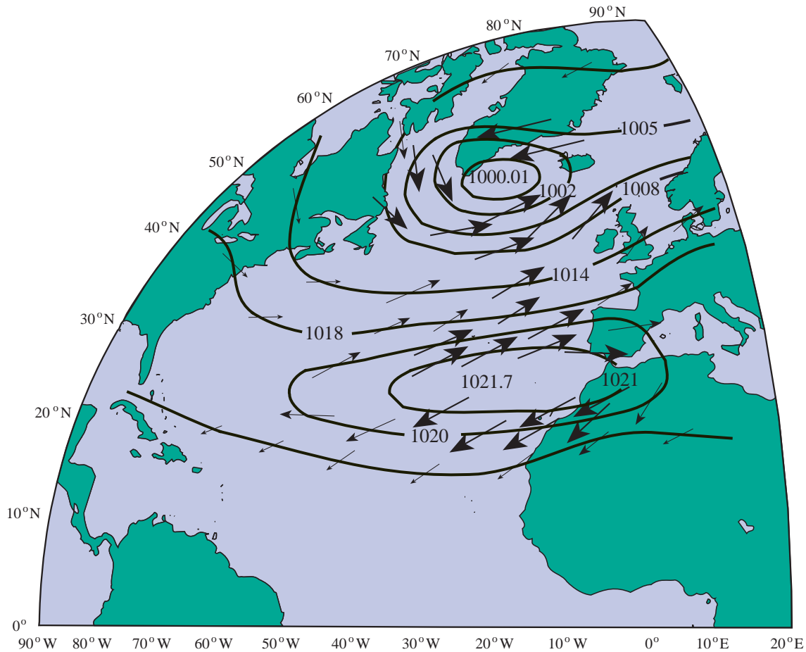
Fig. 6. The long-term (1961–90) mean sea surface pressures during winter (average of December, January and February). A schematic of the associated wind field is also shown.
