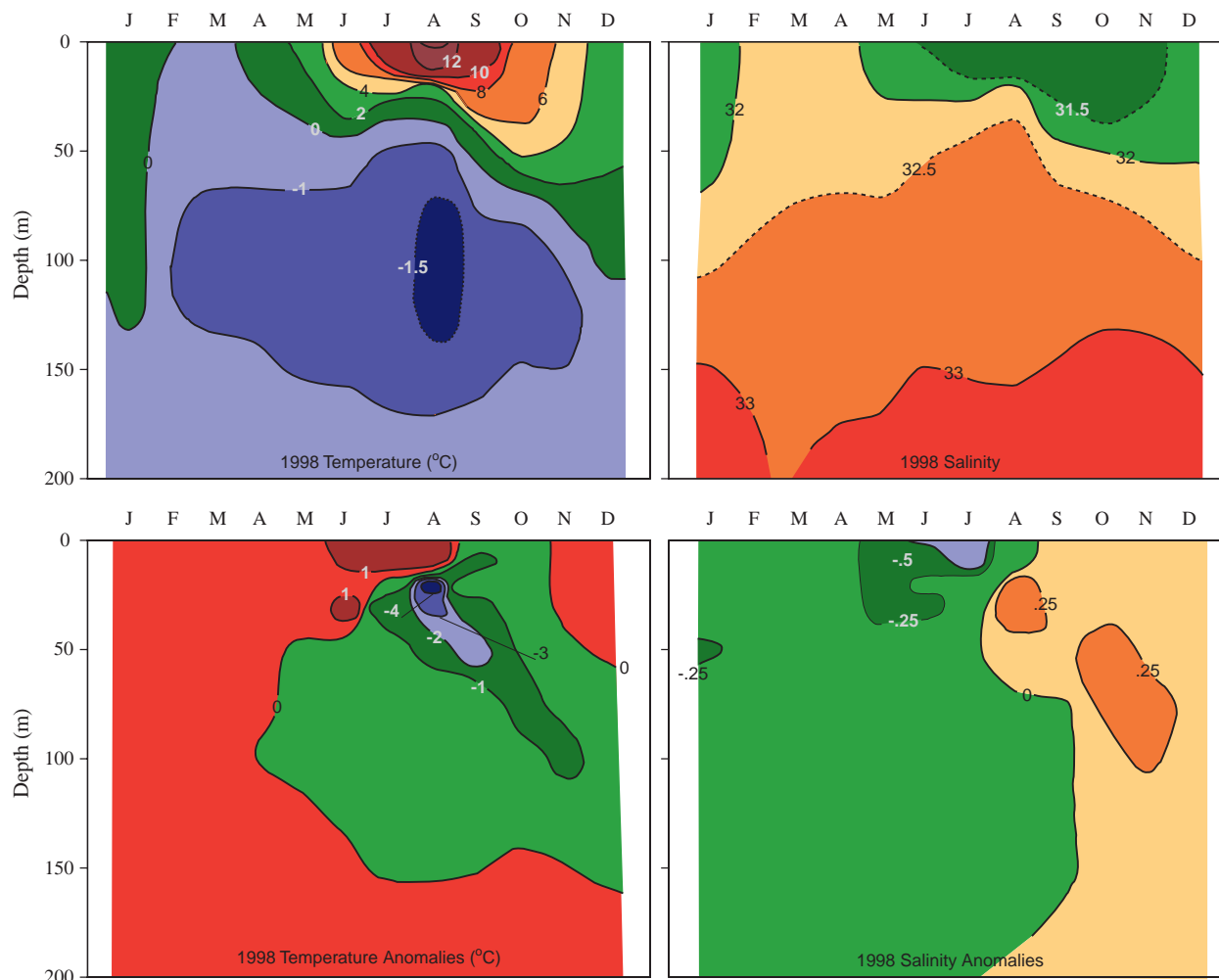
Fig. 17. Monthly mean (top panel) and anomalies relative to the 1961–90 average (bottom panel) of temperature (in °C) and salinity at Station 27 as a function of depth during 1998.
