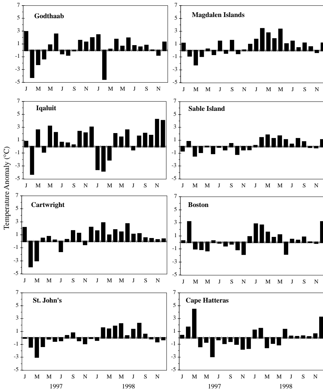
Fig. 4. Monthly air temperature anomalies in 1997 and 1998 at selected coastal sites (see Fig. 3 for locations).
