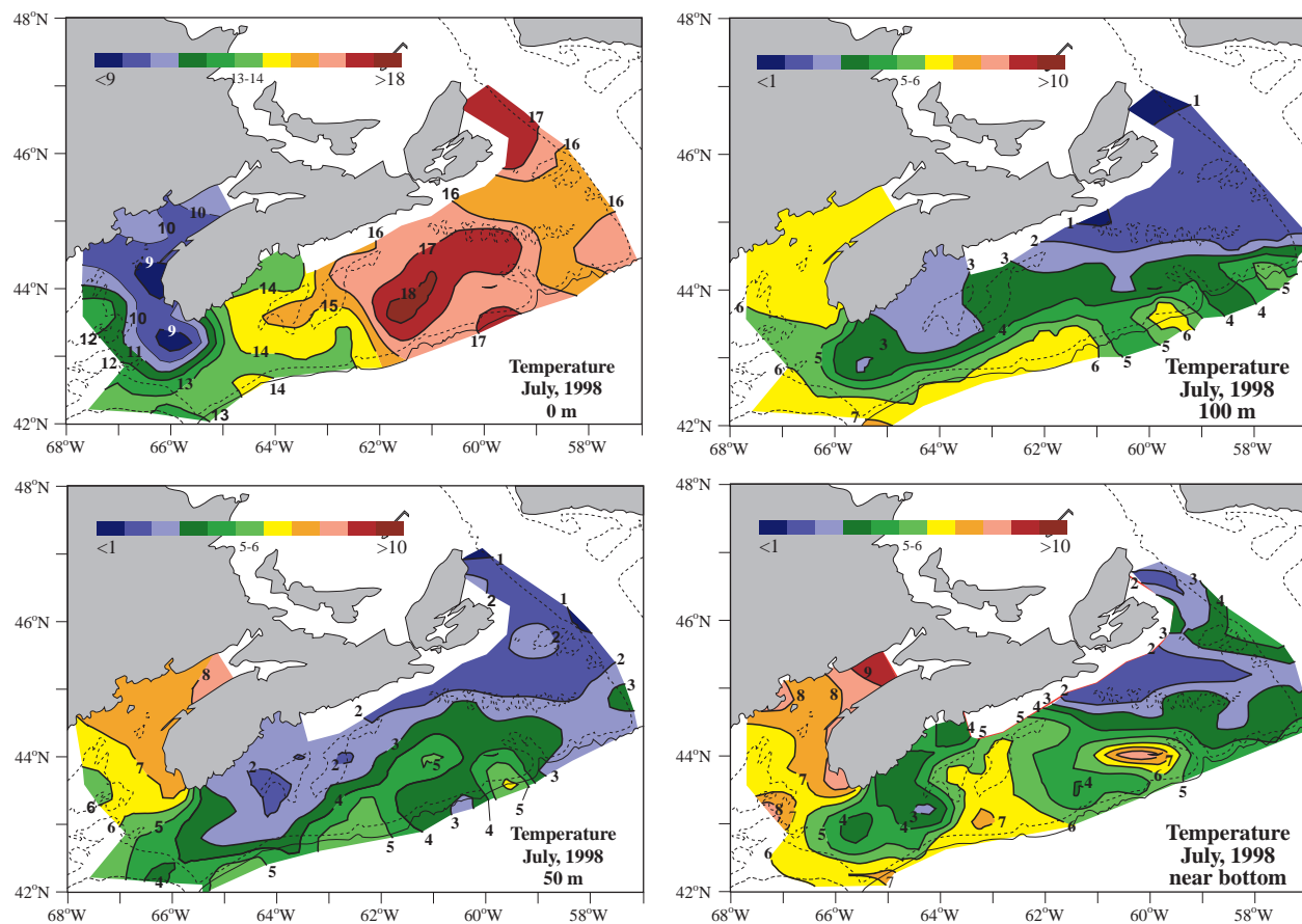
Fig. 46. Contours of optimally estimated temperatures at the surface, 50 m, 100 m and near bottom during the 1998 July groundfish surveys.
