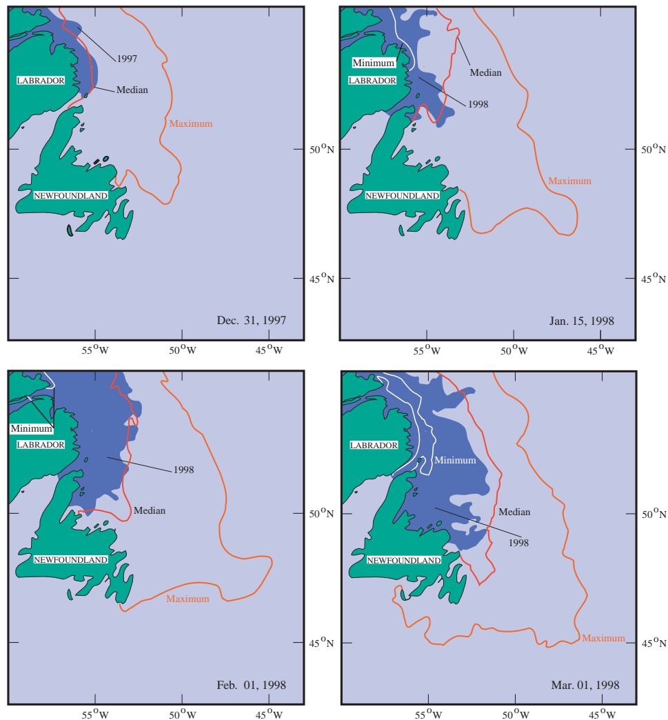
Fig. 9a. The area of sea ice (>10% concentration) together with the historical (1962–87) minimum, median and maximum positions of the ice edge off Newfoundland and Labrador between December 1997 and March 1998.
