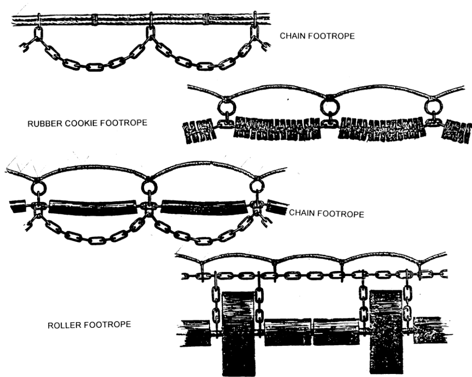
Figure 28. Examples of sweep gear.
