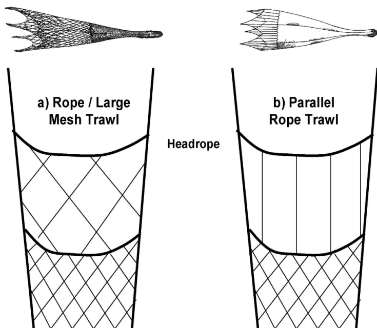
Figure 24. Examples of mid-water nets designed with large meshes (a) and parallel ropes (b).
