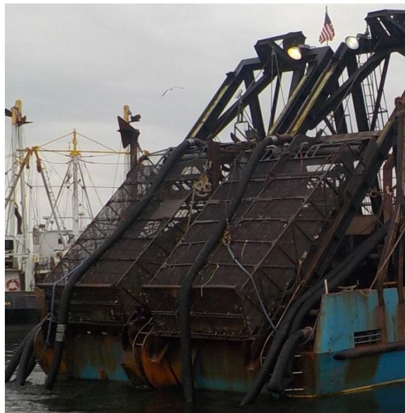
Figure 45. An example of stern-rigged dredges on A-frames.
