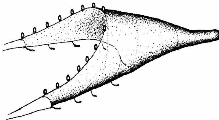
Figure 34. A sweepless raised footrope trawl.
