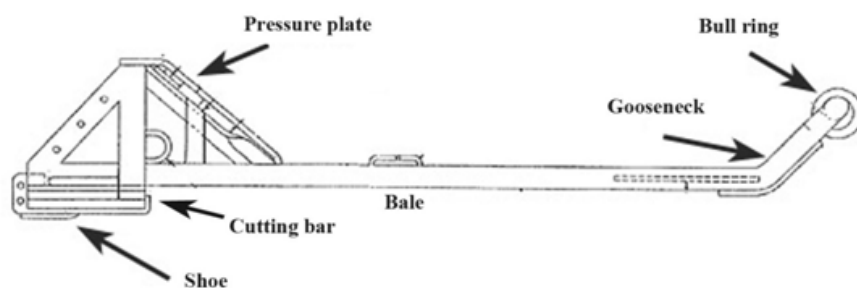
Figure 39. Parts of a scallop dredge frame.
