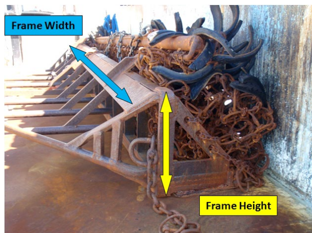
Figure 38. Standard scallop dredge frame showing height and width dimensions.
