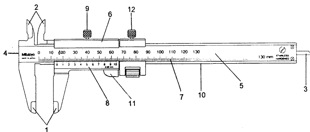
Figure 27. Vernier calipers.
