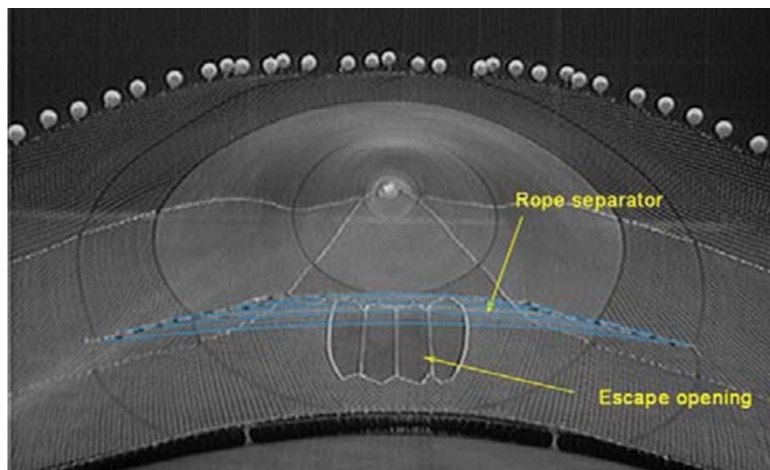
Figure 33. A rope separator trawl.
