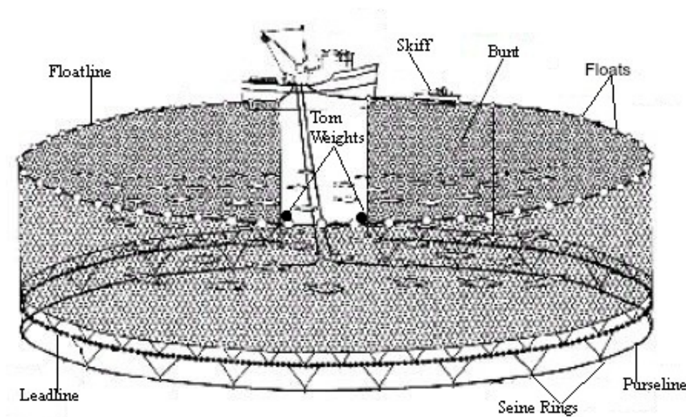
Figure 35. Parts of a purse seine. Source: HTTP://WWW.ICCAT.INT/DOCUMENTS/SCRS/MANUAL/CH3/CHAP%203_1_1_PS_ENG.PDF , modified by FMRD.
