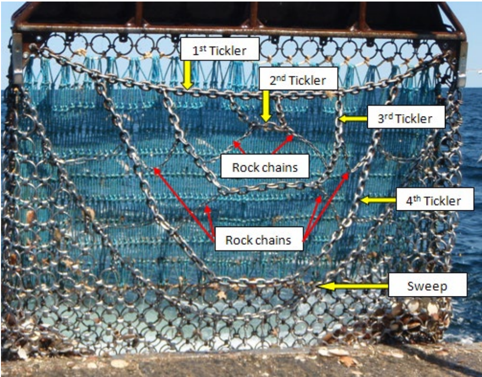
Figure 43. Scallop dredge with spider chain mat.
