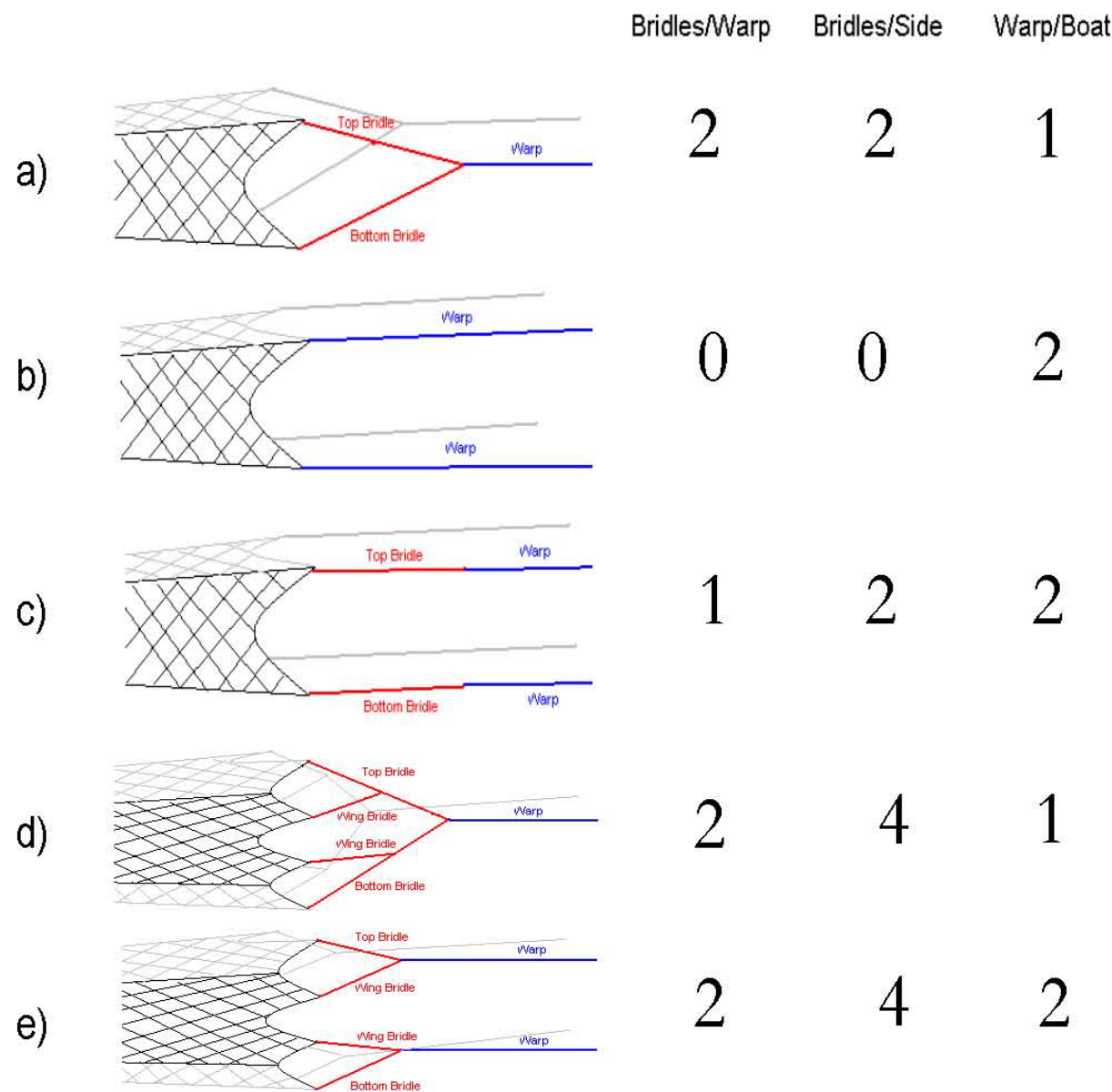
Figure 25. Pair trawl rigging designs showing bridles, warp, and boat relations. Bridles shown in red and warps in blue.
