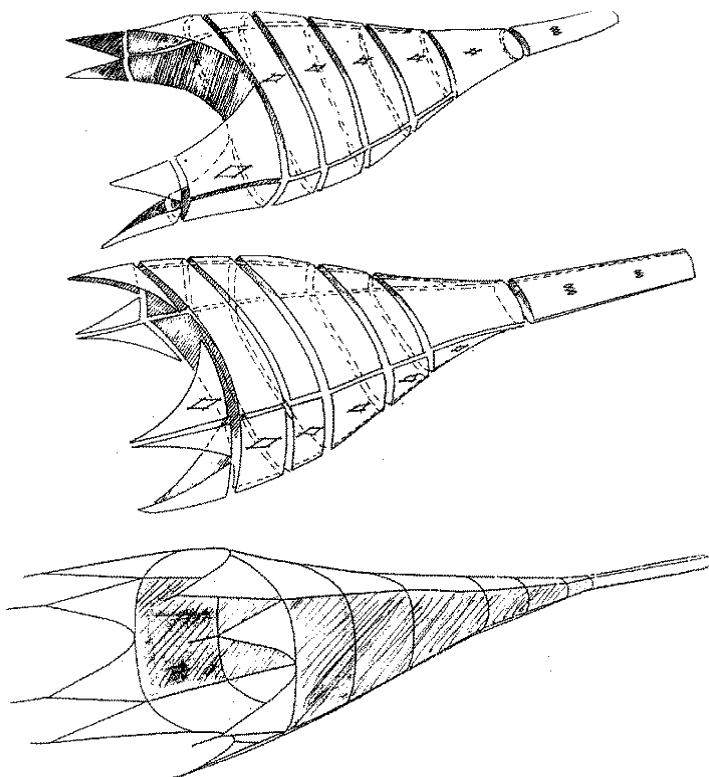
Figure 23. Various configurations of midwater trawl net panels. Top: 2-seam net. Middle: 4-seam net with unequal panels (sides are equal, top and bottom are equal, but sides are not equal to top and bottom). Bottom: 4-seam net with equal panels (sides and top and bottom all equal).
