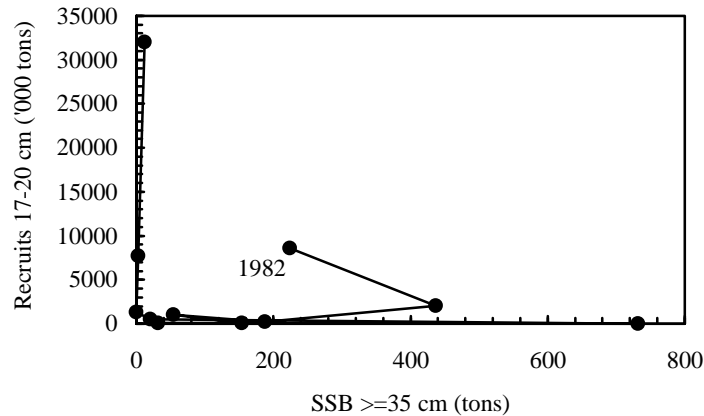
Fig. 16.8. Deep sea redfish in Subarea 1: SSB-recruitment plot as derived from the EU-Germany groundfish survey.
