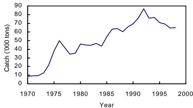
Fig. 1.1. Shrimp in Subareas 0 and 1: total catches (1998 projected to the end of the year).
