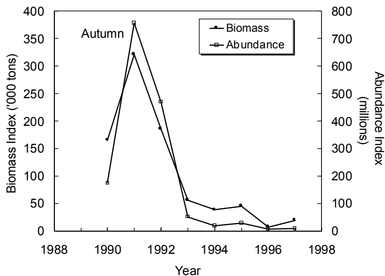
Fig. 9.3. Cod in Div. 3NO: abundance and biomass estimates from Canadian autumn surveys.
