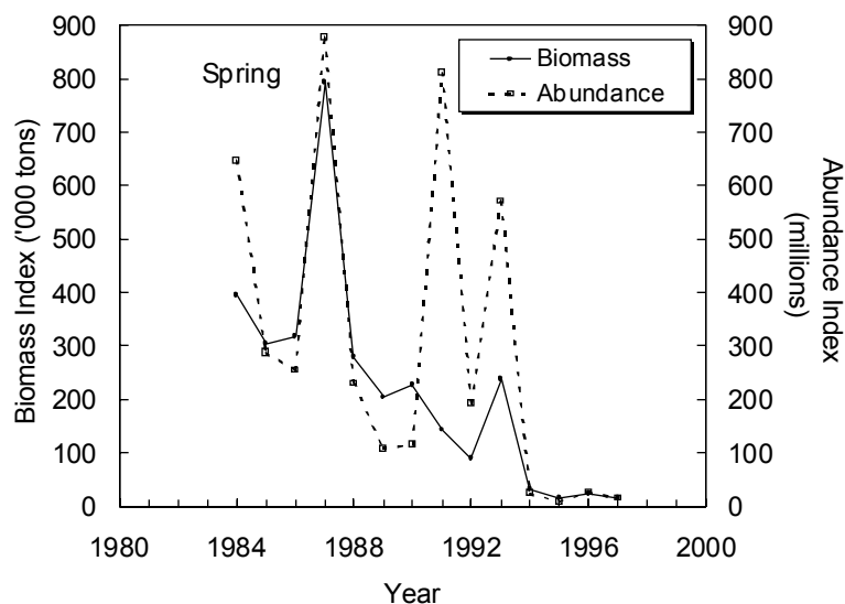
Fig. 9.2. Cod in Div. 3NO: abundance and biomass estimates from Canadian spring surveys.
