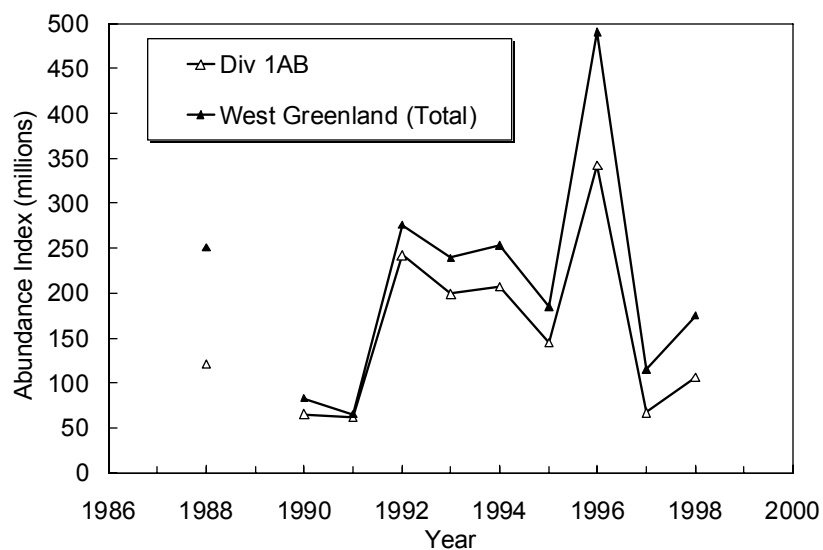
Fig. 1.4. Greenland halibut in Subareas 0+1 (excluding Div. 1A inshore): offshore abundance from shrimp trawl surveys.
