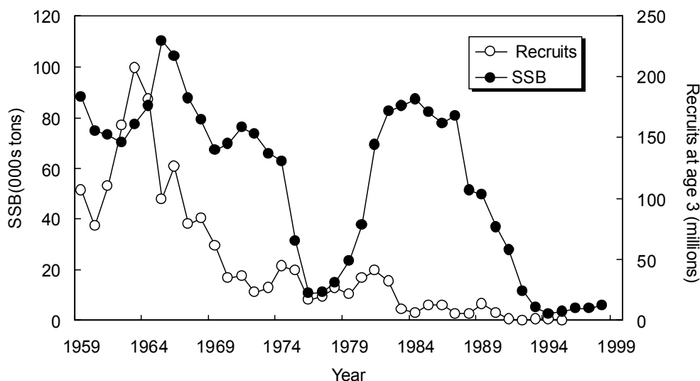
Fig. 9.4. Cod in Div. 3NO: time trend from the SPA of spawner stock biomass (SSB) and corresponding recruitment.
