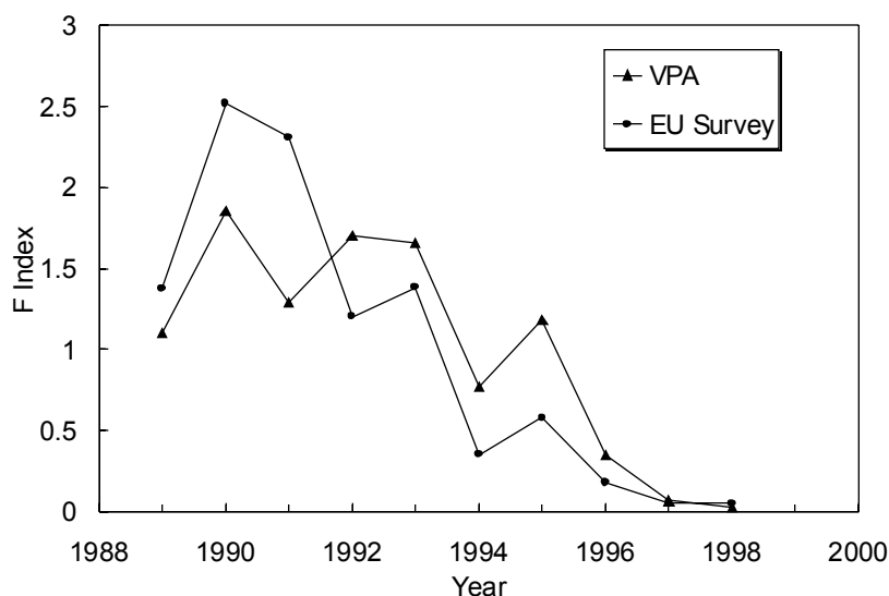
Fig. 7.3. Beaked redfish in Div. 3M: VPA and EU survey fishing mortality trends.
