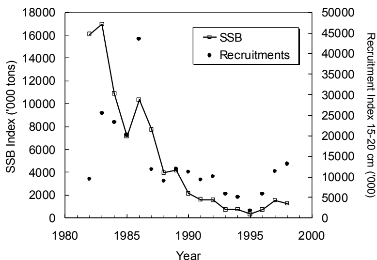
Fig. 5.2 American plaice in Subarea 1: SSB and recruitment indices as derived from the EU-Germany groundfish survey.
