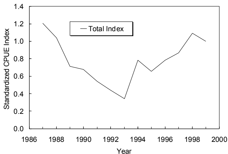
Fig. 3.3. Northern shrimp in Denmark Strait: annual standardized CPUE-indices (relative units) calculated from logbook data from Danish, Faroese and Greenlandic vessels in the total area.
