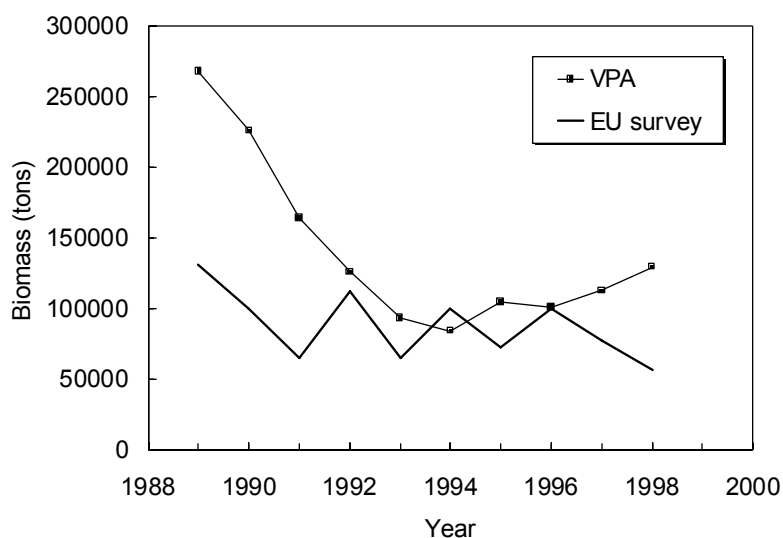
Fig. 7.4. Beaked redfish in Div. 3M: VPA total biomass and EU survey bottom biomass trends.
