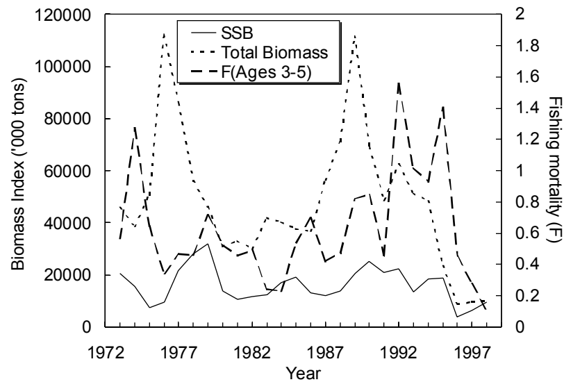
Fig 6.3. Cod in Div. 3M: results from Sequential Population Analysis
