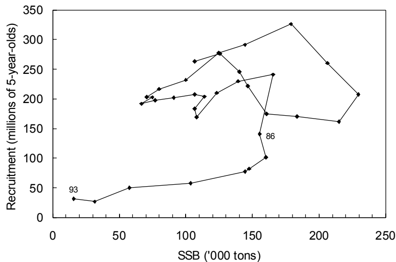
Fig. 11.6. American plaice in Div. 3LNO: spawning stock biomass and recruitment from VPA.
