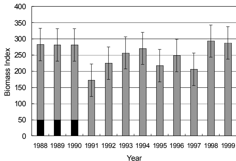
Fig. 2.5. Northern shrimp in Subareas 0 and 1: combined biomass index from inshore and offshore surveys, plus and minus one standard error. 1988-90 includes an average of 50 000 tons for the inshore area indicated by black bars.
