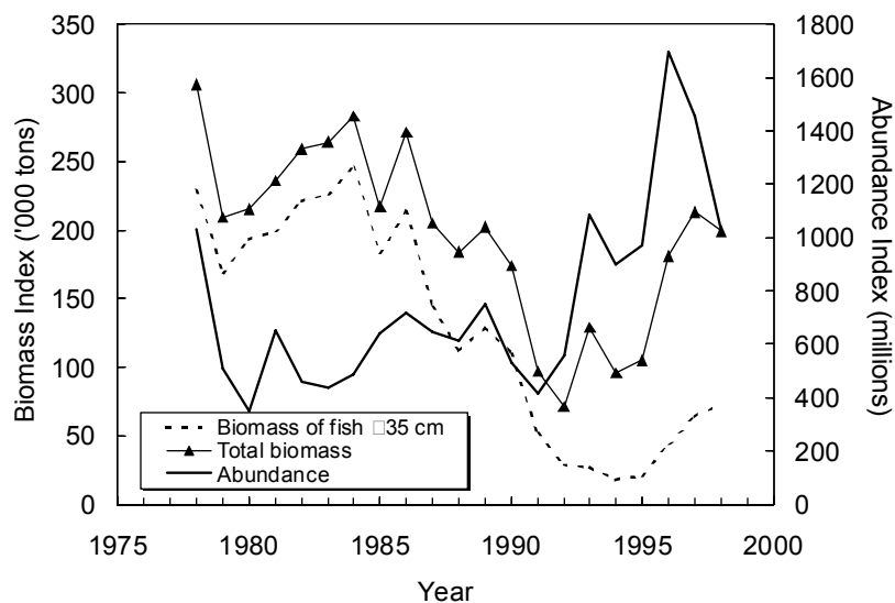
Fig. 16.2. Greenland halibut in Div. 2J and 3K: estimates of biomass and abundance from Canadian surveys.
