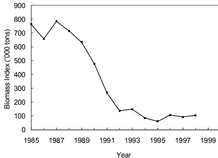
Fig. 11.2. American plaice in Div. 3LNO: biomass from spring surveys.
