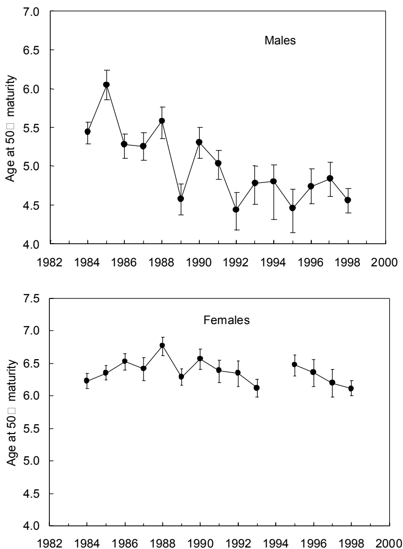
Fig. 12.5. Yellowtail flounder in Div. 3LNO: age at 50
