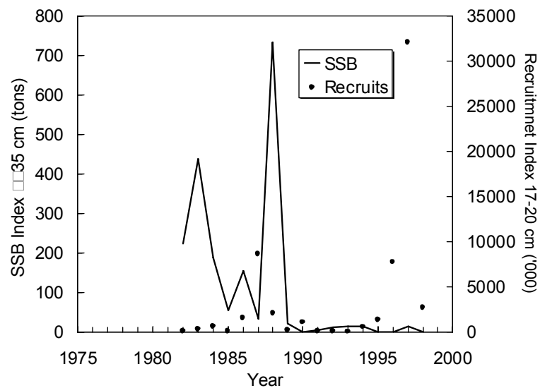
Fig. 4.7 Deep-sea redfish in Subarea 1: SSB and recruitment indices as derived from the EU-Germany groundfish survey in the given years.
