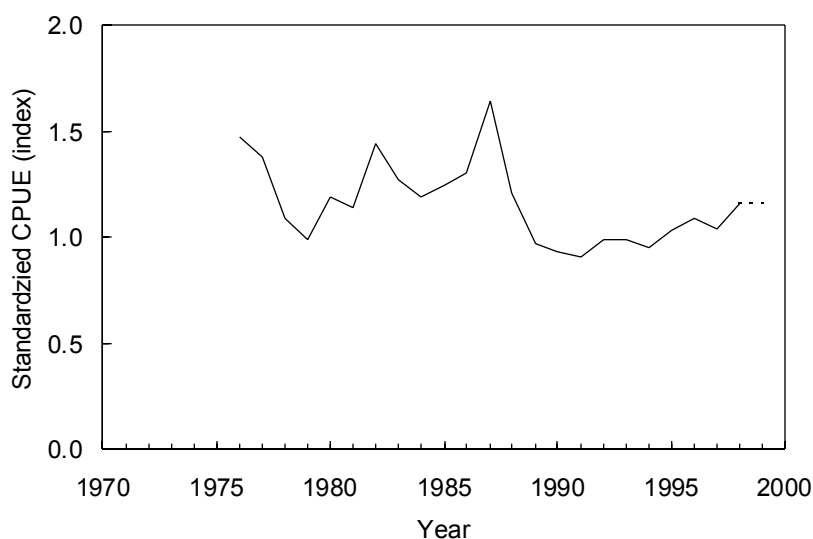
Fig. 2.2. Northern shrimp in Subareas 0 and 1: standardized CPUE index.
