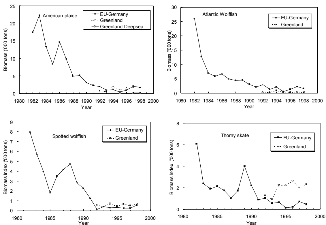
Fig. 5.1. Finfish in Subarea 1: survey biomass indices of various finfish species.
