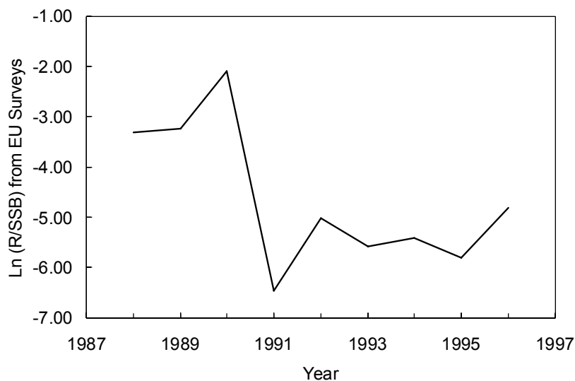
Fig. 8.5. American plaice in Div. 3M: recruits at age 2 produced per Kg of SSB index.
