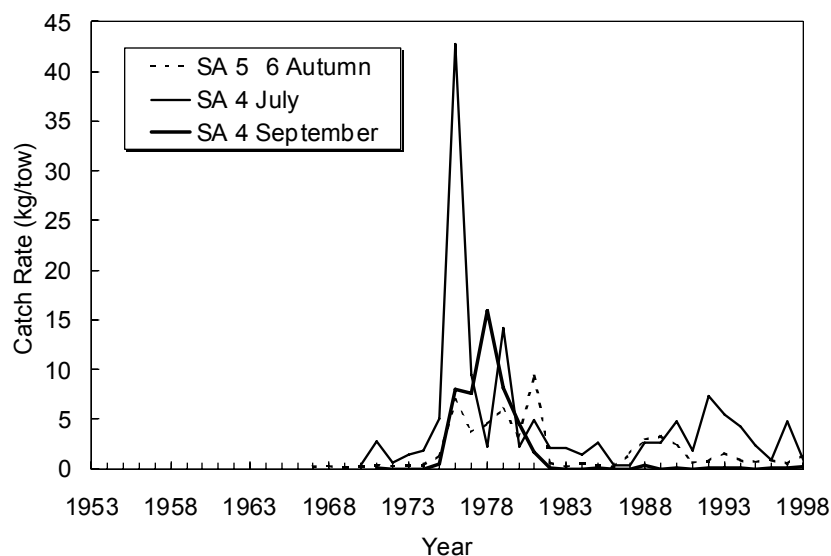
Fig 17.2. Short-finned squid in Subareas 3+4: research survey biomass indices for Subarea 4 during July in Div. 4VWX, and September in Div. 4T, as well as during autumn in Subareas 5+6.
