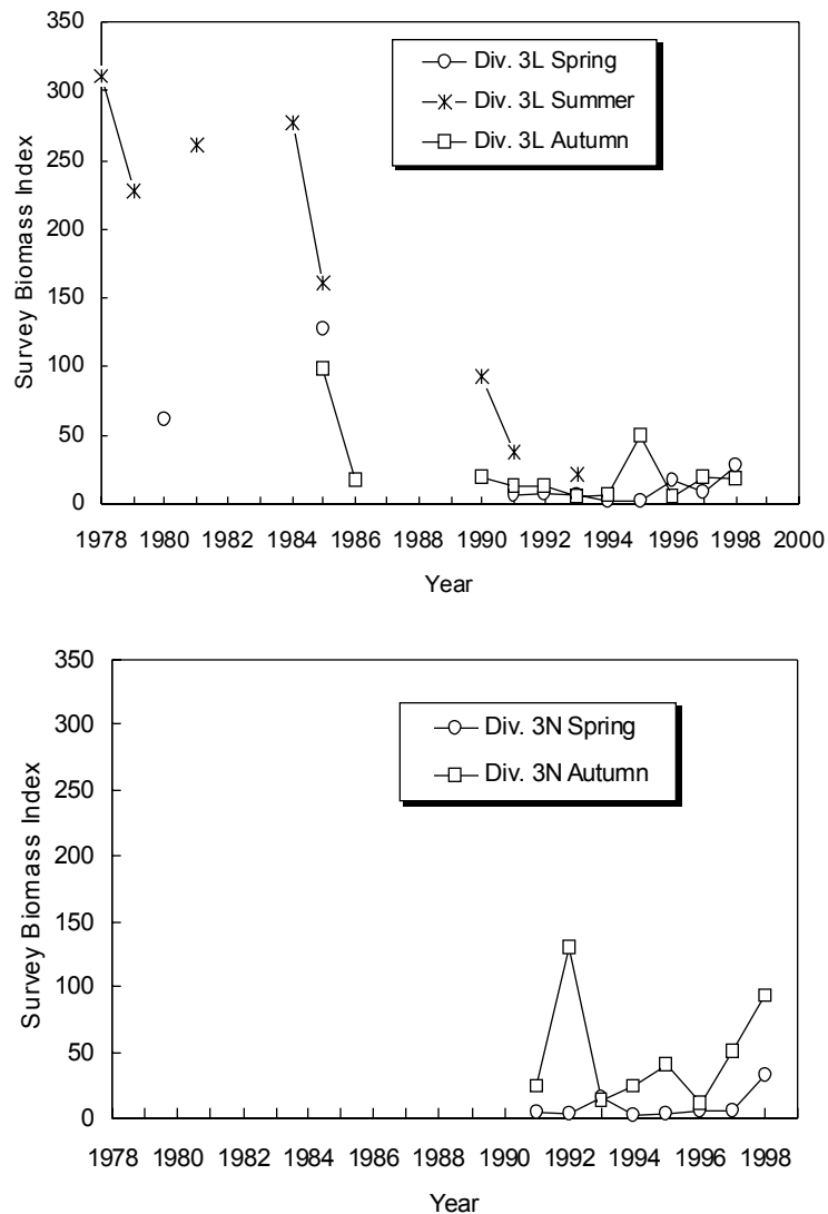
Fig. 10.2. Redfish in Div. 3LN: survey biomass indices from Canadian surveys in Div. 3L and Div. 3N in Campelen equivalent units for surveys prior to autumn 1995.
