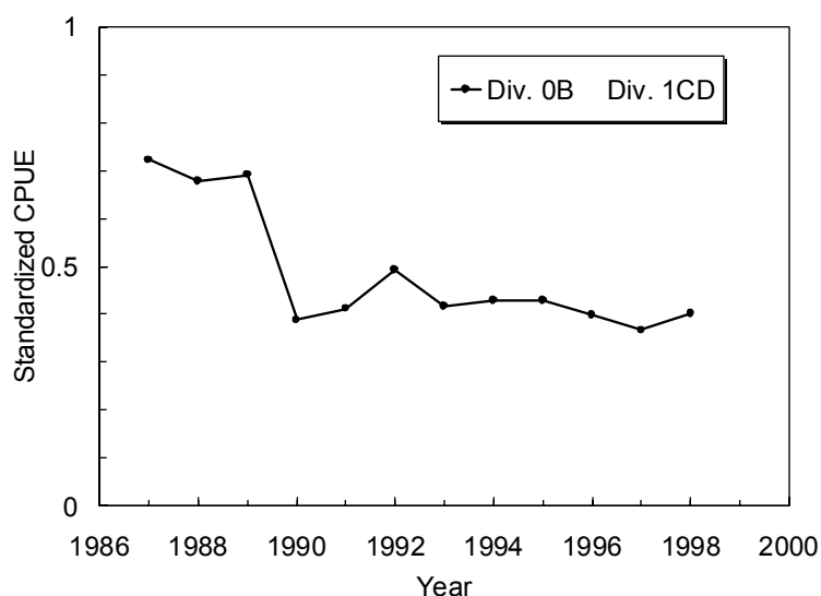
Fig. 1.2. Greenland halibut in Subareas 0+1 (excluding Div. 1A inshore): combined standardized CPUE from Div. 0B and Div. 1CD.
