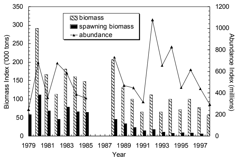
Fig. 7.2. Beaked redfish in Div. 3M: bottom biomass, female spawning biomass and abundance from Canadian (1979-85) and EU (1988-98) surveys.
