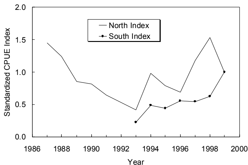
Fig. 3.2. Northern shrimp in Denmark Strait: annual standardized CPUE-indices (relative units) calculated from logbook data from Danish, Faroese and Greenlandic vessels in the areas north and south of 65°N.
