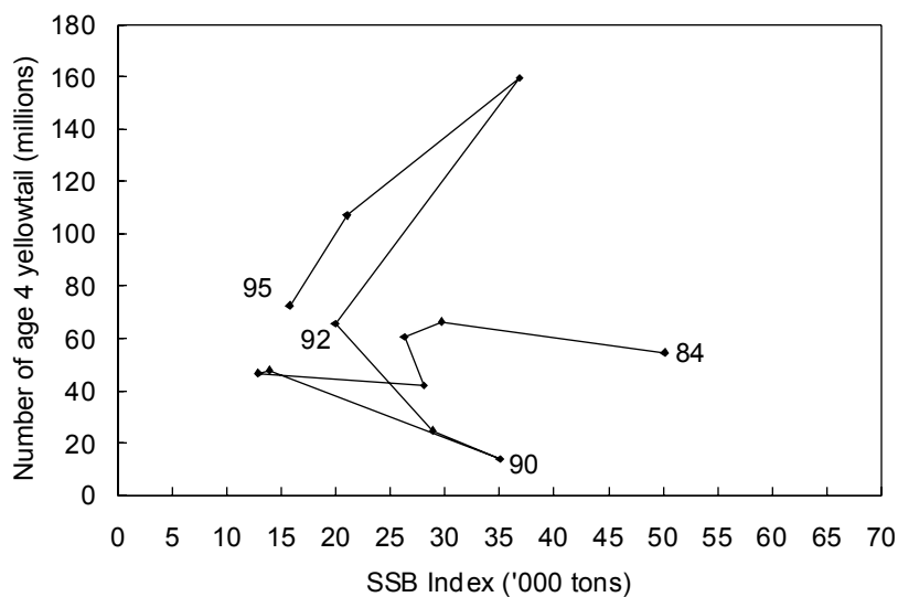
Fig. 12.8. Yellowtail flounder in Div. 3LNO: stock/recruitment plot.
