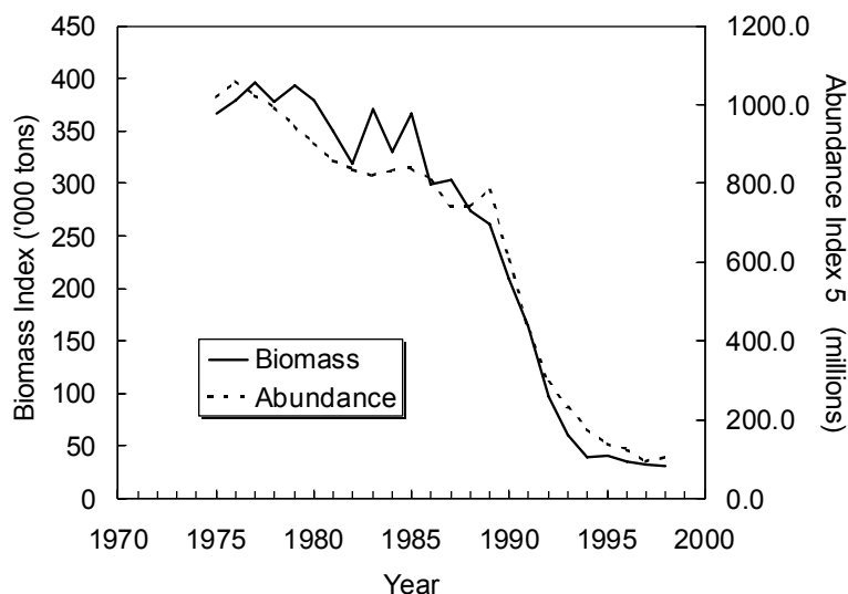
Fig. 11.4. American plaice in Div. 3LNO: population abundance and biomass from VPA.
