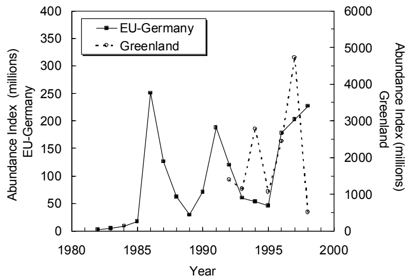
Fig. 4.4. Juvenile redfish (deepsea redfish and golden redfish combined) in Subarea 1: survey abundance indices.
