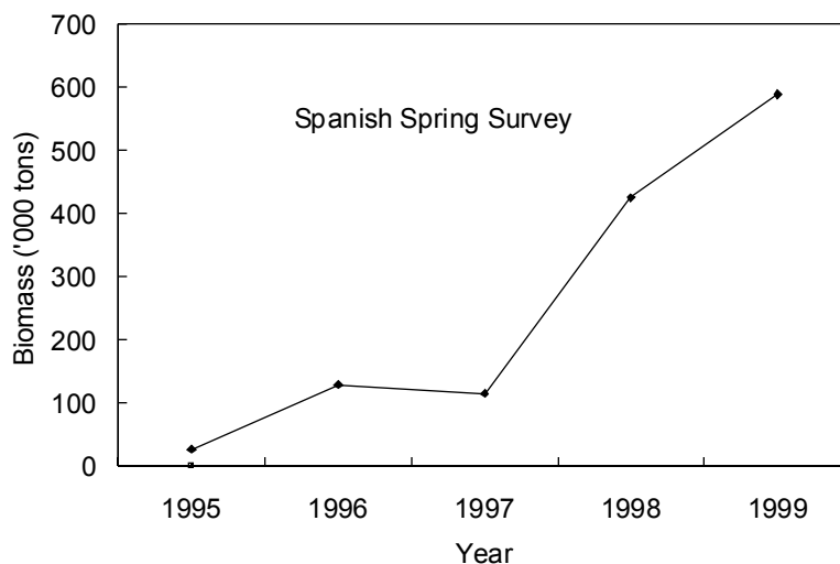
Fig. 12.4. Yellowtail flounder in Div. 3LNO: estimates of biomass from the Spanish surveys in the Regulatory Area of Div. 3NO.
