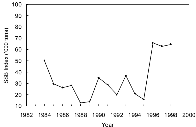
Fig. 12.6. Yellowtail flounder in Div. 3LNO: female spawning stock biomass estimated from the 1984-98 annual spring surveys.
