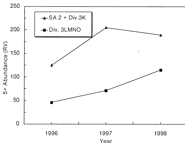
Fig. 1. Greenland halibut: abundance at age 5+ from research vessel (RV) surveys.
