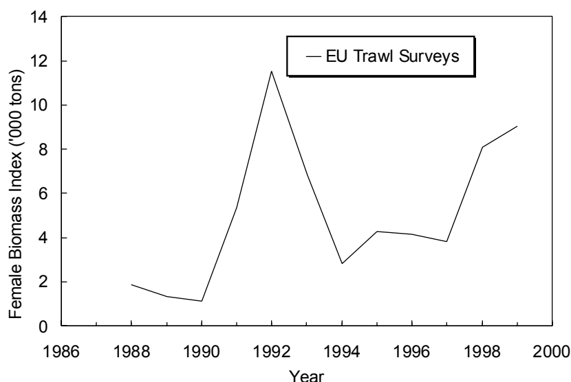
Fig. 1.3. Northern shrimp in Div. 3M: female biomass index from EU trawl surveys, 1988-99.
