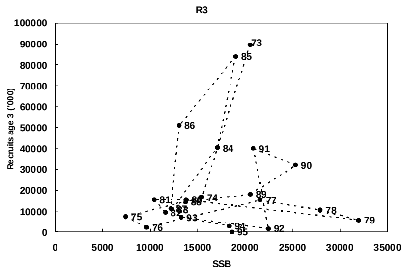
Fig. 6.4. Cod in Div. 3M: total biomass, SSB and recruitment at age 3
