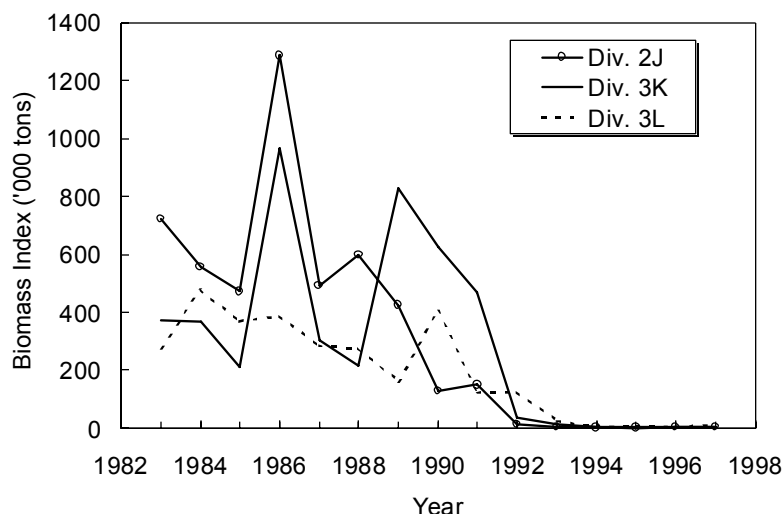
Fig. 18.2. Cod in Div. 2J+3KL: biomass indices from autumn surveys.
