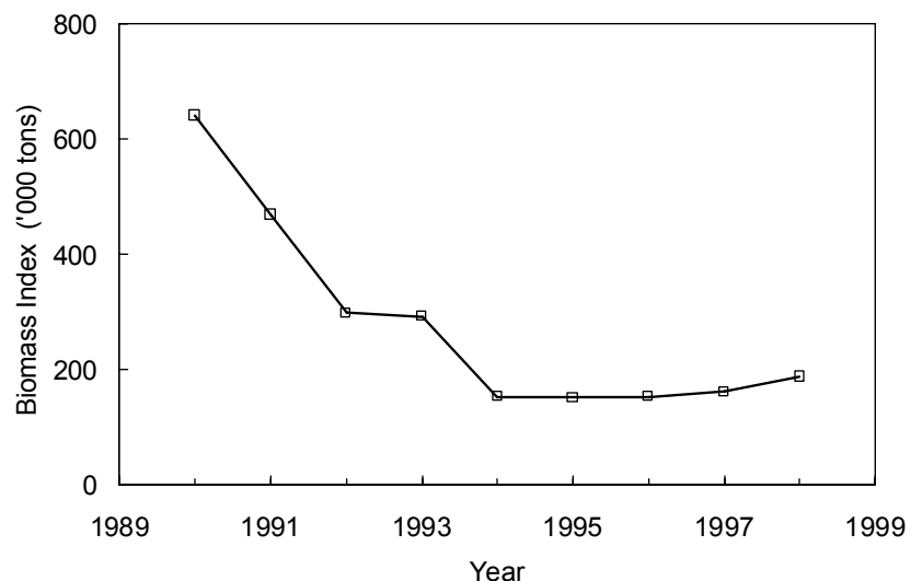
Fig. 11.3. American plaice in Div. 3LNO: biomass from autumn surveys.
