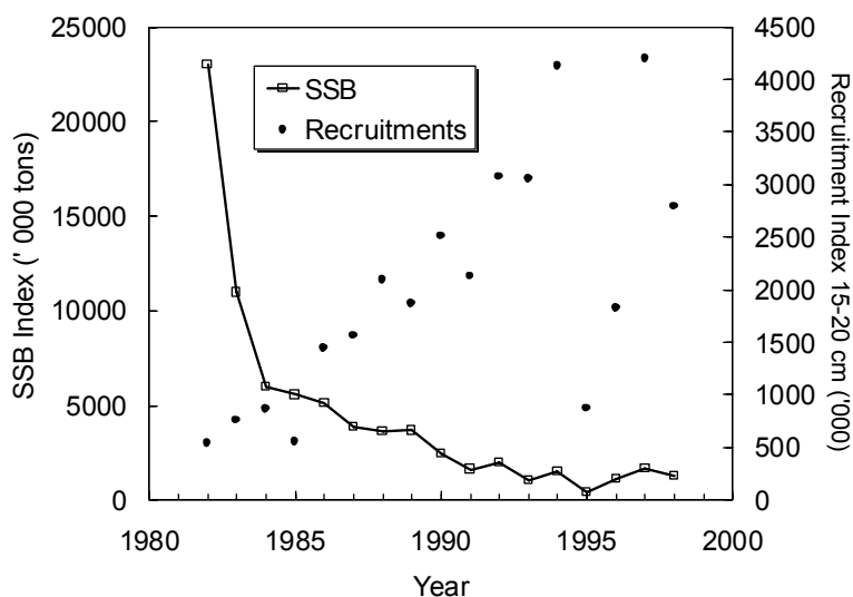
Fig. 5.3. Atlantic wolffish in Subarea 1: SSB and recruitment indices as derived from the EU-Germany groundfish survey.
