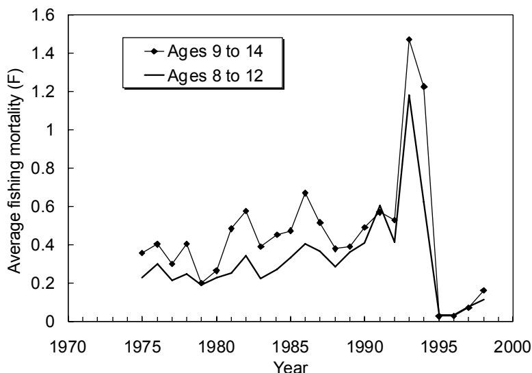
Fig. 11.5. American plaice in Div. 3LNO: Average fishing mortality from VPA.
