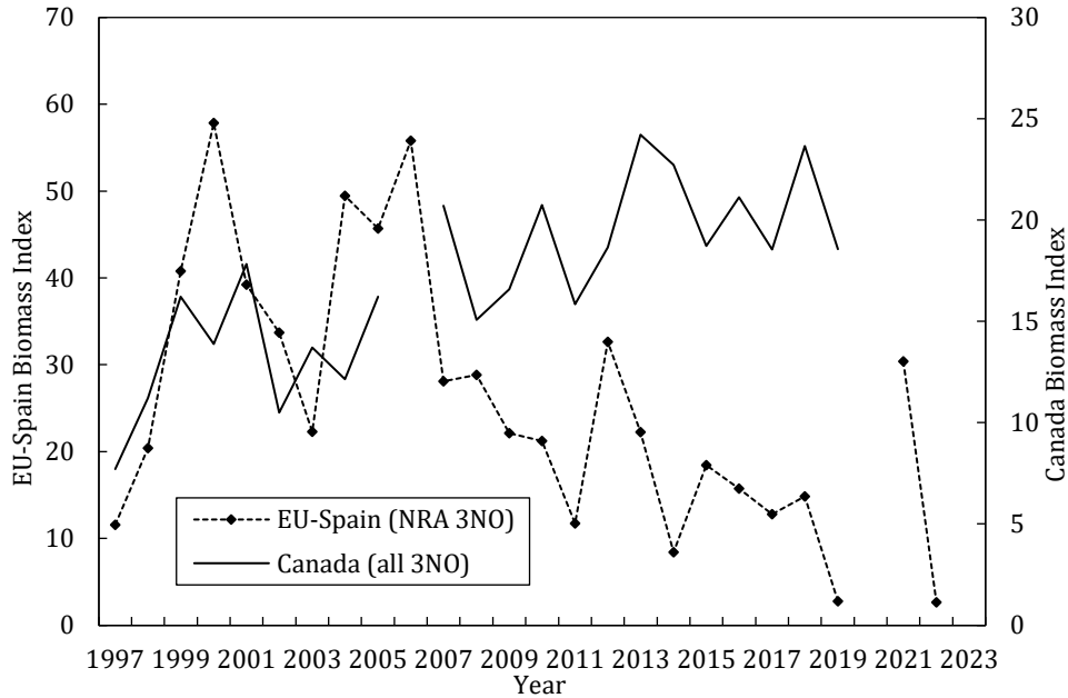
Figure 16.4. Thorny skate in Divs. 3LNOPs: biomass indices from the EU-Spain survey and the Canadian spring survey (1997-2022).
