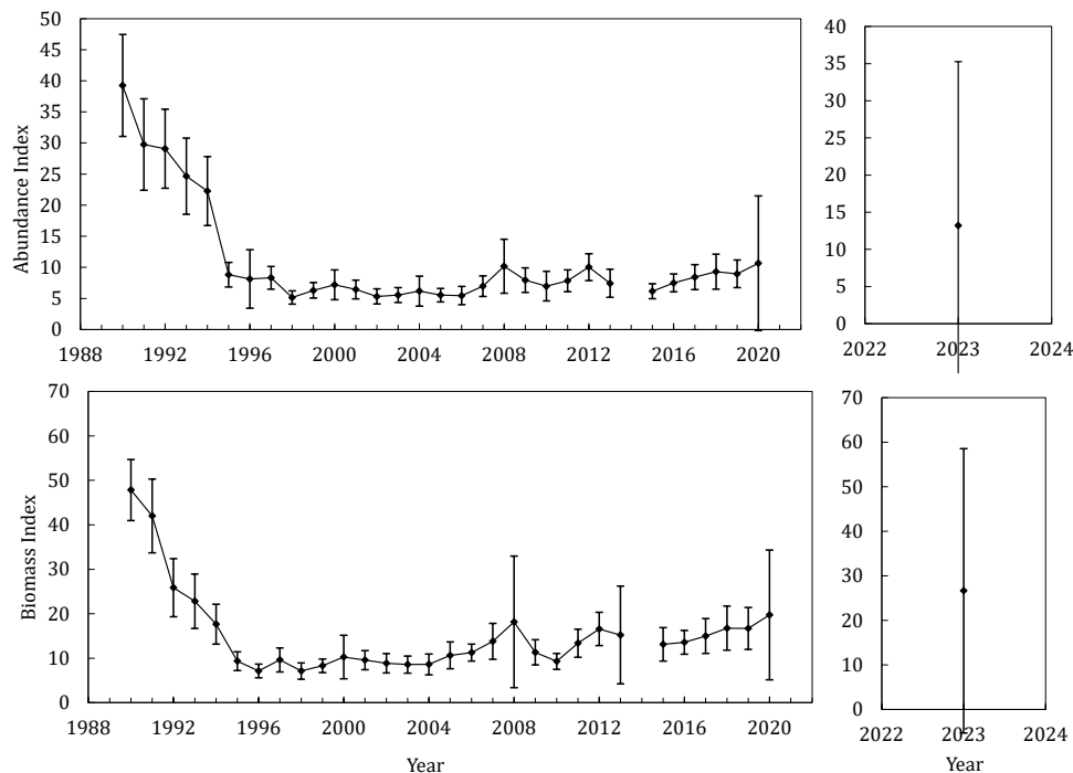
Figure 16.3. Thorny skate in Division 3LNOs: 1990-2020: abundance (top panel) and biomass (bottom panel) indices from Canadian autumn surveys in Division 3LNO. The survey was not conducted in 2021 or 2022.
