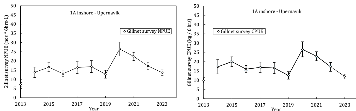
Figure 2.3.4. Greenland halibut in Division 1A inshore: gillnet survey NPUE (left) and CPUE (right) +/- SE.
