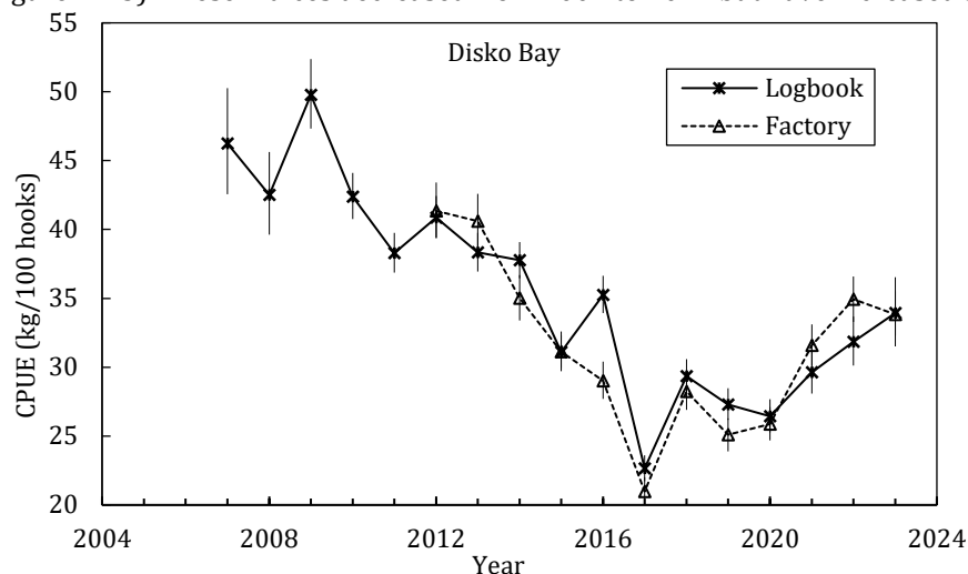
Figure 2.1.3. Greenland halibut in Division 1A inshore: Commercial CPUE from logbooks (vessels) and factory data (vessels, boats and ice fishery) fishing in Disko Bay.
