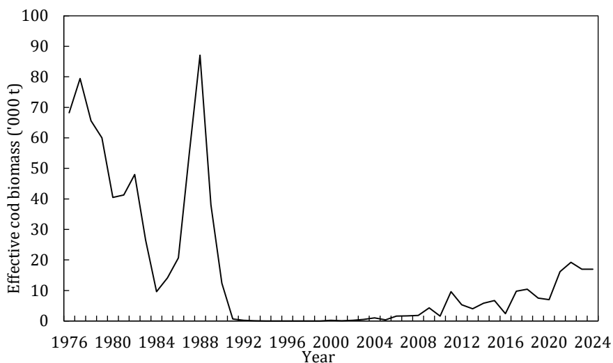
Figure 3.7. Northern shrimp in Subarea 0 and Subarea 1: Indices of the 'effective' cod biomass in Subarea 1 and Division 0A, 1976 - 2024.
