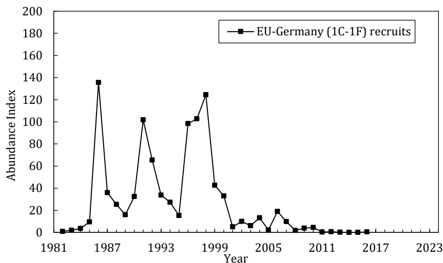
Figure 3.4. Juvenile redfish abundance indices for the EU-Germany survey ( Sebastes spp. <17cm).
