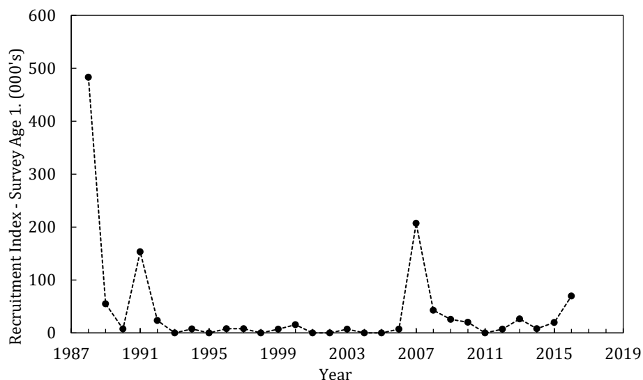
Figure 8.3. American plaice in Division 3M: Recruitment index, trends in survey age 1 abundance.
