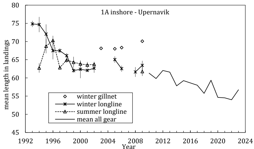
Figure. 2.3.2. Greenland halibut in Division 1A inshore: mean length in landings from longline fishery by season (summer and winter) and after 2010 overall mean taking account of fishing ground, season and gear.
