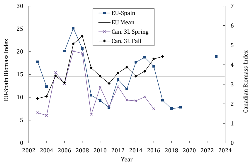
Figure 16.5. Thorny skate in Divisions 3LNOPs: Biomass indices from EU-Spain Division 3L survey and the Canadian spring and autumn surveys of Division 3L in 2003-2023. The Canadian spring and fall surveys conducted in 2022 and 2023 are not comparable to the earlier time series.
