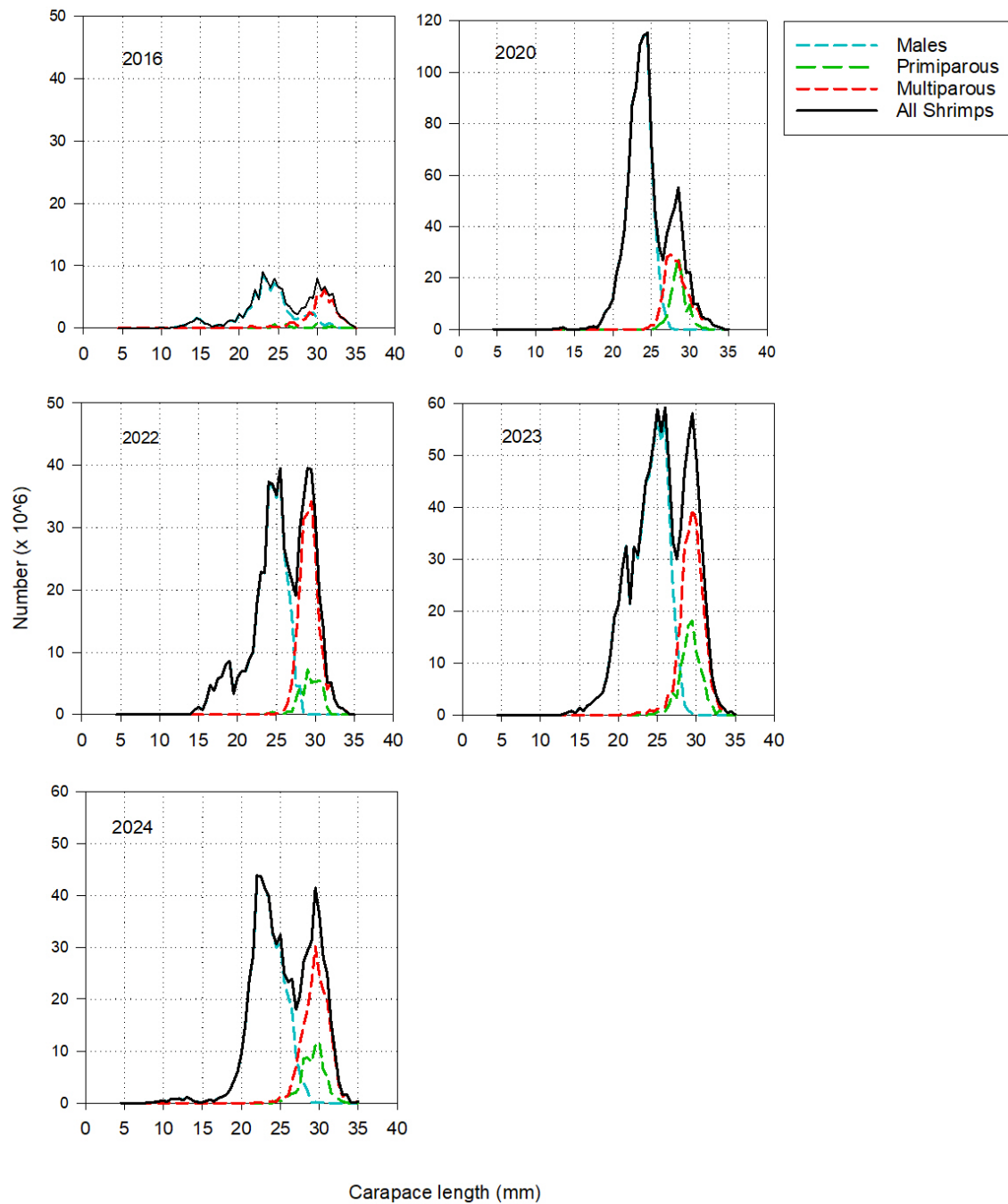
Figure 4.6. Northern shrimp in Denmark Strait and off East Greenland: Numbers of shrimp by length group (CL) in the total survey area in 2016 - 2024. No survey was carried out in the period 2017 - 2019 and in 2021.
