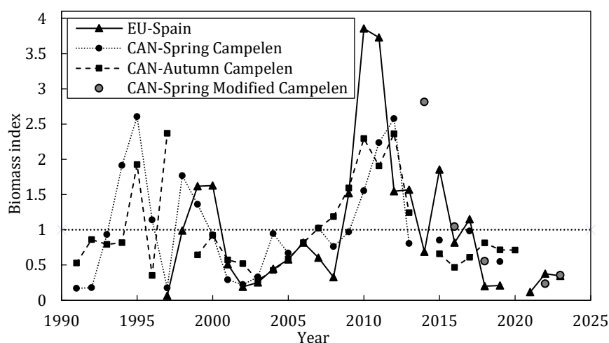
Figure 15.2. Redfish in Division 30: Survey biomass indices from Canada and EU-Spain. Indices were normalized by dividing by their time-series means. The CAN-Autumn survey in 2023 is not presented as it is a single year of a new series.
