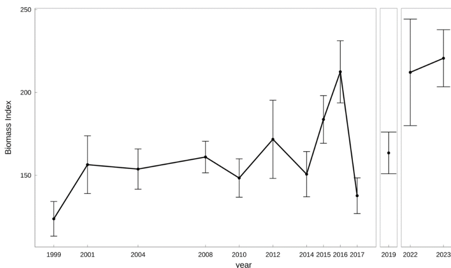
Figure 1.4. Greenland halibut in Subareas 0+1 (offshore): Divisions 0A-South and Divisions 1CD combined biomass index from surveys with the R/V Paamiut and Alfredo 3 gear (left panel), C/V Helga Maria and Alfredo 3 gear (middle panel) and R/V Tarajó and Bacalao 476 gear (right panel).
