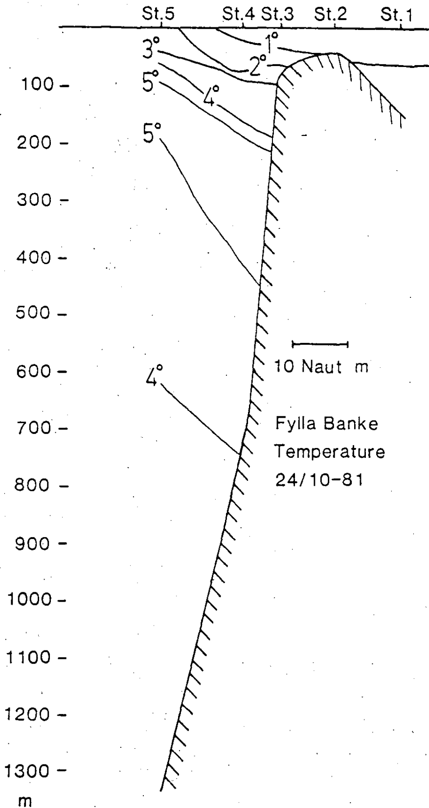
Figure 9 b. Temperature distribution across Fylla Bank in October.
