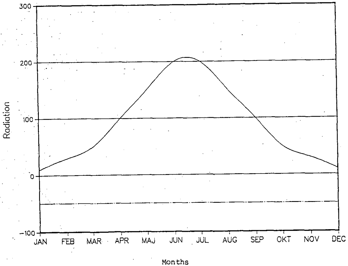
Figure 6. Incoming shortwave and outgoing longwave radiation throughout the year at West Greenland.
