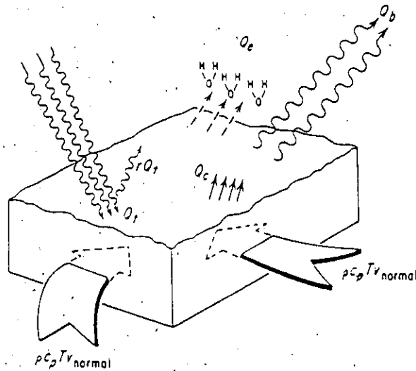
Figure 1. Quantities that are involved in the computation of the heat budget of the oceans. Q_s is the short wave radiation reaching the sea surface, rQ_s is the short wave radiation reflected from the sea surface, Q_e is the heat lost from the sea surface by evaporation, Q_b is the net loss of heat from the sea surface due to long-wave radiation, Q_c is the heat lost, or gained, by convection, and \rho C_p T_v normal is the heat transported normal to the boundary walls. After Neumann and Pier-son (1966).
