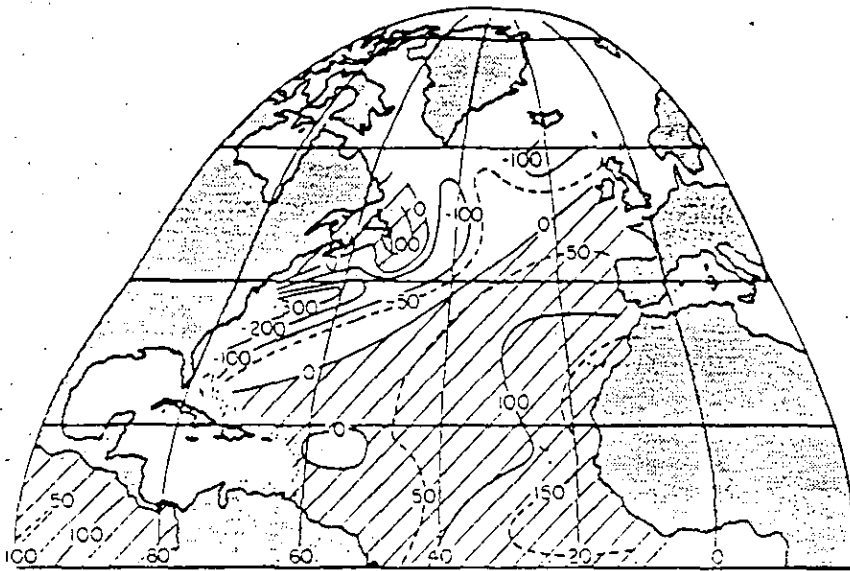
Figure 5. Net annual radiation surplus of the ocean minus annual heat deliveries to the atmosphere (gram calories per square centimeter per day) (from Sverdrup, 1942).
