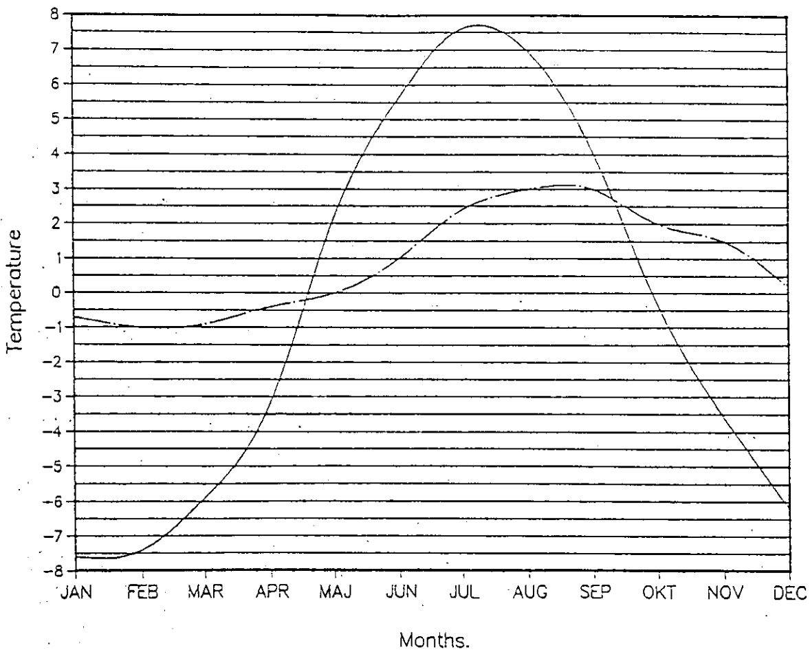
Figure 7. Mean air and seasurface temperatures from the Fylla Bank area, West Greenland.
