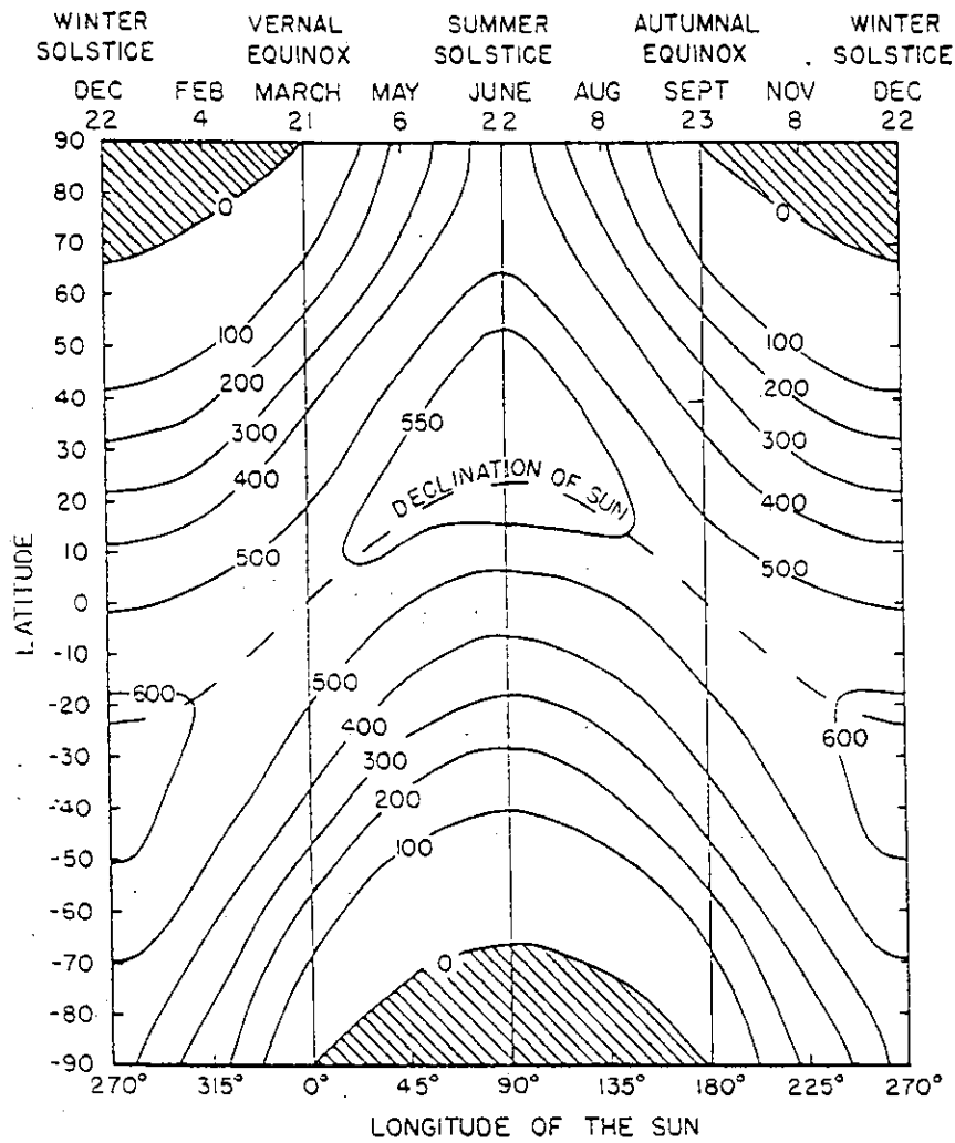
Figure 3. Solar radiation in \text{ly day}^{-1} arriving at the earth's surface when the atmosphere transmits 0.7 of a vertical beam. After Hess (1966).
