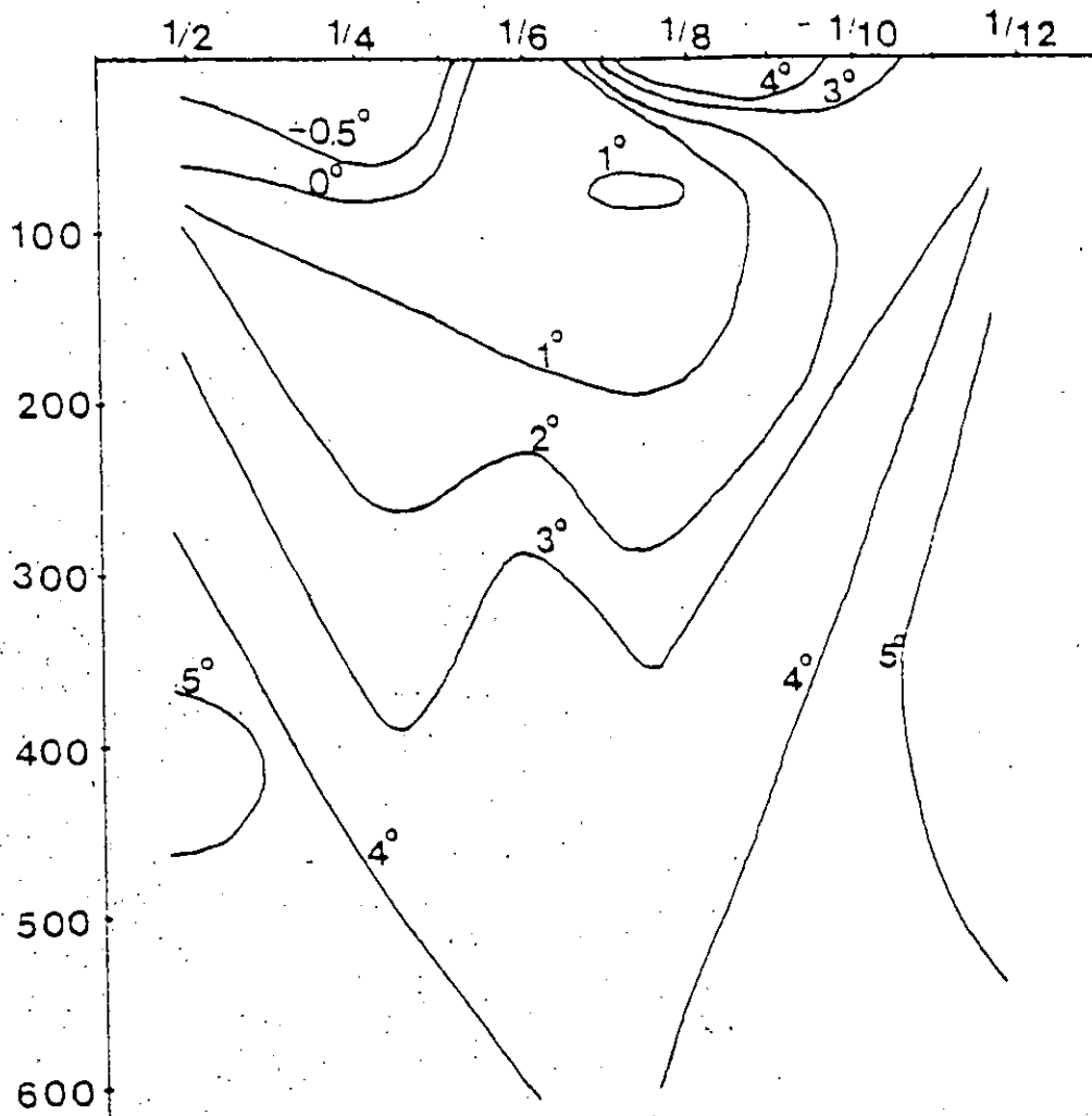
Figure 8. Temperature distribution just west of Fylla Bank in 1974.
