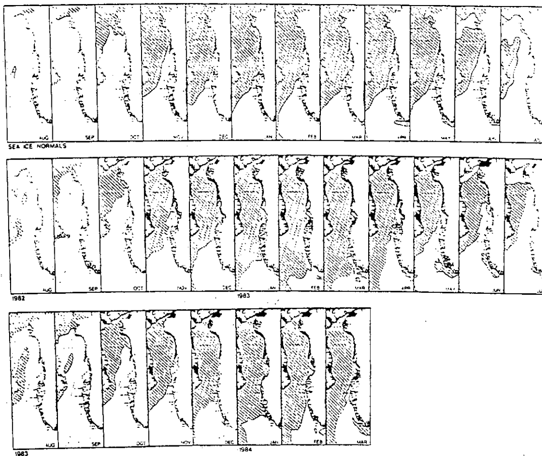
Fig. 10 Sea ice distribution in the Davis Strait. Upper row: normal distribution. Middle and lower row: distribution in the period August 1982 to March 1984.
