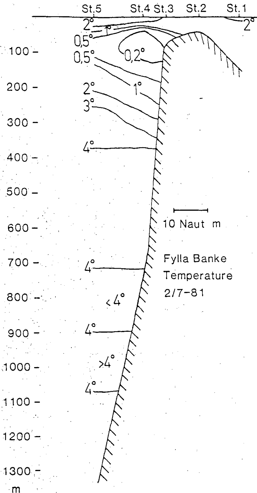
Figure 9 a. Temperature distribution across Fylla Bank in July.
