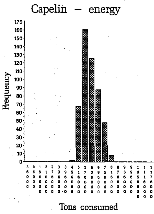
Fig. 3. Frequency distributions of 500 realizations of capelin consumption taking into account uncertainty in population size, residency, energy requirements and diet.
