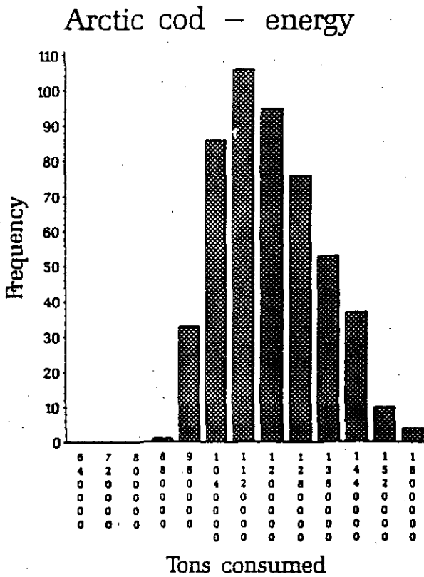
Fig. 4. Frequency distributions of 500 realizations of Arctic cod consumption taking into account uncertainty in population size, residency, energy requirements and diet.
