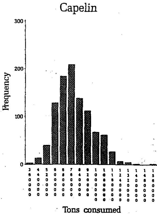
Fig. 5. Plot of 50 realizations of cod consumption trajectories over the period 1981 to 1994 together with frequency distributions of cod, capelin and Arctic cod consumption from 1000 realizations taking into account all four sources of uncertainty simultaneously.
