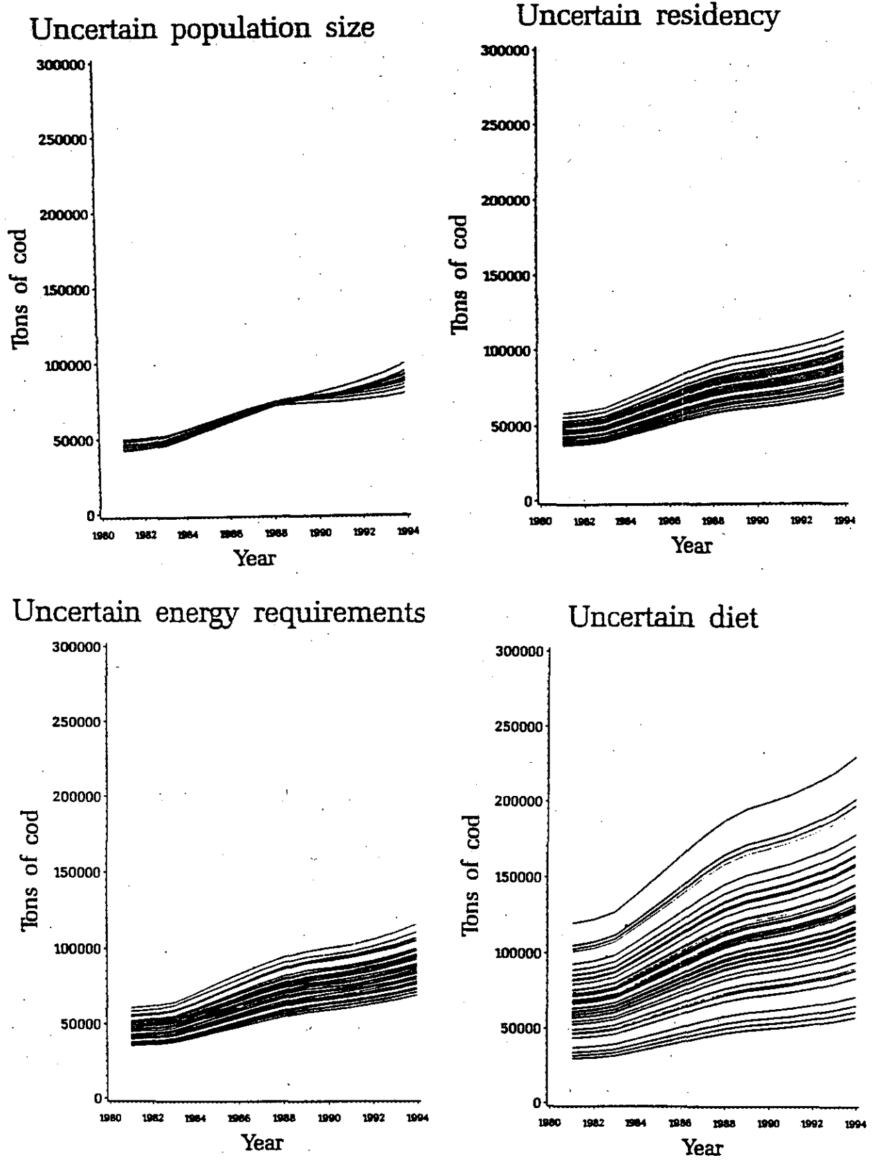
Fig. 1. Plots of 50 realizations of cod consumption trajectories for the period 1981 to 1994 taking into account uncertainty in population size, residency, energy requirements and diet.
