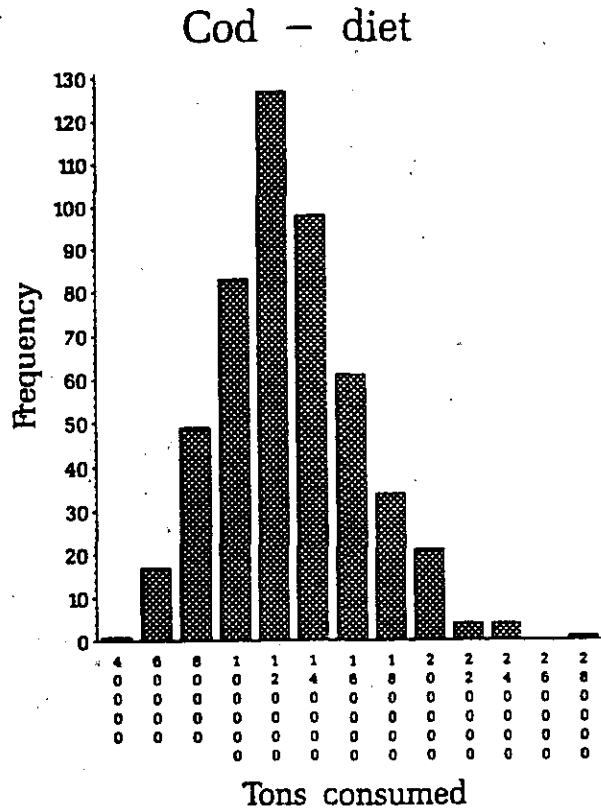
Fig. 2. Frequency distributions of 500 realizations of cod consumption taking into account uncertainty in population size, residency, energy requirements and diet.
