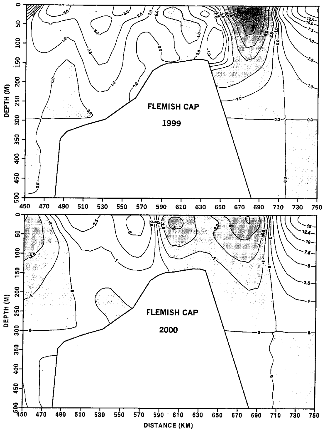
Fig. 12. The vertical distribution of the N-S geostrophic current field in cm/s over the Flemish Cap during July of 1999 and 2000 calculated from the density data. Negative (shaded) currents are southward and positive are northward.
