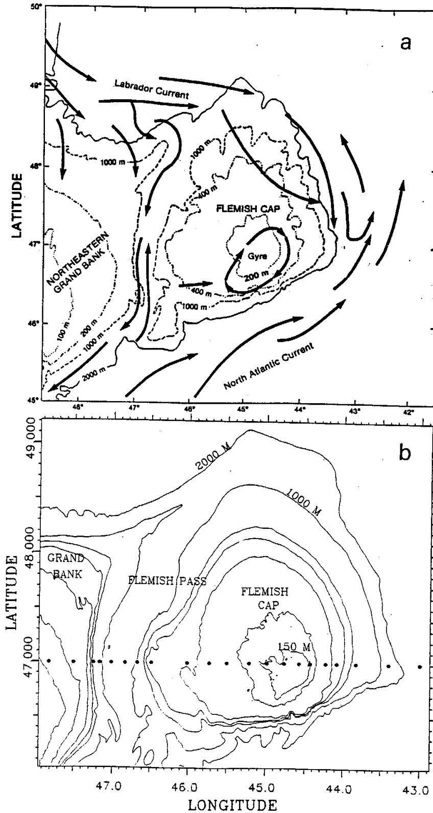
Fig. 1. (a) The major circulation features around the Flemish Cap area (Adapted from Anderson, 1984) and (b) the location of stations occupied during the summer of 1999 and 2000. Bathymetry lines are 2000, 1000, 500, 400, 300, 200 and 150 m.
