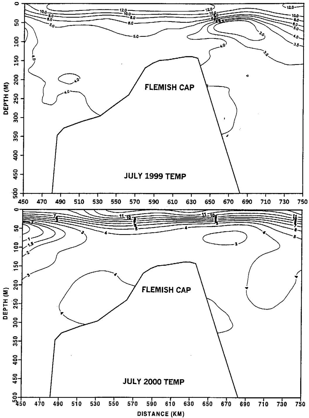
Fig. 3. The vertical distribution of temperature over the Flemish Cap (along 47^{\circ}\text{N} ) for July of 1999 and 2000.
