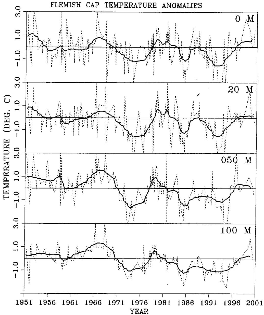
Fig. 5. Time series of monthly temperature anomalies at standard depths of 0, 20, 50 and 100 m on the Flemish Cap in NAFO Division 3M. The solid line represents the smoothed temperature anomalies.
