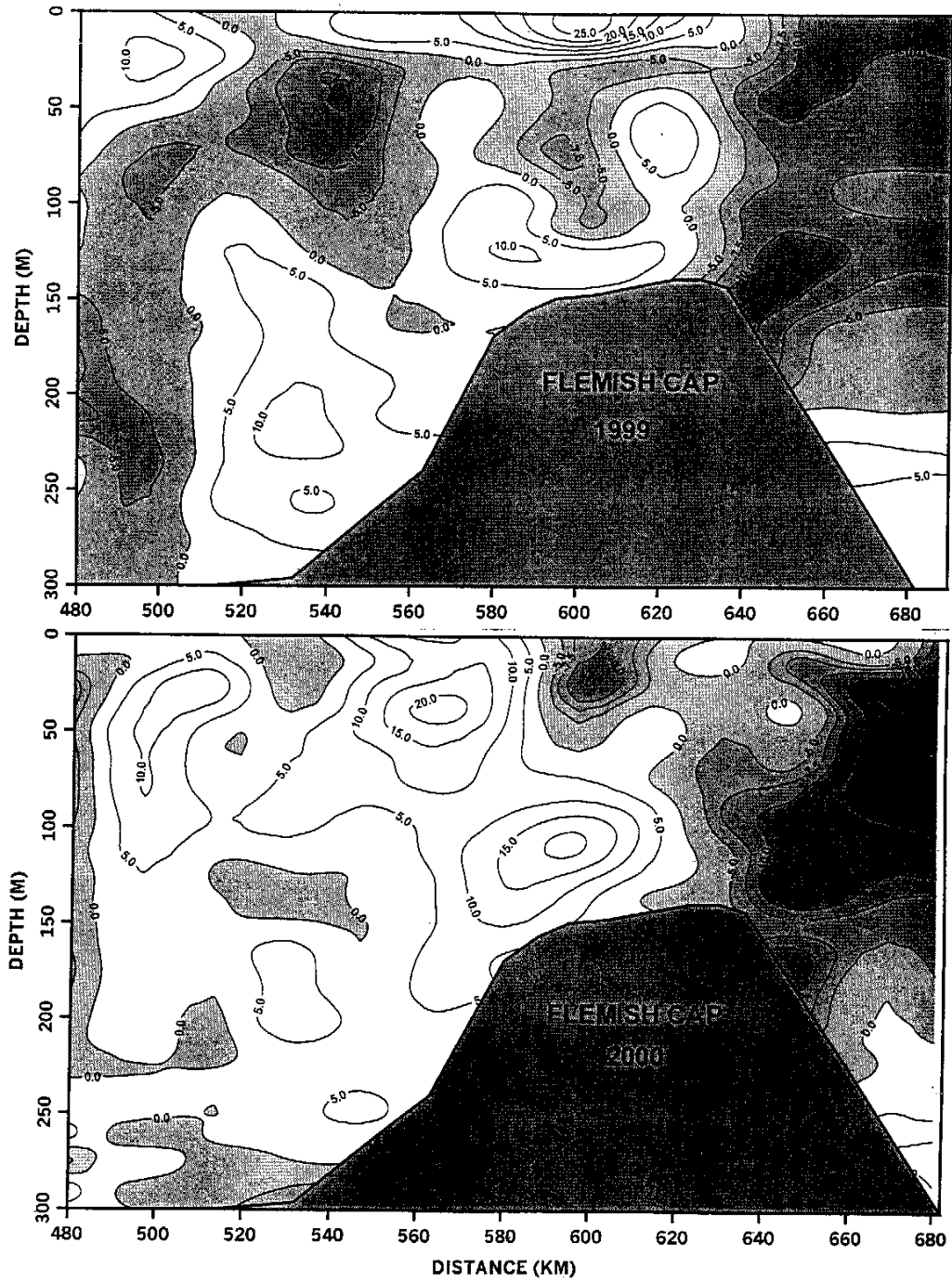
Fig. 11. A vertical cross-section of the N-S current field in cm/s over the Flemish Cap (along 47^{\circ} N) during July of 1999 and 2000 measured with a 150 kHz ADCP. Negative (shaded) currents are southward and positive are northward.
