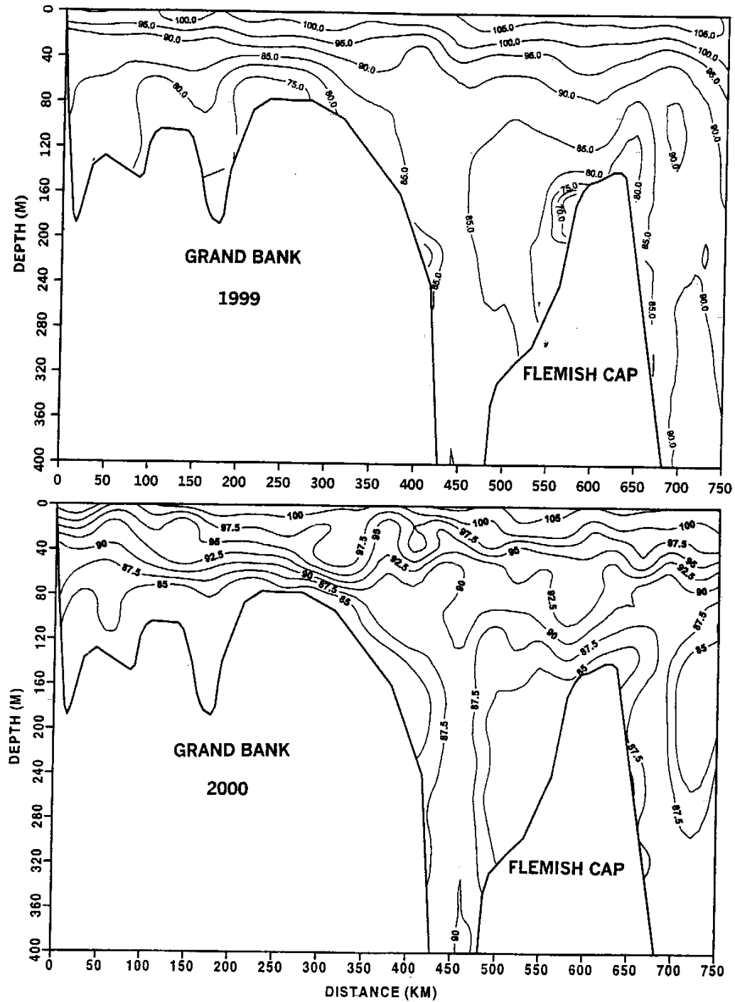
Fig. 10. The vertical distribution of dissolved oxygen percent saturation along 47^{\circ}\text{N} for July of 1999 and 2000.
