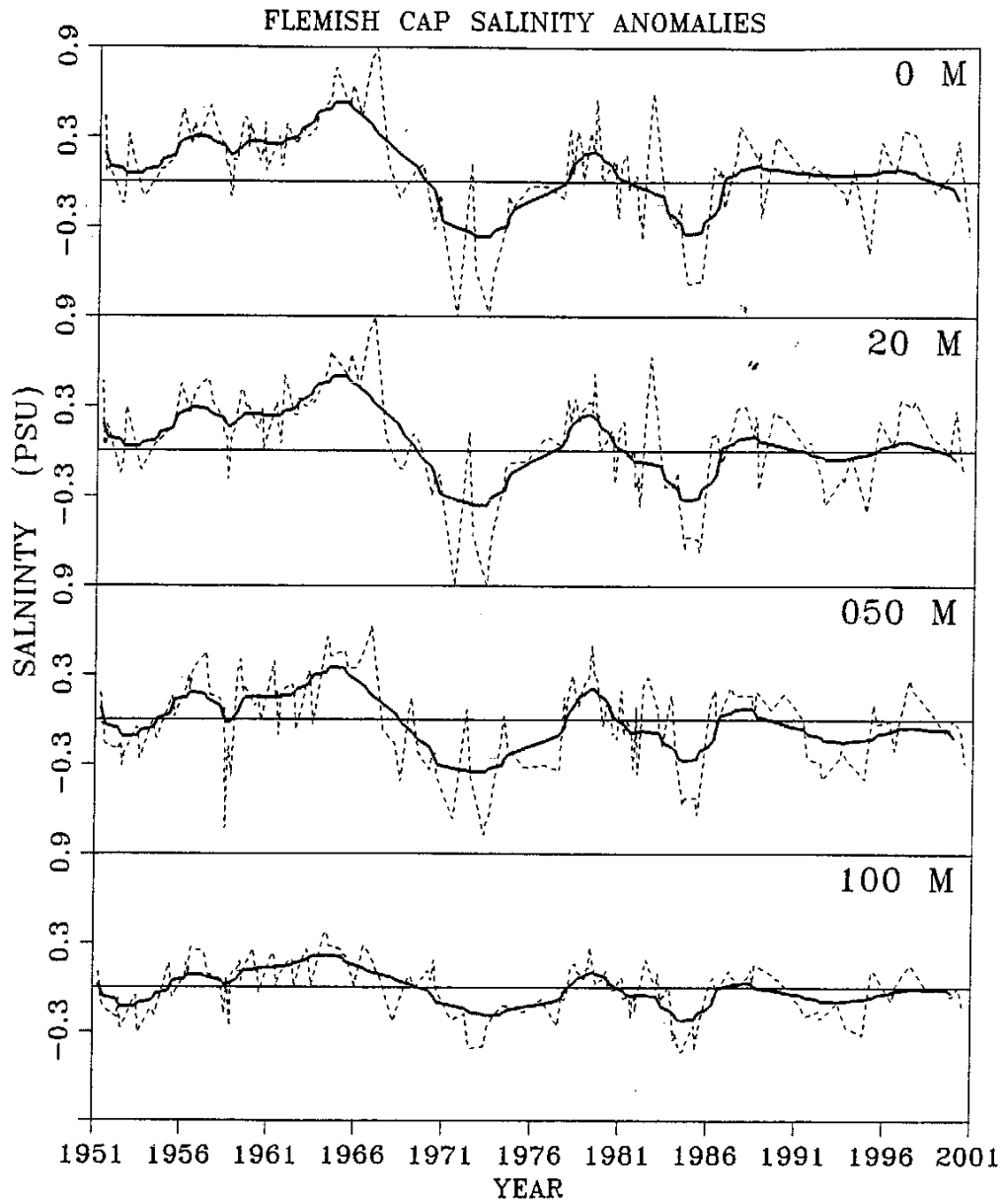
Fig. 8. Time series of monthly salinity anomalies at standard depths of 0, 20, 50 and 100 m on the Flemish Cap in NAFO Division 3M. The solid line represents the smoothed salinity anomalies.
