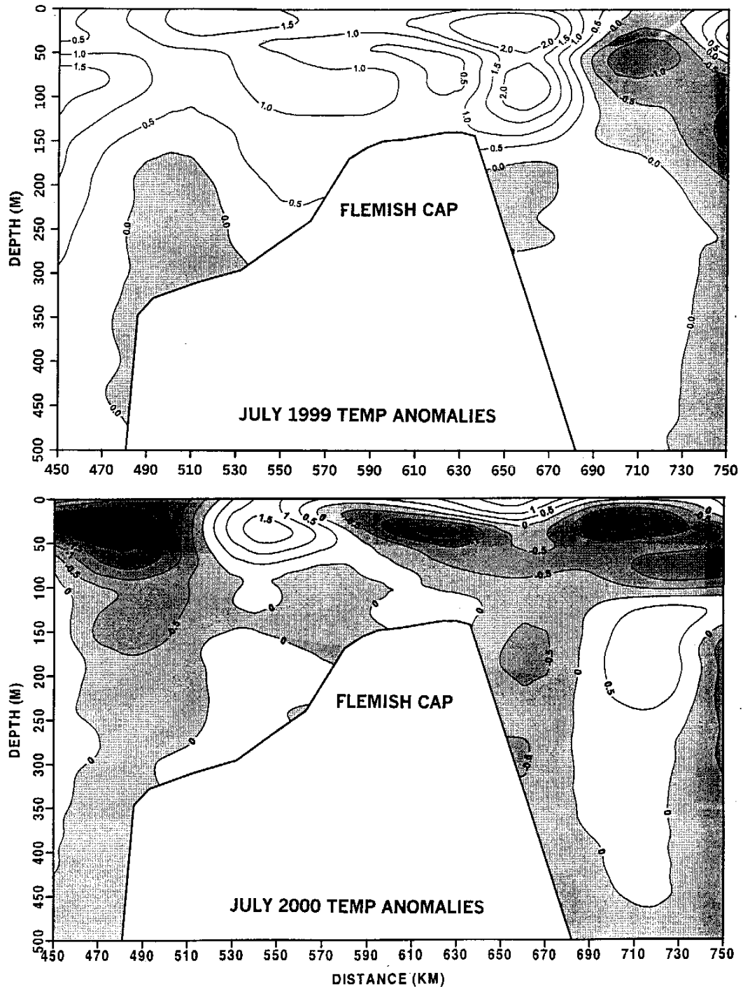
Fig. 4. The vertical distribution of temperature anomalies over the Flemish Cap (along 47^{\circ} N) for July of 1999 and 2000. Negative anomalies are shaded.
