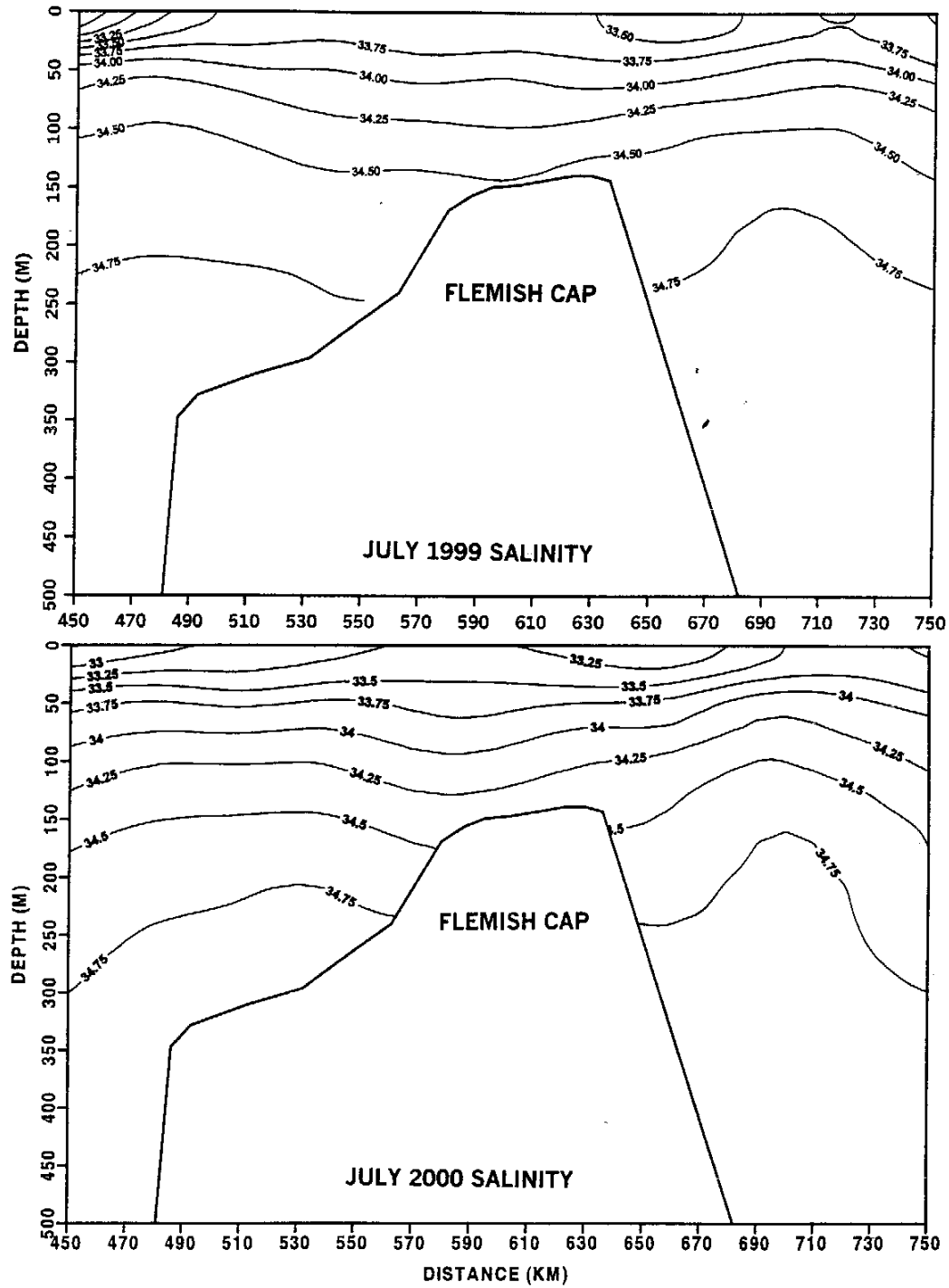
Fig. 6. The vertical distribution of salinity over the Flemish Cap (along 47^{\circ}\text{N} ) for July of 1999 and 2000.
