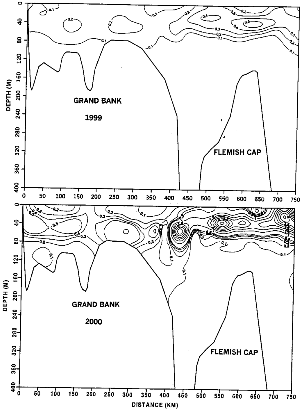
Fig. 9. The vertical distribution of chlorophyll concentrations (mg/l) along the 47°N transect for July of 1999 and 2000.
