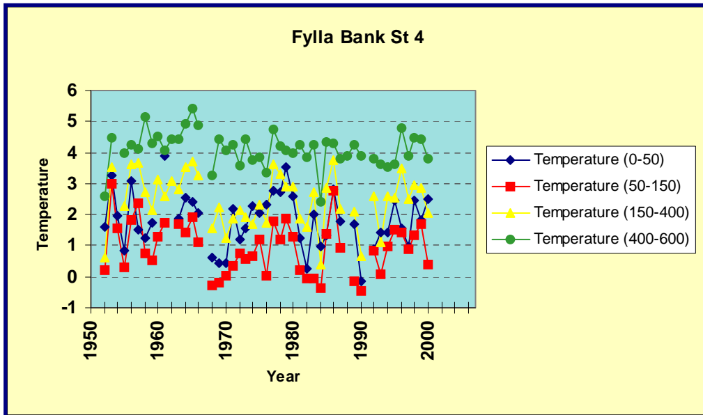
Fig. 8. Time-series of: a) mean temperature, and b) mean salinity in four depth intervals at Fylla Bank St. 4, primo July.
