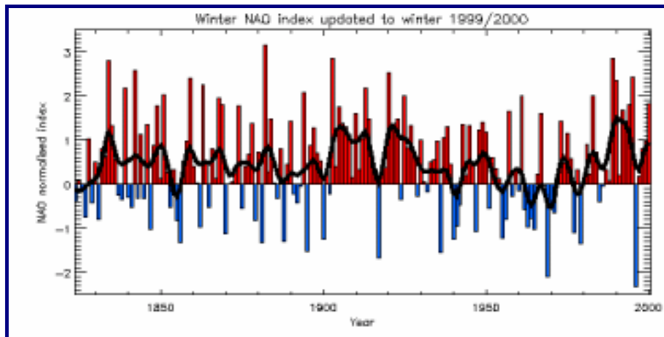
Fig. 1. Time series of the winter NAO (December to March average). After Jones et al. (1997) updated to the winter 1999/2000.
