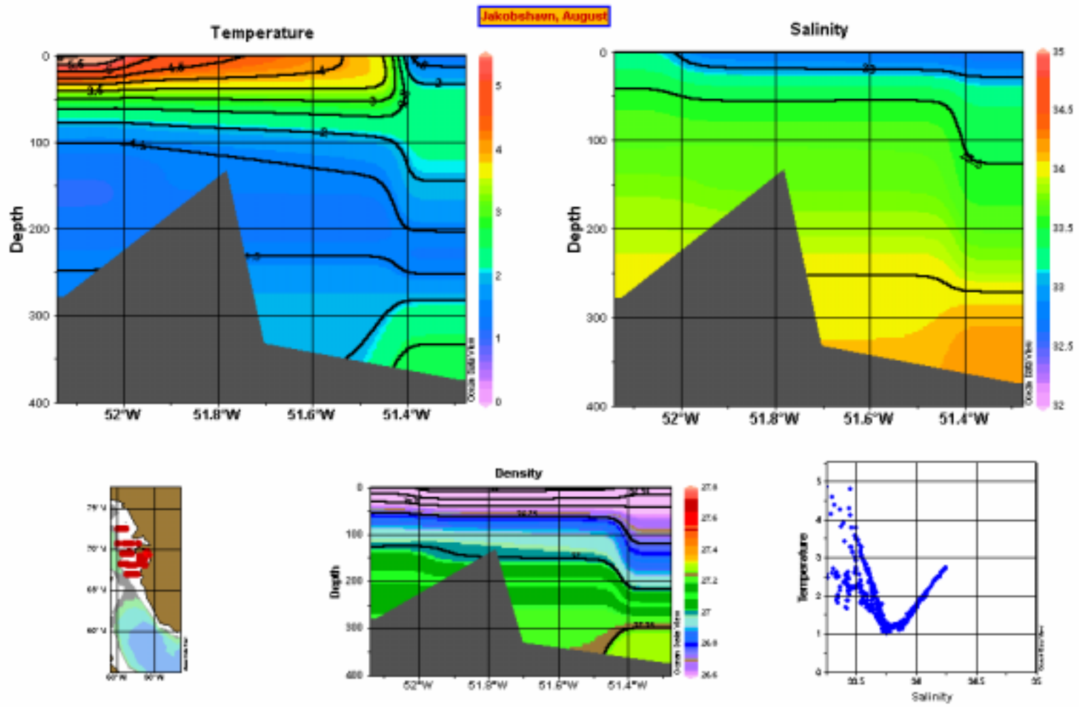
Fig. 20. Vertical distribution of temperature, salinity and density at the Jakobshavn Section, August 24, 2000
