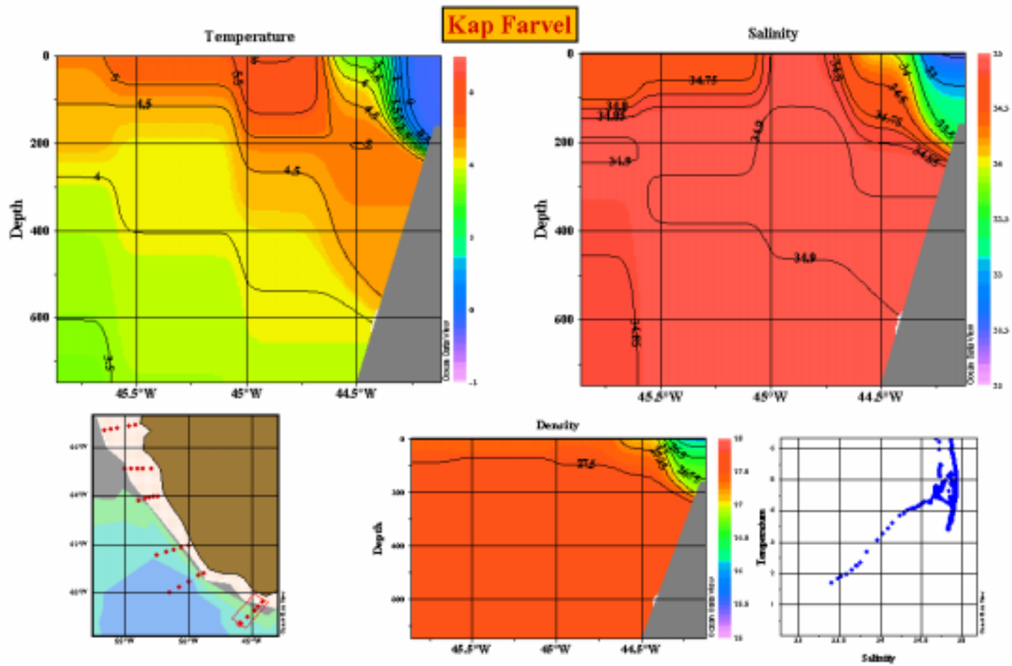
Fig. 10. Vertical distribution of temperature, salinity and density at the Cape Farewell section, June 29, 2000.
