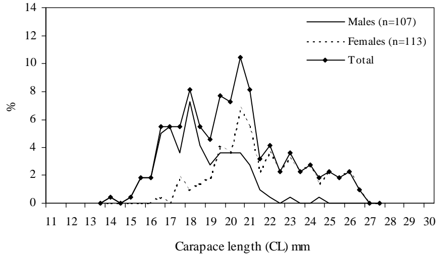
Fig. 4. Length frequency distributions (%) of northern shrimp in Div. 1B by sex and gear.
