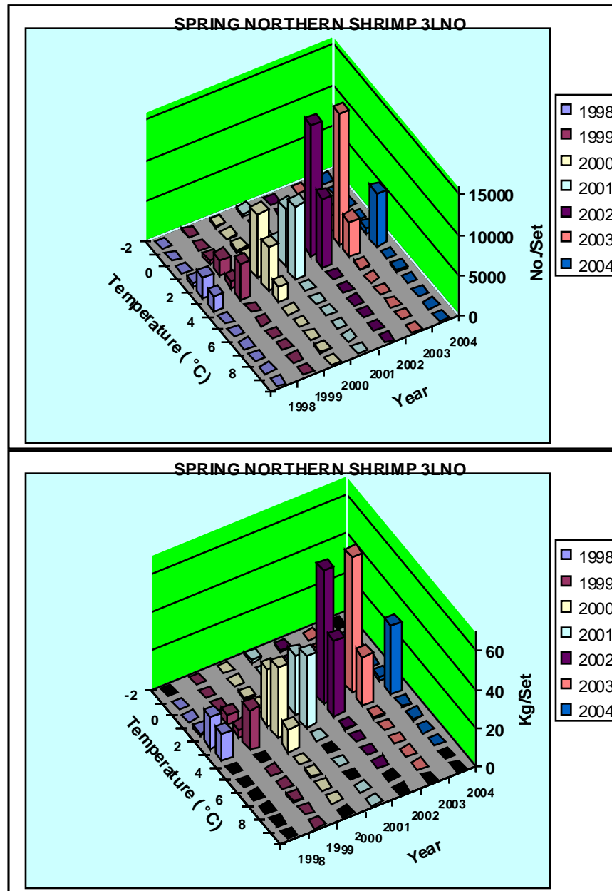
Fig. 2. The average number (top panel) and weight (bottom panel) of northern shrimp per fishing set in 1°C temperature bins for the spring surveys in NAFO Div. 3LNO for the years 1998-2004.
