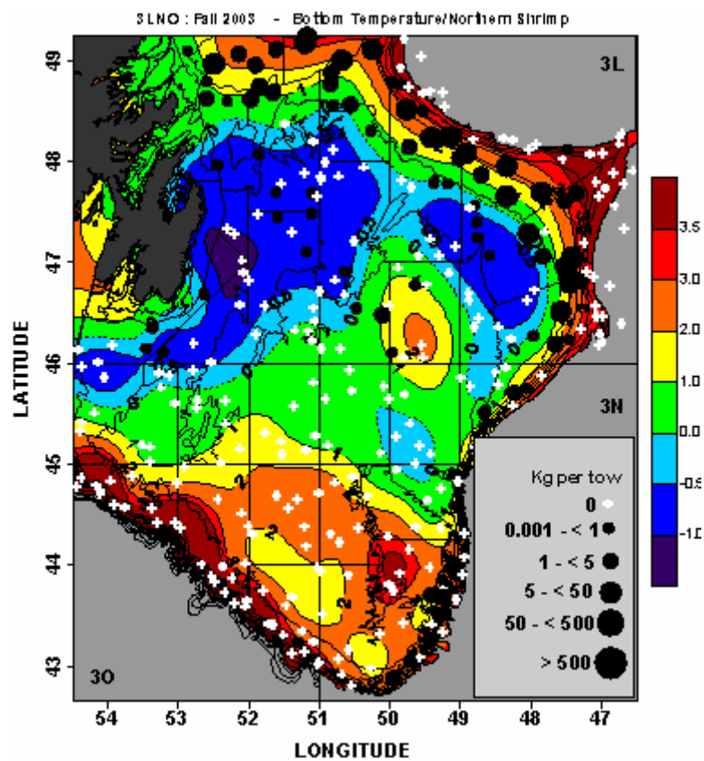
Fig. 11. (Cont.). Bottom temperature contour maps (in °C) for the fall of 2003 from the annual 3LNO survey and the weight of shrimp in each fishing set shown as solid circles. The white crosses represent zero catches
