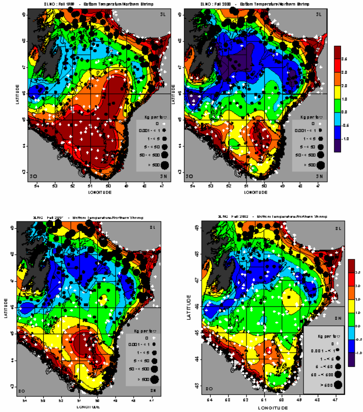
Fig. 11. (Cont.). Bottom temperature contour maps (in °C) for the fall of 1999-2002 from the annual 3LNO survey and the weight of shrimp in each fishing set shown as solid circles. The white crosses represent zero catches.
