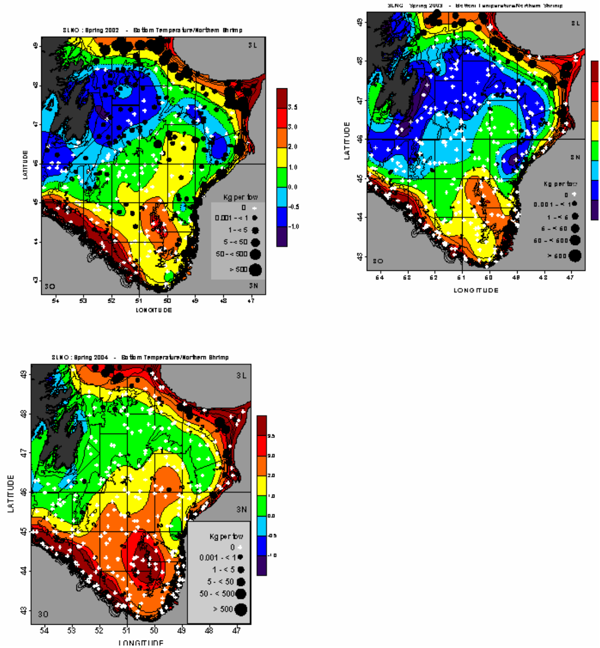
Fig. 9. (Cont.). Bottom temperature contour maps (in °C) for the spring of 2002-2004 from the annual 3LNO survey and the total weight of shrimp in each fishing set shown as solid circles. The white crosses represent zero catches.
