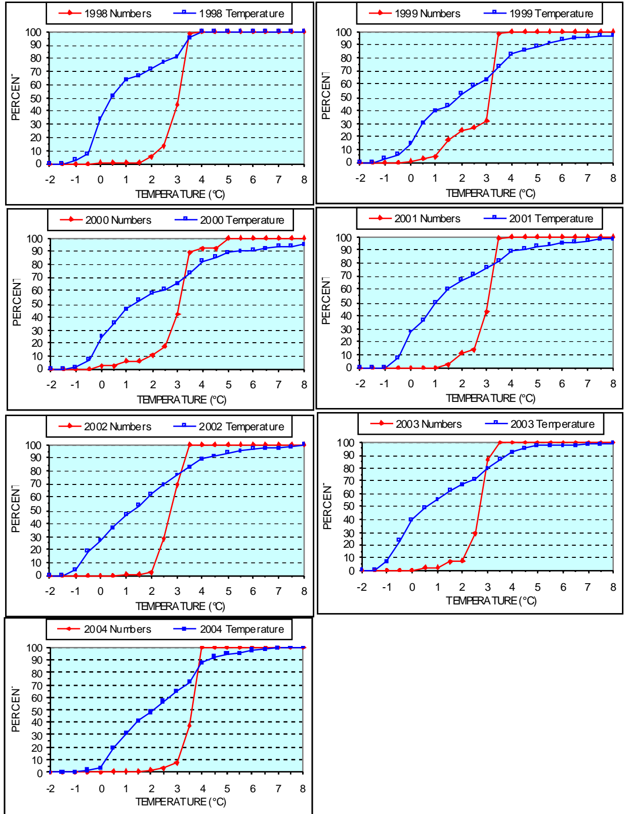
Fig. 4. Cumulative frequency distributions of the number of sets in the 3LNO survey in 1°C temperature bins and the cumulative frequency distribution of the number of shrimp caught in 1°C temperature bins for the spring surveys from 1998-2004.
