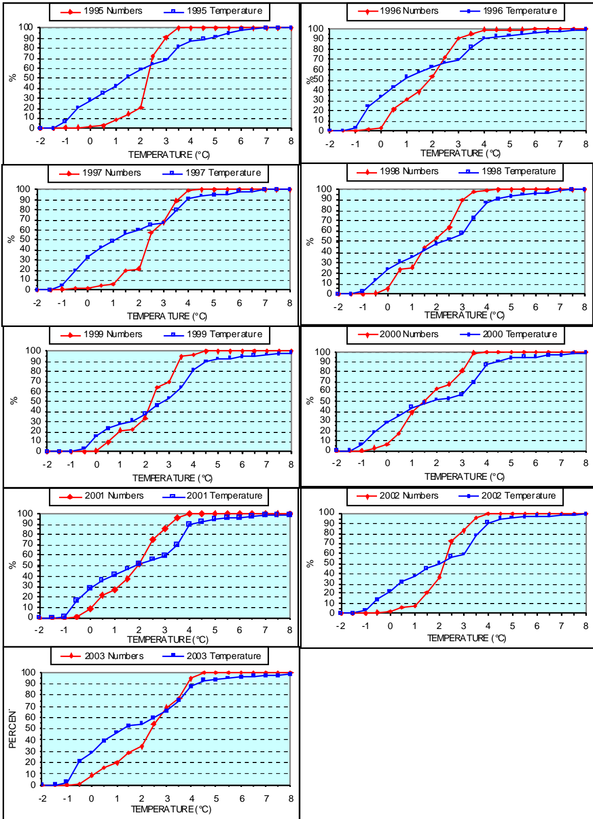
Fig. 5. Cumulative frequency distributions of the number of sets in the 3LNO survey in 1°C temperature bins and the cumulative frequency distribution of the number of shrimp caught in 1°C temperature bins for the fall surveys from 1995 to 2003.
