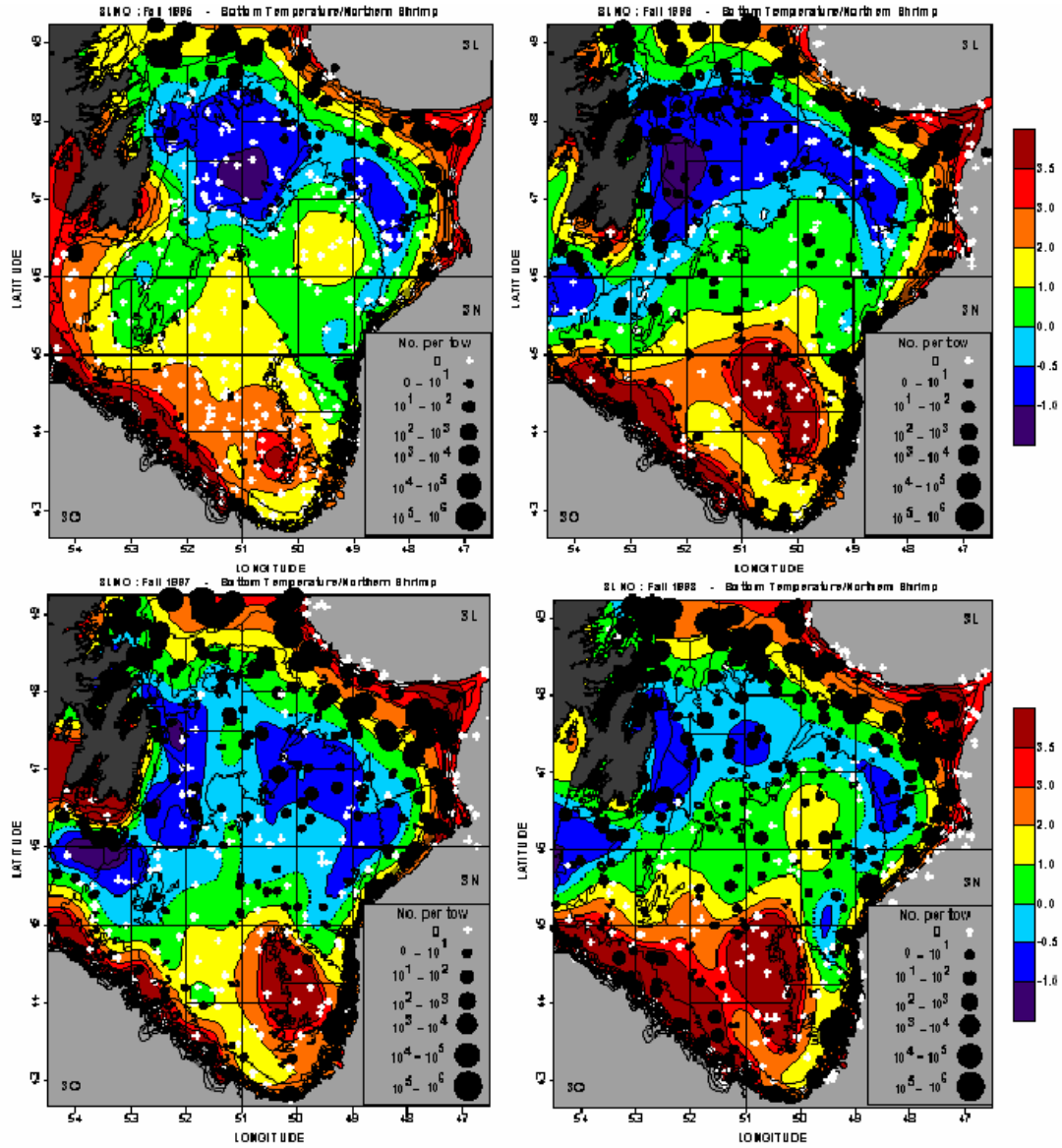
Fig. 10. Bottom temperature contour maps (in °C) for the fall of 1995-1998 from the annual 3LNO survey. The numbers of shrimp in each fishing set are shown as solid circles. The white crosses represent zero catches.
