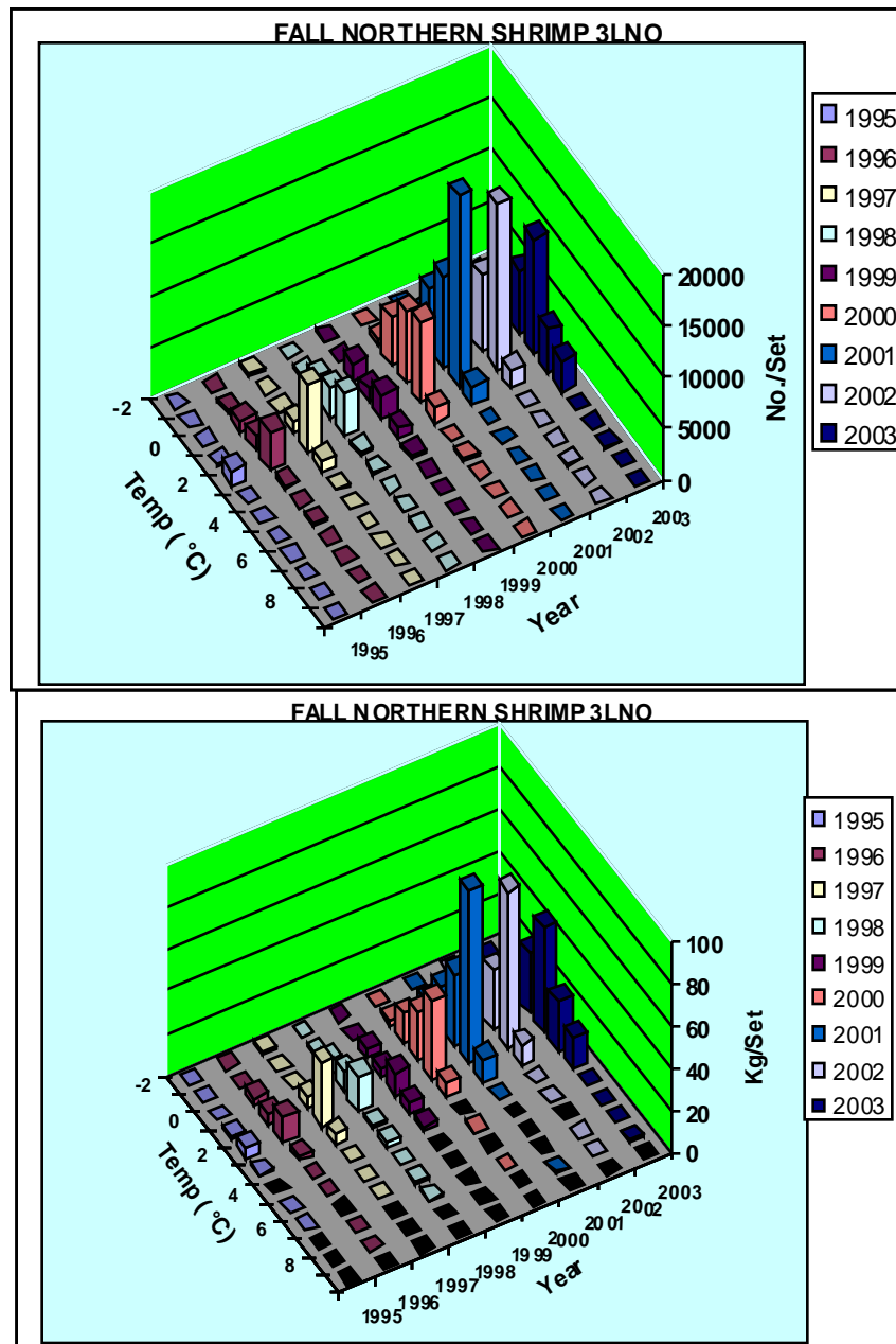
Fig. 3. The average number (top panel) and weight (bottom panel) of northern shrimp per fishing set in 1°C temperature bins for the fall surveys in NAFO Div. 3LNO for the years 1995-2003.
