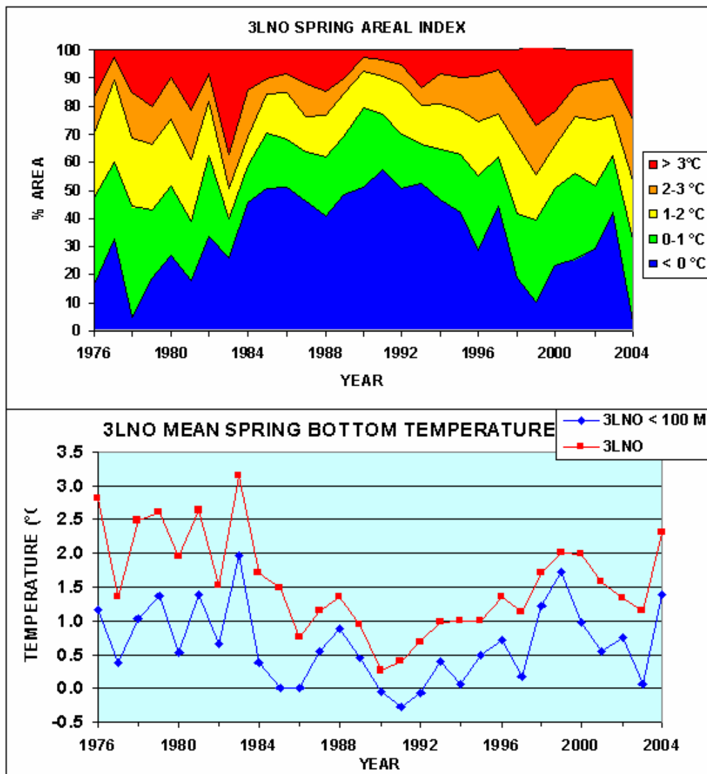
Fig. 7. Time series of the percentage area of the bottom in NAFO Div. 3LNO covered by water with temperatures \leq 0^{\circ}\text{C} , 0-1^{\circ}\text{C} , 1-2^{\circ}\text{C} , 2-3^{\circ}\text{C} and \geq 3^{\circ}\text{C} during spring (top panel) and the spatially averaged spring bottom temperature (bottom panel).
