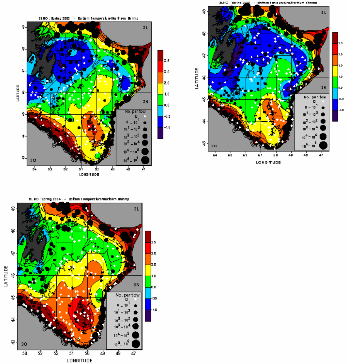
Fig. 8 (cont.). Bottom temperature contour maps (in °C) for the spring of 2002-2004 from the annual 3LNO survey and the numbers of shrimp in each fishing set shown as solid circles. The white crosses represent zero catches.
