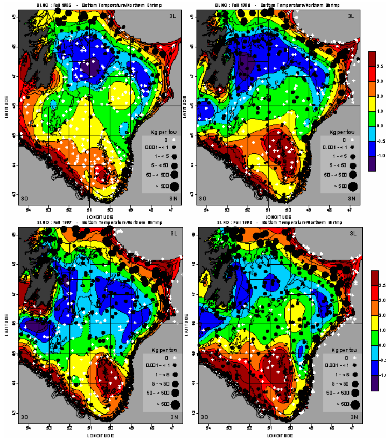
Fig. 11. Bottom temperature contour maps (in °C) for the fall of 1995-1998 from the annual 3LNO survey and the weight of shrimp in each fishing set shown as solid circles. The white crosses represent zero catches
