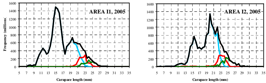
Fig. 6c. Length frequencies of northern shrimp in inshore areas I1 and I2 (Disko Bay / Vaigat) in 2005.
