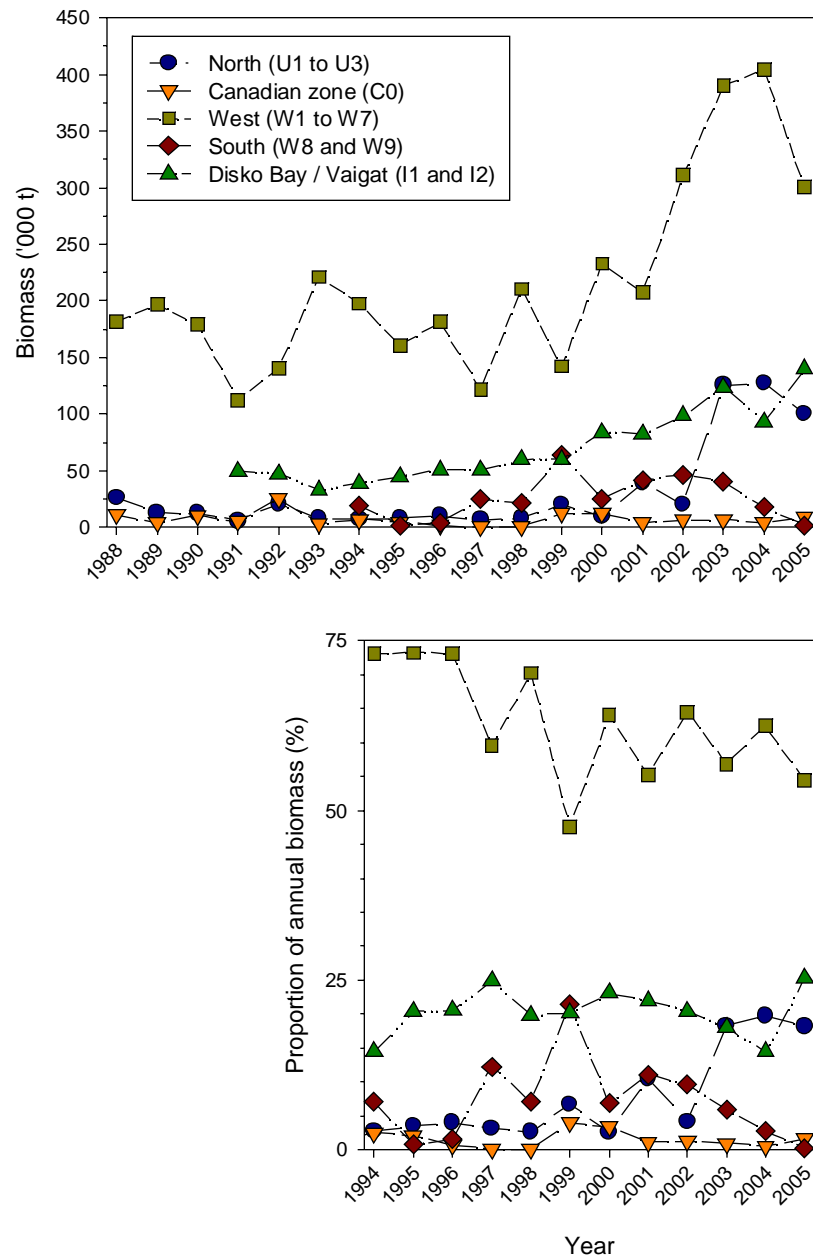
Fig. 4. Biomass in the five main survey regions 1988-2005 (area names are given in brackets, see Fig. 1 for location) and contribution of these regions to the total biomass 1994-2005.
