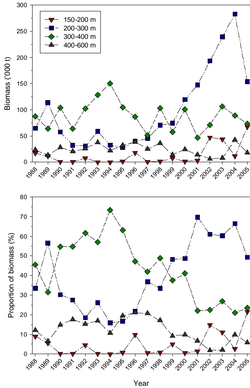
Fig. 5. Biomass distribution in the four depth strata in areas C and W1-W7 1988-2005.
