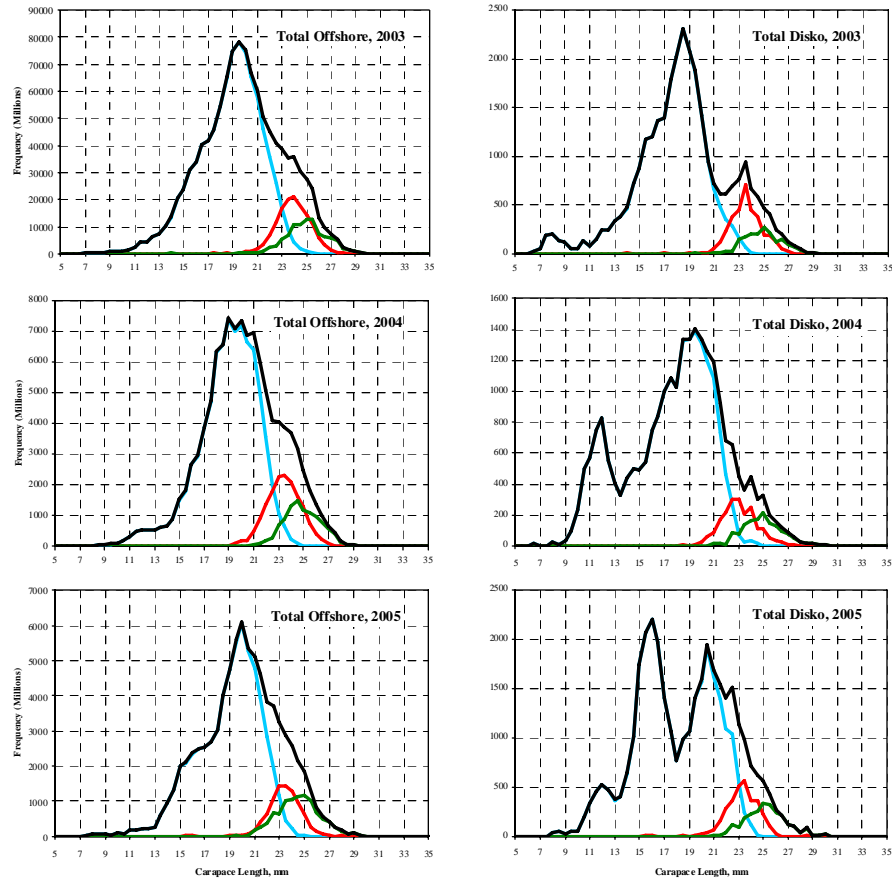
Fig. 7d. Length frequencies of northern shrimp in the total offshore and the Disko Bay/Vaigat area, 2003 to 2005 (2003 and 2004 data converted from Skjervøy to Cosmos trawl)
