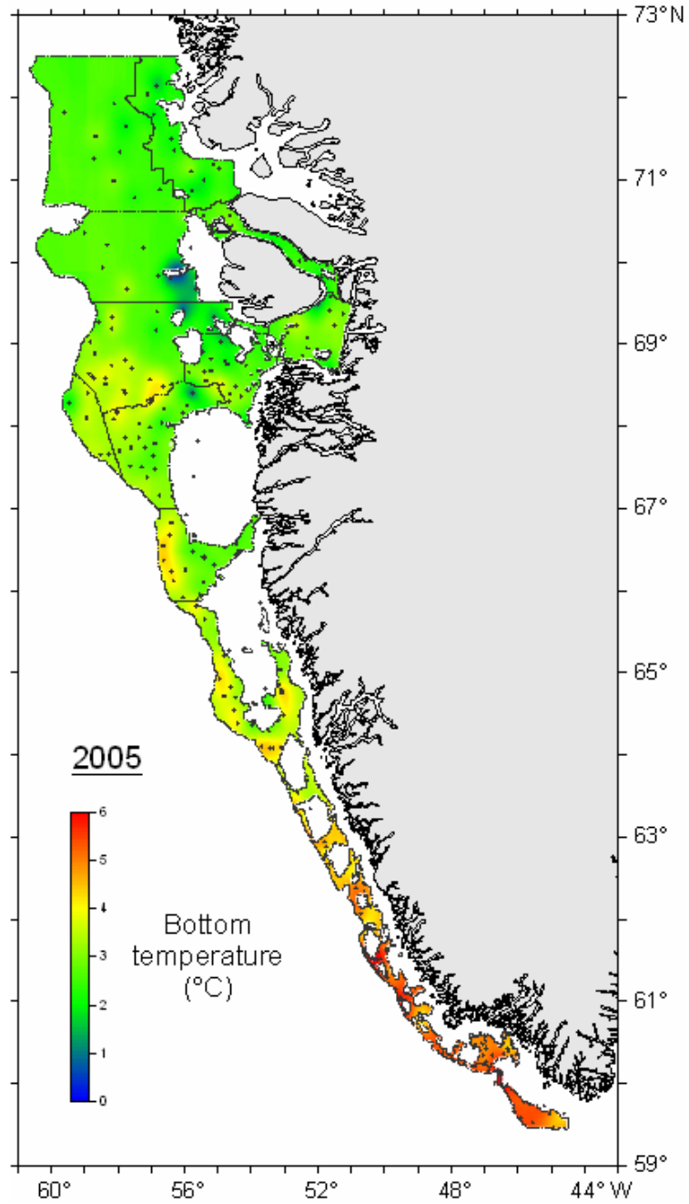
Fig. 14. Distribution of bottom temperature in the survey area between 150 and 600 m depth in 2005 (crosses indicate sampling locations).
