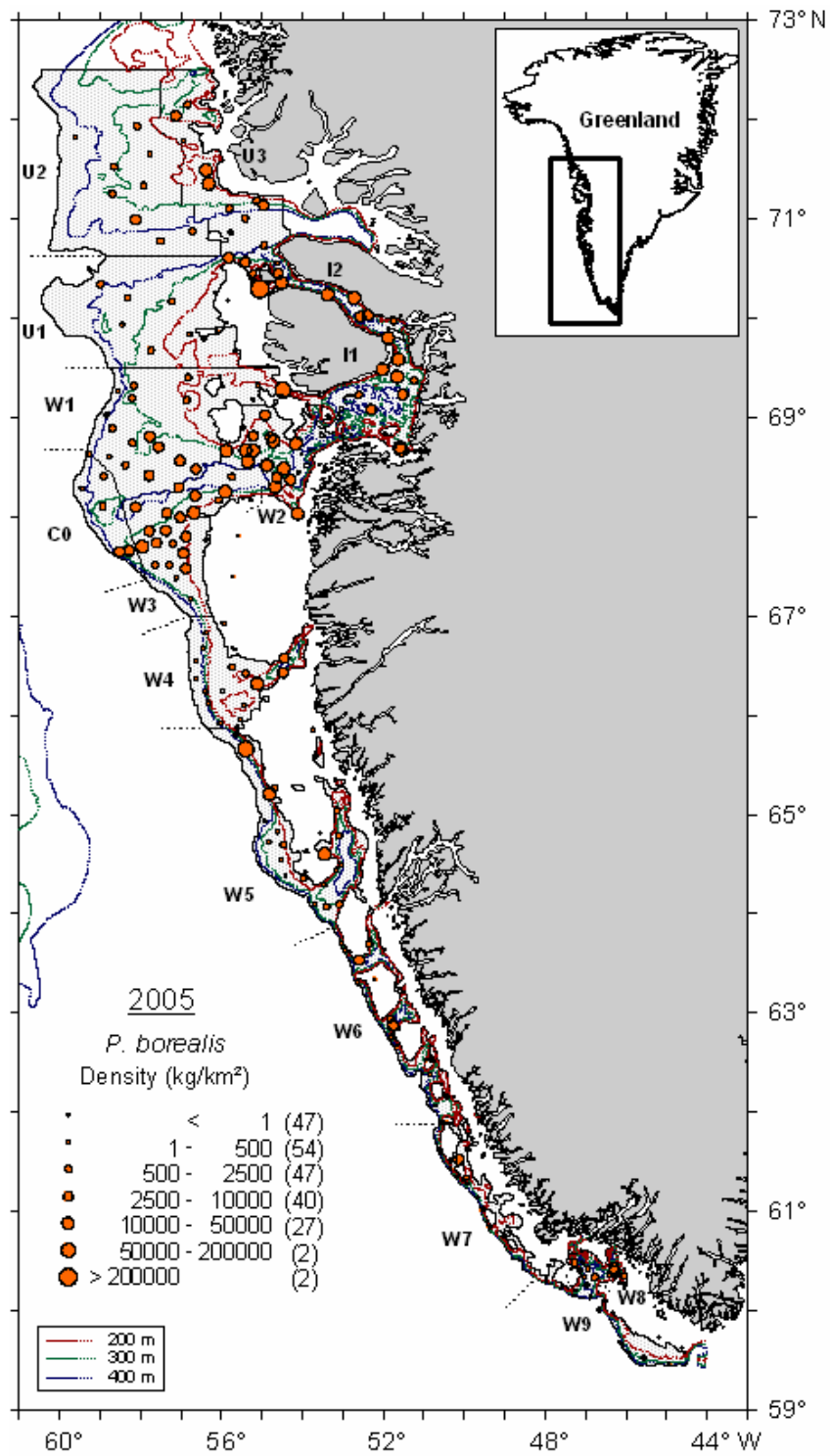
Fig. 1. Survey stratification and geographical distribution of northern shrimp density in 2005.
