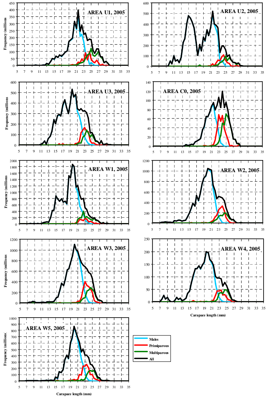
Fig. 6a. Length frequencies of northern shrimp in offshore areas U1 to U3, C0 and W1 to W5 in 2005.
