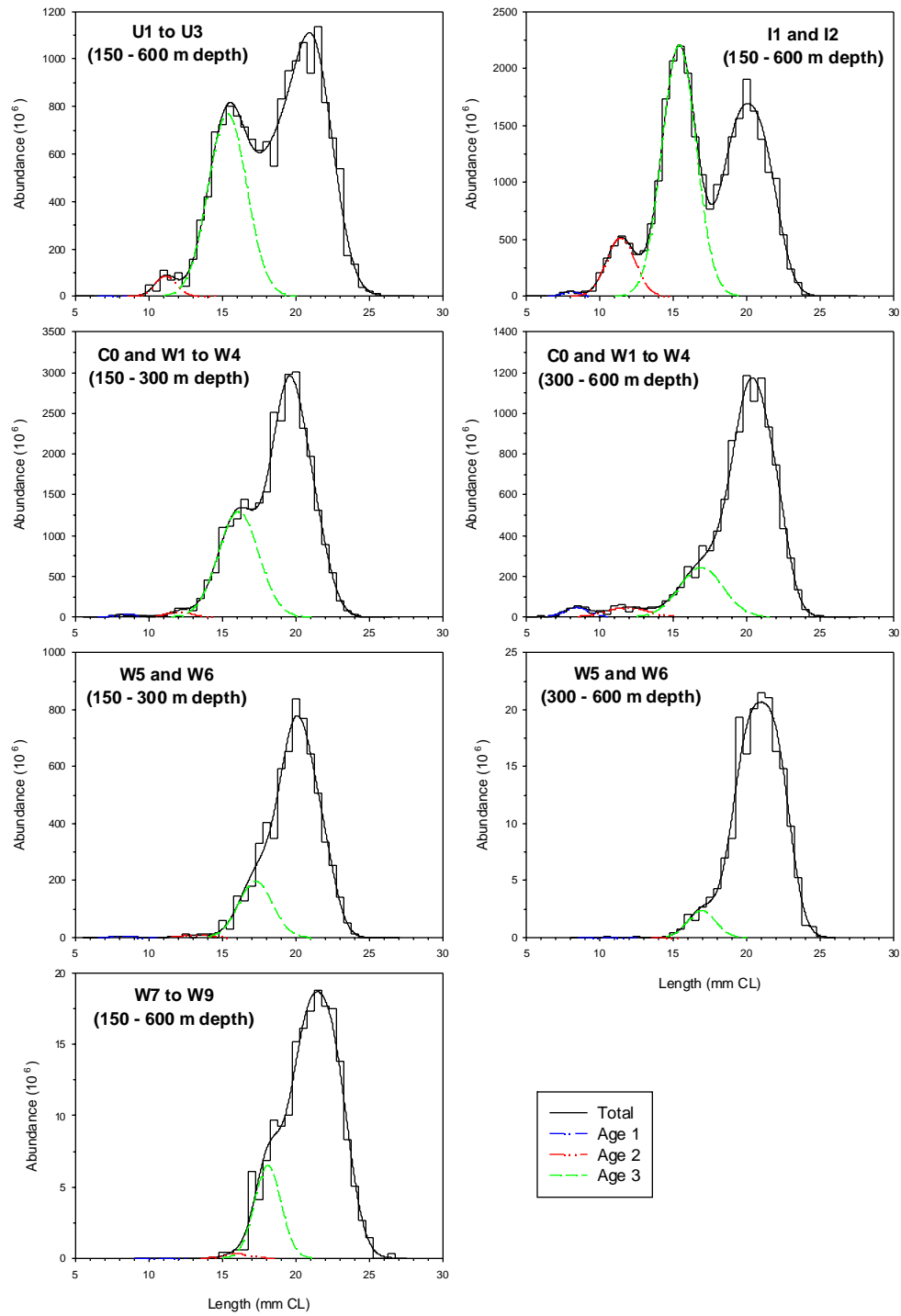
Fig. 10. Regional length frequencies of northern shrimp (juveniles and males) off West Greenland in 2005.
