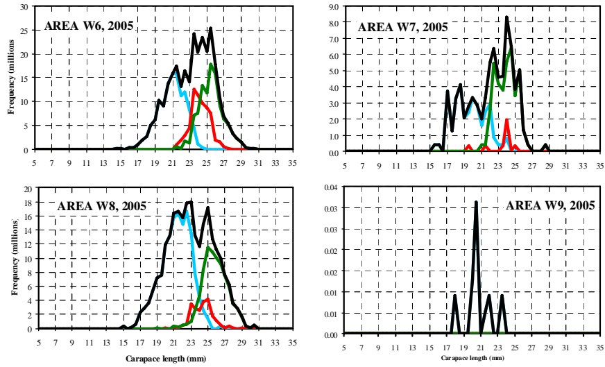
Fig. 6b. Length frequencies of northern shrimp in offshore areas W6 to W9 in 2005.
