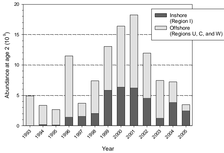
Fig. 11. Abundance indices for northern shrimp at age 2 off West Greenland, 1993-2005.
