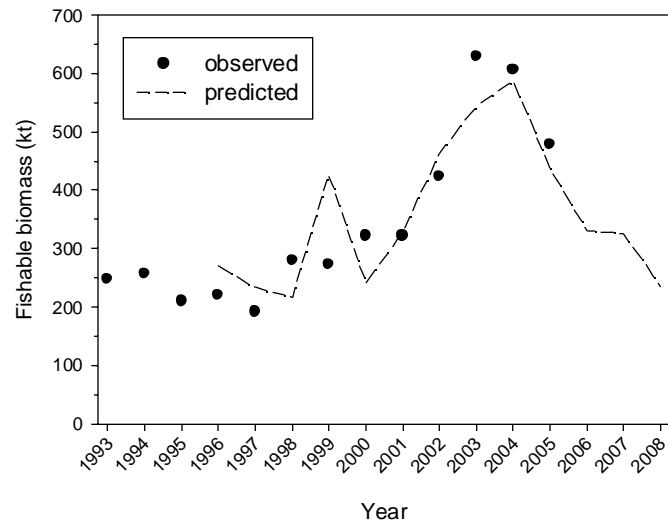
Fig. 13. Prediction of fishable biomass of northern shrimp off West Greenland from abundance at age 2 three years before.
