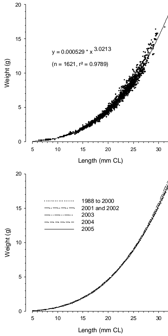
Fig. 9. Length-weight relationship of northern shrimp off West Greenland in 2005 and comparison with length-weight relationships used in previous years.
