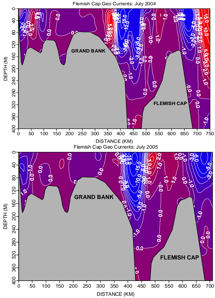
Fig. 9. The vertical distribution of the N-S geostrophic current field (in cm/s) along the Flemish Cap Section during the summer of 2004 (top panel) and 2005 (bottom panel) estimated from the density data. Negative currents (blue) are southward and positive currents (red) are northward.
