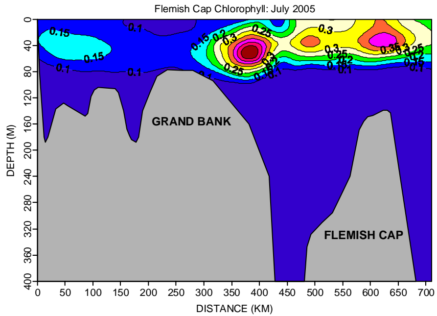
Fig. 8. The vertical distribution of chlorophyll concentrations (mg/l) along the 47°N section for the summer of 2005.
