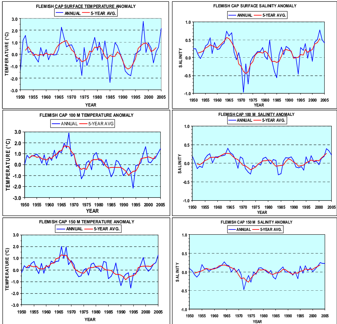
Fig. 6. Annual temperature and salinity anomalies at standard depths on the Flemish Cap in NAFO Division 3M. The solid line represents a 5-year running mean.
