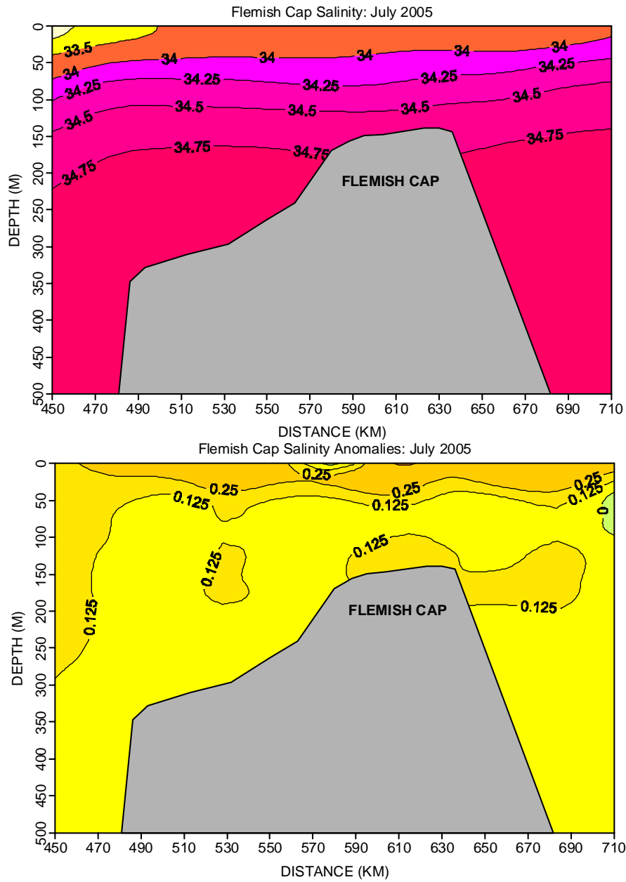
Fig. 4. The vertical distribution of salinity and salinity anomalies over the Flemish Cap (along 47^{\circ} N) for the summer of 2005.
