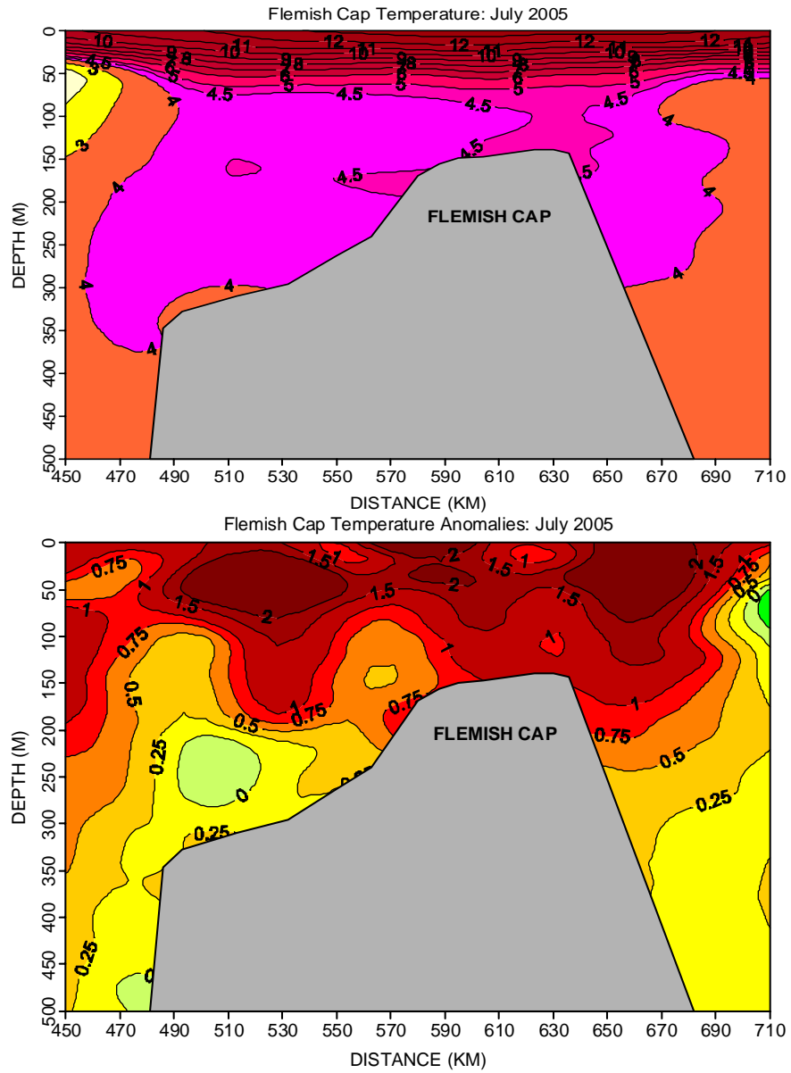
Fig. 3. The vertical distribution of temperature and temperature anomalies (in °C) over the Flemish Cap (along 47°N) for the summer of 2005.
