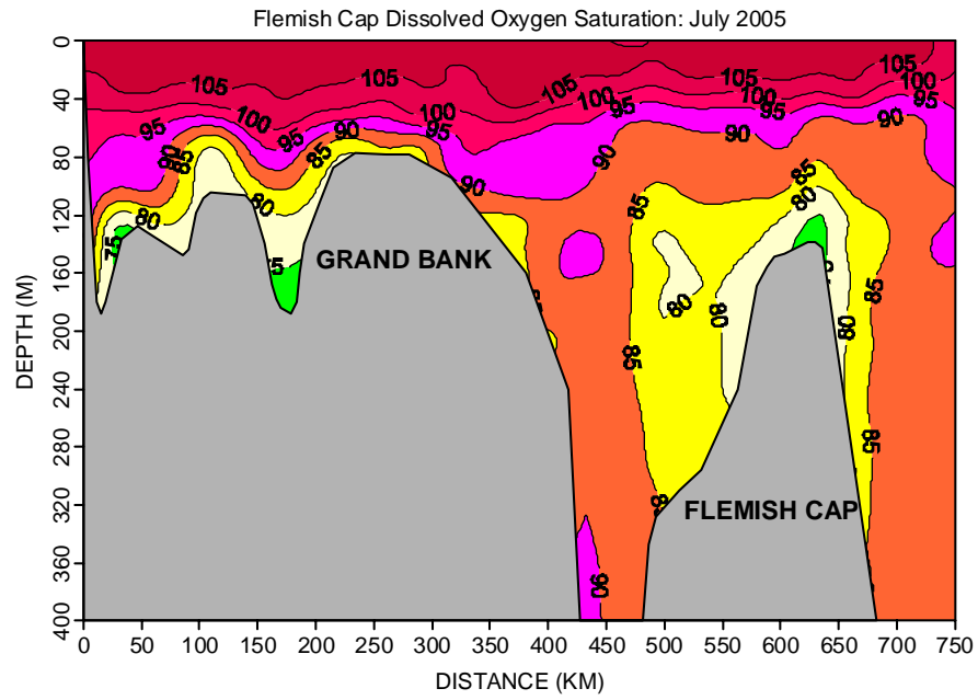
Fig. 7. The vertical distribution of dissolved oxygen percent saturation along 47°N for the summer of 2005.
