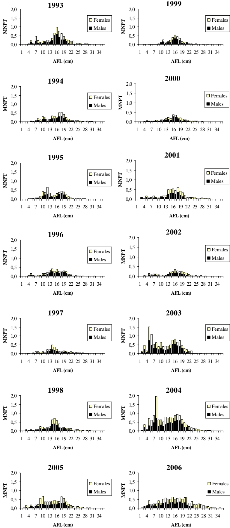
Figure 2.- Annual length distribution by sex in Flemish Cap 1993-2006.
