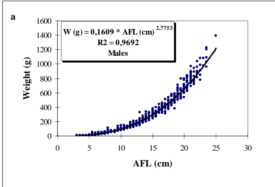
Figure 9.- Length weight relationship for (a) males and (b) females of roughhead grenadier in 2006.
