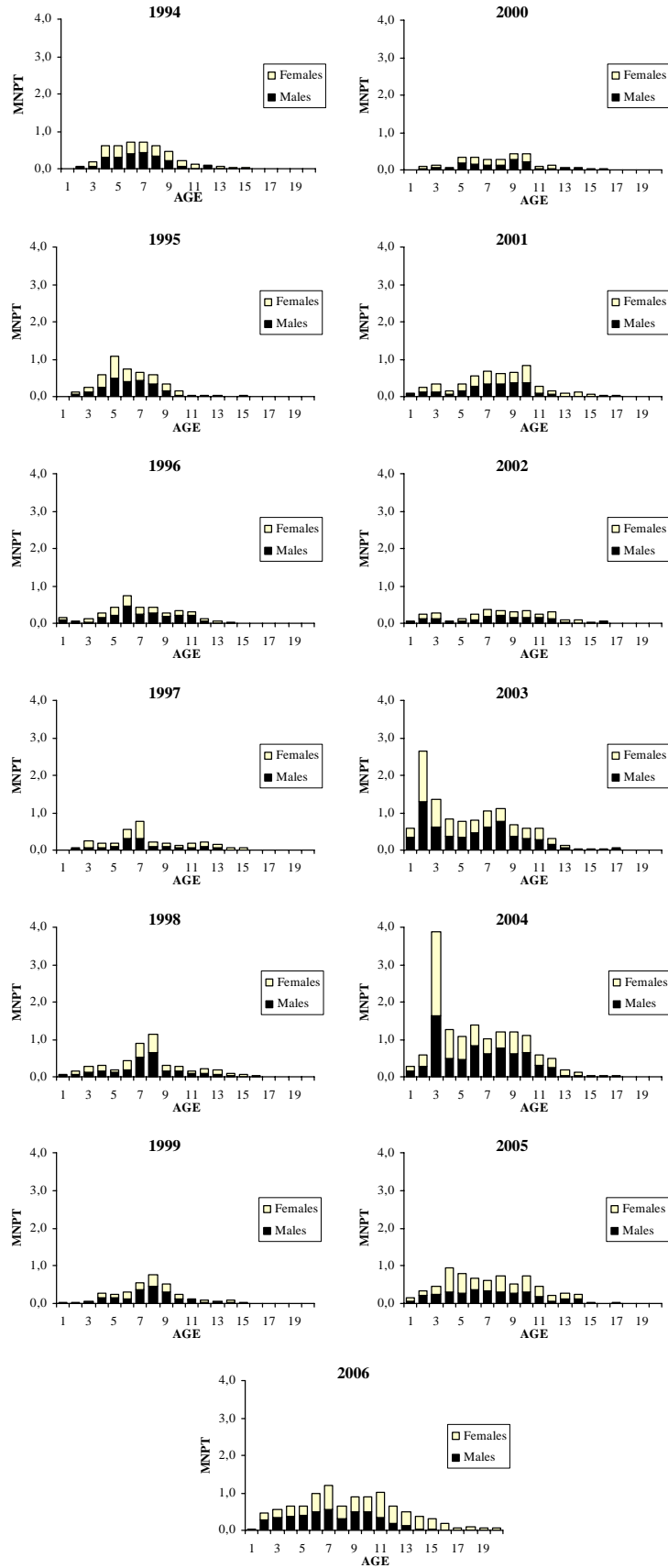
Figure 3.- Annual age composition by sex in Flemish Cap 1994-2006.
