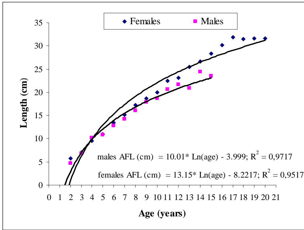
Figure 7.- Logarithmic growth curve by sexes in Flemish Cap 2006.
