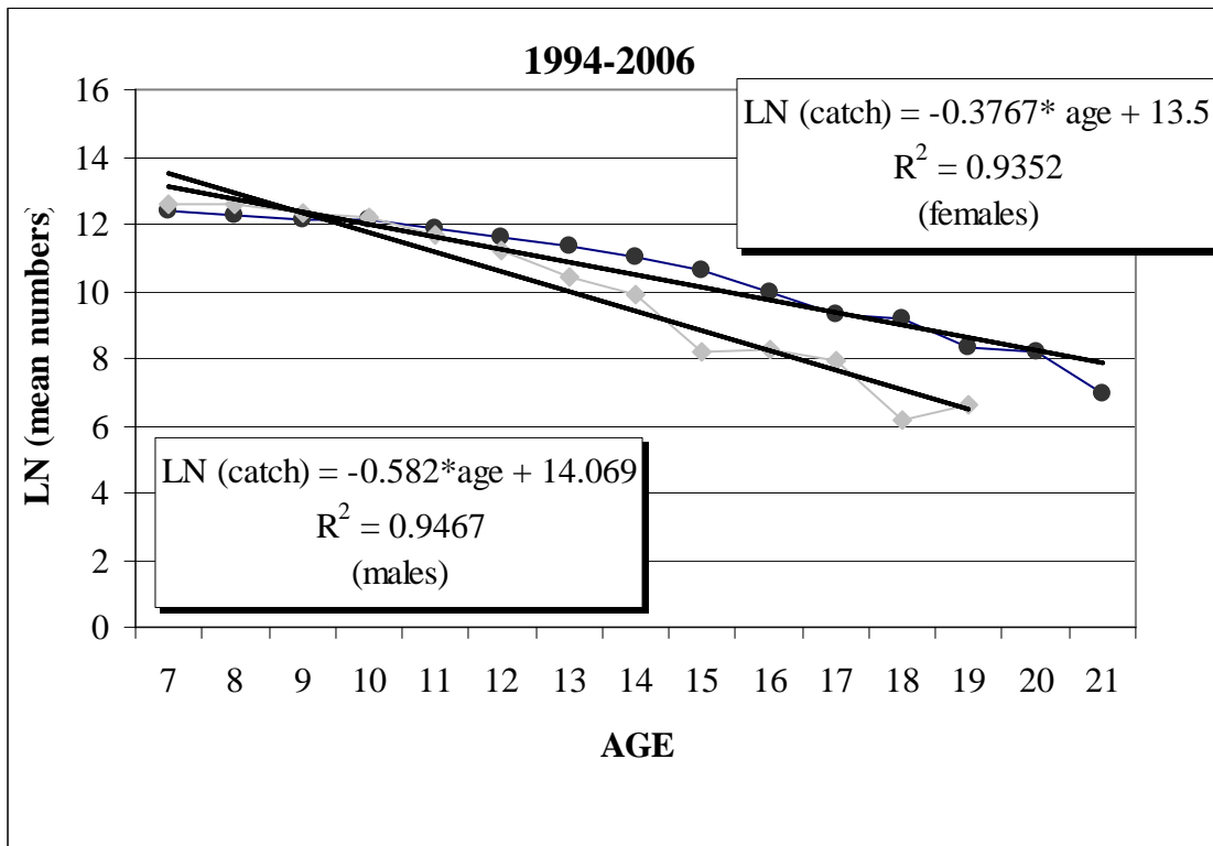
Figure 8.- Catch curves by sex for roughhead grenadier in Flemish Cap 1994-2006.
