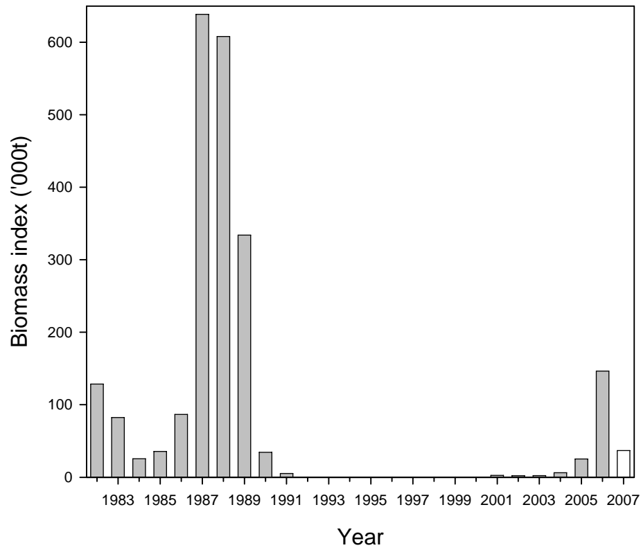
Fig. 4. Survey indices of Atlantic cod biomass for West Greenland offshore waters, 1982-2007 (1982-2006: original estimates from the German groundfish survey; 2007: estimate based on the Greenland Bottom Trawl Survey).
