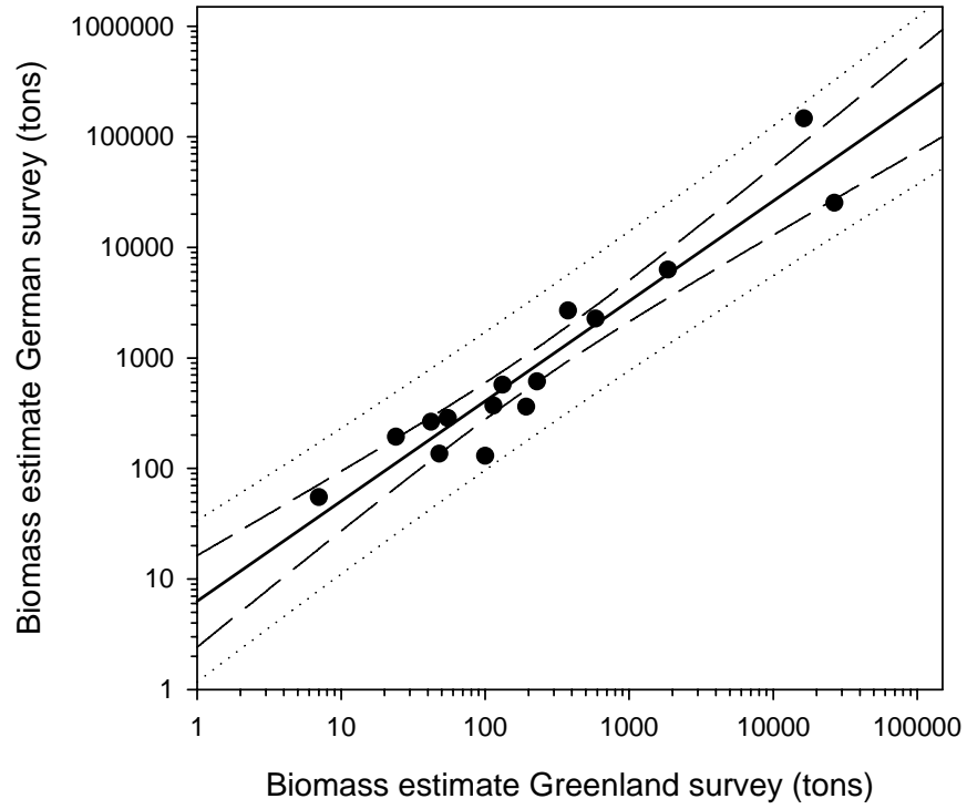
Fig. 2. Relationship between estimates of cod biomass in the overlapping area of the German groundfish survey and the Greenland Bottom Trawl Survey, 1992-2006. Dashed and dotted lines indicate limits of the 95% confidence and prediction intervals, respectively.
