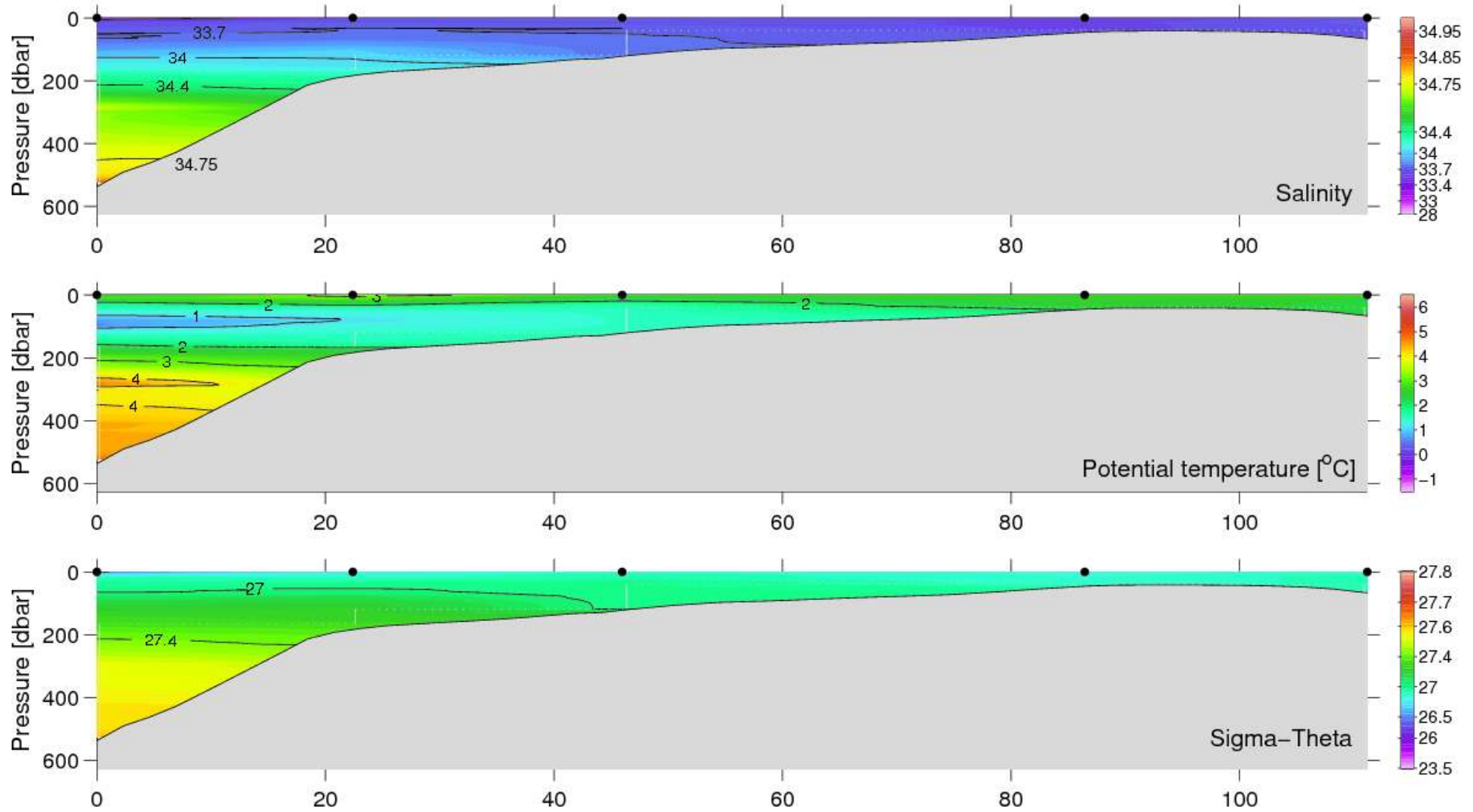
Figure 30. Vertical distribution of temperature, salinity and density at the Sisimiut (Holsteinsborg) section, July 4–5, 2007.
