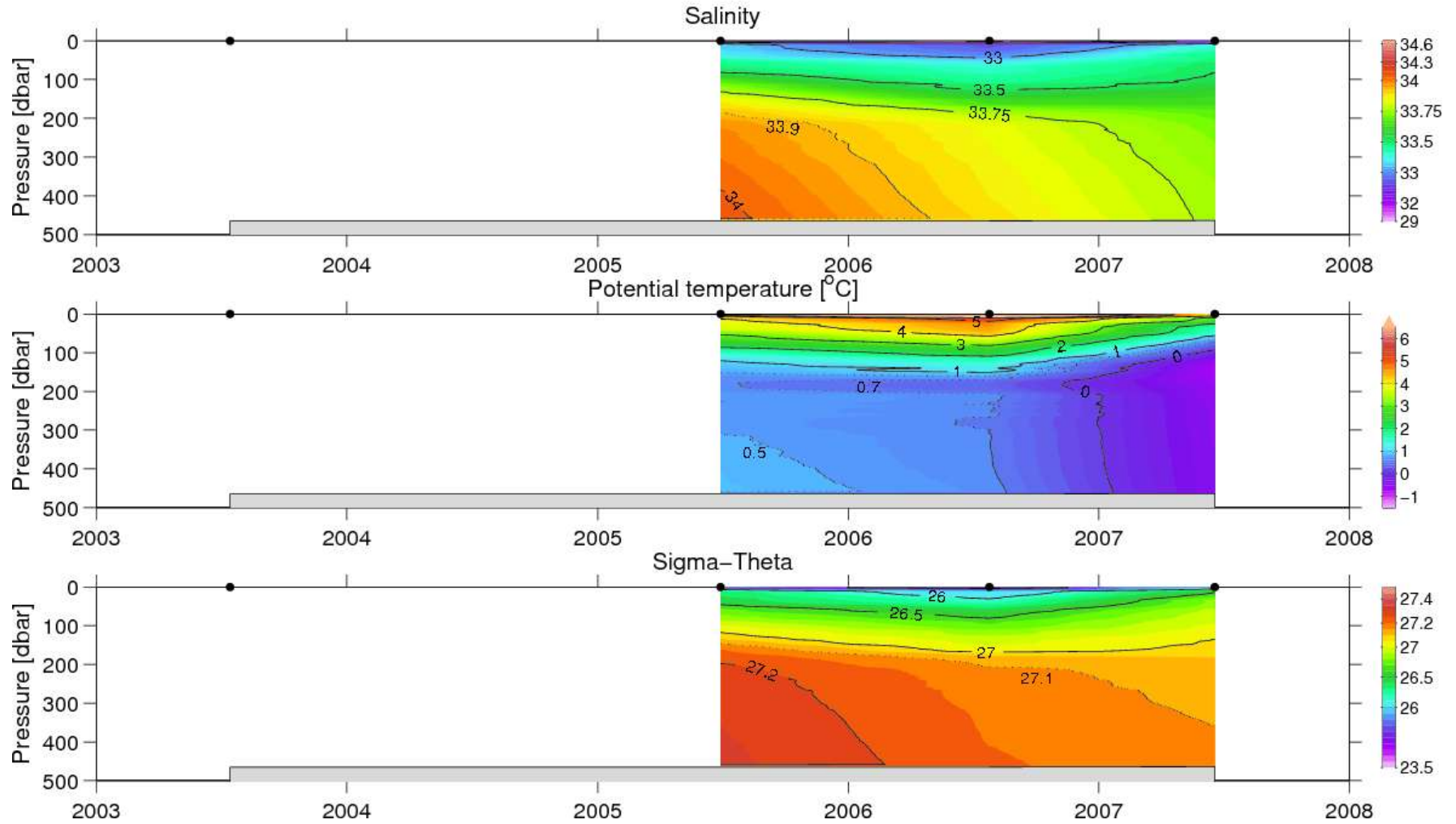
Figure 46. Hovmöller diagram of vertical distribution of temperature, salinity and density at the Itivdleq fjord st.4, late June/July 2005–2007.
