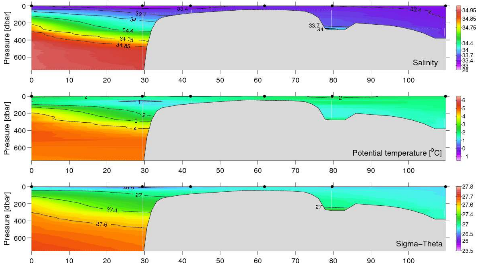
Figure 27. Vertical distribution of temperature, salinity and density at the Fylla Bank section, June 12–13, 2007. The section is extended by Godthaab (Nuuk) fjord st. 3 (“hovedstationen”) on right side of the plot.
