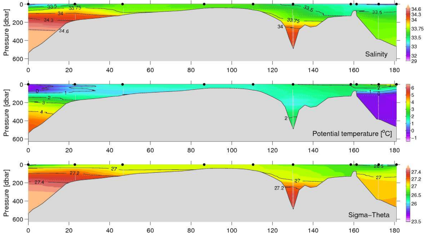
Figure 42. Vertical distribution of temperature, salinity and density at the Itivdleq fjord, June 21, 2007. Sisimiut section left (identical to Figure 27).
