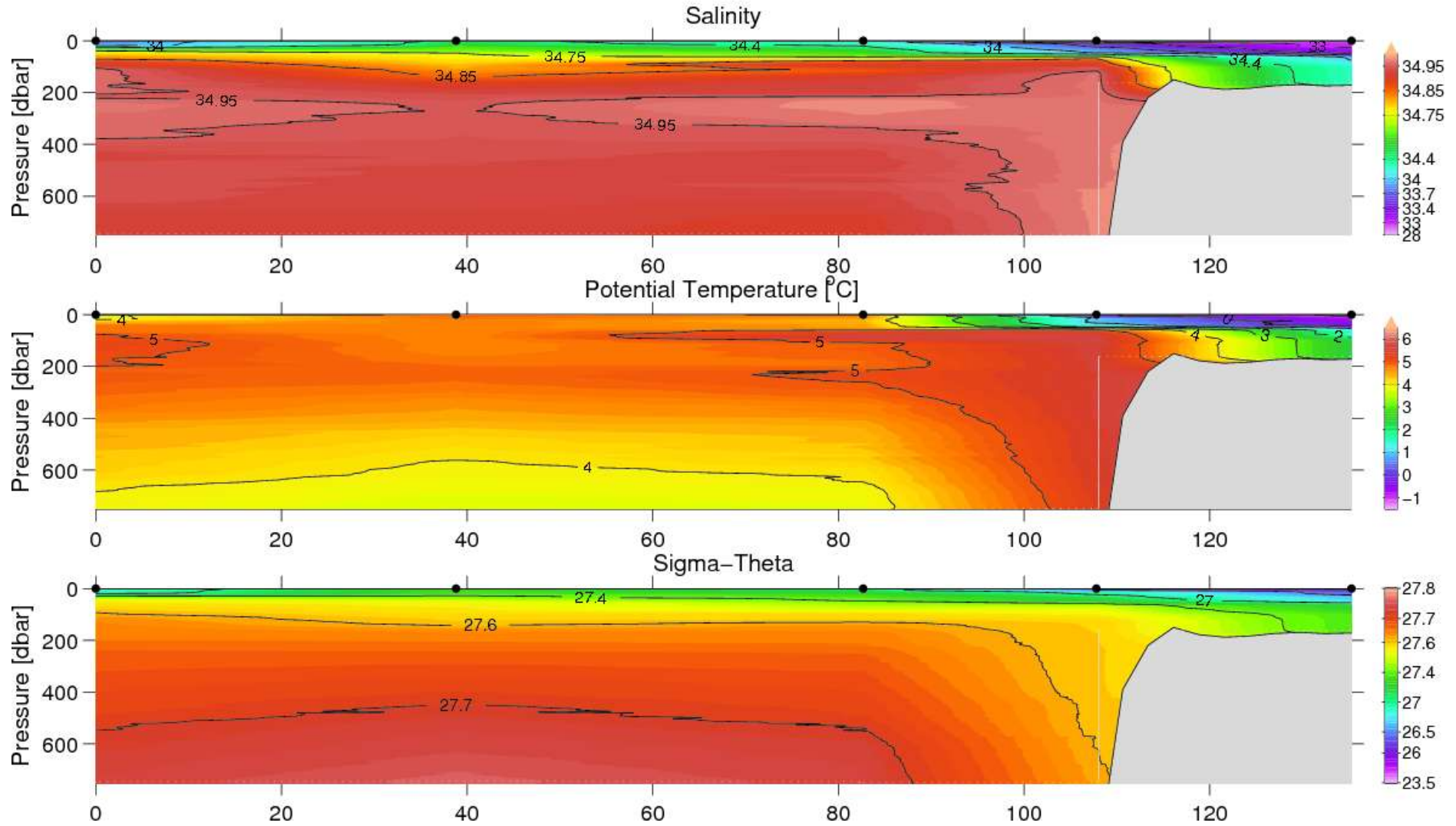
Figure 24. Vertical distribution of temperature, salinity and density at the Cape Farewell section, June 9–10, 2007.
