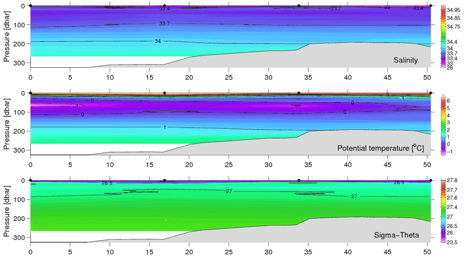
Figure 34. Vertical distribution of temperature, salinity and density at the Upernavik section, July 22–23, 2007.
