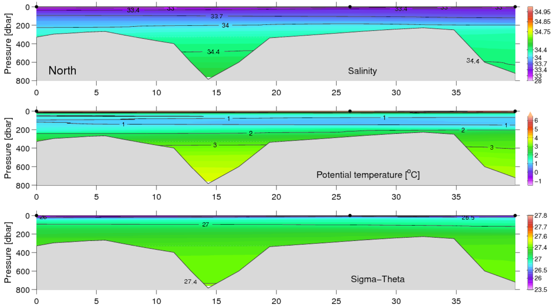
Figure 35. Vertical distribution of temperature, salinity and density at the Aasiaat–Qeqertarsuaq (Egedesminde–Godhavn) section, July 13–14, 2007.
