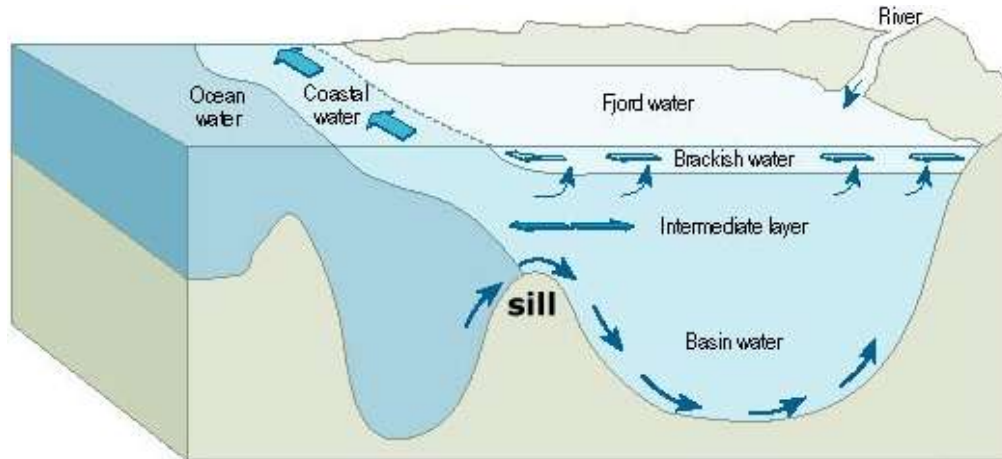
Figure 19. Sketch of the circulation in a fjord (modified from http://www.amap.no/maps-gra/show.cfm?figureId=58 ).
