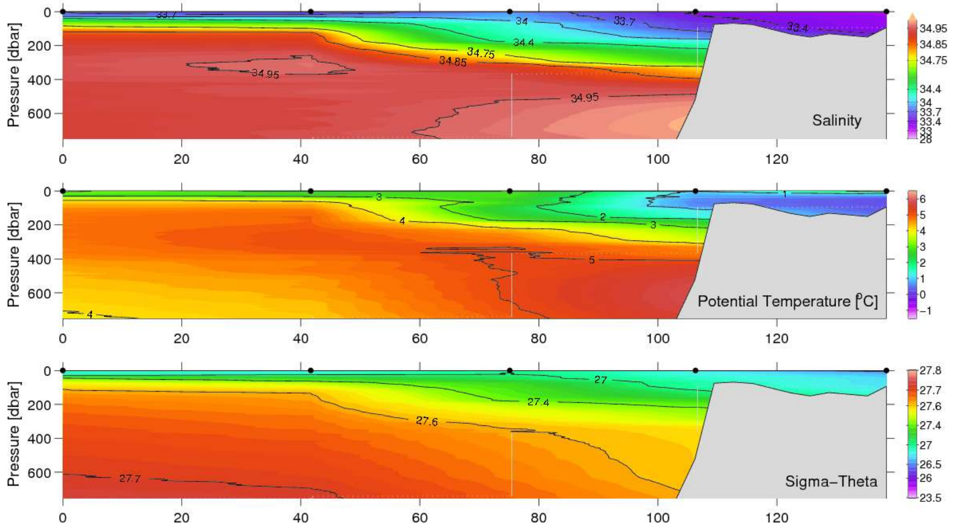
Figure 26. Vertical distribution of temperature, salinity and density at the Paamiut (Frederikshaab) section, June 12, 2007.
