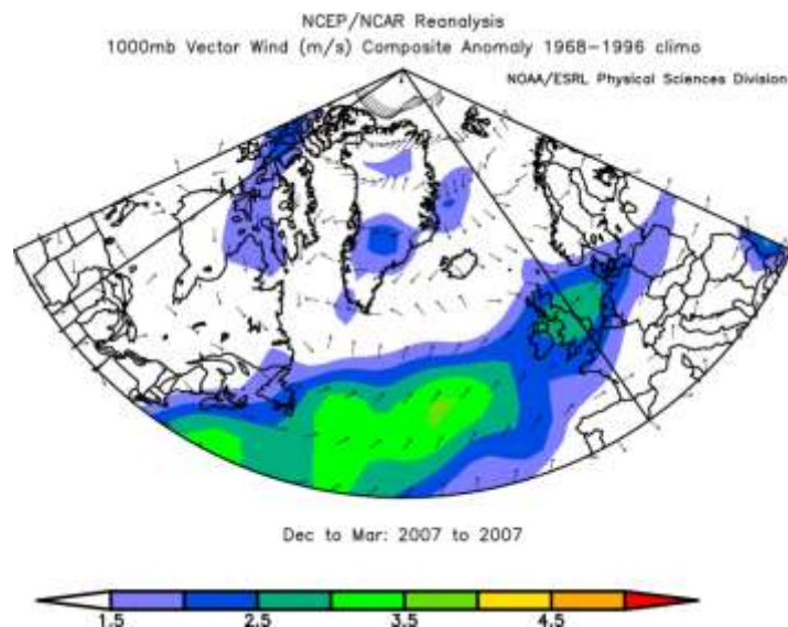
Figure 12. Winter (DJFM) wind anomaly for 2006/2007 in the North Atlantic region. NCEP/NCAR re-analysis (from http://www.cdc.noaa.gov ).
