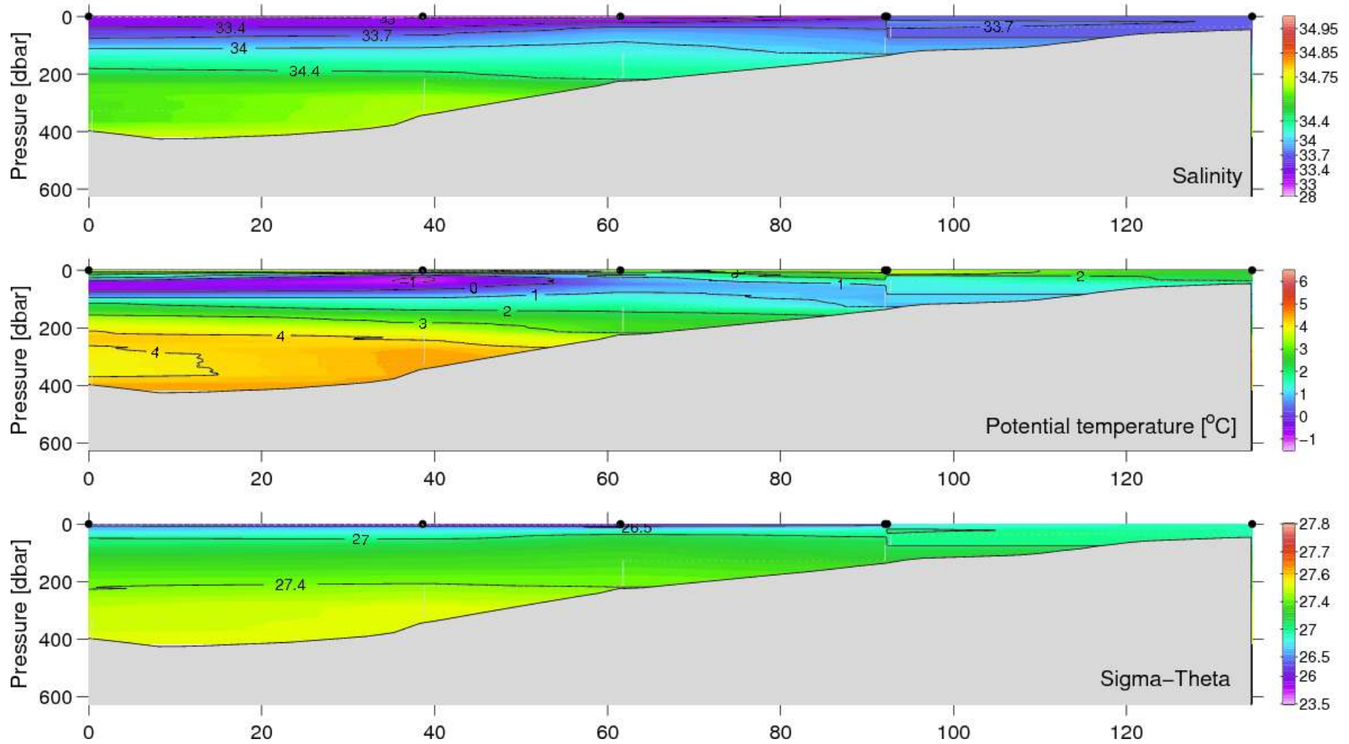
Figure 31. Vertical distribution of temperature, salinity and density at the Aasiaat (Egedesminde) section, July 7–8, 2007.
