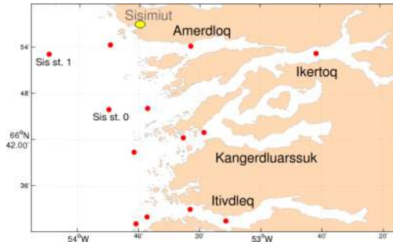
Figure 4. Position of the oceanographic stations around Sisimiut where measurements were performed in 2007. See Figure 1 for position of all sections measured in 2007.
