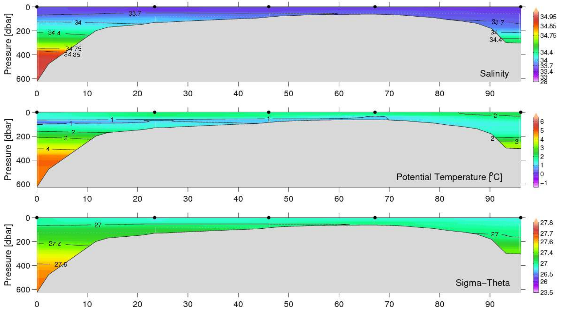
Figure 28. Vertical distribution of temperature, salinity and density at the Maniitsoq (Sukkertoppen) section, June 17–18, 2007.
