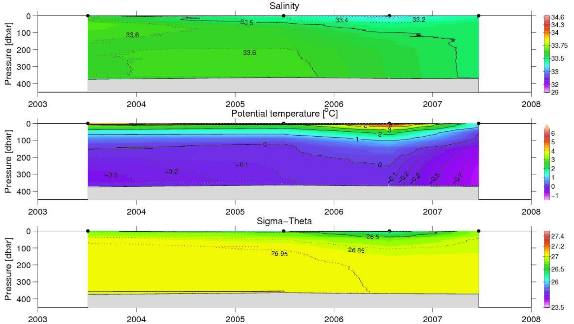
Figure 45. Hovmöller diagram of vertical distribution of temperature, salinity and density at the Kangerdluarssuk fjord st.3, late June/July 2003, 2005–2007.
