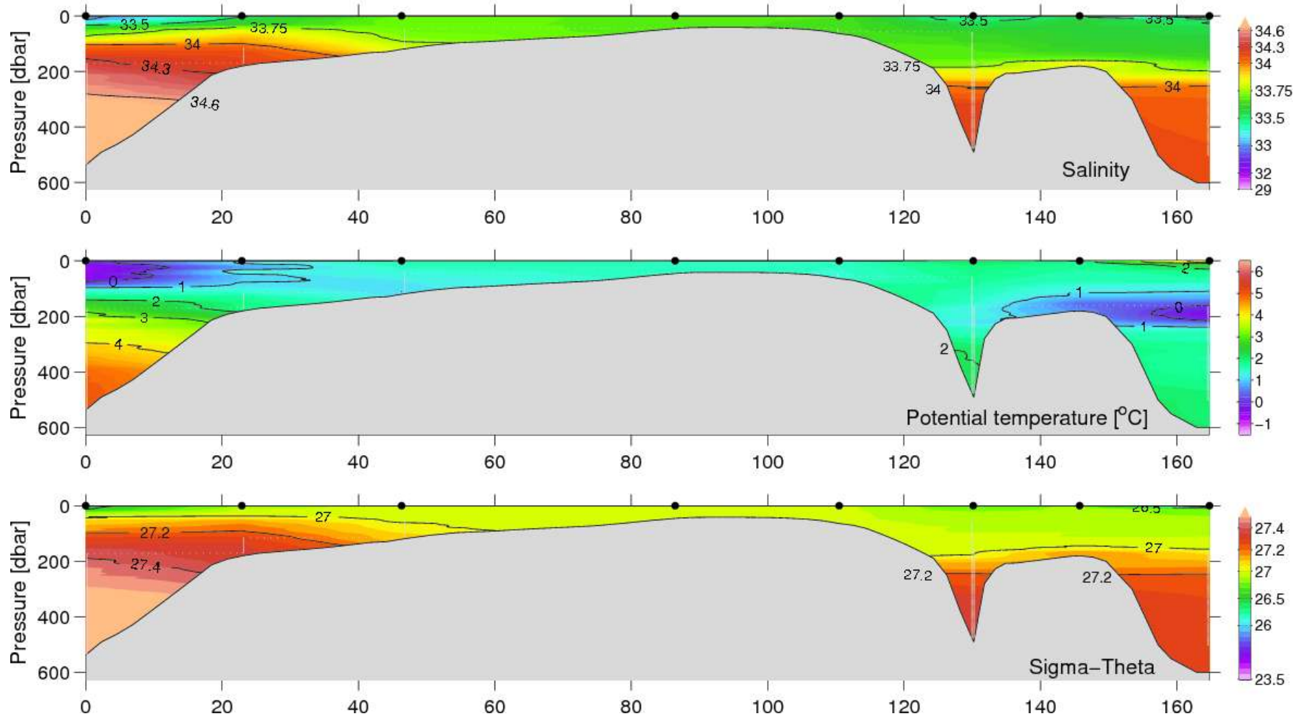
Figure 39. Vertical distribution of temperature, salinity and density at the Amerdloq fjord, June 19–20, 2007. Sisimiut section left (identical to Figure 27).
