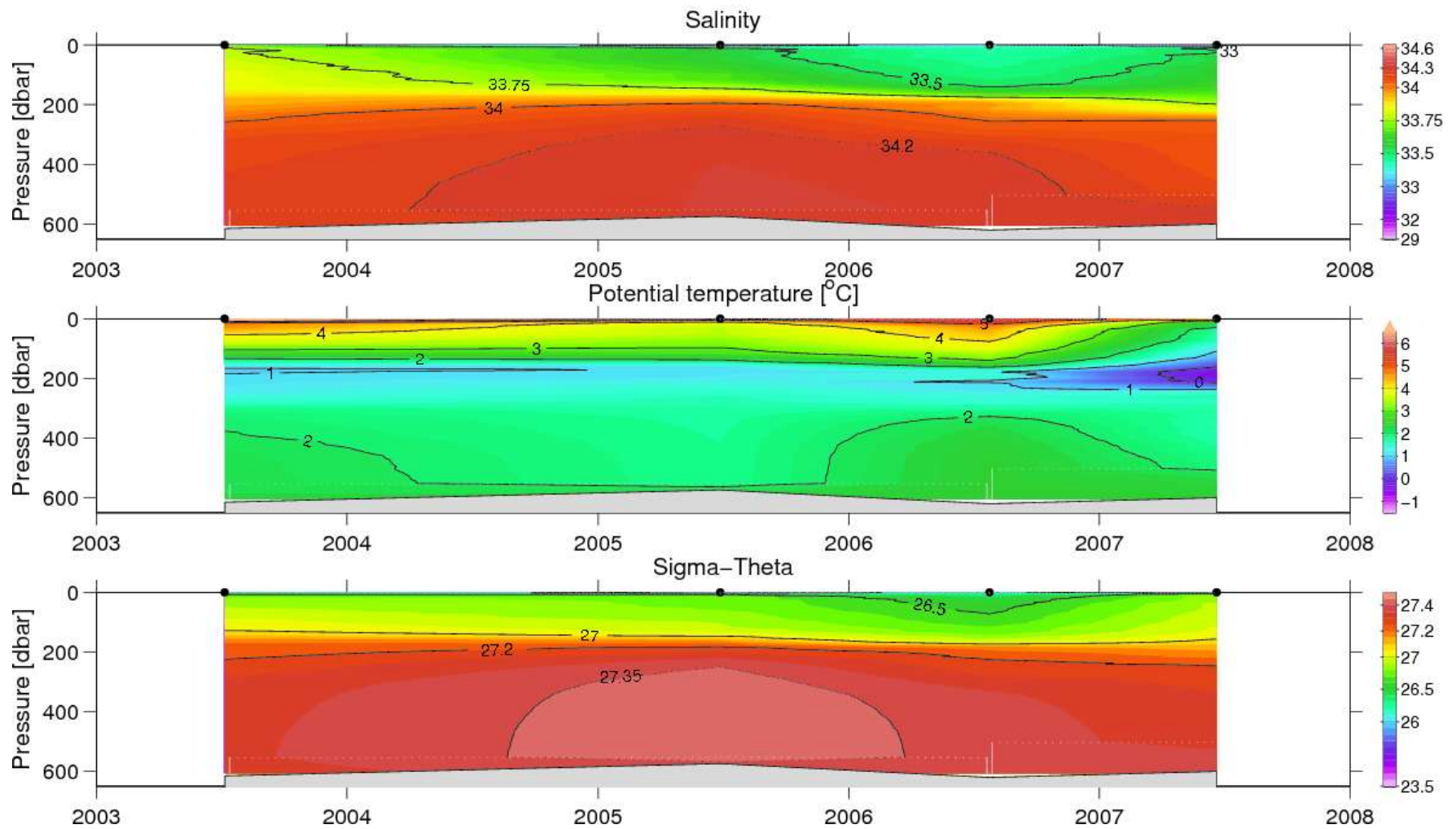
Figure 43. Hovmöller diagram of vertical distribution of temperature, salinity and density at the Amerdloq fjord st.4, late June/July 2003, 2005–2007.
