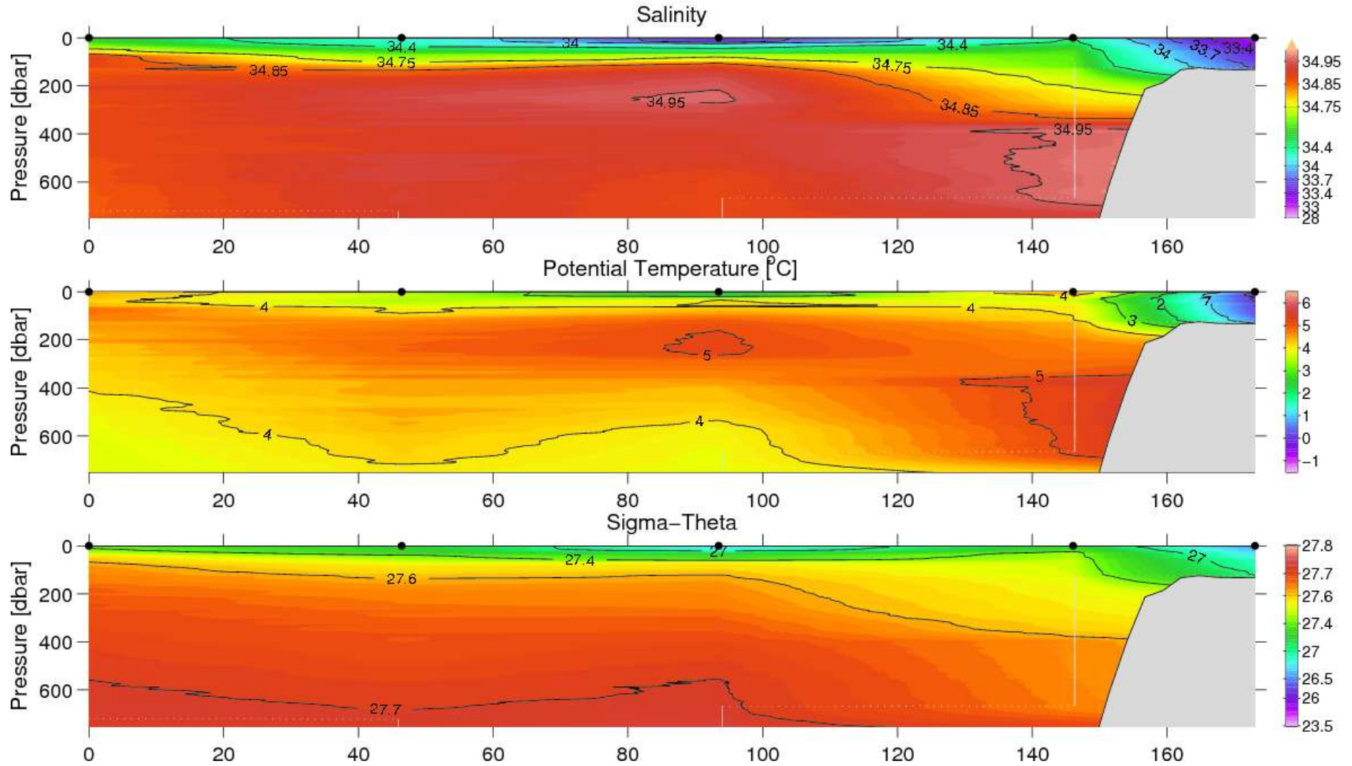
Figure 25. Vertical distribution of temperature, salinity and density at the Cape Desolation section, June 10–11, 2007.
