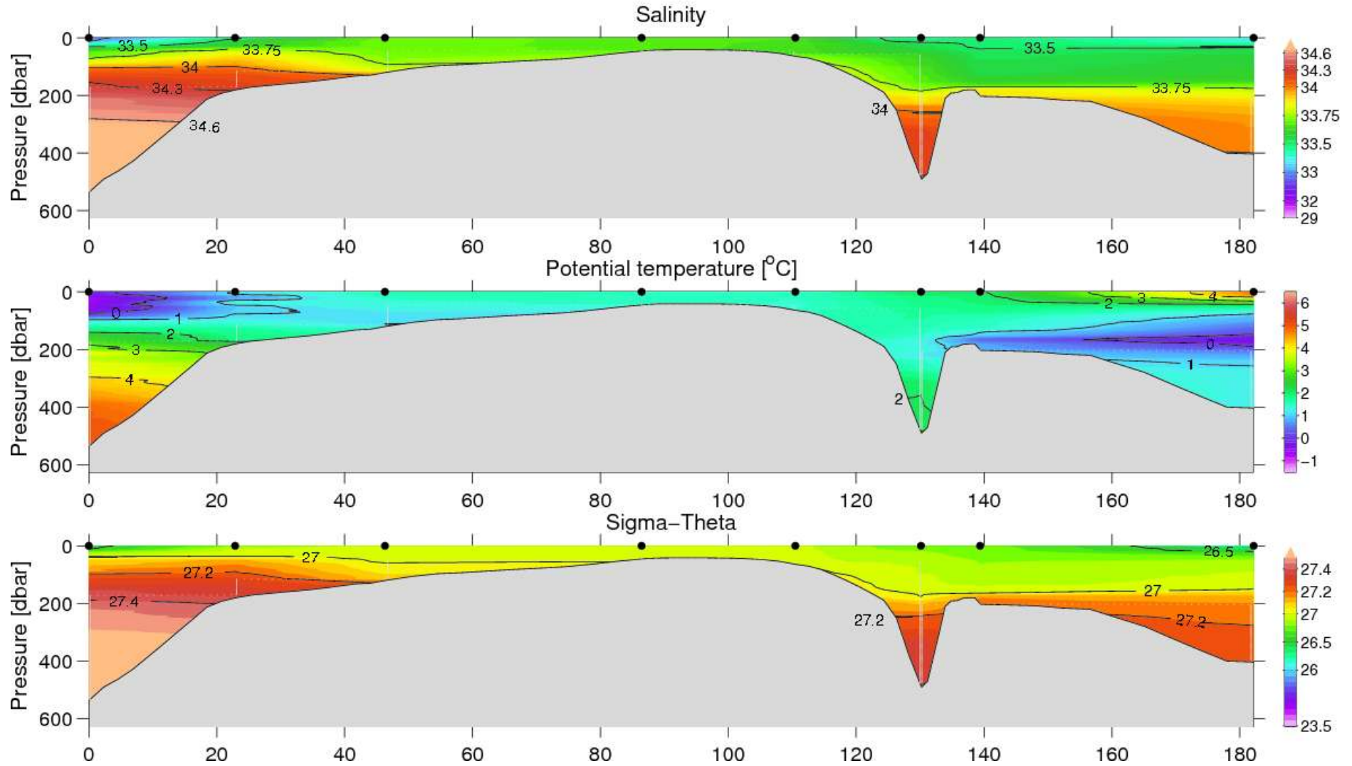
Figure 40. Vertical distribution of temperature, salinity and density at the Ikertoq fjord, June 20, 2007. Sisimiut section left (identical to Figure 27).
