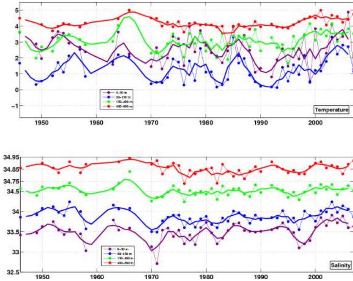
Figure 20. Timeseries of mean temperature (top) and mean salinity (bottom) for the period 1946–2007 in four different depth intervals west of “Sukkertop Banke” (Maniitsoq, st.5) over the continental slope. The thick curves are the 3 year running mean values. Note the change in scales at 34.75 for salinity. Statistics is shown in Table 3.
