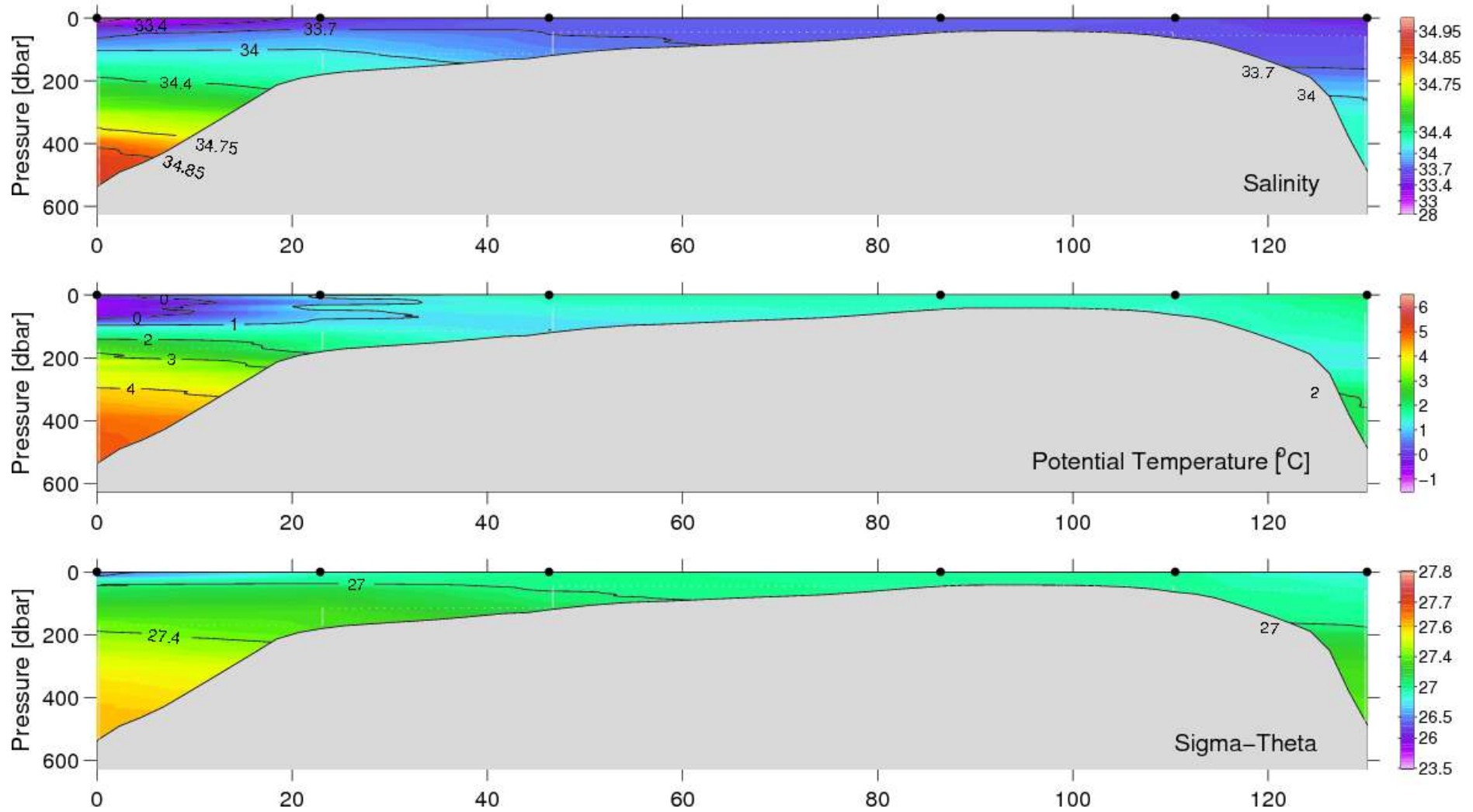
Figure 29. Vertical distribution of temperature, salinity and density at the Sisimiut (Holsteinsborg) section, June 19–20, 2007. Sisimiut st. 0 right.
