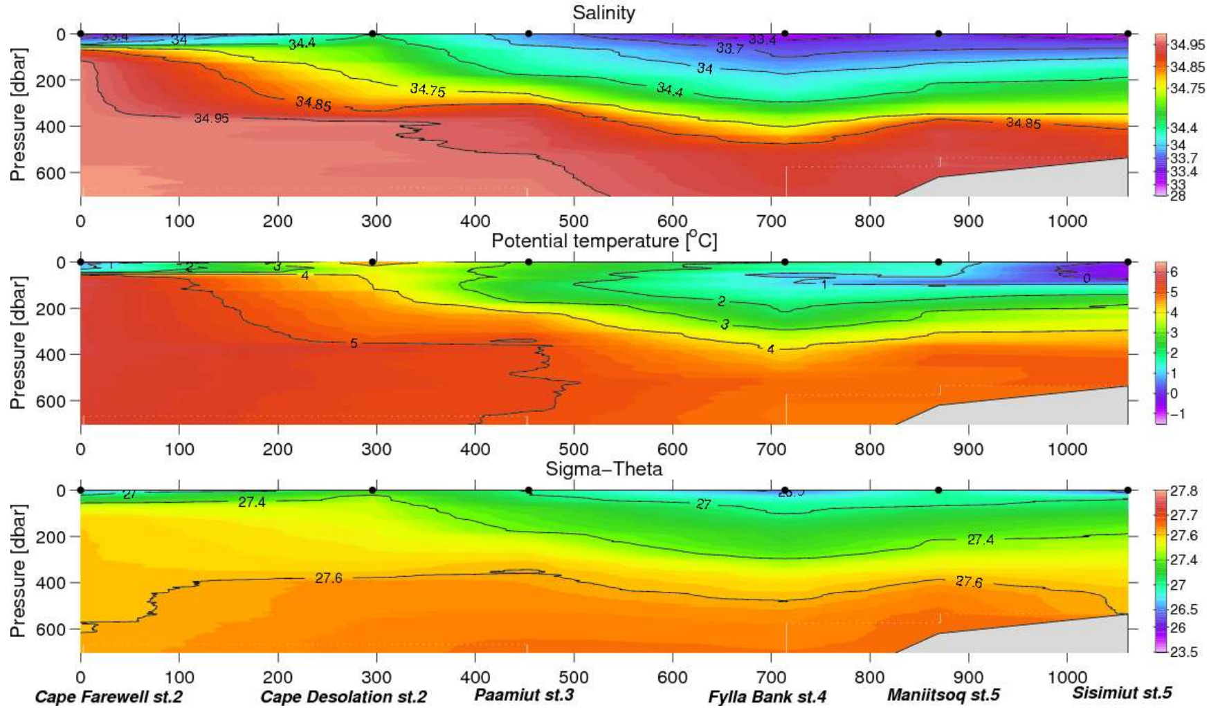
Figure 22. Vertical distribution of temperature, salinity and density over the continental shelf break from Cape Farewell to Sisimiut, June 9–20, 2007.
