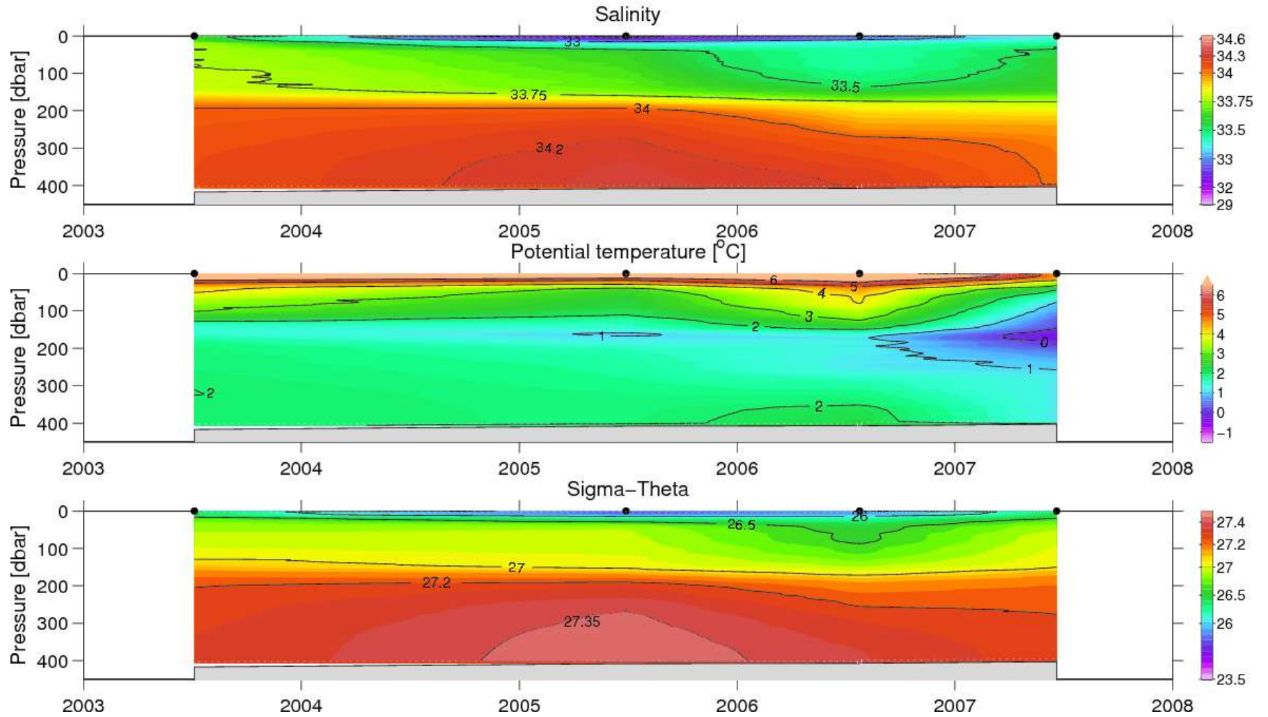
Figure 44. Hovmöller diagram of vertical distribution of temperature, salinity and density at the Ikertoq fjord st.4, late June/July 2003, 2005–2007.
