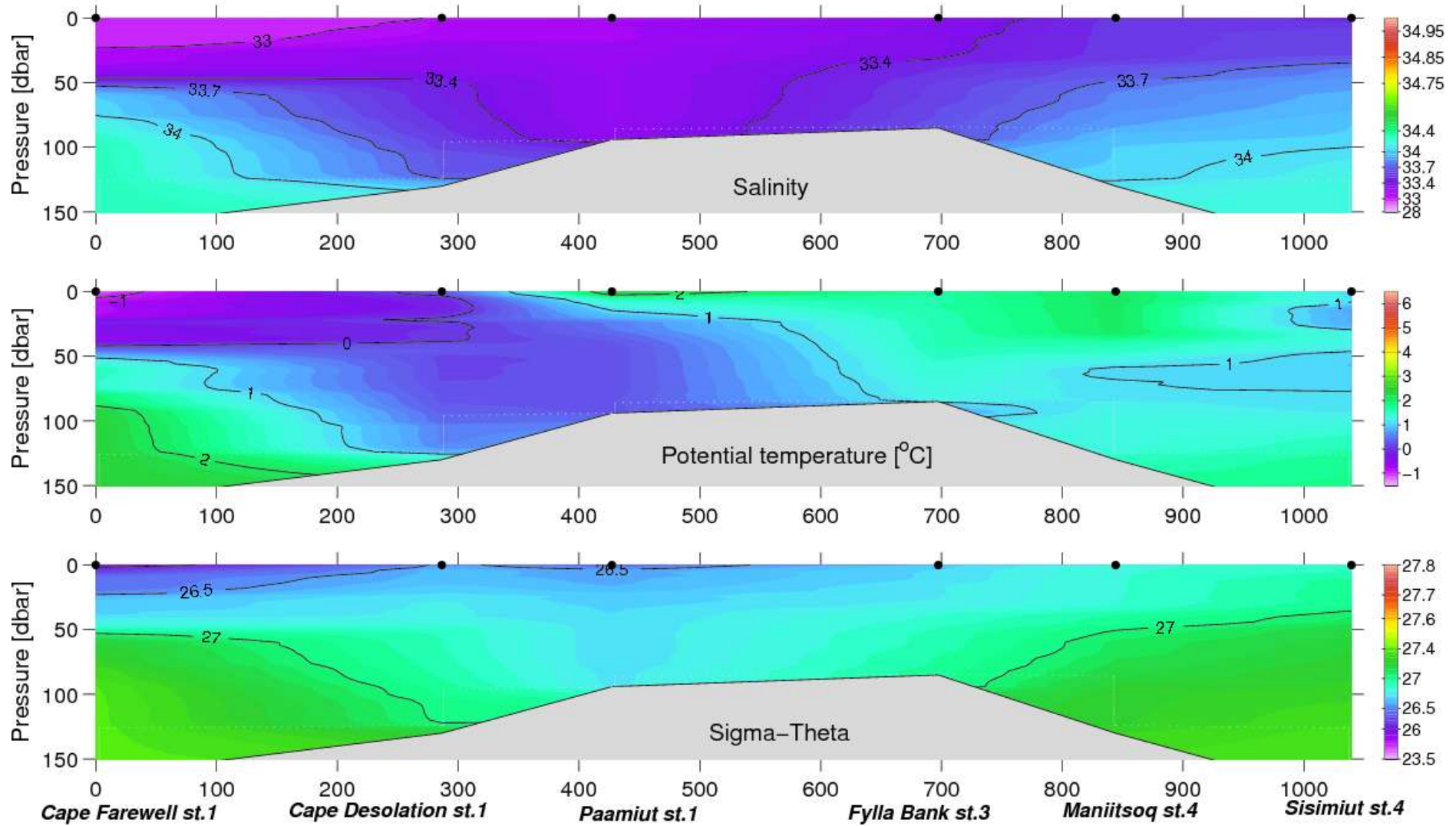
Figure 23. Vertical distribution of temperature, salinity and density over the shelf banks from Cape Farewell to Sisimiut, July 10–19, 2007.
