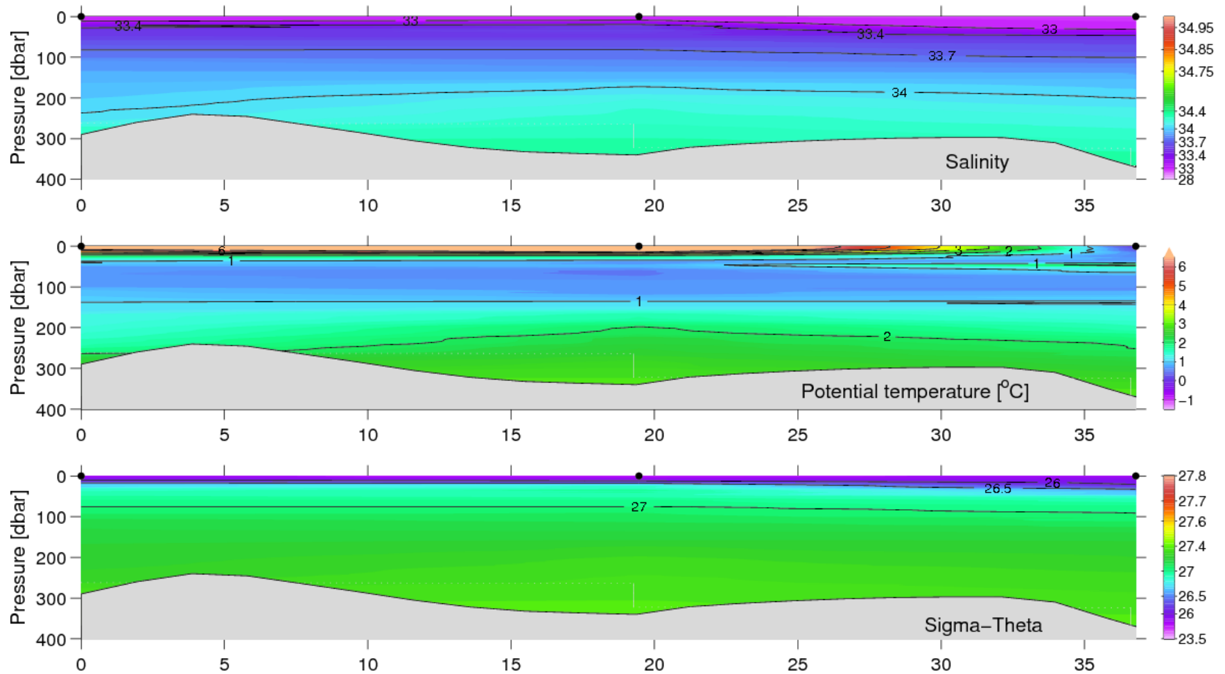
Figure 37. Vertical distribution of temperature, salinity and density at the Skansen–Ilulissat (Skansen–Jakobshavn) section, July 15, 2007.
