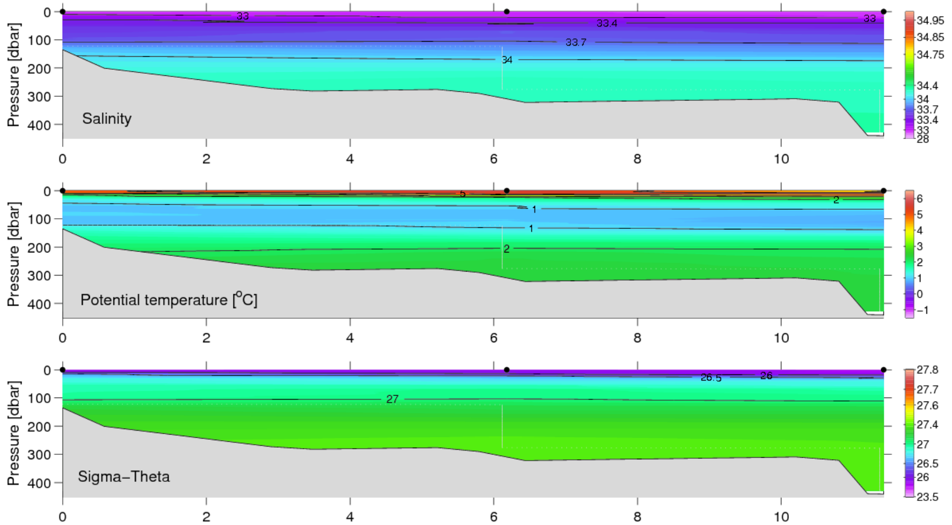
Figure 38. Vertical distribution of temperature, salinity and density at the Appat (Arveprins Ejlande) section, July 18, 2007.
