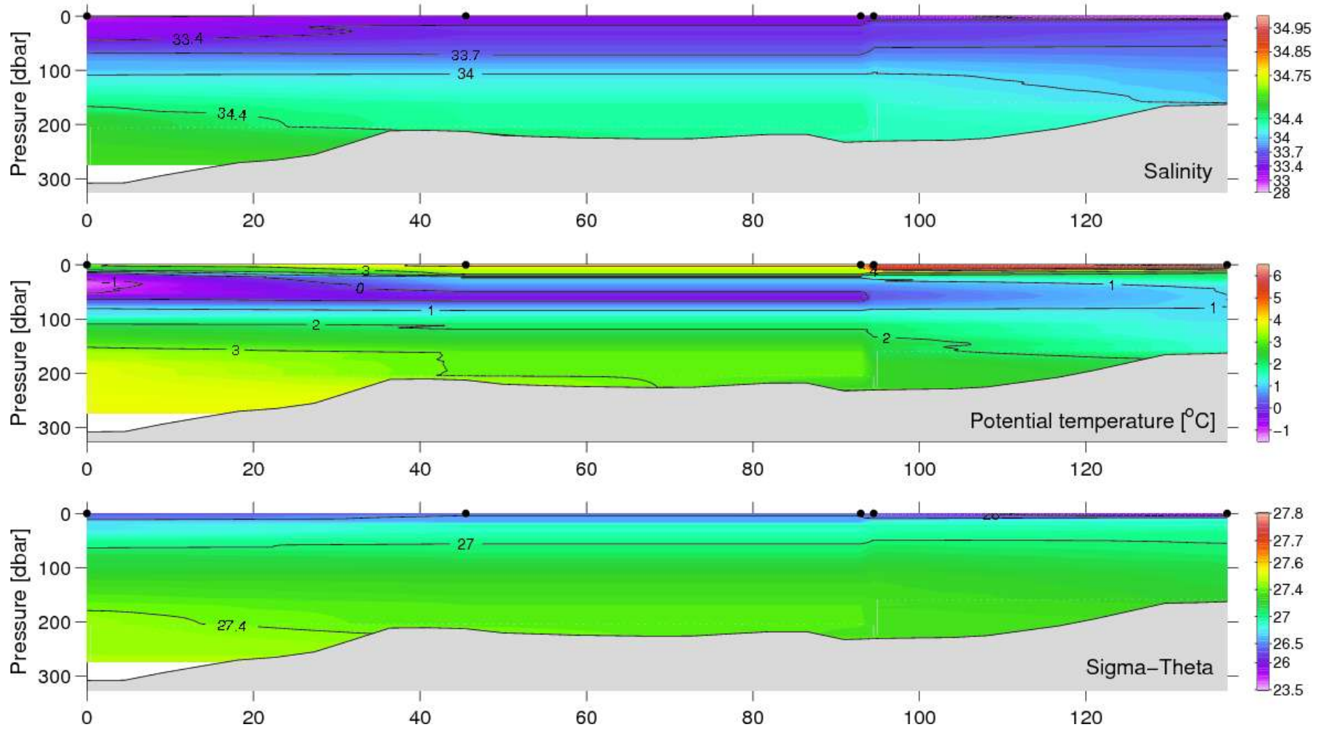
Figure 32. Vertical distribution of temperature, salinity and density at the Kangerluk (Disko Fjord) section, July 10–11, 2007.
