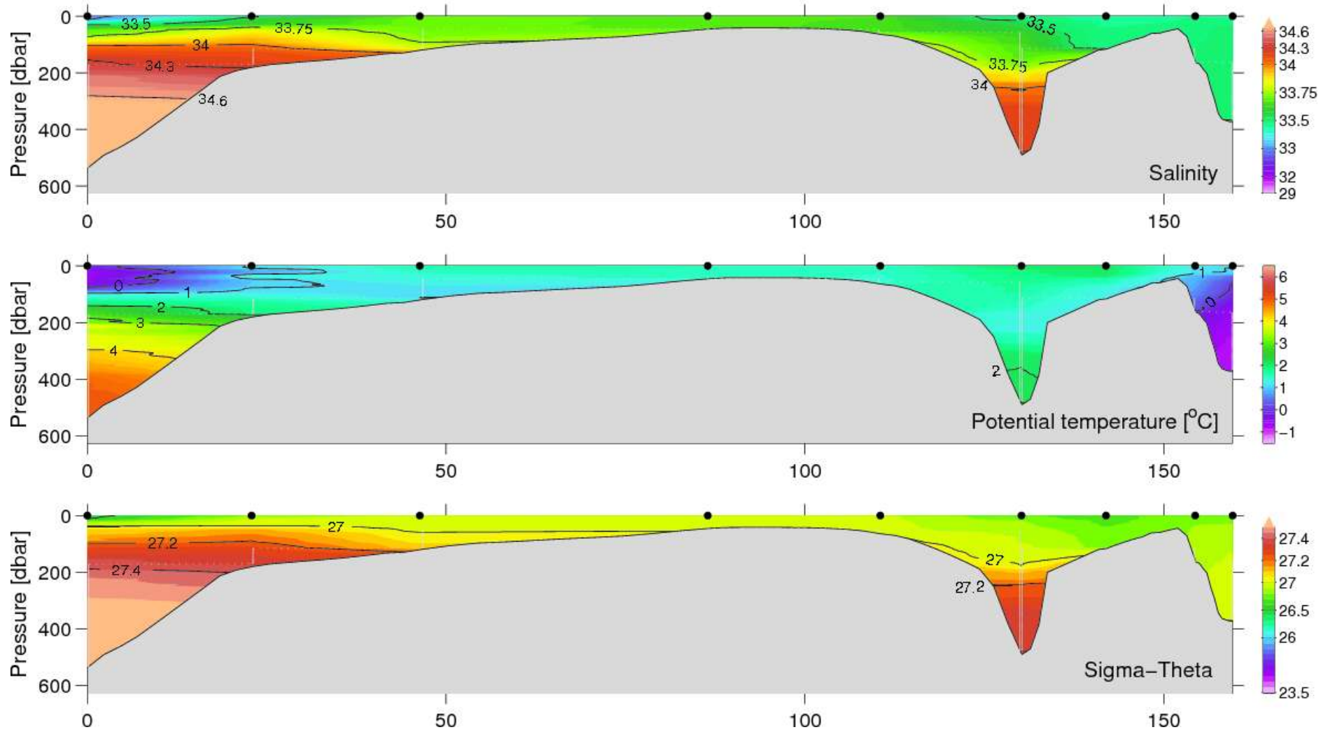
Figure 41. Vertical distribution of temperature, salinity and density at the Kangerdluarssuk fjord, June 20, 2007. Sisimiut section left (identical to
