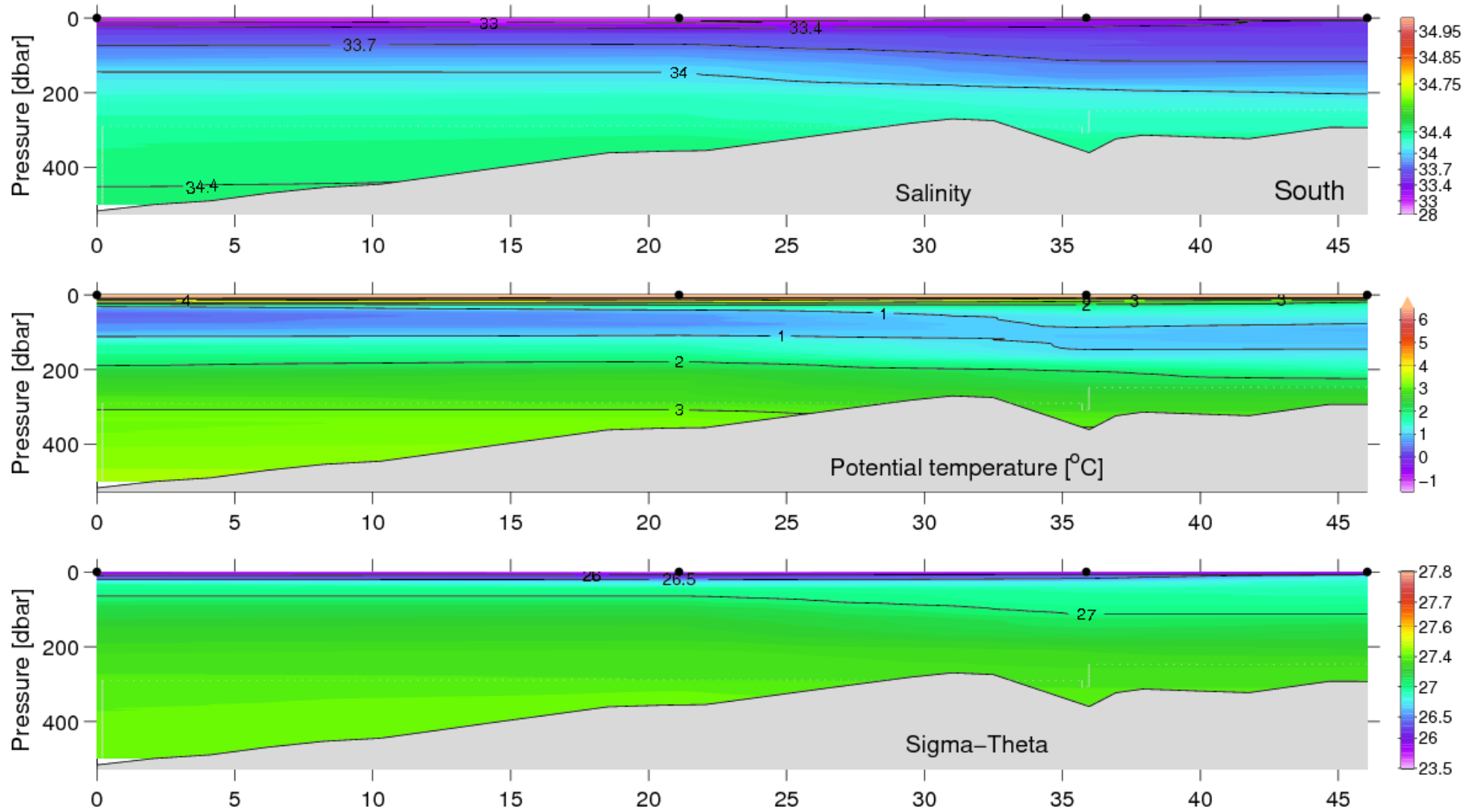
Figure 36. Vertical distribution of temperature, salinity and density at the Skansen–Akunaq section, July 14, 2007.
