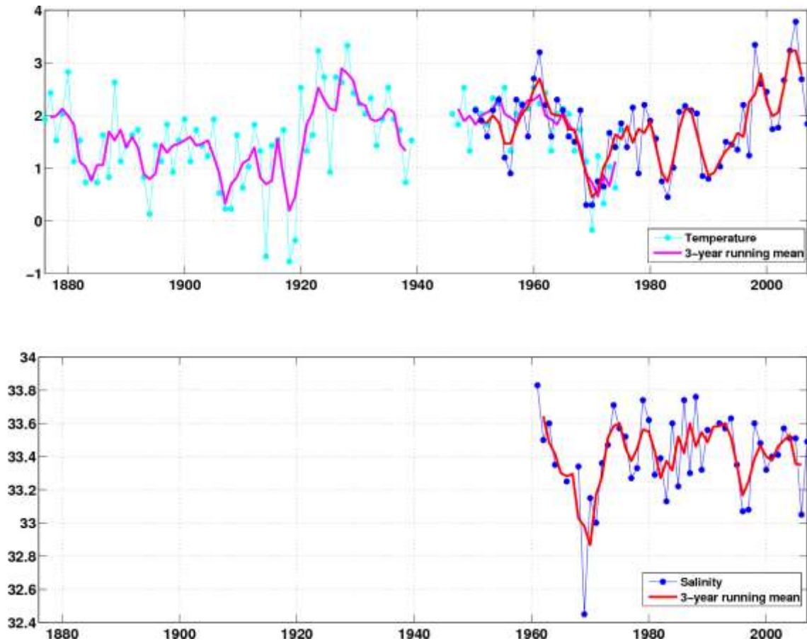
Figure 15. Timeseries of mean temperature (top) and mean salinity (bottom) on top of Fylla Bank (0–40 m) in the middle of June for the period 1950–2007. The red curve is the 3 year running mean value. Statistics is shown in Table 1. The timeseries for temperature (top, magenta/purple) is extended back to 1875 using Smed-data for area A1 (see chapter 4.1. for details).
