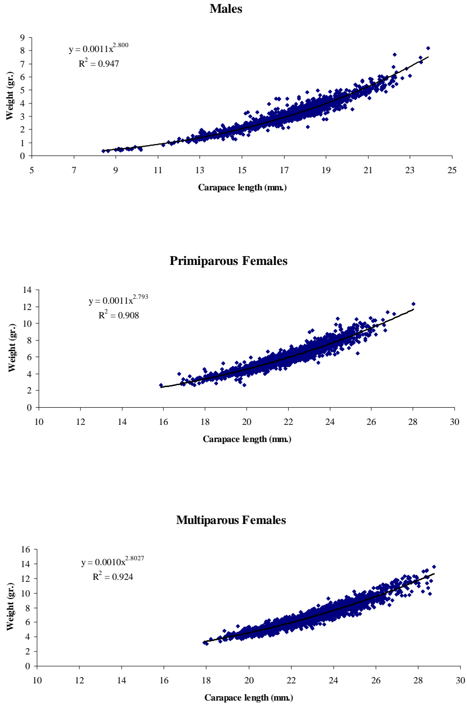
Figure 8. Shrimp length-weight relationships by sex and maturity stages in 2008 on EU Flemish Cap survey.
