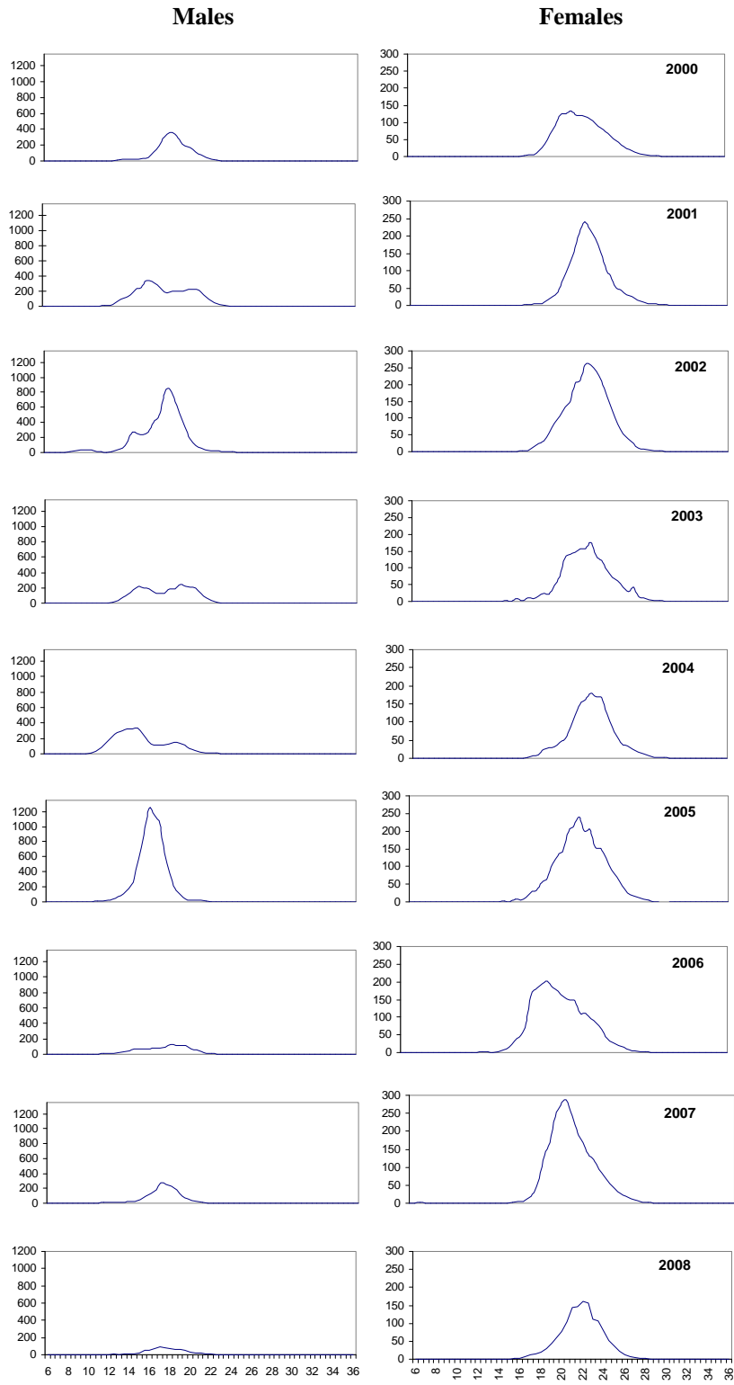
Figure 6. Shrimp size distribution from Flemish Cap 2000-2008 surveys. Y-Axis=Frequency (10 6 ), X-Axis=Carapace Length (mm).
