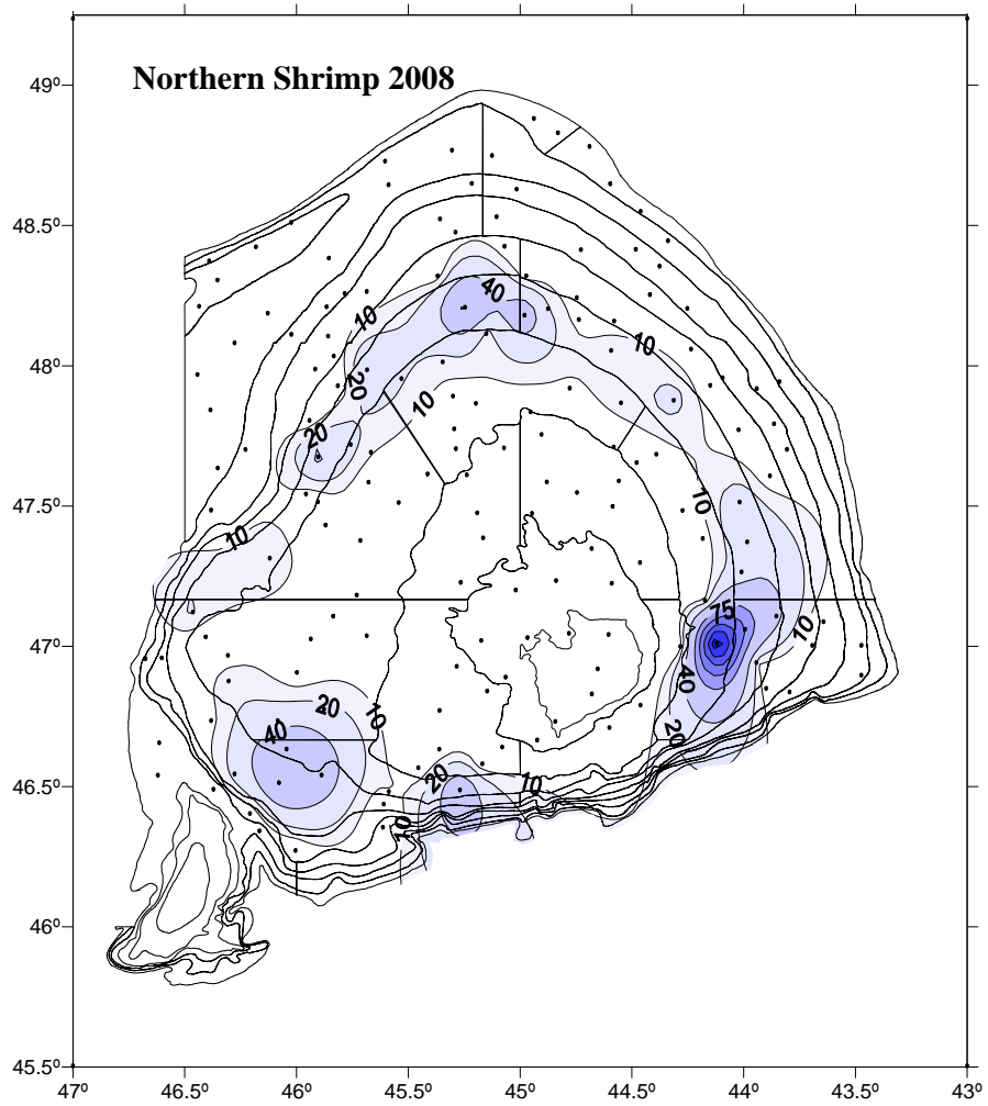
Figure 3. Shrimp catches distribution (kg/tow) from EU Flemish Cap survey in summer 2008.
