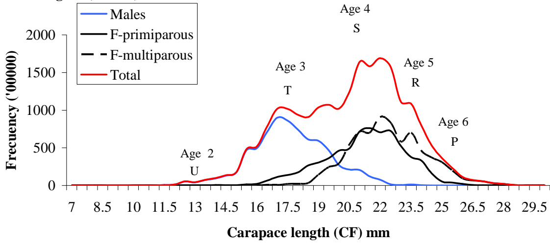
Figure 9. Shrimp modal and age groups in 2008 EU Flemish Cap survey (letters from table 9).
