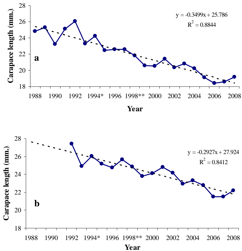
Figure 5.- Lengths (CL) at sex change (a) and maturity (b) of shrimp in the series of EU Flemish Cap surveys
