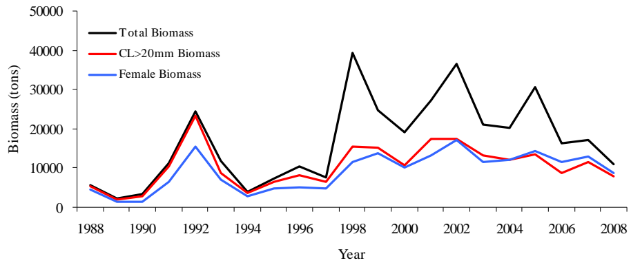
Figure 2. Total, female and adult biomass (shrimp bigger than 20 mm CL) from EU Flemish Cap 1988-2008 surveys.
