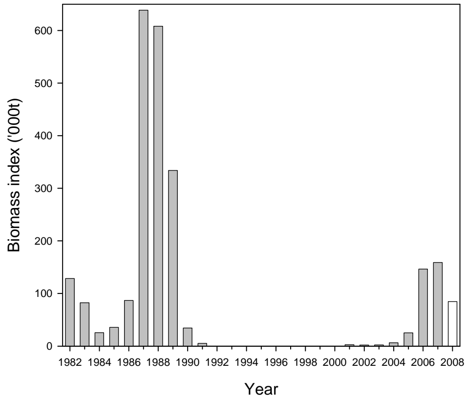
Fig. 4. Survey indices of Atlantic cod biomass for West Greenland offshore waters, 1982-2008 (1982-2007: original estimates from the German groundfish survey; 2008: estimate based on the Greenland Bottom Trawl Survey).
