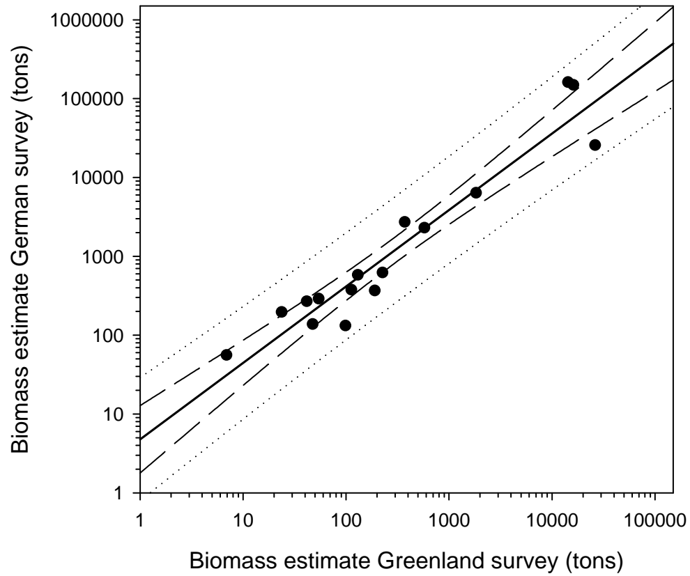
Fig. 2. Relationship between estimates of cod biomass in the overlapping area of the German groundfish survey and the Greenland Bottom Trawl Survey, 1992-2007. Dashed and dotted lines indicate limits of the 95% confidence and prediction intervals, respectively.
