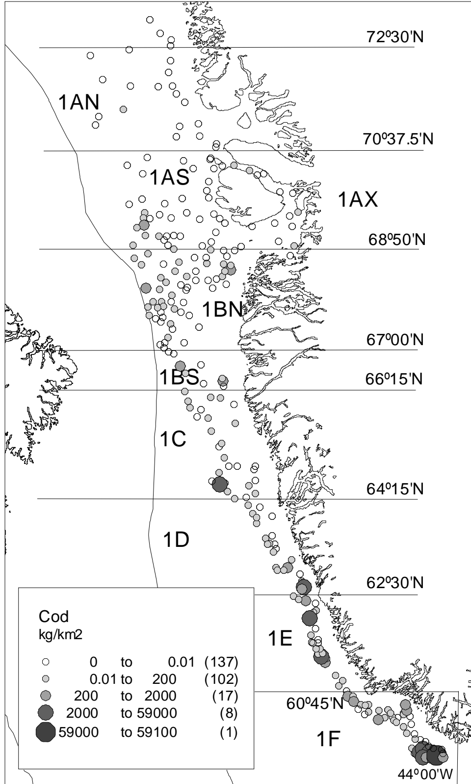
Fig. 3. Geographical distribution of cod density (in kg/km 2 ) in the Greenland Bottom Trawl Survey in 2008. Numbers in parentheses denotes number of tows.
