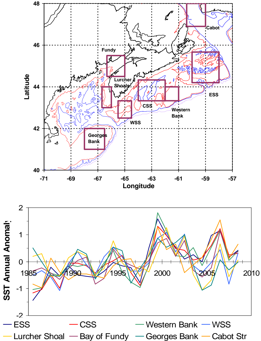
Fig. 7. Scotian Shelf-Gulf of Maine areas used for extraction of sea-surface temperature (upper panel). The annual sea surface temperature anomalies derived from satellite imagery compared to their long-term means (lower panel). Pathfinder estimates were used for September 1985-May 2003. Estimates for June 2003-December 2008 were from the remote sensing laboratory, Ocean Research and Monitoring Section of the Ecosystem Research Division at BIO. These values were adjusted by the regression \text{Pathfinder} = 0.976 \cdot \text{ORMS} + 0.46 based on a comparison between overlapping Pathfinder-ORMS data.
