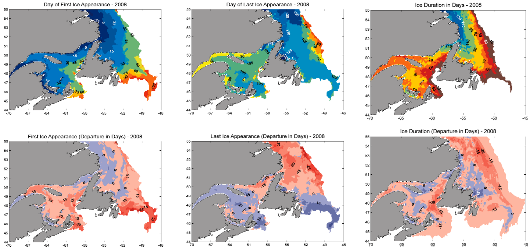
Fig. 5. The time when ice first appeared during 2008 in days from the beginning of the year (left, top panel) and its anomaly from the 1971-2000 mean in days (left, bottom panel). Negative (positive) anomalies indicate earlier (later) than normal appearance. The time when ice was last seen in 2008 in days from the beginning of the year (centre, top panel) and its anomaly from the 1971-2000 mean in days (centre, bottom panel). Positive (negative) anomalies indicate later (earlier) than normal disappearance. The duration of ice in days (right, top panel) during 2008 and the anomalies from the 1971-2000 mean in days (right, bottom panel). Positive (negative) anomalies indicate durations longer (shorter) than the mean.
