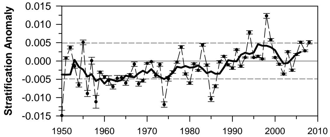
Fig. 11. The mean annual (dashed line with circles) and 5-yr running mean (heavy solid line) of the stratification index (0-50 m density gradient) averaged over the Scotian Shelf (areas 4-23 inclusive, see Fig. 2). The horizontal dashed lines are \pm 1 SD. Standard error estimates for each annual value are also shown.
