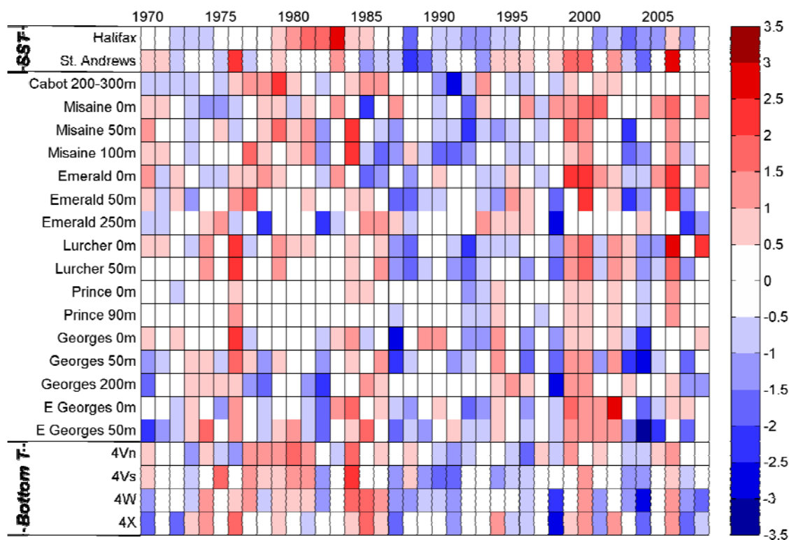
Fig. 13. Normalized annual anomalies of temperatures at the bottom and discrete depths for the Scotian Shelf-Gulf of Maine region. These normalized, annual anomalies are based on the 1971-2000 means, divided by the standard deviation. The scale represents the number of standard deviations an anomaly is from normal; blue indicates below normal, red above normal.
