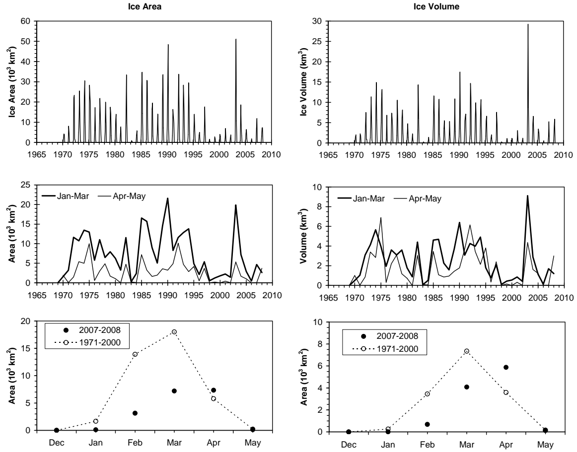
Fig. 6. Time series of the monthly mean ice area for the Scotian Shelf (top panel), the average ice area during the usual periods of advancement (January-March) and retreat (April-May) (middle panel) and the comparison of the monthly areas and volumes to the 1971-2000 means (bottom panel)
