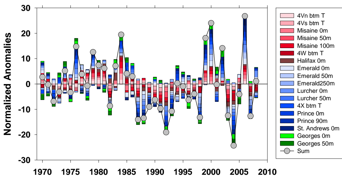
Fig. 14. The contributions of each of the normalized anomalies are shown as a bar chart and their summation as a time series (grey circles, black line).
