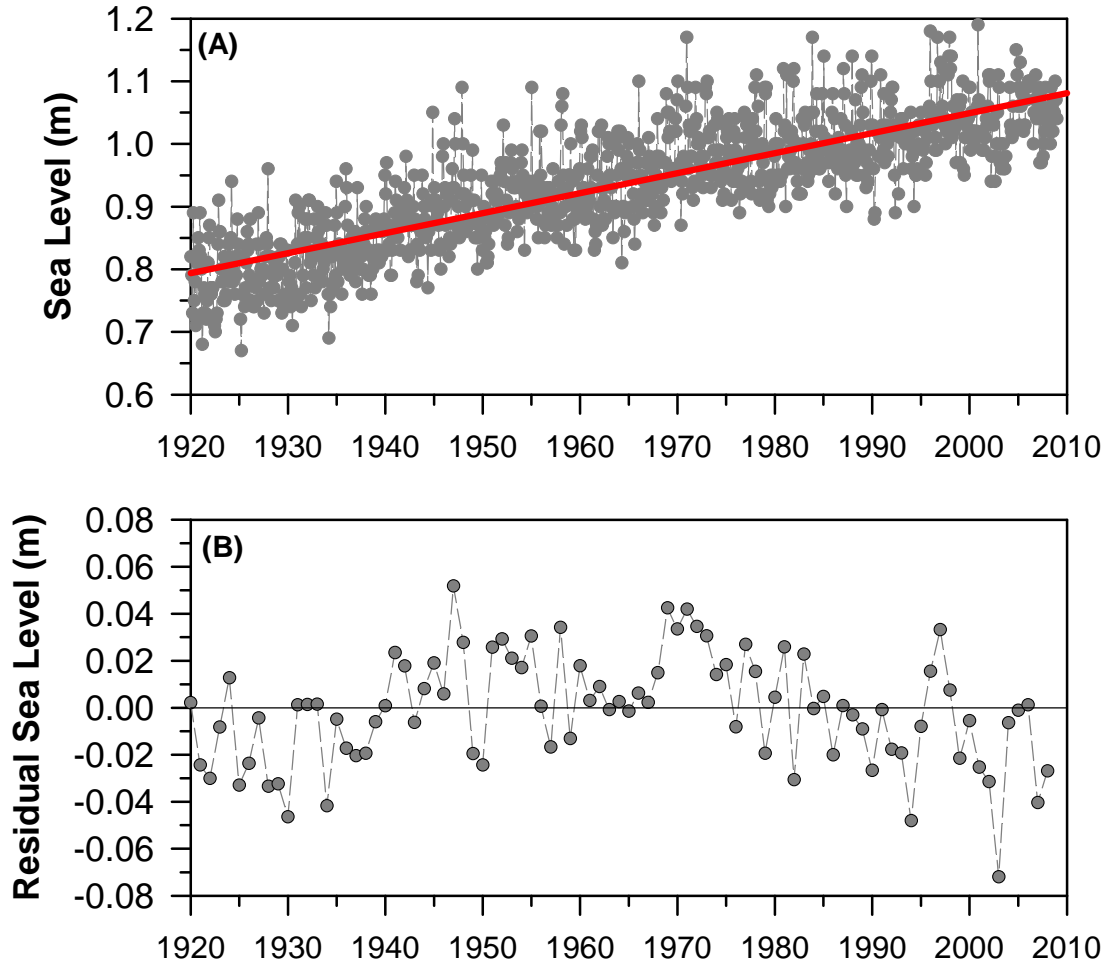
Fig. 12. (A) The time series of the monthly means and a 12 month running mean of the relative sea level elevations at Halifax, along with the linear trend (1920-2008). (B) Residual relative sea level (monthly observed values – linear trend, averaged to annual estimates).
