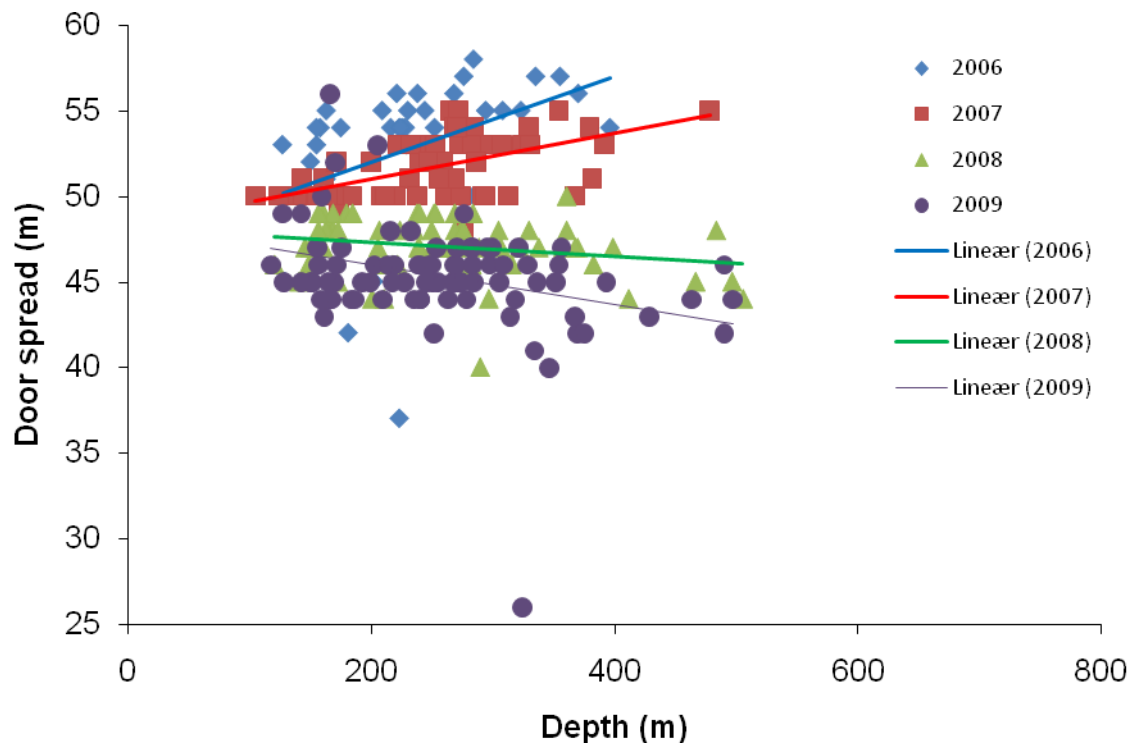
Fig. 4. Door spread vs. depth on the shrimp survey in Skagerrak and the Norwegian Deep (ICES Divs. IIIa and IVa east) in 2006-2009. Strapping was used in 2008 and 2009, but not in 2006 and 2007.
