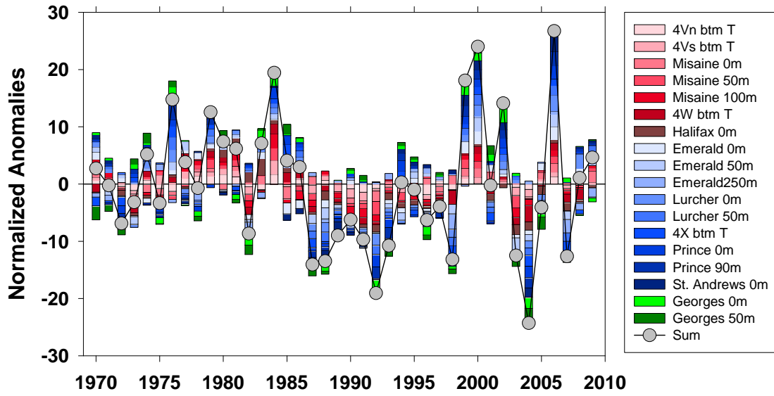
Fig. 15. The contributions of each of the normalized anomalies are shown as a bar chart and their summation as a time series (grey circles, black line).
