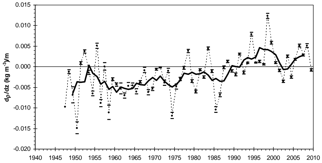
Fig. 11. The mean annual (dashed line with circles) and 5-yr running mean (heavy solid line) of the stratification index (0-50 m density gradient) averaged over the Scotian Shelf (areas 4-23 inclusive, see Fig. 2). The horizontal dashed lines are \pm 1 SD. Standard error estimates for each annual value are also shown.
