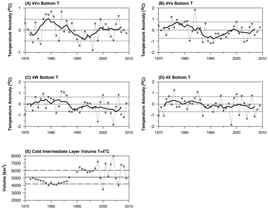
Fig. 10. Time series of July bottom temperature anomalies (dashed lines with circles) and 5 year running mean filtered series (heavy line) for areas (A) 4Vn, (B) 4Vs, (C) 4W and (D) 4X. The horizontal dashed lines are \pm 1 SD. (E) Time series of the Cold Intermediate Layer (CIL, defined as waters with T < 4^{\circ}\text{C} ) volume on the Scotian Shelf based on the July ecosystem survey. The solid horizontal line is the long-term mean, the dashed horizontal lines are the mean \pm 1 SD.
