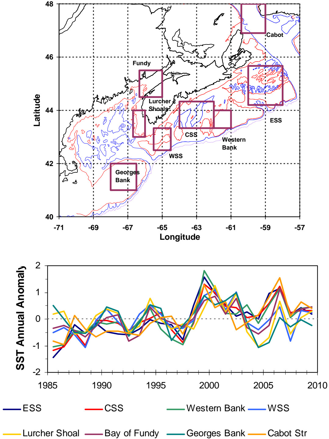
Fig. 7. Scotian Shelf-Gulf of Maine areas used for extraction of sea-surface temperature (upper panel). The annual sea surface temperature anomalies derived from satellite imagery compared to their long-term means (lower panel). Pathfinder estimates were used for September 1985-May 2003. Estimates for June 2003-December 2009 were from the remote sensing laboratory, Ocean Research and Monitoring Section of the Ecosystem Research Division at BIO. These values were adjusted by the regression \text{Pathfinder} = 0.976 * \text{ORMS} + 0.46 based on a comparison between overlapping Pathfinder-ORMS data.
