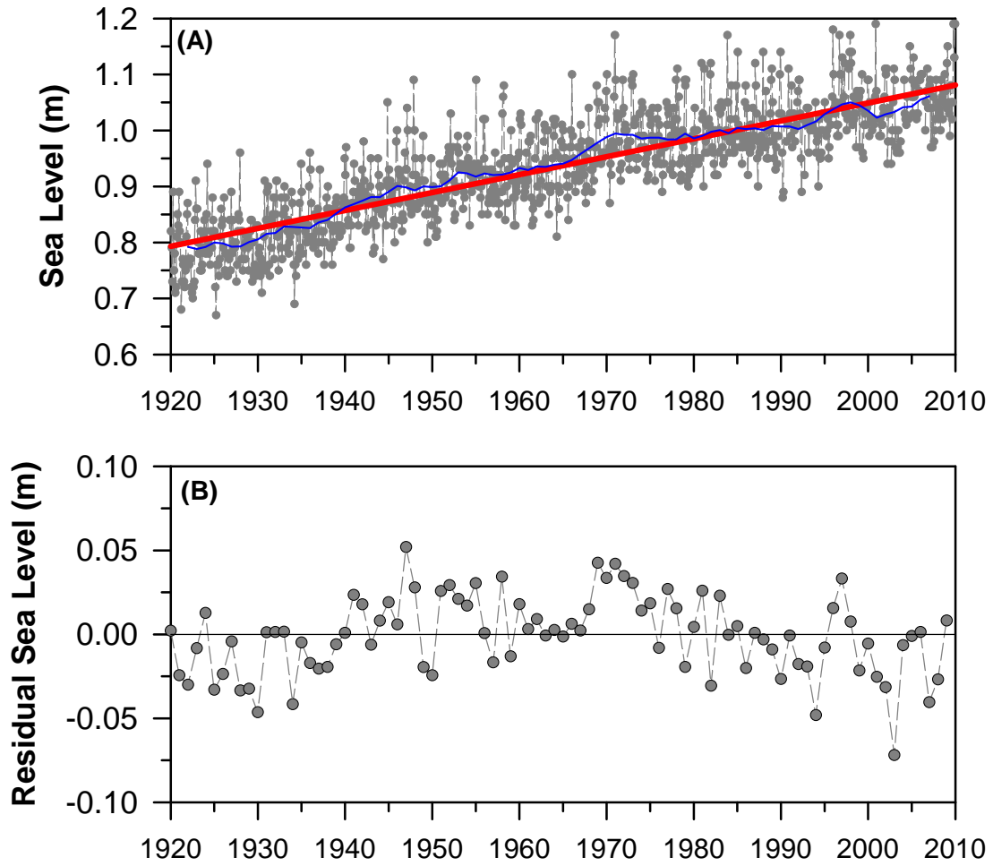
Fig. 12. (A) The time series of the monthly means (grey) and a 5 year running mean (blue) of the relative sea level elevations at Halifax, along with the linear trend (1920-2009, red). (B) Residual relative sea level (monthly observed values – linear trend, averaged to annual estimates).
