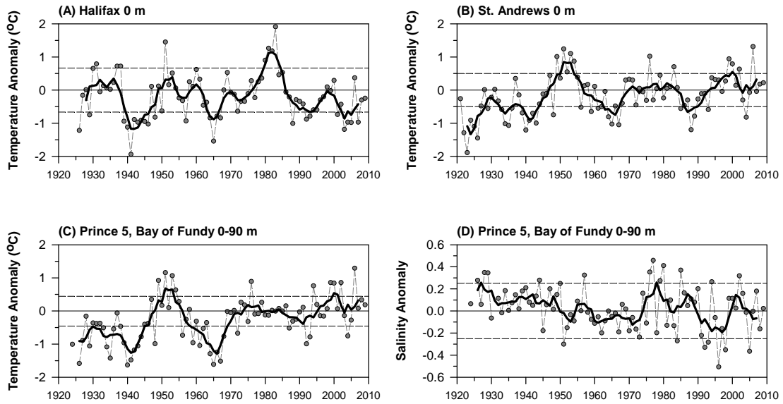
Fig. 8. The annual surface temperature anomalies (dashed line with circles) and their 5-year running means (heavy black line) for (A) Halifax Harbour and (B) St. Andrews; annual depth-averaged (0-90 m) (C) temperature and (D) salinity anomalies for the Prince 5 monitoring station at the mouth of the Bay of Fundy. Horizontal dashed lines mark \pm 1 standard deviation.
