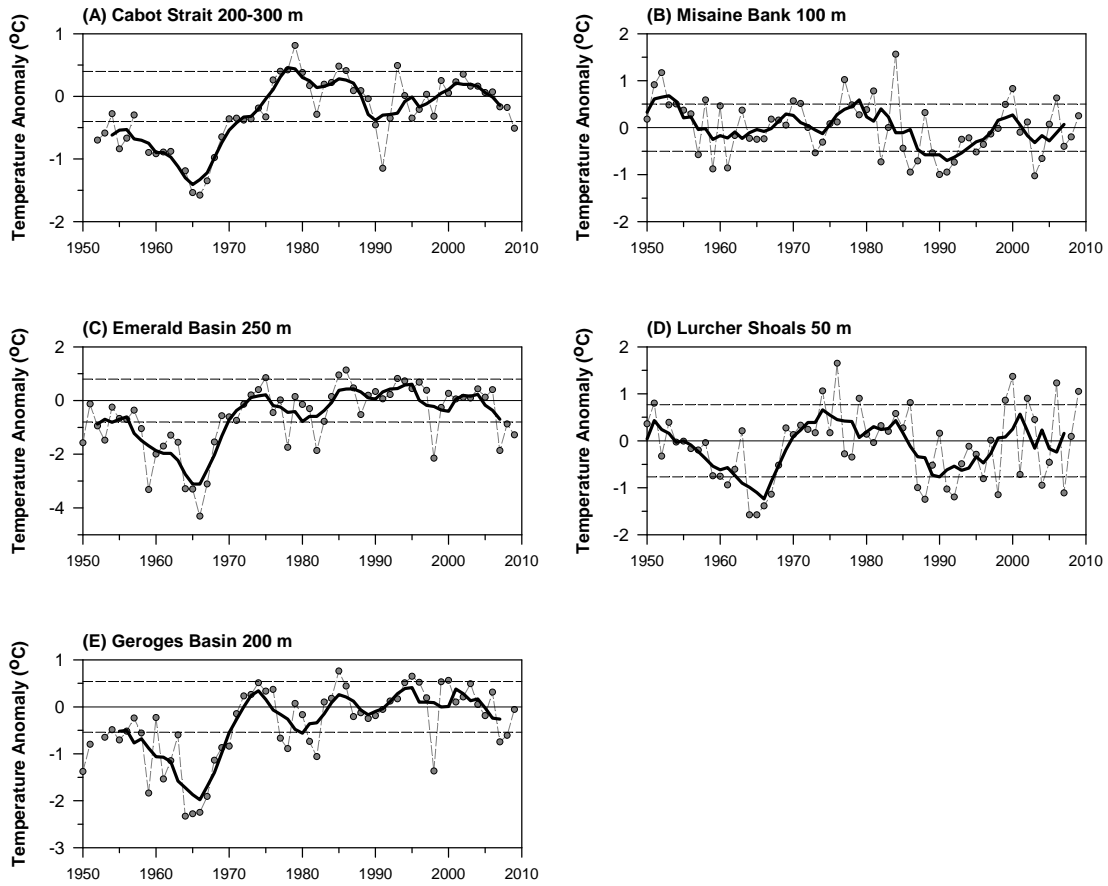
Fig. 9. The annual mean temperature anomaly time series (dashed line with circles) and the 5 year running mean filtered anomalies (heavy solid line) on the Scotian Shelf and in the Gulf of Maine at (A) Cabot Strait 200-300 m; (B) Misaine Bank 100 m; (C) Emerald Basin 250 m; (D) Lurcher Shoals 50 m; and Georges Basin (200 m) (see Fig. 2).
