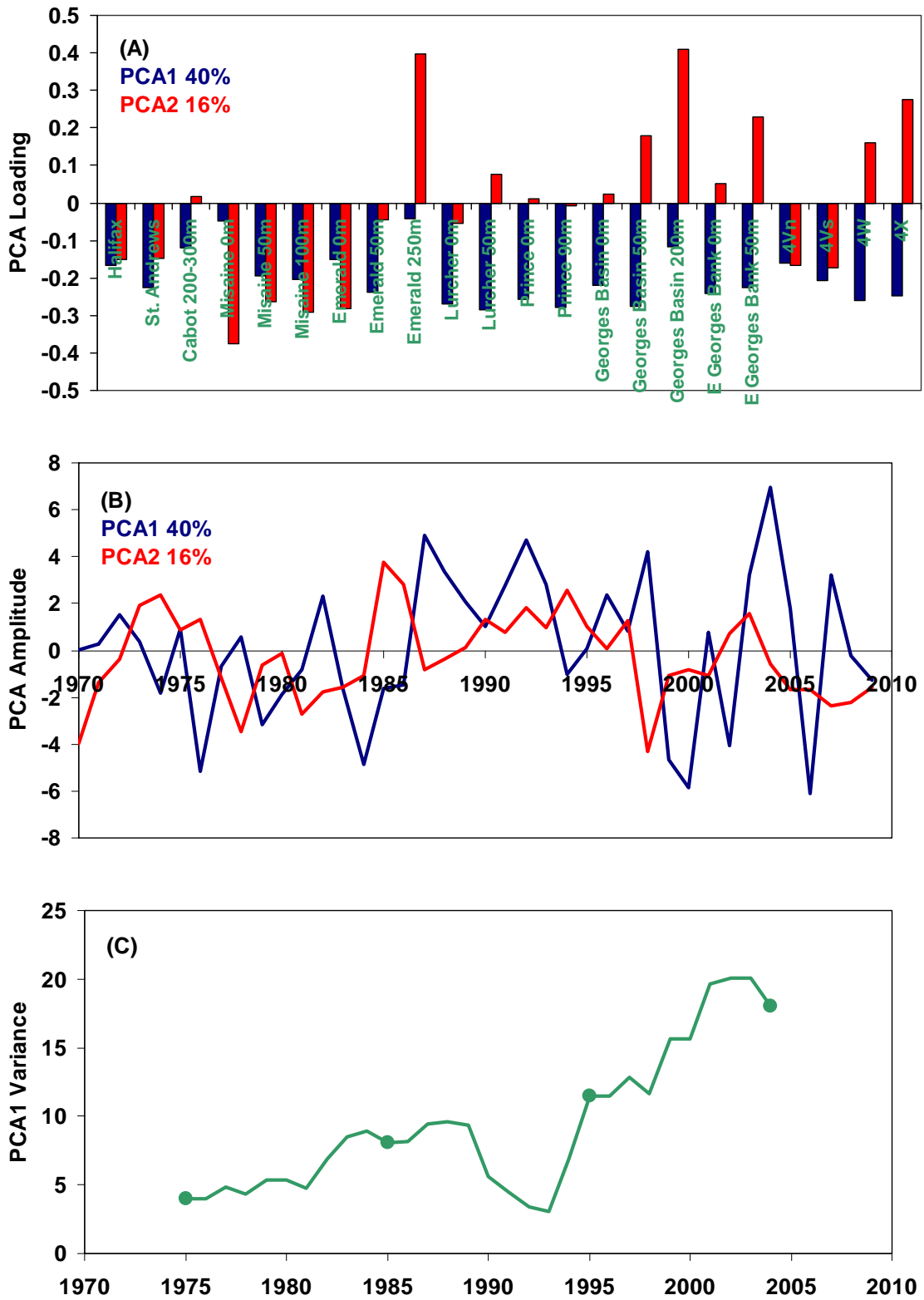
Figure 14. (A) Principal components 1 and 2 loadings. (B) Times series of PCA1, 2. (C) Variance in 11 year blocks of PCA1; points indicate values for blocks 1970-80, 1980-90, 1990-2000 and 1999-2009.
