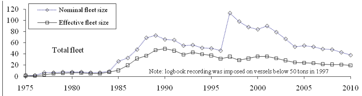
Fig. 1a. Nominal and effective sizes of the trawler fleet in the West Greenland shrimp fishery, 1975–2010, from logbook records.
