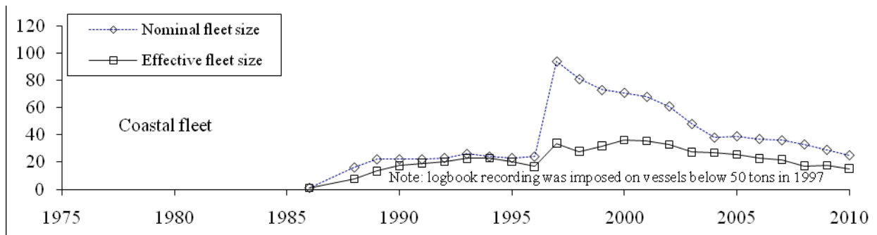
Fig. 1c. Nominal and effective sizes of the coastal trawler fleet in the West Greenland shrimp fishery, 1986–2010, from logbook records.
