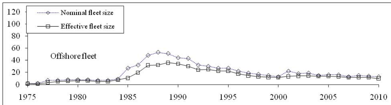
Fig. 1b. Nominal and effective sizes of the offshore trawler fleet in the West Greenland shrimp fishery, 1975–2010, from logbook records.
