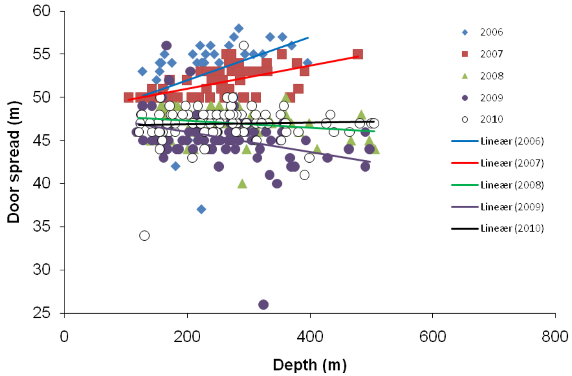
Fig. 5. Door spread vs. depth on the shrimp survey in Skagerrak and the Norwegian Deep (ICES Divs. IIIa and IVa east) in 2006-2010. Strapping was used in 2008-2010, but not in 2006 and 2007.
