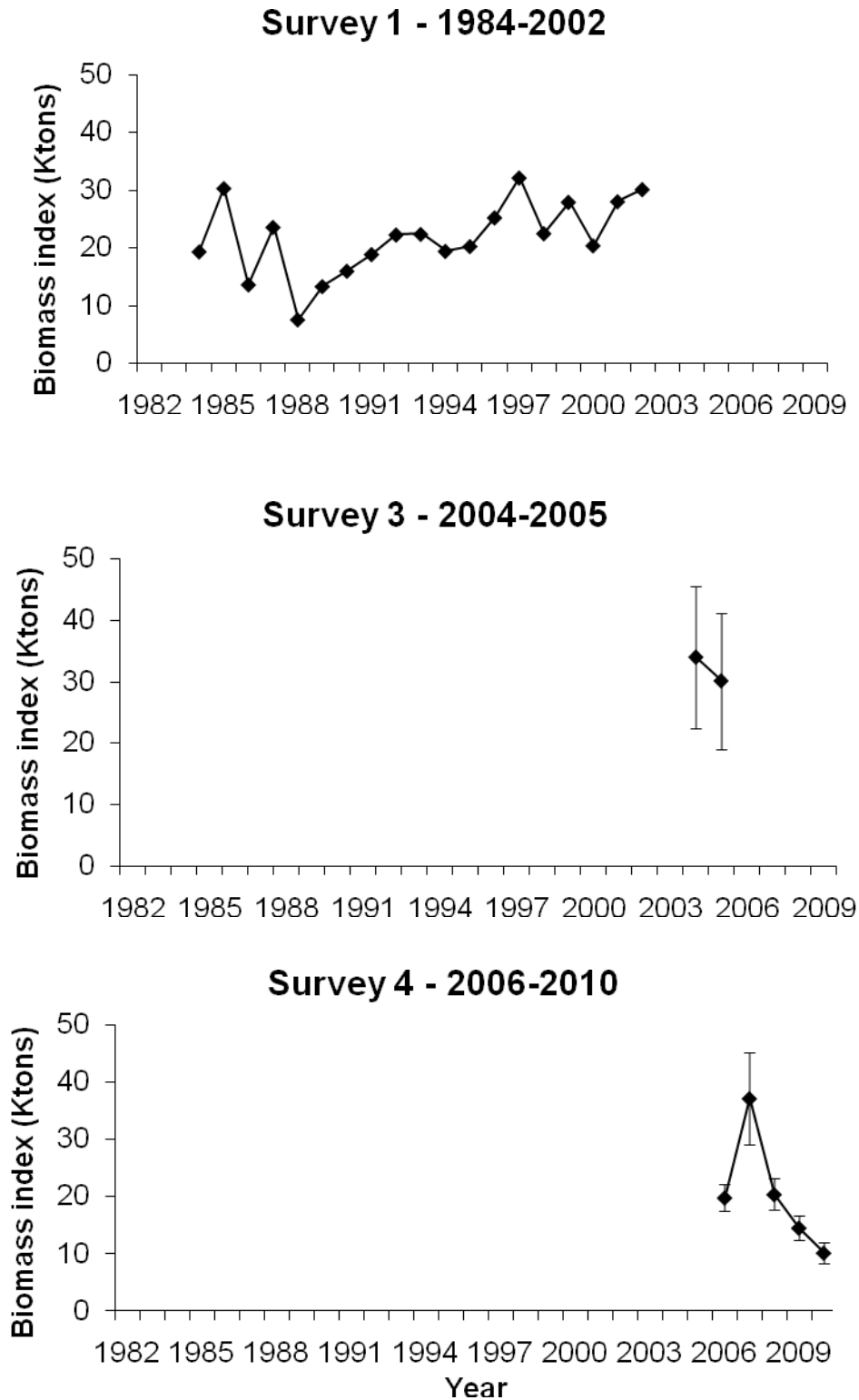
Fig. 6. Estimated survey biomass indices of shrimp ( Pandalus borealis ) in Skagerrak and the Norwegian Deep (ICES Divs. IIIa and IVa east), 1984-2010 (see Table 3). The 2003-estimate is not shown. Standard errors have been calculated for the 2004-2010 surveys.
