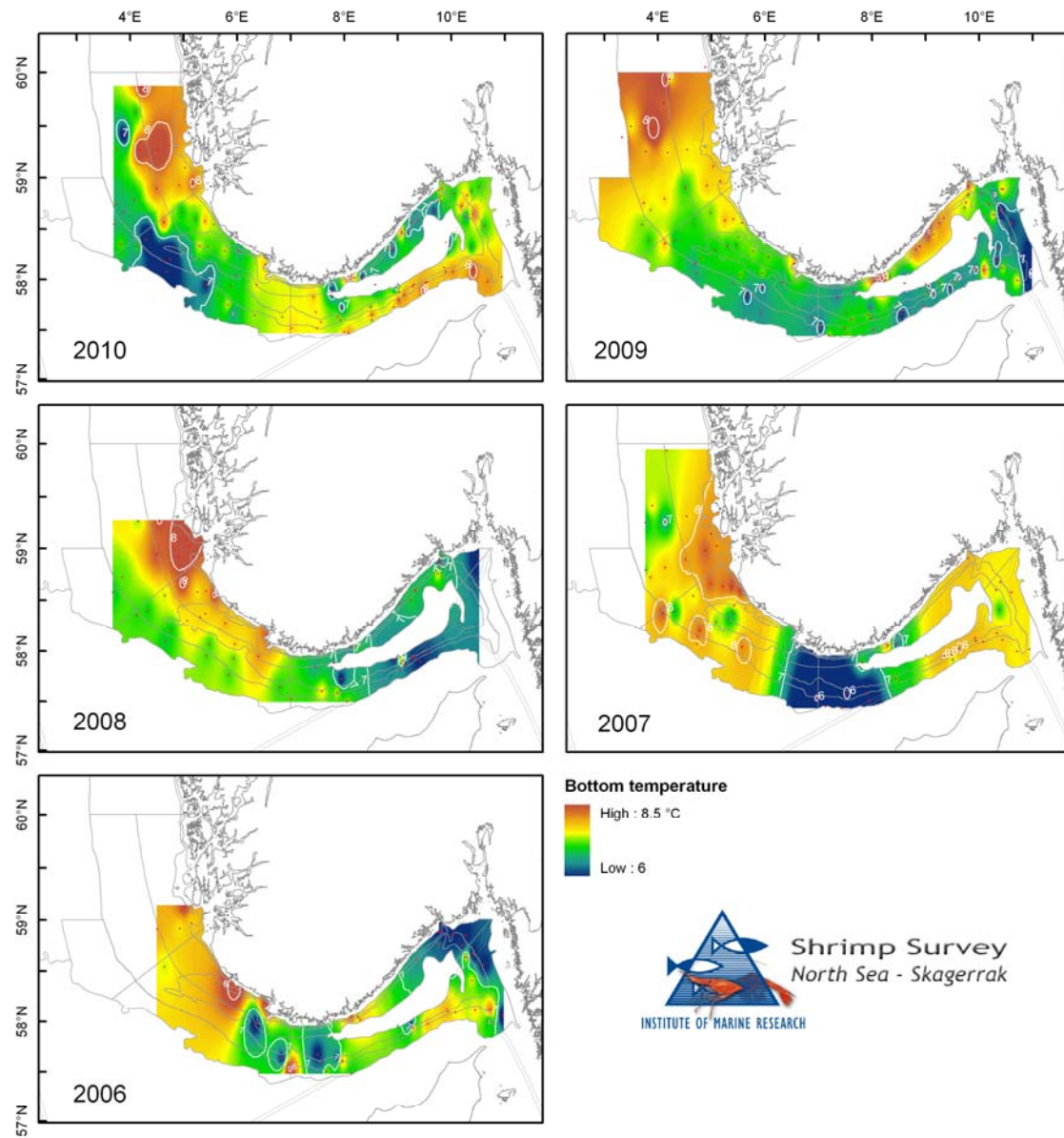
Fig. 4. Temperatures (°C) measured with CTD on trawl stations during the 2006-2010 shrimp surveys in Skagerrak and the Norwegian Deep (ICES Divs. IIIa and IVa east).
