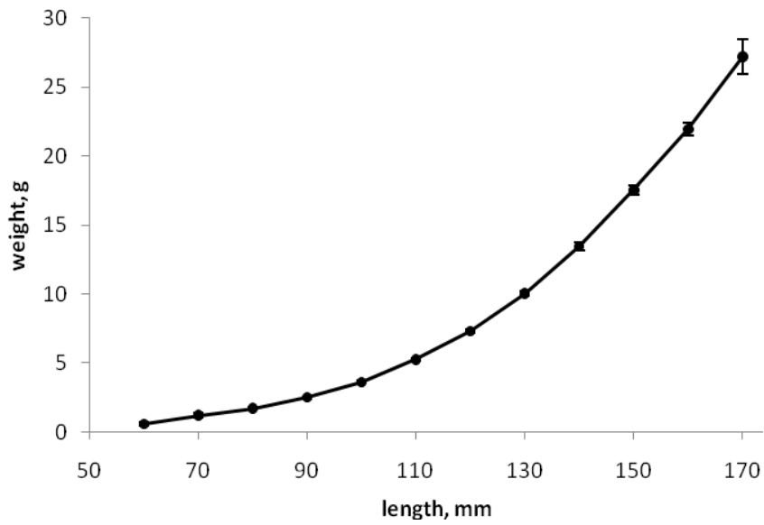
Fig. 3. 3NO capelin length-weight relationship in 2010.
