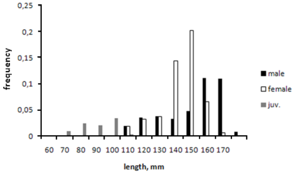
Fig. 2. Length composition of capelin on the spring survey data in 2010
