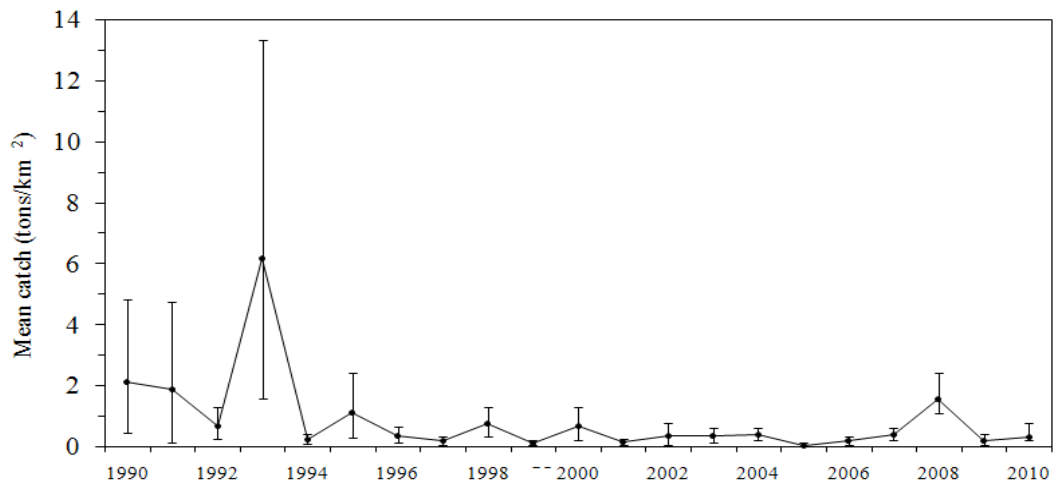
Fig. 5. Average catch ( t/km^2 ) according to the data of Canadian spring surveys in Div. 3NO.
