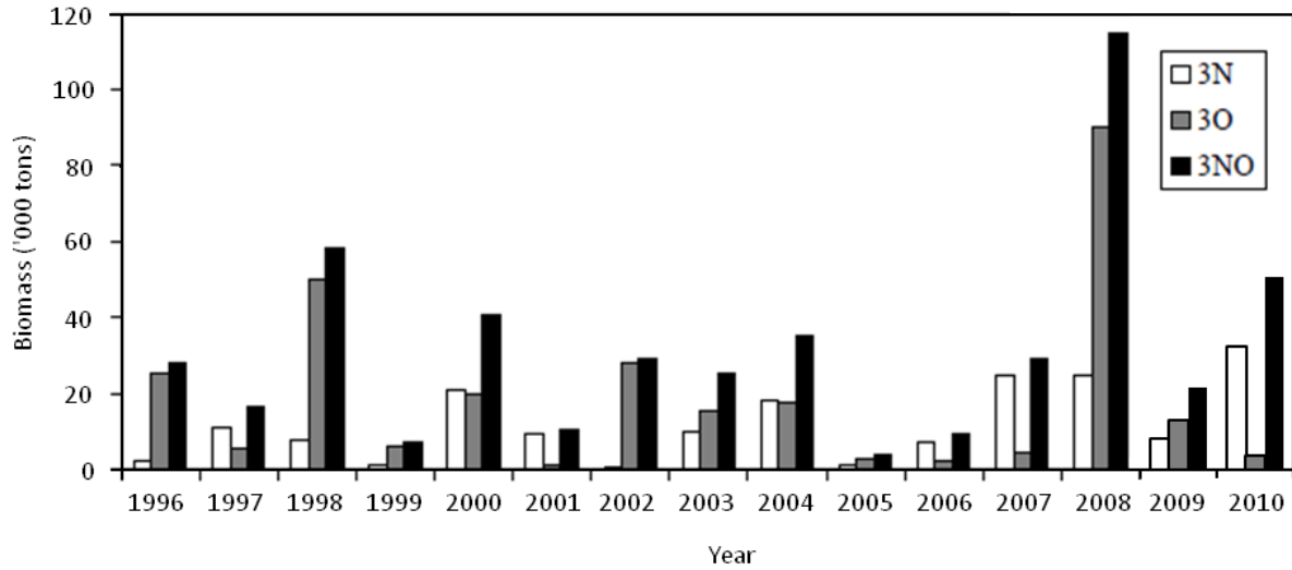
Fig. 4. Estimates of trawl biomass of capelin in Div. 3NO according to the data of Canadian spring surveys conducted in 1996-2010.
