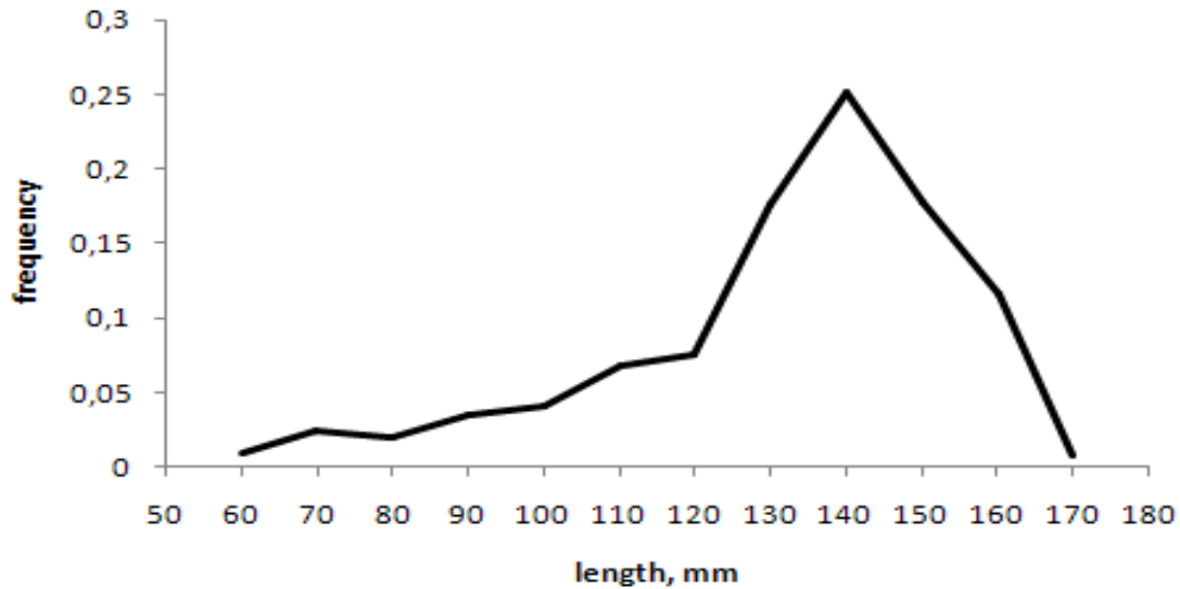
Fig. 1. 3NO capelin length series from spring surveys in 2010
