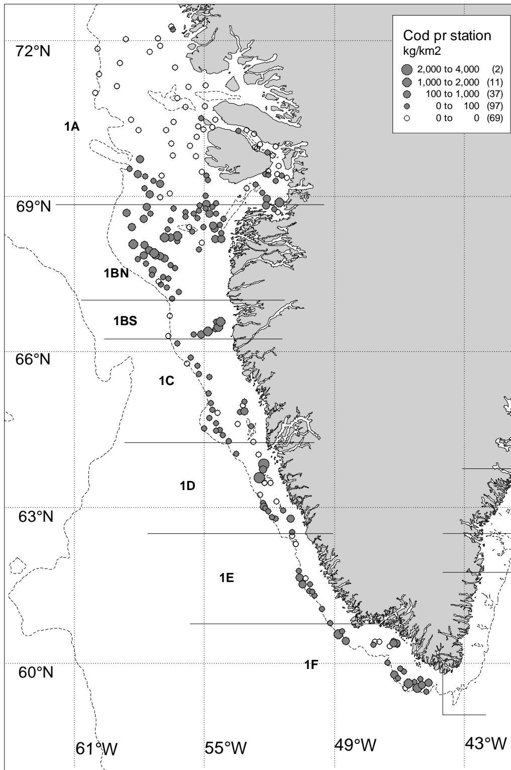
Fig. 3. Geographical distribution of cod density (in kg/km 2 ) in the Greenland Bottom Trawl Survey in 2011. Numbers in parentheses denotes number of tows.
