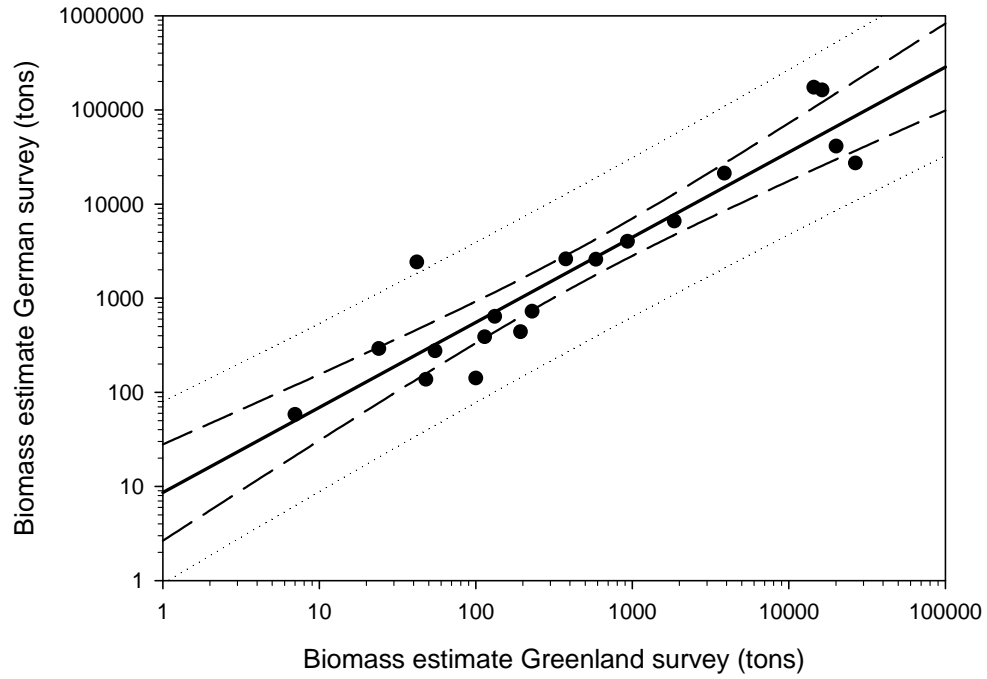
Fig. 2. Relationship between estimates of cod biomass in the overlapping area of the German groundfish survey and the Greenland Bottom Trawl Survey, 1992-2010. Dashed and dotted lines indicate limits of the 95% confidence and prediction intervals, respectively.
