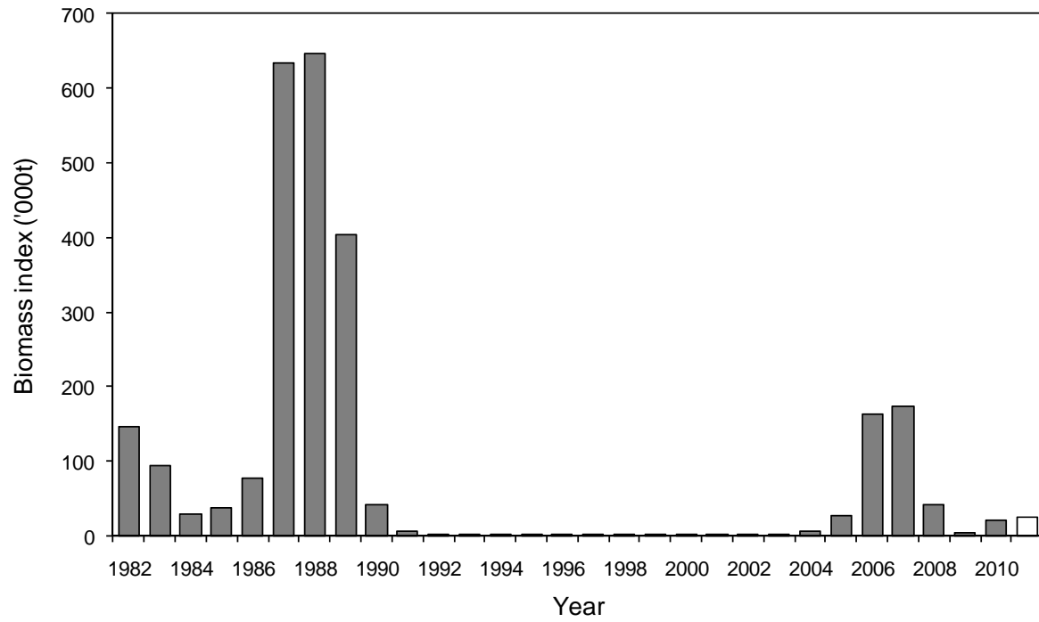
Fig. 4. Survey indices of Atlantic cod biomass for West Greenland offshore waters, 1982-2011 (1982-2010: original estimates from the German groundfish survey; 2011: estimate based on the Greenland Bottom Trawl Survey).
