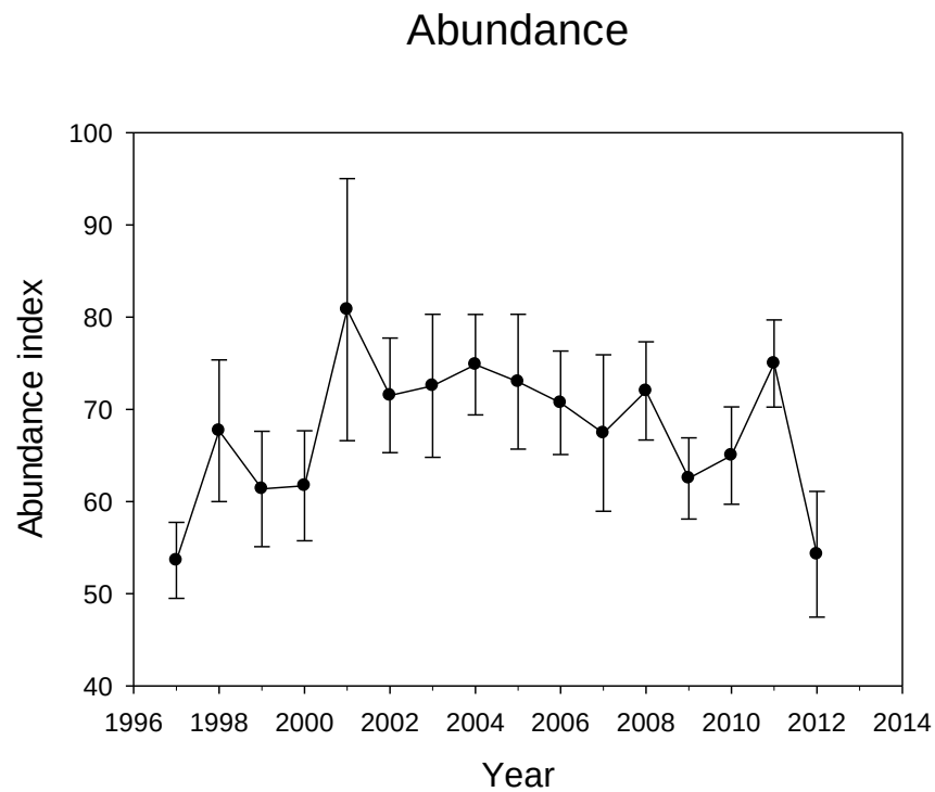
Fig. 5. Abundance (millions) of Greenland halibut in Div. 1CD by year with 1*S.E.
