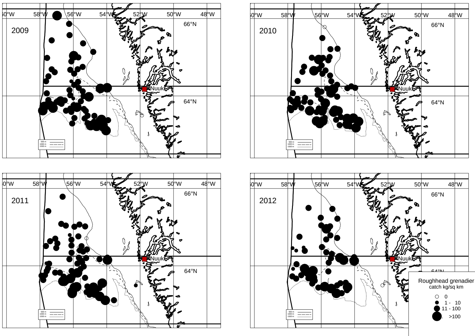
Fig. 11 cont.. Distribution of catches of roughhead grenadier during 2009-2012 \text{km}^{-2} .
