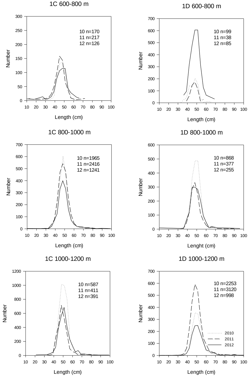
Fig. 7. Length distribution of Greenland halibut in numbers \text{km}^{-2} by year, Division and depth stratum. Div 1CD 600-1200 m.
