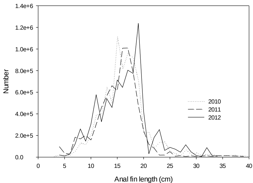
Fig. 10. Overall length distribution (pre anal fin length) of roughhead grenadier in numbers (weighted by stratum area) in Div. 1CD by year.
