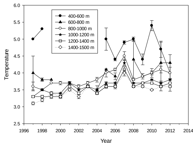
Fig 14. Mean temperatures by division depth stratum and year with 1*S.E.
