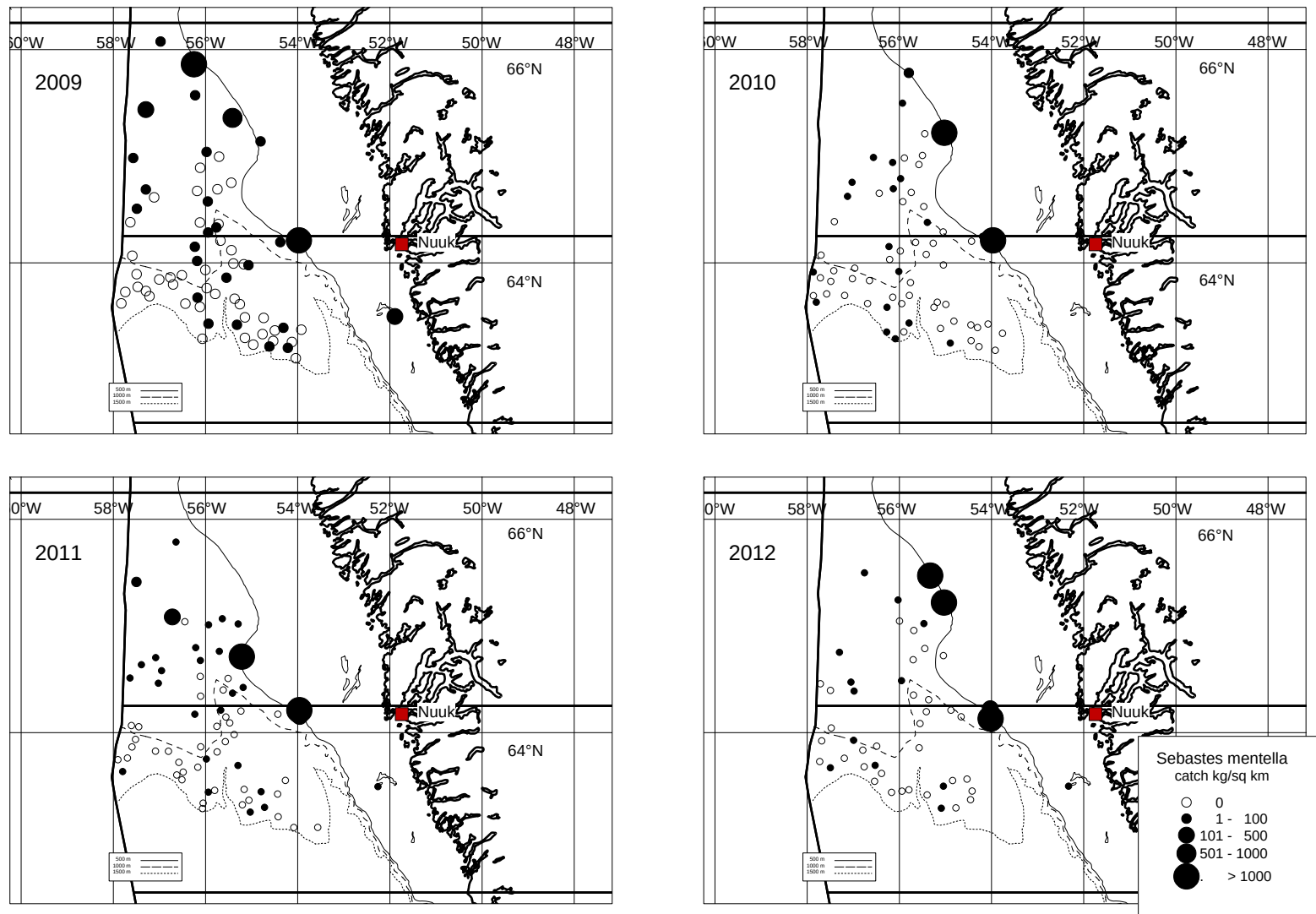
Fig. 13. Distribution of catches of deep sea redfish during 2009-2012 \text{km}^{-2} .
