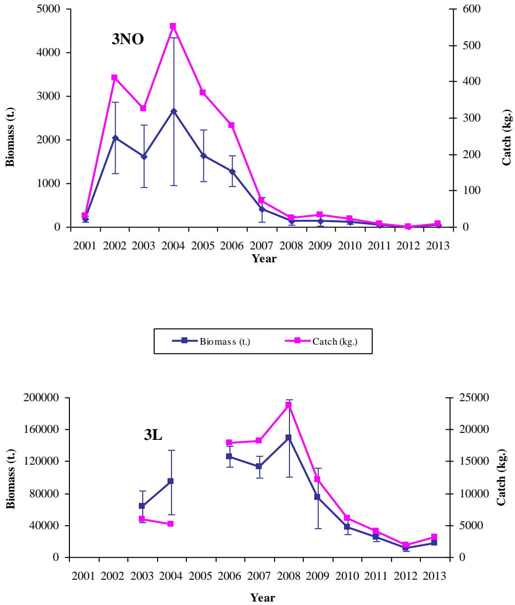
Figure 1.- Northern shrimp biomass (tons) and catch (kg) from Spanish research surveys in NAFO Div. 3NO 2001-2013 and 3L 2003-2013.
