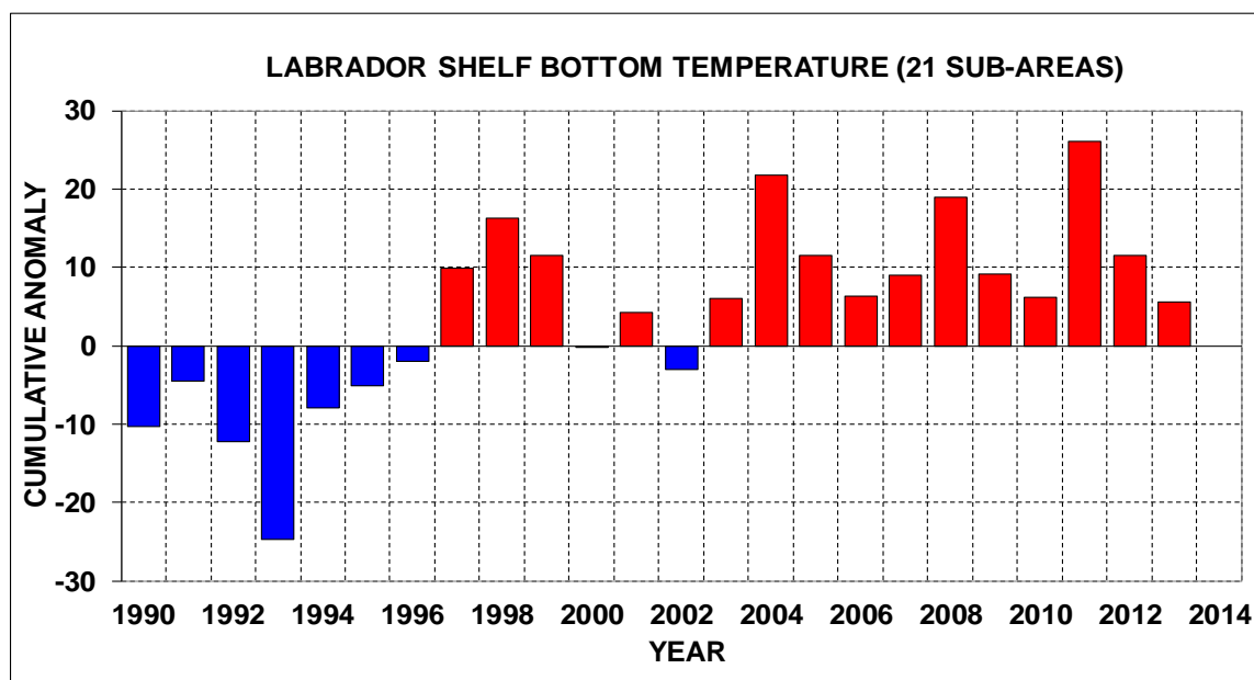
Figure 21. Cumulative bottom temperature anomalies based on the values presented in Fig. 20 for the Labrador Shelf.
