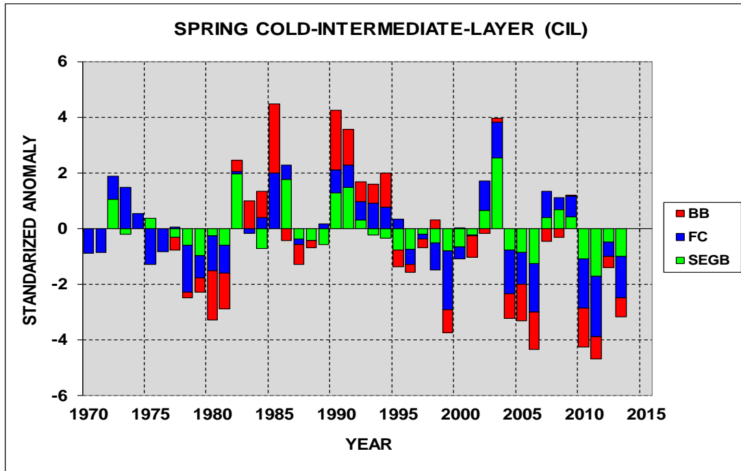
Figure 26. Cold-Intermediate-Layer areas during the spring along the Bonavista, Flemish Cap and the south east Grand Bank sections displayed as cumulative standardized anomalies relative to 1981-2010.
