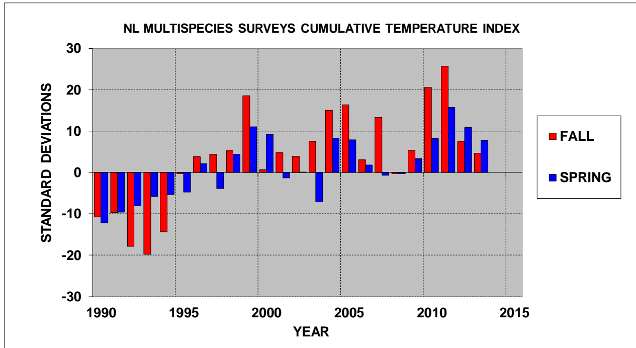
Figure 35. Temperature indices derived from data collected during fall multi-species survey. The anomalies are normalized with respect to their standard deviations.
