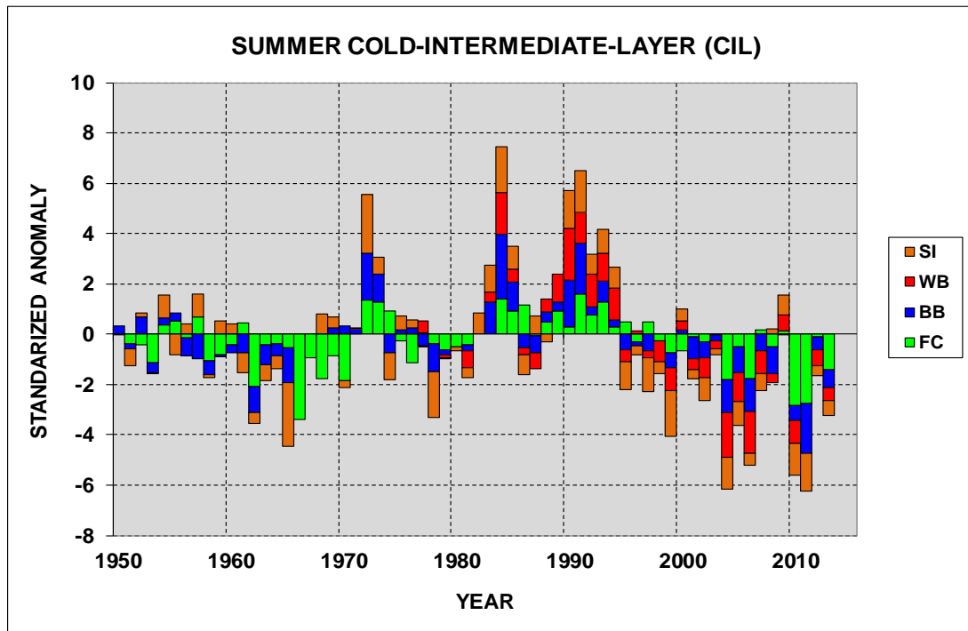
Figure 27. Cold-Intermediate-Layer areas during the summer along the Seal Island, White Bay, Bonavista and Flemish Cap sections displayed as cumulative standardized anomalies relative to 1981-2010.
