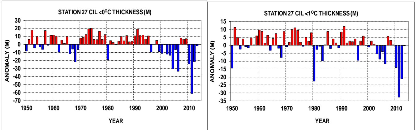
Figure 15. Annual Station 27 CIL (<0°C, <1°C) thickness anomalies referenced to the 1981-2010 mean.
