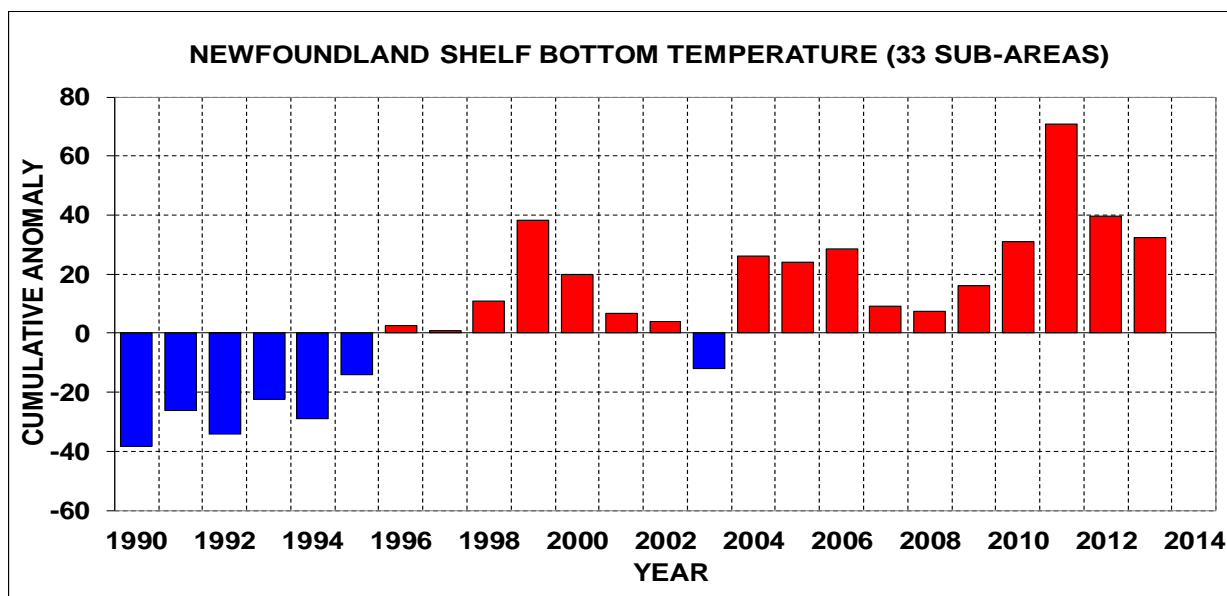
Figure 23. Cumulative bottom temperature anomalies based on the values presented in Fig. 22 for the areas on the Newfoundland Shelf shown in Fig. 19.
