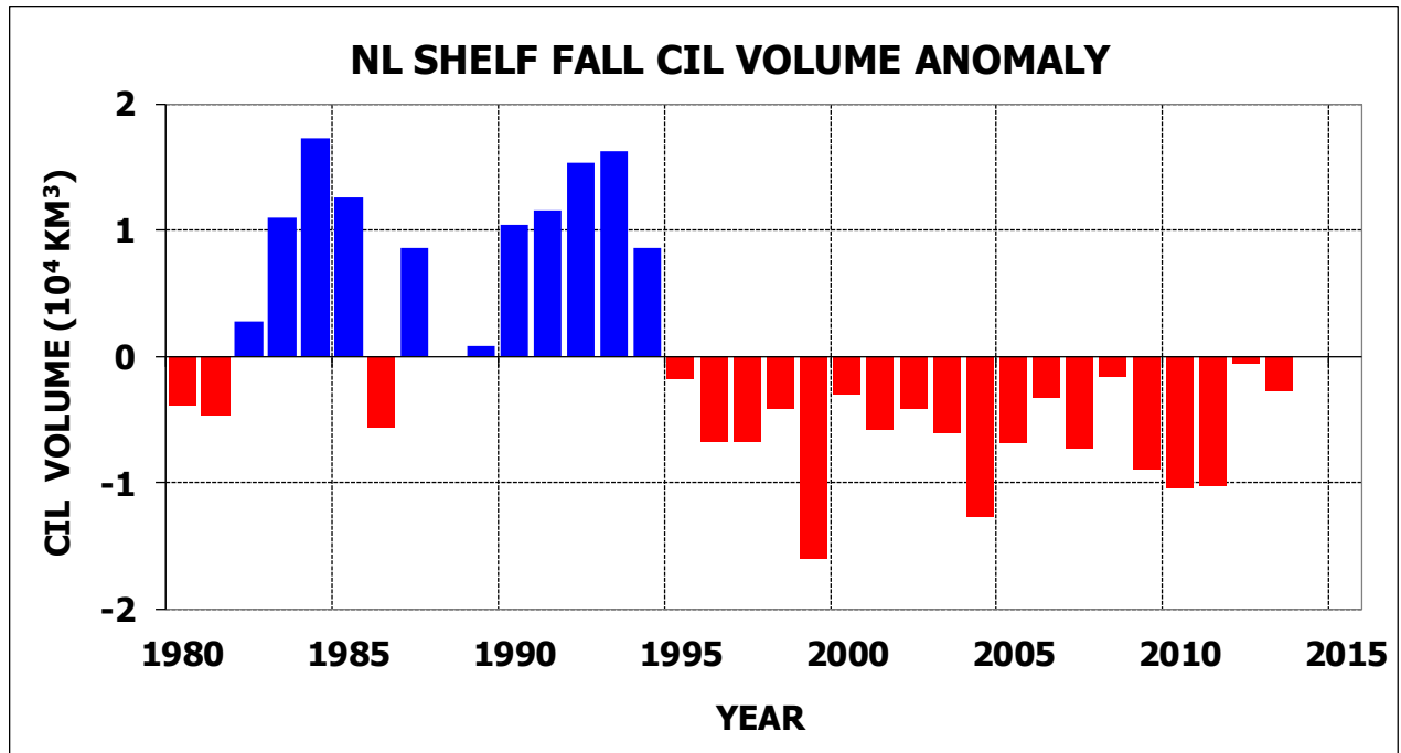
Figure 37. Time series of the CIL ( <0^{\circ}\text{C} ) volume anomaly on the NL shelf bounded by NAFO Divs. 2J3KL based on the fall multi-species survey temperature data profiles. No data were available in 1988.
