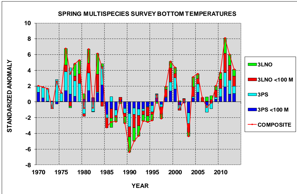
Figure 31. Standardized bottom temperature anomalies from the spring multi-species surveys in NAFO Divs. 3LNOP.
