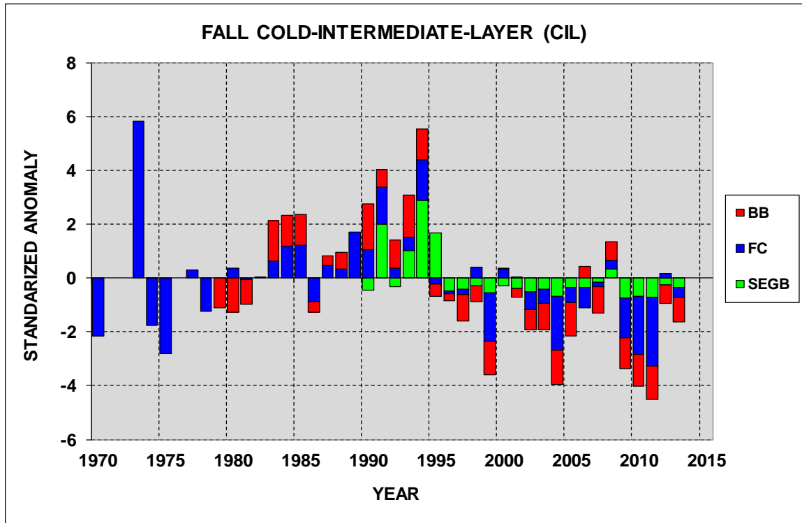
Figure 28. Cold-Intermediate-Layer areas during the fall along the Bonavista, Flemish Cap and the south east Grand Bank sections displayed as cumulative standardized anomalies relative to 1981-2010.
