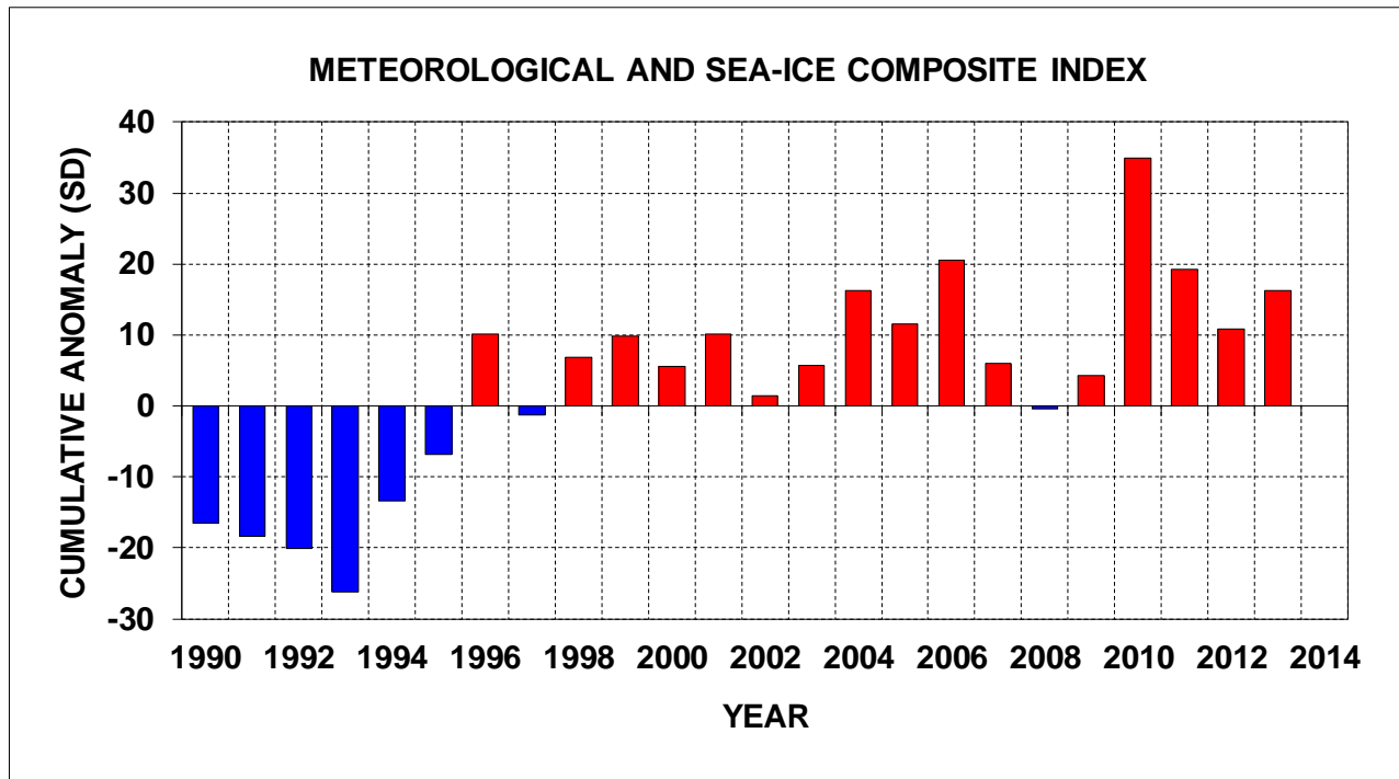
Figure 7. Meteorological and sea-ice composite index derived by summing the standardized anomalies from Fig. 5.
