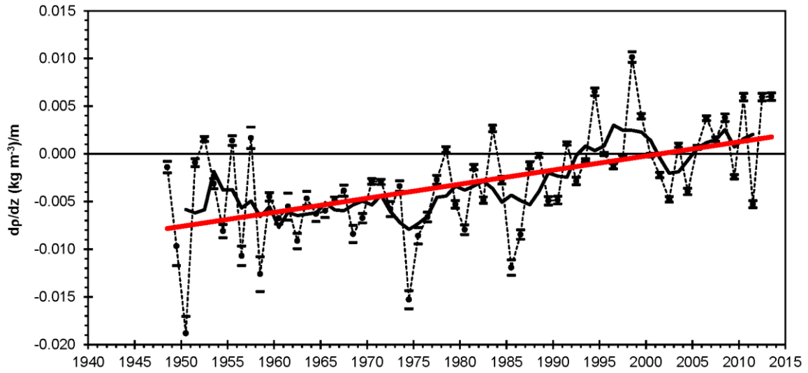
Fig. 13. The mean annual anomaly (dashed line with circles) and 5-yr running mean (heavy solid line) of the stratification index (0-50 m density gradient) averaged over the Scotian Shelf (areas 4-23 inclusive, see Fig. 2). Standard error estimates for each annual anomaly value are also shown. The linear trend (red line) shows a change in the 0-50 m density difference of 0.37 \text{ kg m}^{-3} over 50 years.
