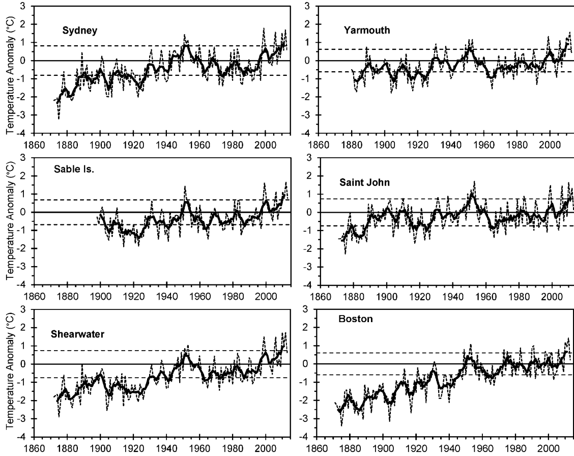
Fig. 3. Annual air temperature anomalies in ^{\circ}\text{C} (dashed line) and five year running means (solid line) at selected sites (Sydney, Sable Island, Shearwater, Yarmouth, Saint John and Boston) in the Scotian Shelf-Gulf of Maine region (years 1860 to 2013). Horizontal dashed lines represent \pm 1 SD for the 1981-2010 period.
