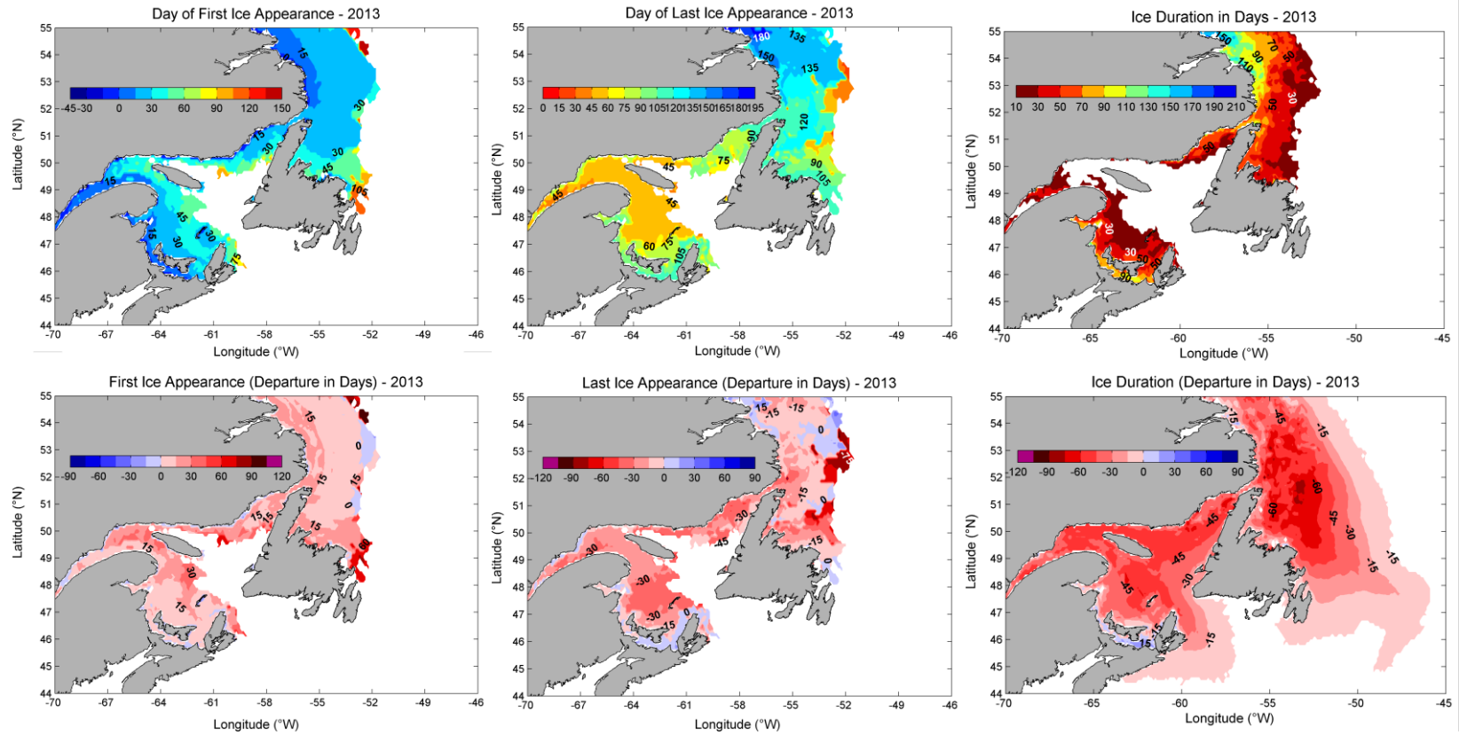
Fig. 5. The time when ice first appeared during 2013 in days from the beginning of the year (left, top panel) and its anomaly from the 1981-2010 mean in days (left, bottom panel). Negative (positive) anomalies indicate earlier (later) than normal appearance. The time when ice was last seen in 2013 in days from the beginning of the year (centre, top panel) and its anomaly from the 1981-2010 mean in days (centre, bottom panel). Positive (negative) anomalies indicate later (earlier) than normal disappearance. The duration of ice in days (right, top panel) during 2013 and the anomalies from the 1981-2010 mean in days (right, bottom panel). Positive (negative) anomalies indicate durations longer (shorter) than the mean.
