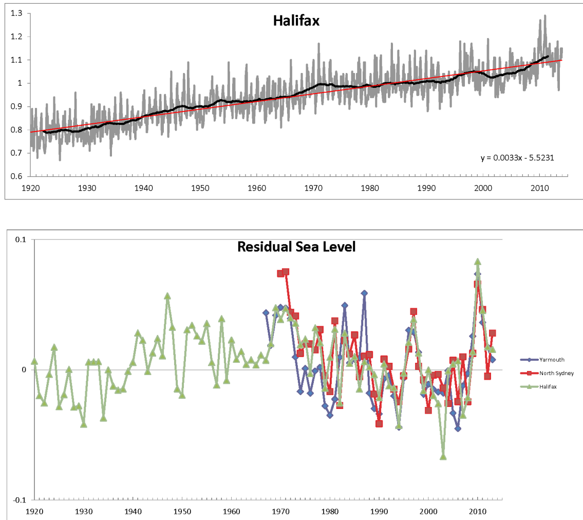
Fig. 14. The time series of the monthly means (gray) and a 5 year running mean (black) of the relative sea level elevations at Halifax, along with the linear trend (red) over 1920-2013 (upper panel). Residual relative sea level (monthly observed values – (1981-2010) linear trend, averaged to annual estimates) for Halifax (green), Yarmouth (blue) and North Sydney (red).
