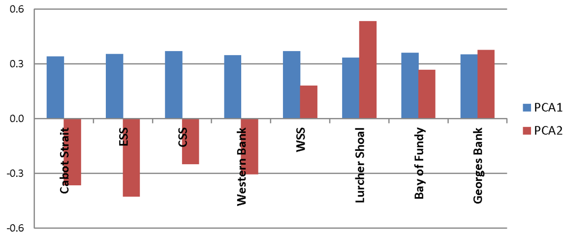
Fig. 8. First (PCA1: 83% of the variance) and second (PCA2: 8% of the variance) loadings from a principal components analysis of the annual mean temperature anomalies (Figure 7, lower panel) for the eight Scotian Shelf and Gulf of Maine regions (Cabot Strait, Eastern Scotian Shelf (EES), Western Bank, Central Scotian Shelf (CSS), Western Scotian Shelf (WSS), Georges Bank, Lurcher Shoals and Bay of Fundy -Figure 7, upper panel).
