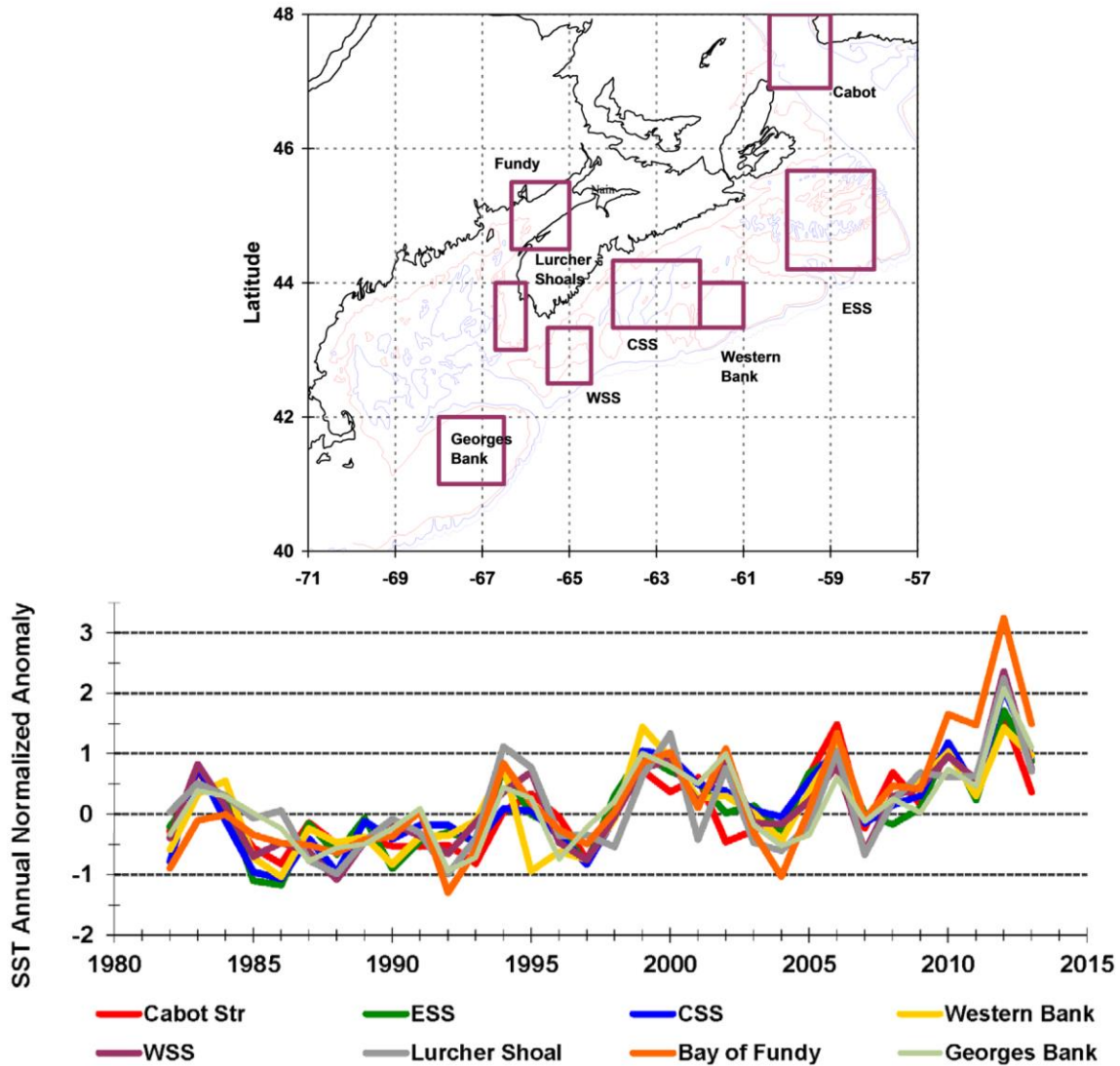
Fig. 7 Scotian Shelf-Gulf of Maine areas (Cabot Strait, Eastern Scotian Shelf (EES), Western Bank, Central Scotian Shelf (CSS), Western Scotian Shelf (WSS), Georges Bank, Lurcher Shoals and Bay of Fundy) used for extraction of sea surface temperature (upper panel). The annual sea surface temperature anomalies derived from satellite imagery compared to their long-term monthly means (lower panel).
