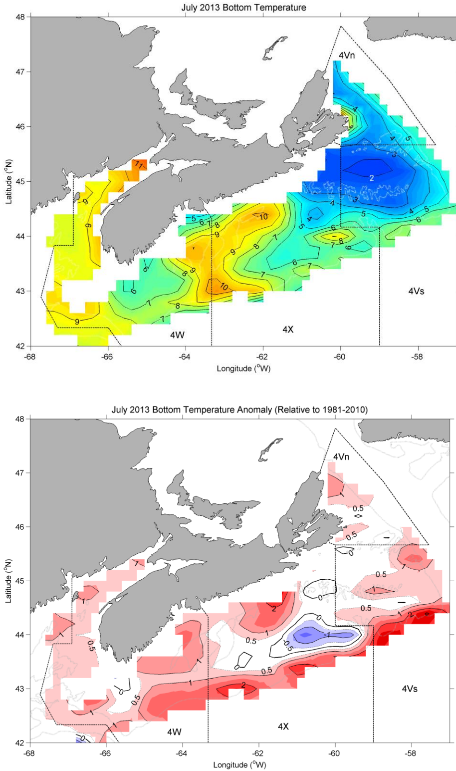
Fig. 11. July bottom temperature (upper panel) and anomaly (lower panel) maps for 2013. NAFO areas 4Vn, 4Vs, 4X and 4W are shown.
