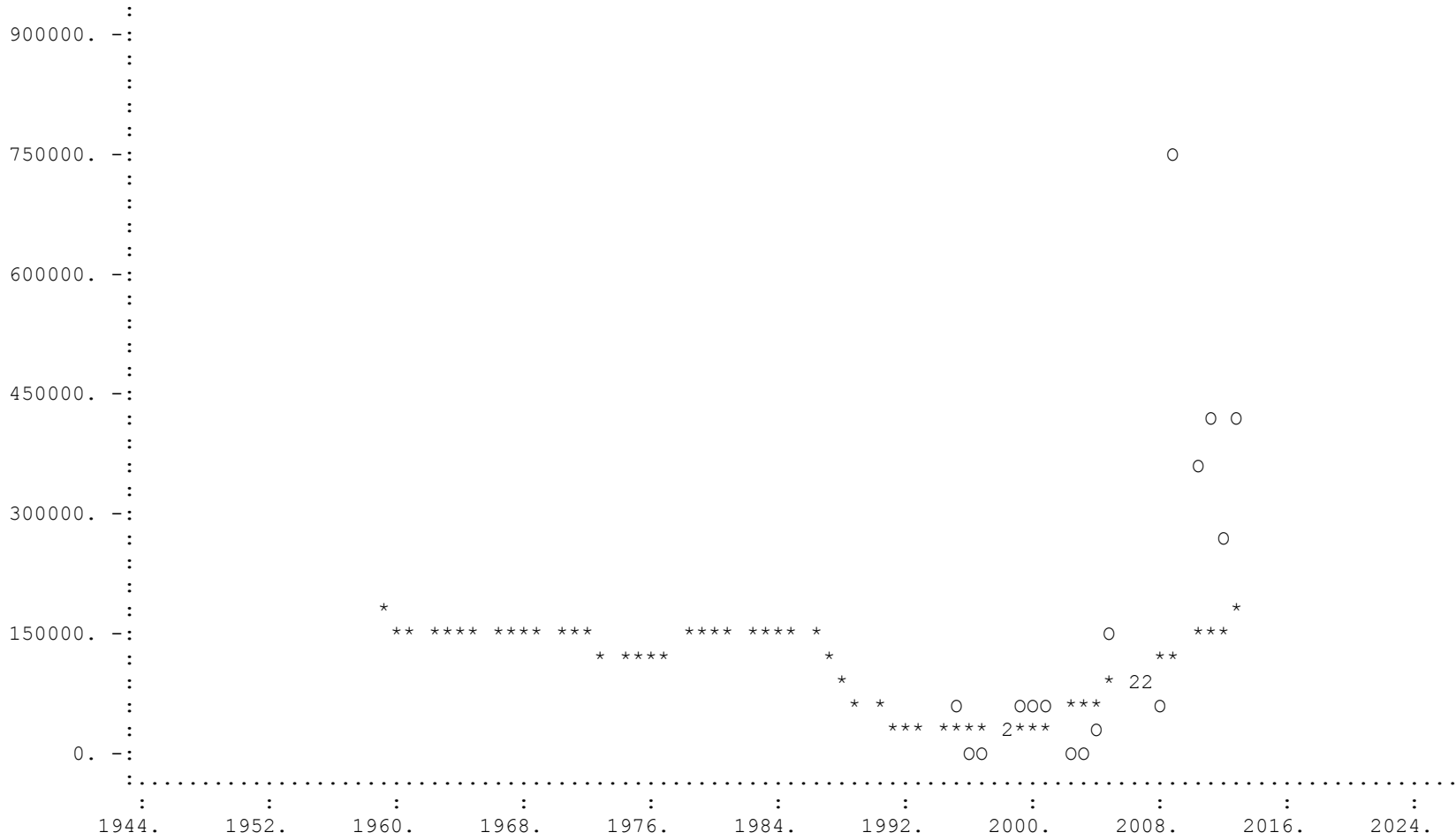
Observed (O) and Estimated (*) CPUE for Data Series # 8 -- 3N spanish survey
