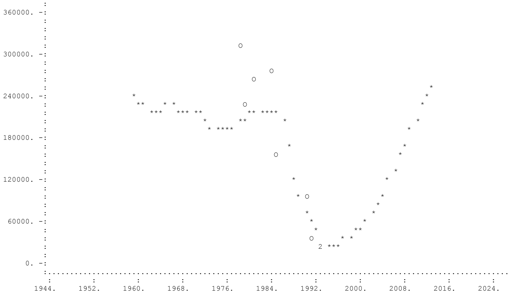
Observed (O) and Estimated (*) CPUE for Data Series # 6 -- 3L summer survey
