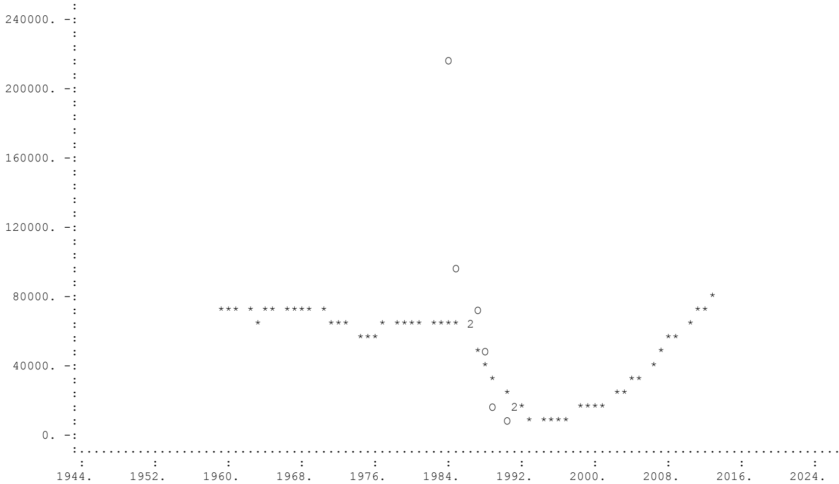
Observed (O) and Estimated (*) CPUE for Data Series # 4 -- 3LN Power russian survey
