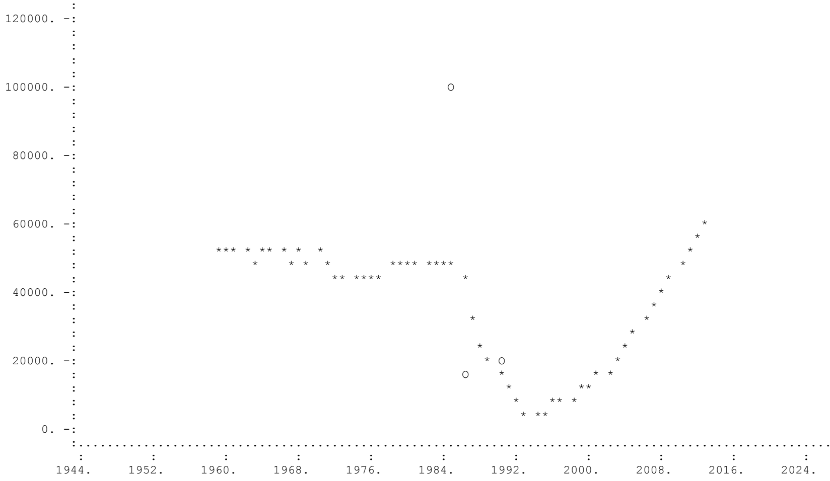
Observed (O) and Estimated (*) CPUE for Data Series # 7 -- 3L autumn survey
