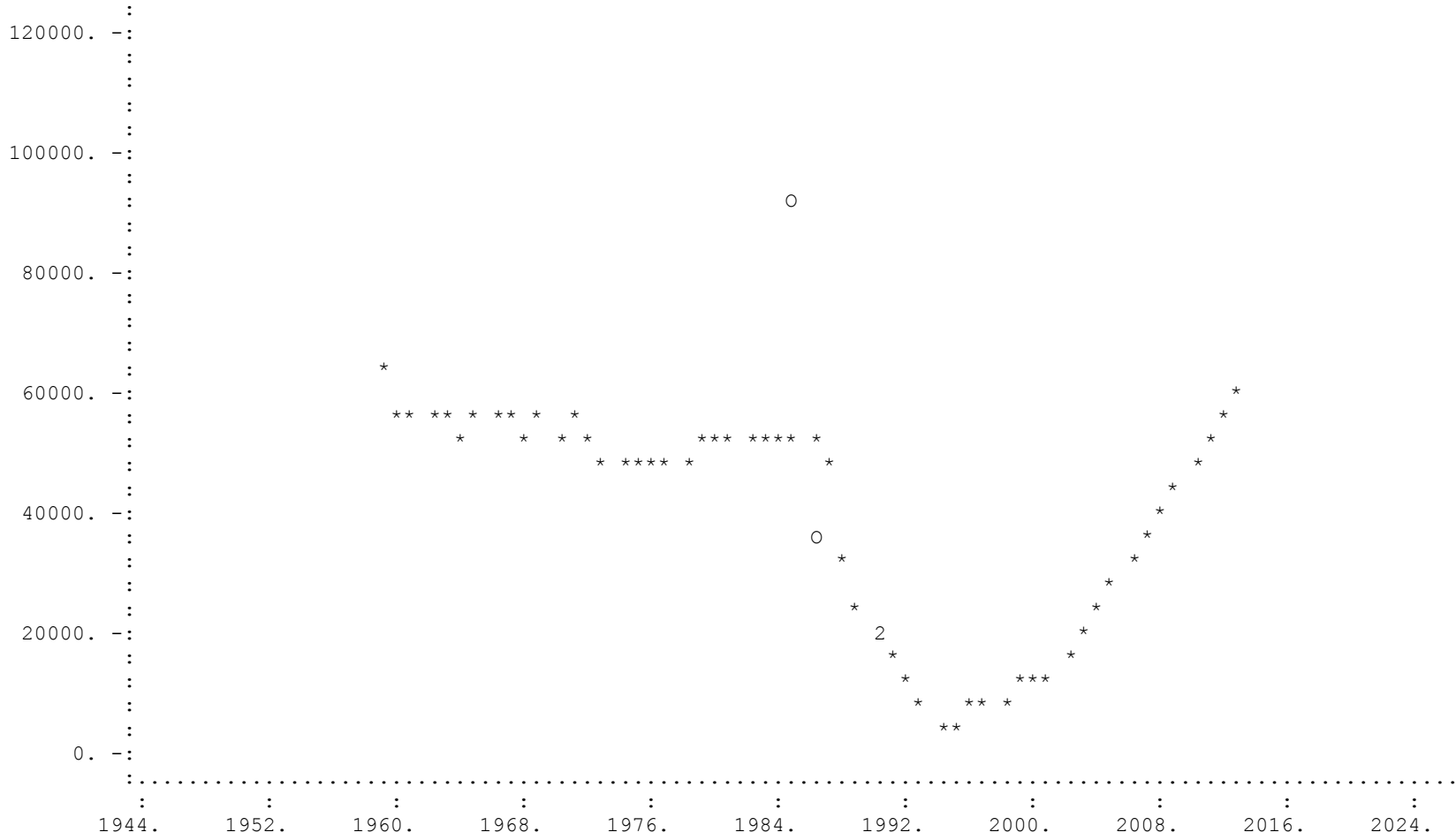
Observed (O) and Estimated (*) CPUE for Data Series # 5 -- 3L winter survey
