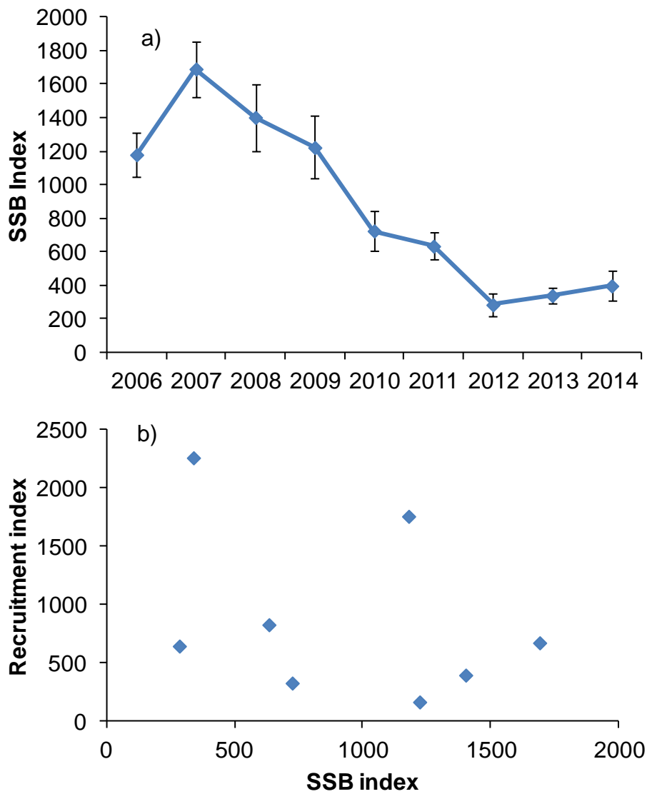
Fig. 13. a) SSB index (abundance in millions) in 2006-2014, and b) SSB-recruitment relationship 2006-2014 in ICES Divs. IIIa and IVa east (Skagerrak and the Norwegian Deep).
