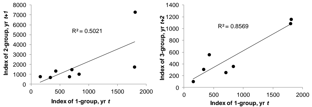
Fig. 2. Correlation between the index of 1-year old shrimp (abundance in millions) in January/February, year t and the index of 2-year old shrimp (abundance in millions) in January/February, year t+1 (left); and correlation between the index of 1-year old shrimp in year t and the index of 3-year old shrimp in year t+2 (right), in ICES Divs. IIIa and IVa east (Skagerrak and the Norwegian Deep). Data from 2006-2014.
