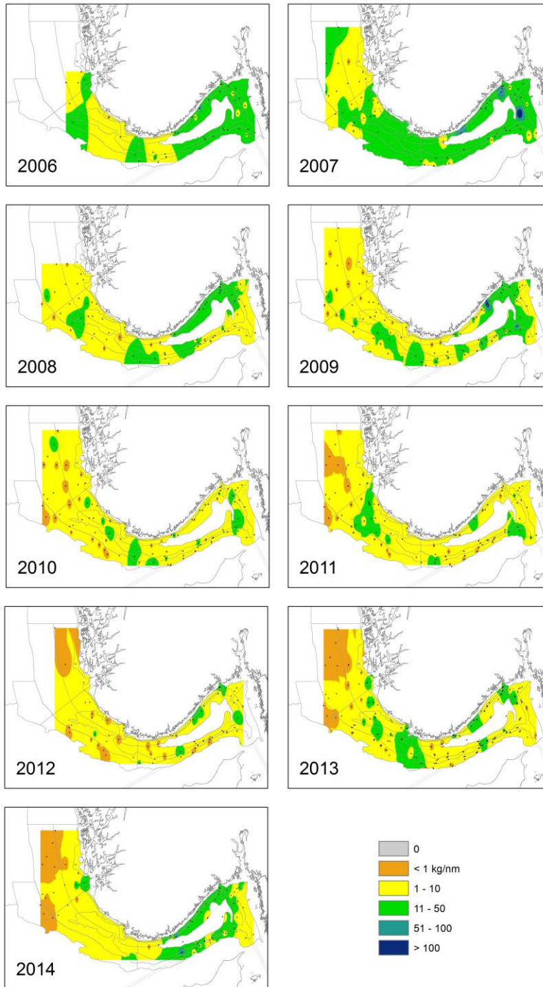
Fig. 7b. The distribution of shrimp biomass (kg/nm) from the Norwegian shrimp survey in ICES Divs. IIIa and IVa east (Skagerrak and the Norwegian Deep) in January/February 2006-2014.
