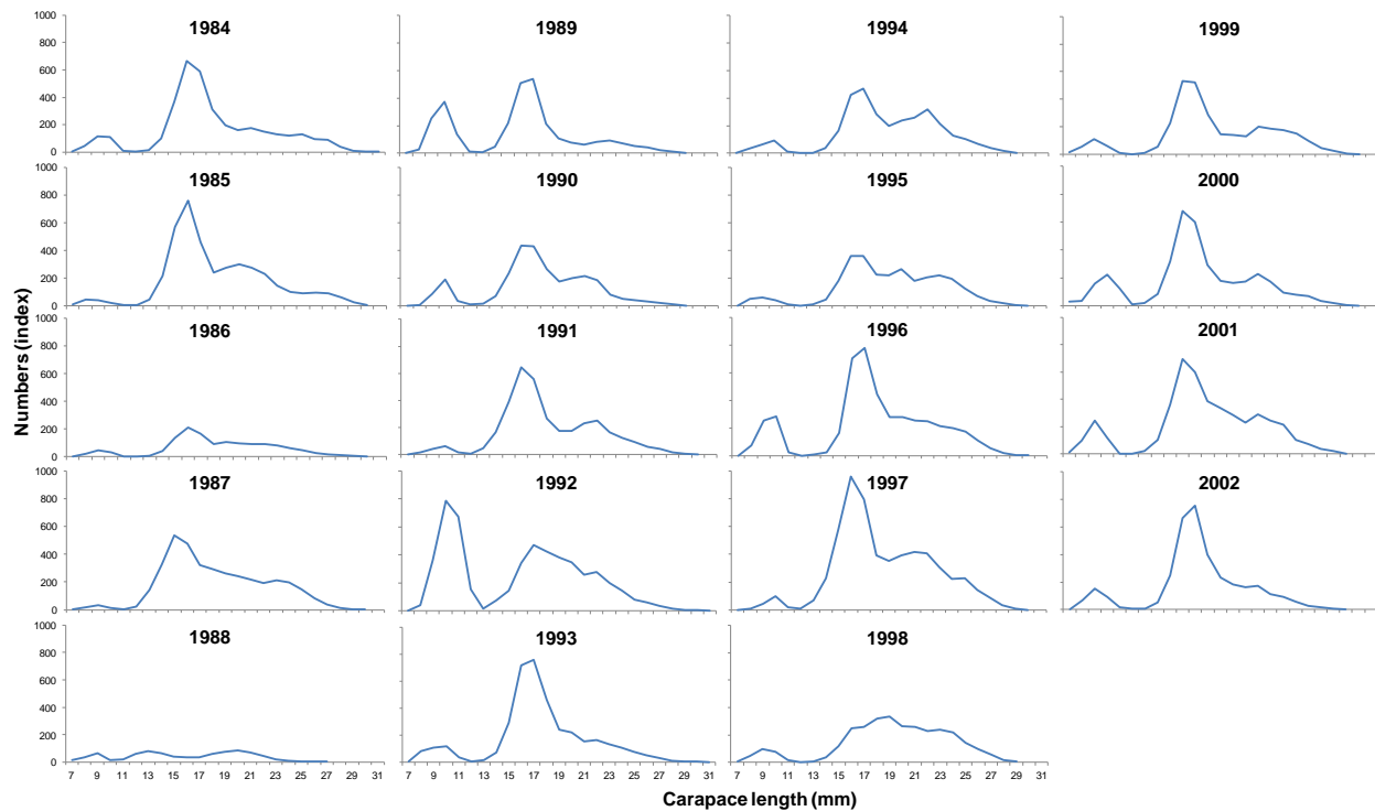
Fig. 11b. Length frequency distributions for the shrimp stock in ICES Divs. IIIa and IVa east (Skagerrak and the Norwegian Deep) in 1984-2002.
