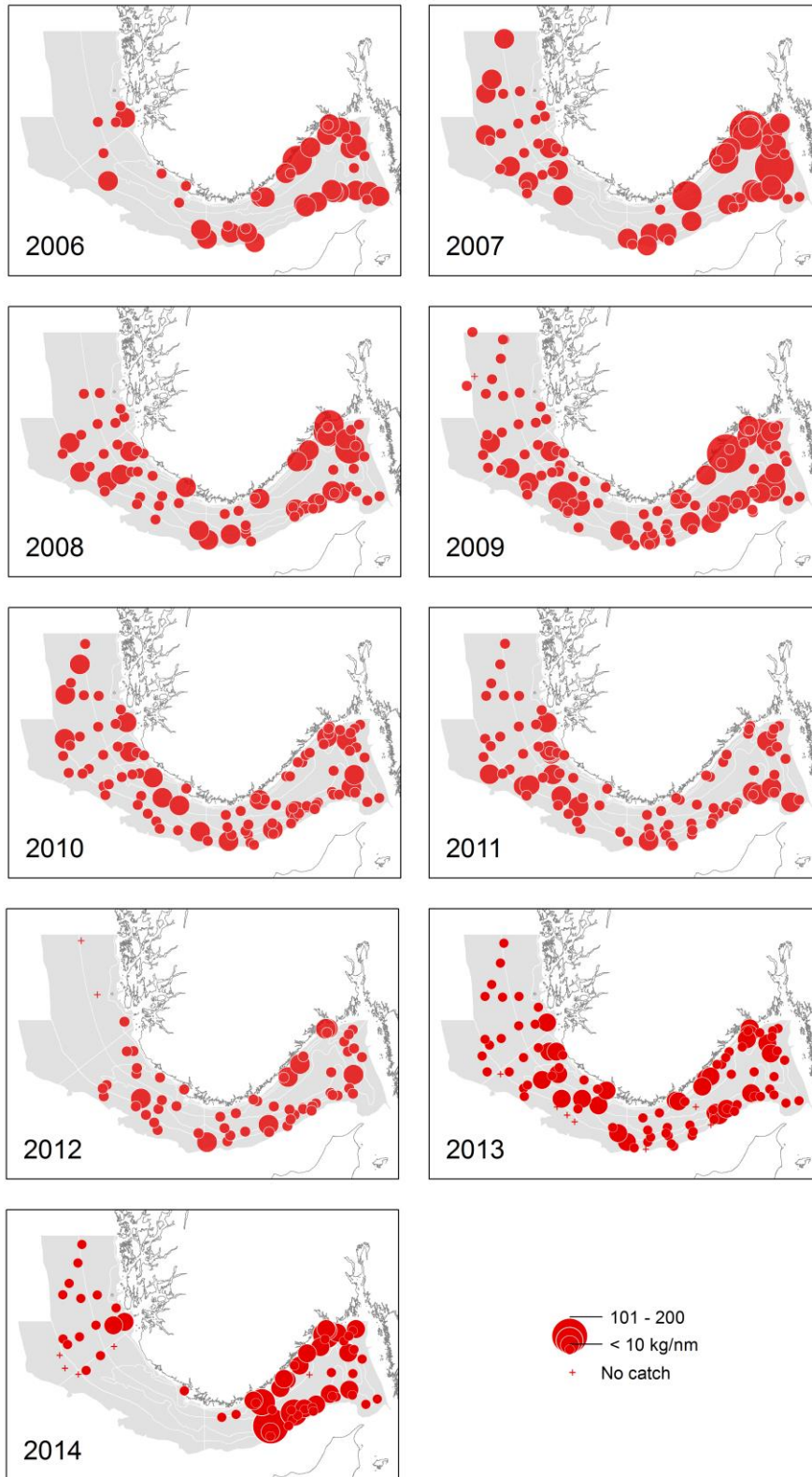
Fig. 7a. Shrimp catches per trawl station (kg/nm) from the Norwegian shrimp survey in ICES Divs. IIIa and IVa east (Skagerrak and the Norwegian Deep) in January/February 2006-2014.
