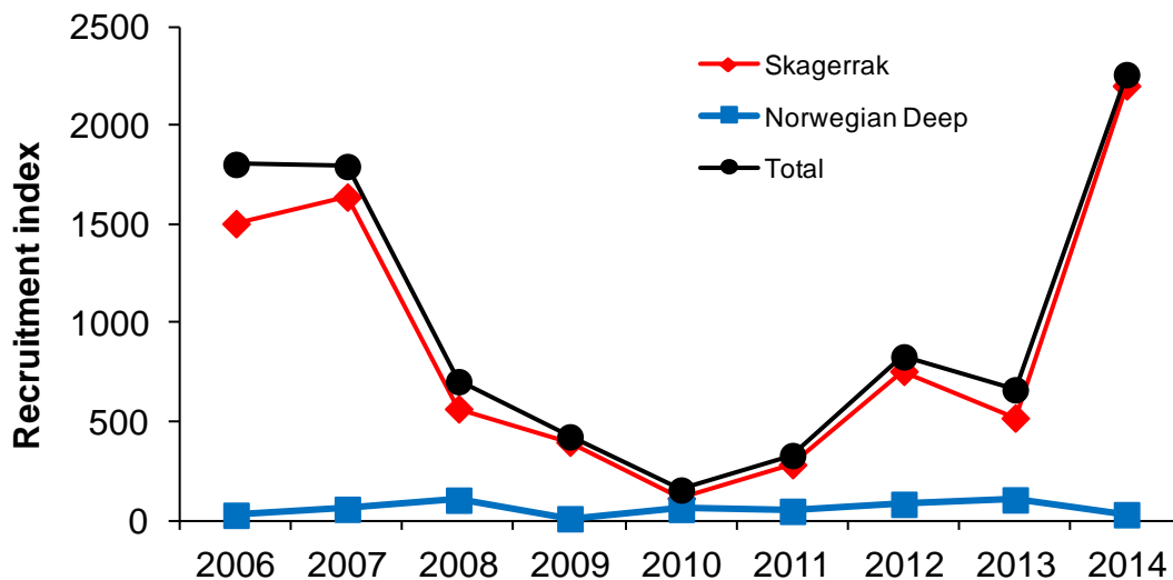
Fig. 12. Recruitment index (abundance in millions) of 1-year old shrimp in ICES Div. IIIa (Skagerrak), Div. IVa east (the Norwegian Deep), and in the overall area for 2006-2014. The higher number of 1-year old shrimp in the whole area in 2006 compared with Skagerrak, despite hardly any 1-year old shrimp in the Norwegian Deep, can be explained the 1-groups in the two areas being slightly skewed. In the total area, shrimps < 15.5 mm are defined as 1-year old by the modal analysis, while the analysis put shrimp > 12 mm in the 2-group in the Norwegian Deep (see Fig. 11a).
