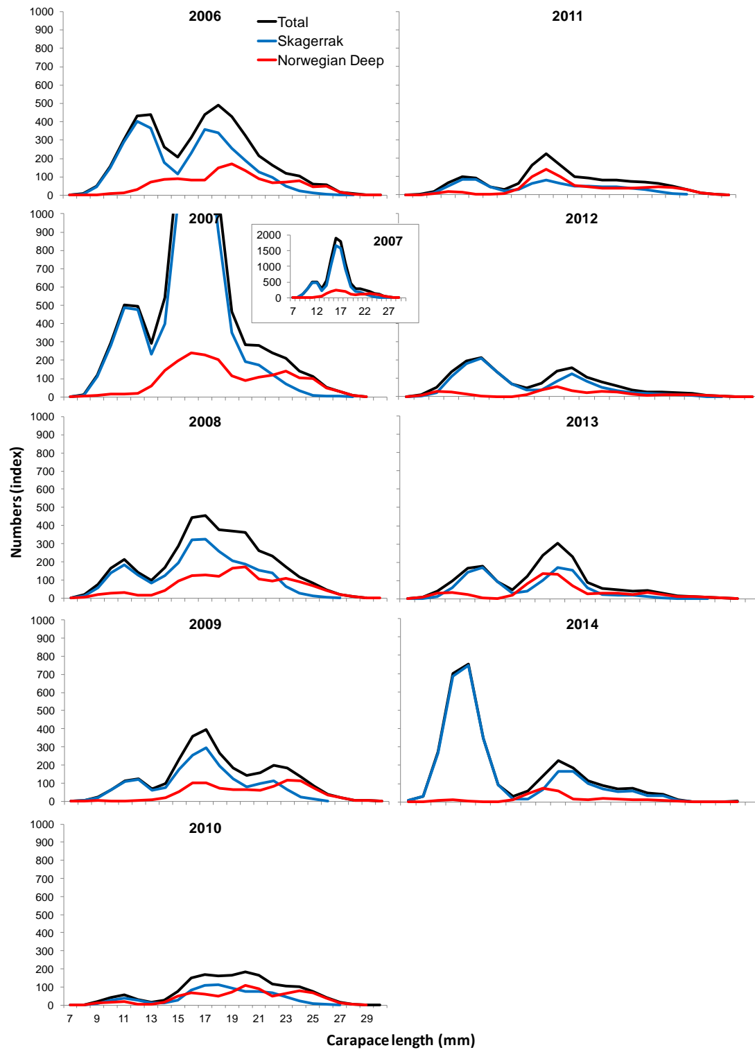
Fig. 11a. Length frequency distributions for the shrimp stock in ICES Divs. IIIa and IVa east (Skagerrak and the Norwegian Deep) by area and total, in 2006-2014.
