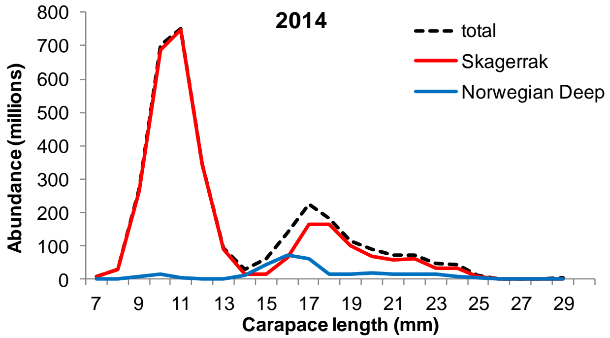
Fig. 10. Length frequency distributions for the shrimp stock in ICES Divs. IIIa and IVa east (Skagerrak and the Norwegian Deep) by area and total, in 2014.
