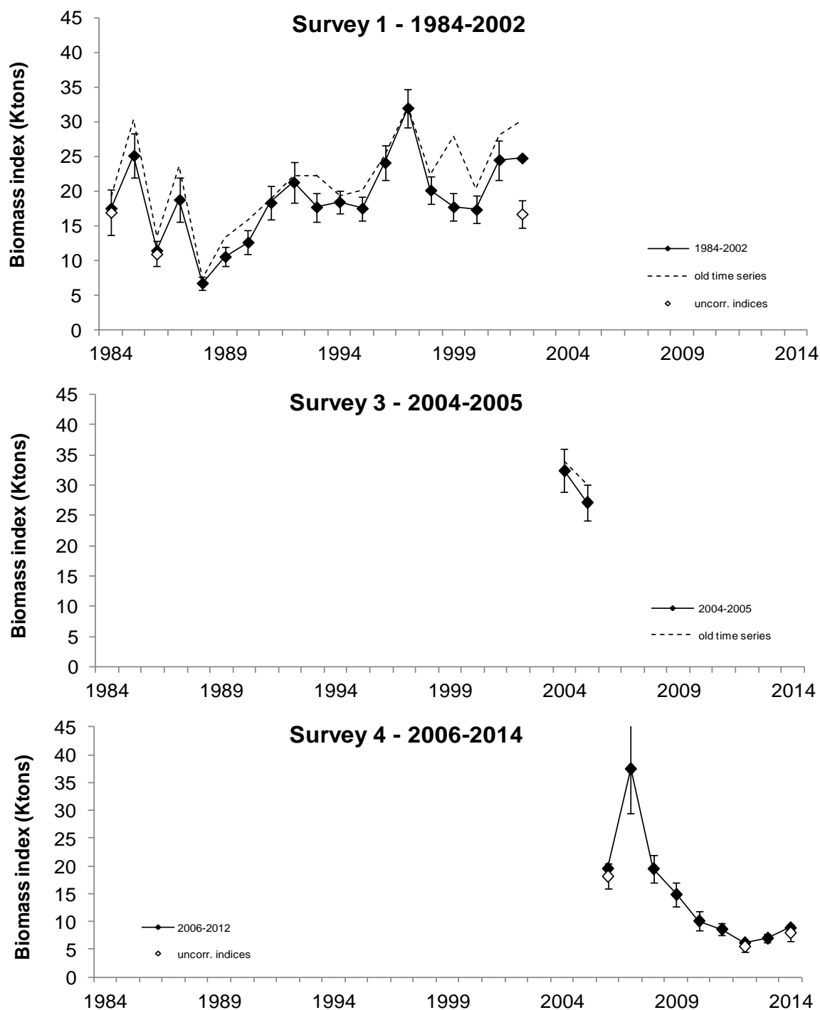
Fig. 6. Estimated total biomass index (with standard error) of shrimp ( Pandalus borealis ) in ICES Divs. IIIa and IVa east (Skagerrak and the Norwegian Deep), 1984-2014. The 2003-value is not shown. The old indices (---) for 1984-2002 and 2004-2005 are plotted together with the recalculated indices (♦). Uncorrected values (◇) due to missing strata (see Table 5) are plotted.
