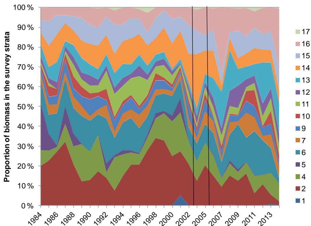
Fig. 9. The proportion of shrimp biomass per stratum from the Norwegian shrimp survey in ICES Divs. IIIa and IVa east (Skagerrak and the Norwegian Deep) in 1984-2014. The vertical lines mark the different survey time series (1984-2002, 2004-2005, 2006-2014). The 2003-value is not shown.
