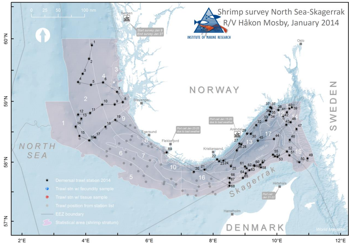
Fig. 4. The Norwegian shrimp survey in ICES Divs. IIIa and IVa east (Skagerrak and the Norwegian Deep) in January 2014 with R/V Håkon Mosby : sailing route and trawled stations.
