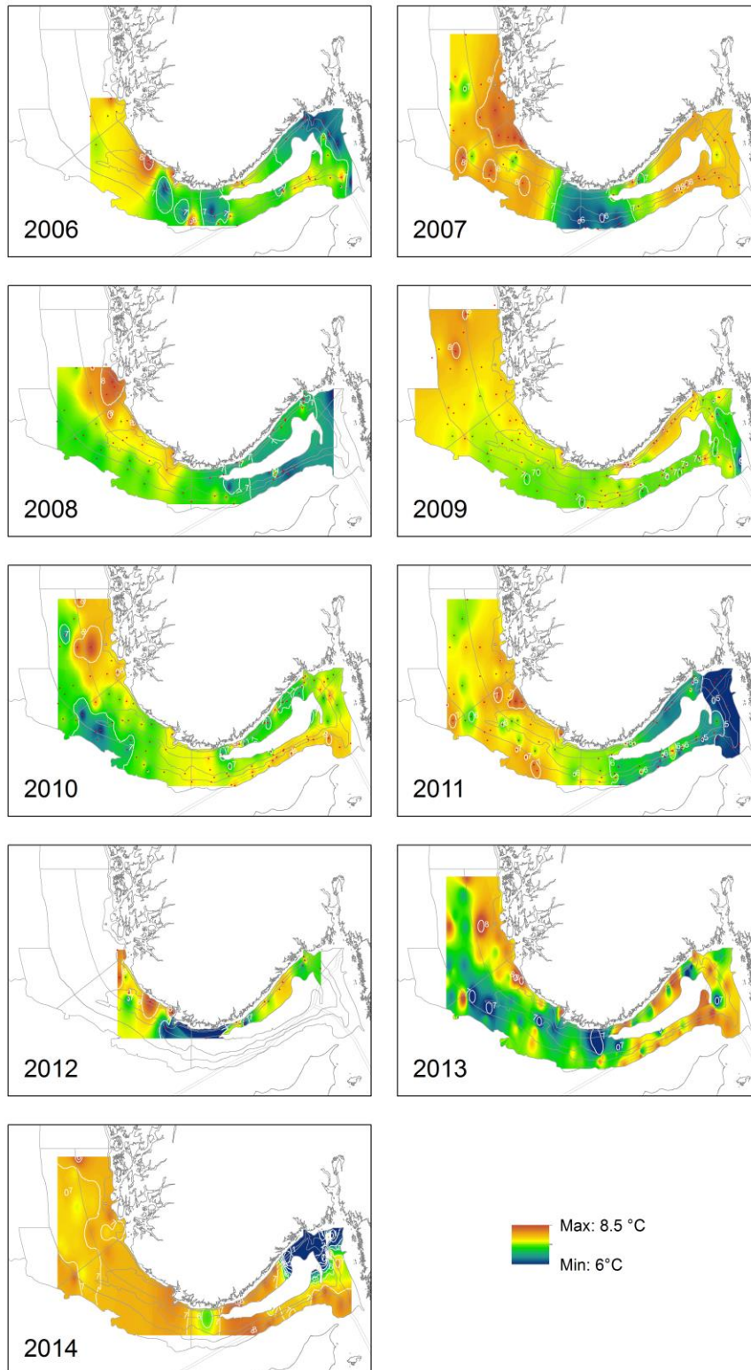
Fig. 5. Bottom temperatures (°C) measured with CTD on fixed trawl stations from the 2006-2014 Norwegian shrimp surveys in ICES Divs. IIIa and IVa east (Skagerrak and the Norwegian Deep).
