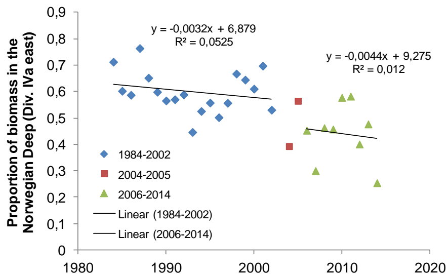
Fig. 8. The proportion of shrimp biomass in the Norwegian Deep from the Norwegian shrimp survey in ICES Divs. IIIa and IVa east (Skagerrak and the Norwegian Deep) in 1984-2014. The 2003-value is not shown.
