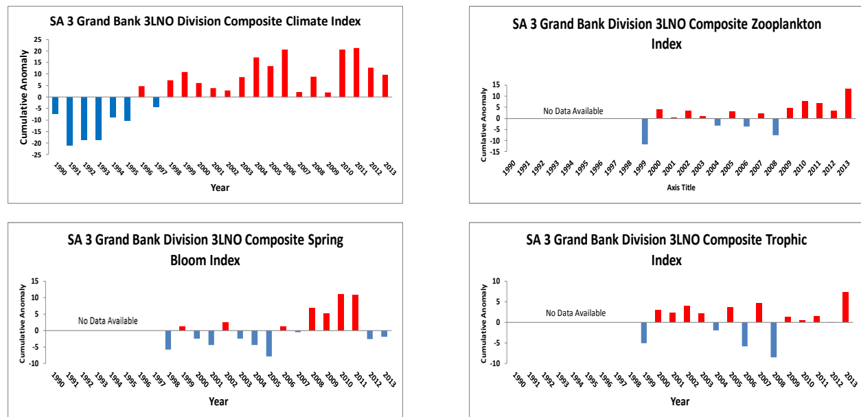
Fig. 3. Composite ocean climate index for NAFO Subarea 3 (SA3 Div. 3LNO) derived by summing the standardized anomalies (top left panel) during 1990-2013, composite spring bloom (summed background chlorophyll a , magnitude and amplitude indices) index (Div. 3LNO) during 1998-2013 (bottom left panel), composite zooplankton (cumulative anomalies of the four functional plankton taxa) index during 1999-2013 (top right panel), and composite trophic (summed anomalies of nutrient and standing stocks of phyto- and zooplankton indices) index (bottom right panel) during 1999-2013. Note the 2012 value for the composite trophic index is near zero and is not readily visible on the plot. Red bars are positive anomalies indicating above average levels while blue bars are negative anomalies indicating below average values.
