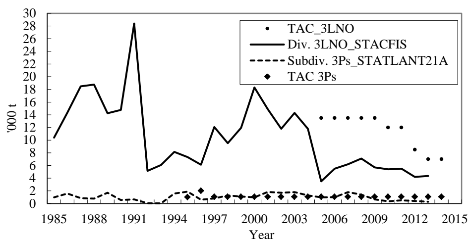
Fig. 16.1. Thorny skate catch in Div. 3LNO and Subdiv. 3Ps and TAC, 1985-20143.
