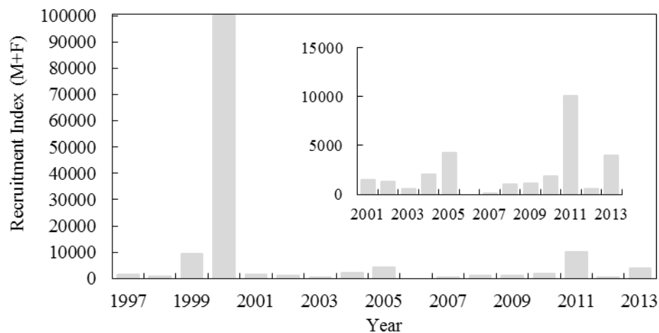
Fig. 17.4 White hake in Div. 3NO and Subdiv. 3Ps: recruitment index (Young of the year male and female=M+F) from Canadian Campelen spring surveys in Div. 3NO and Subdiv. 3Ps during 1997-2013. Estimates from 2006 are not shown, since survey coverage in that year was incomplete. Inset plot depicts 2001-2013 on a smaller scale.
