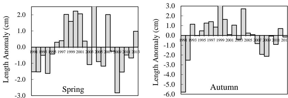
Fig. 10.3. Redfish in Div. 3LN: annual anomalies of the mean length on the spring and autumn survey, 1991-2013.
