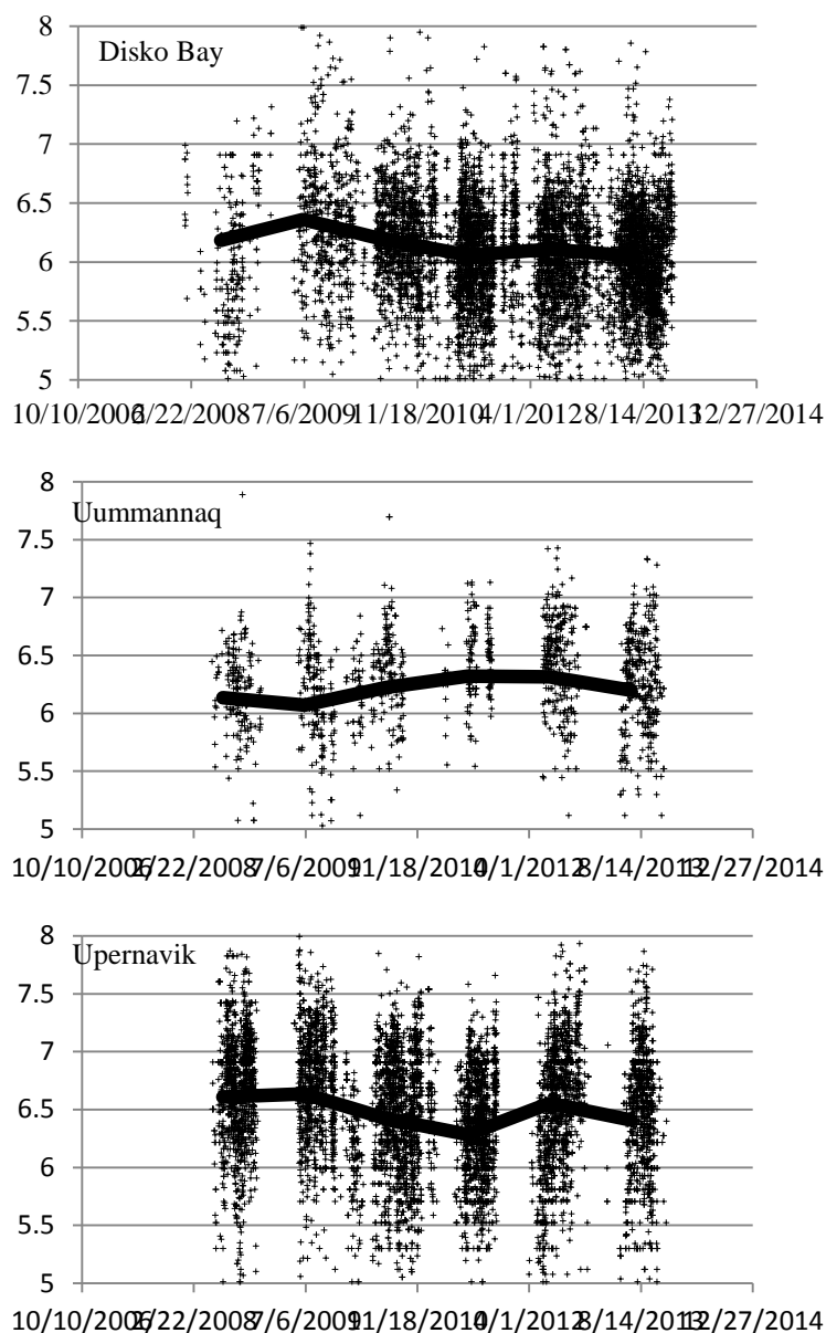
Fig 2.5. Greenland halibut in Division 1A inshore: Standardized longline logbook catch rates. (Points are LogCPUE, line is GLM: \log_{cpue} = \text{overall mean} + \text{yr} + \text{month} + \text{vessel} )
