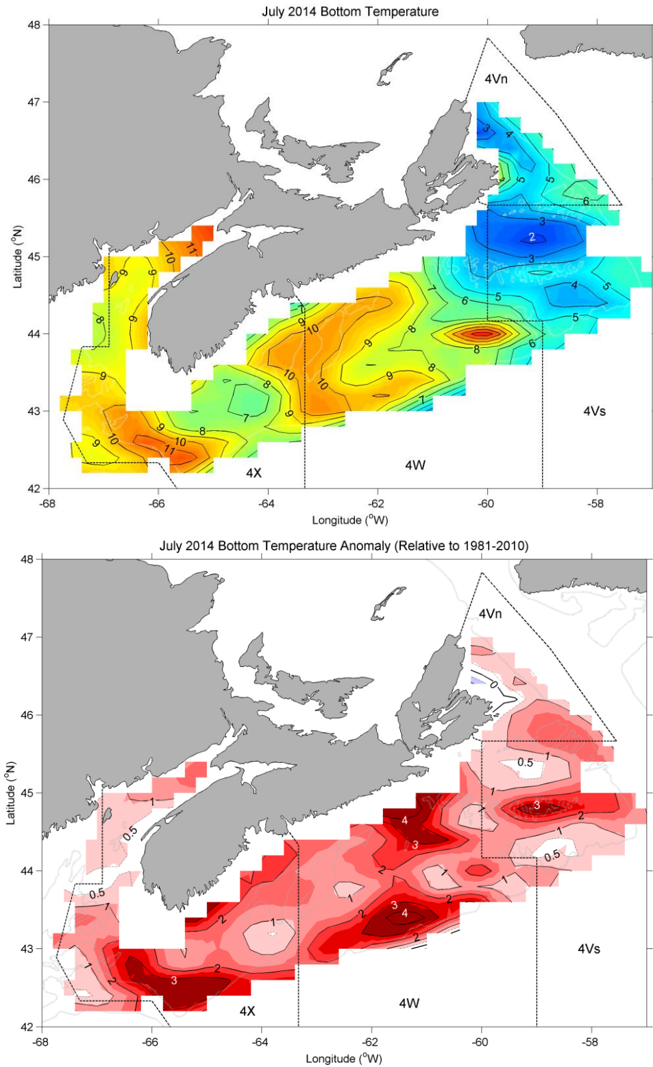
Fig. 11. July bottom temperature (upper panel) and anomaly (lower panel) maps for 2014. NAFO areas 4Vn, 4Vs, 4X and 4W are shown.
