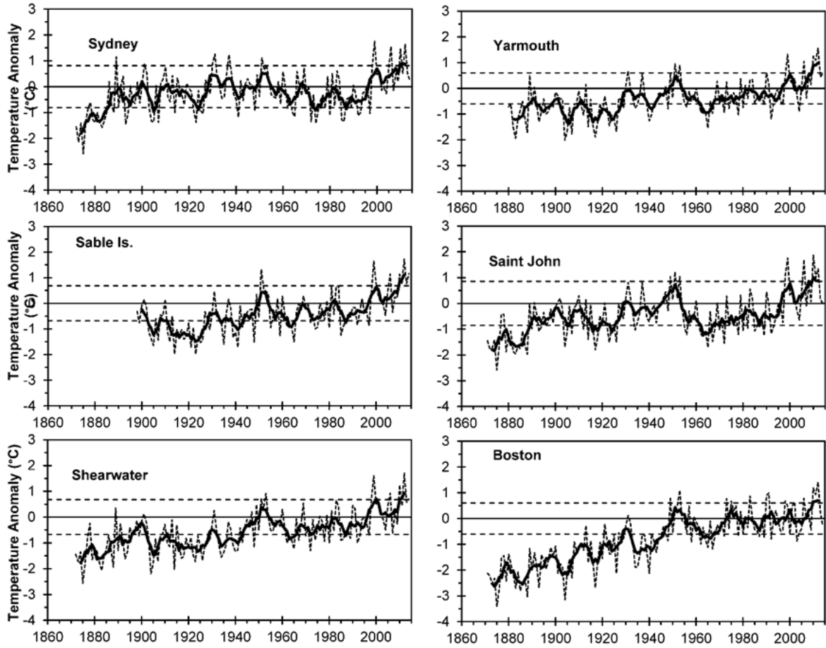
Fig. 2. Annual air temperature anomalies in °C (dashed line) and five year running means (solid line) at selected sites (Sydney, Sable Island, Shearwater, Yarmouth, Saint John and Boston) in Scotian Shelf-Gulf of Maine region (years 1860 to 2014). Horizontal dashed lines represent \pm 1 SD for the 1981-2010 period.
