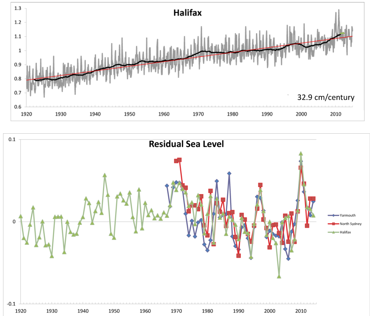
Fig. 14. The time series of the monthly means (gray) and a 5 year running mean (black) of the relative sea level elevations at Halifax, along with the linear trend (red) over 1920-2014 (upper panel). Residual relative sea level (monthly observed values – (1981-2010) linear trend, averaged to annual estimates) for Halifax (green), Yarmouth (blue) and North Sydney (red).
