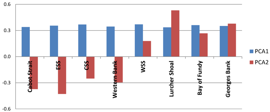
Fig. 7. First (PCA1: 83% of the variance) and second (PCA2: 8% of the variance) loadings from a principal components analysis of the annual mean temperature anomalies (Figure 6, lower panel) for the eight Scotian Shelf and Gulf of Maine regions (Cabot Strait, Eastern Scotian Shelf (EES), Western Bank, Central Scotian Shelf (CSS), Western Scotian Shelf (WSS), Georges Bank, Lurcher Shoals and Bay of Fundy -Figure 6, upper panel).
