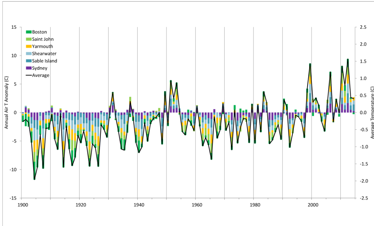
Fig. 3. The contributions of each of the annual temperature anomalies for 6 Scotian Shelf-Gulf of Maine sites (Boston, Saint John, Yarmouth, Shearwater, Sable Island and Sydney) are shown as a stacked bar chart and the average anomaly as a line. Anomalies referenced to 1981-2010.
