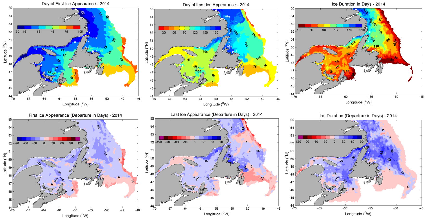
Fig. 4. The time when ice first appeared during 2014 in days from the beginning of the year (left, top panel) and its anomaly from the 1981-2010 mean in days (left, bottom panel). Negative (positive) anomalies indicate earlier (later) than normal appearance. The time when ice was last seen in 2014 in days from the beginning of the year (centre, top panel) and its anomaly from the 1981-2010 mean in days (centre, bottom panel). Positive (negative) anomalies indicate later (earlier) than normal disappearance. The duration of ice in days (right, top panel) during 2014 and the anomalies from the 1981-2010 mean in days (right, bottom panel). Positive (negative) anomalies indicate durations longer (shorter) than the mean.
