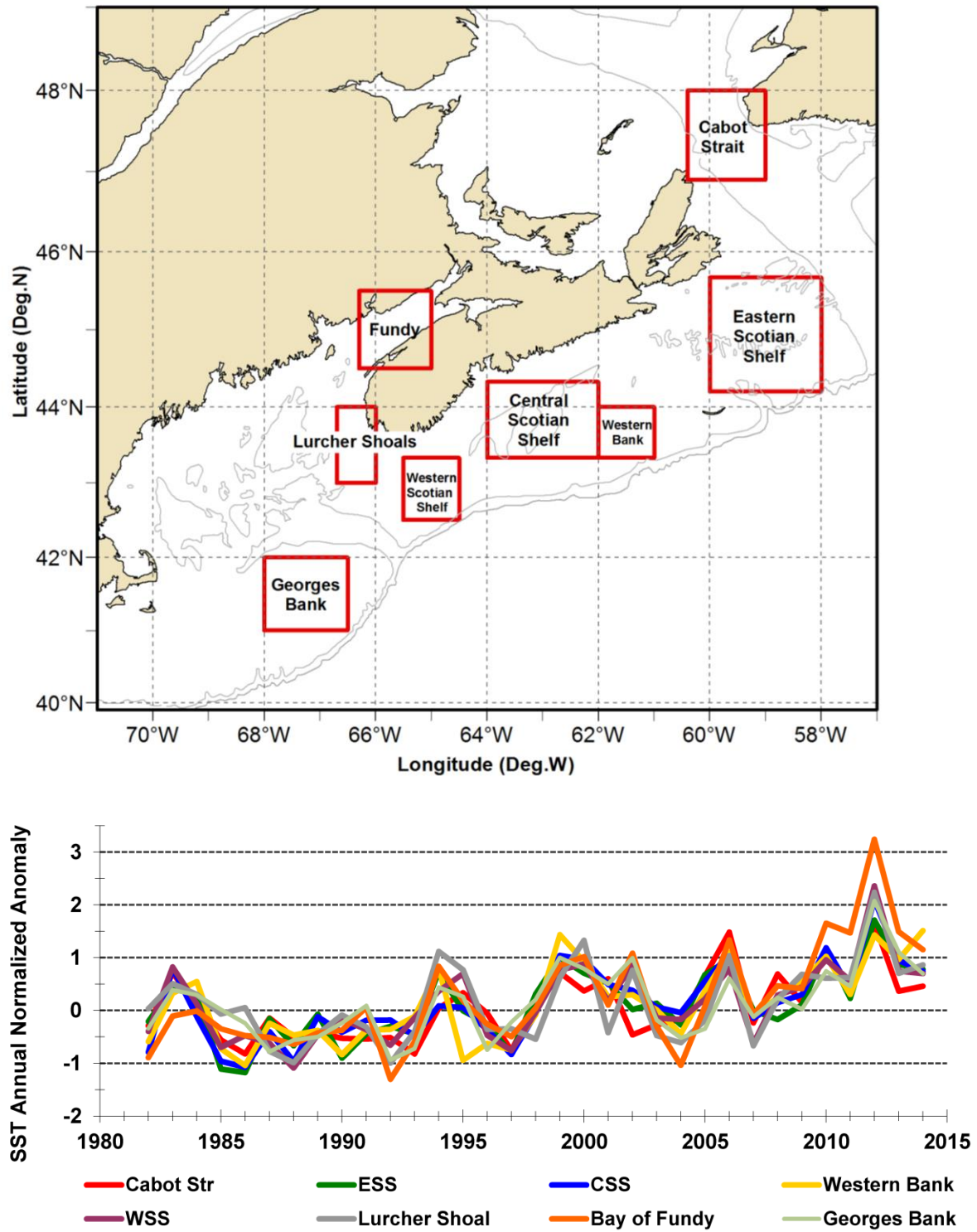
Fig. 6. Scotian Shelf-Gulf of Maine areas (Cabot Strait, Eastern Scotian Shelf (EES), Western Bank, Central Scotian Shelf (CSS), Western Scotian Shelf (WSS), Georges Bank, Lurcher Shoals and Bay of Fundy) used for extraction of sea surface temperature (upper panel). The annual sea surface temperature anomalies derived from satellite imagery compared to their long-term monthly means (lower panel).
