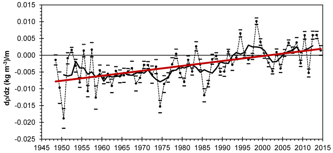
Fig. 13. The mean annual anomaly (dashed line with circles) and 5-yr running mean (heavy solid line) of the stratification index (0-50 m density gradient) averaged over the Scotian Shelf. Standard error estimates for each annual anomaly value are also shown. The linear trend (red line) shows a change in the 0-50 m density difference of 0.31 \text{ kg m}^{-3} over 50 years.
