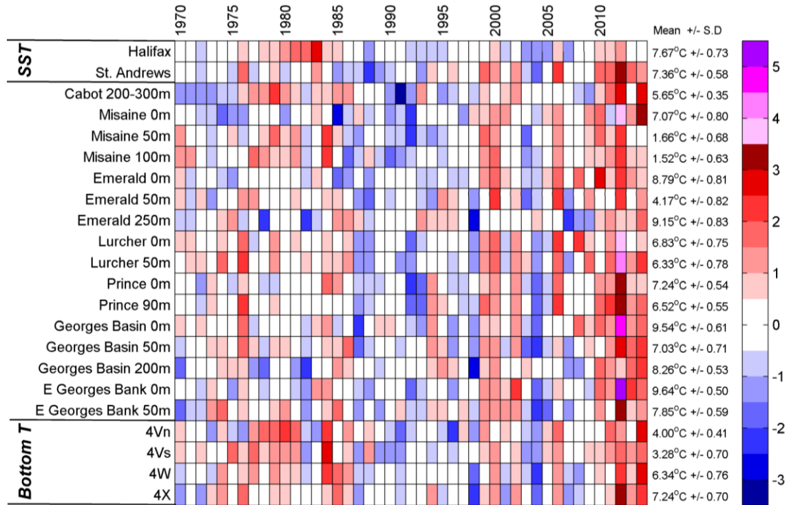
Fig. 15. Normalized annual anomalies of temperatures at the bottom and discrete depths for the Scotian Shelf-Gulf of Maine region. These normalized, annual anomalies are based on the 1981-2010 means, divided by the standard deviation. Blue colours indicates below normal anomalies, red and purple (for 2012, the colour scale had to be increased above +3.5 SD and is shaded in purple) colours above normal anomalies.
