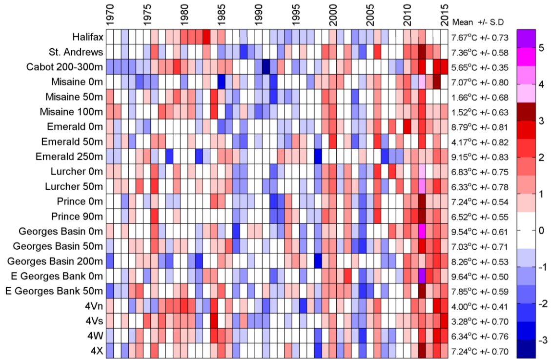
Fig. 14. Normalized annual anomalies of temperatures at the bottom and discrete depths for the Scotian Shelf-Gulf of Maine region. These normalized, annual anomalies are based on the 1981-2010 means, divided by the standard deviation. Blue colours indicates below normal anomalies, red and purple (for 2012, the colour scale had to be increased above +3.5 SD and is shaded in purple) colours above normal anomalies.
