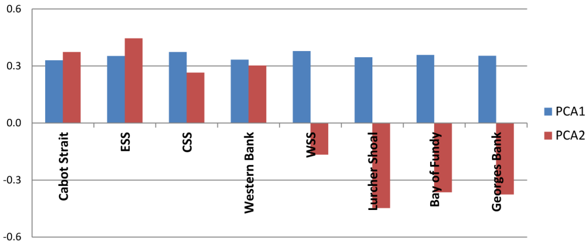
Fig. 7. First (PCA1: 83% of the variance) and second (PCA2: 8% of the variance) loadings from a principal components analysis of the annual mean temperature anomalies (Figure 6, lower panel) for the eight Scotian Shelf and Gulf of Maine regions (Cabot Strait, Eastern Scotian Shelf (EES), Western Bank, Central Scotian Shelf (CSS), Western Scotian Shelf (WSS), Georges Bank, Lurcher Shoals and Bay of Fundy -Figure 6, upper panel).
