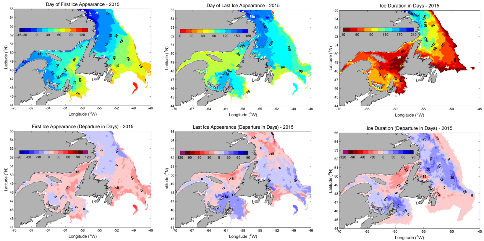
Fig. 4. The time when ice first appeared during 2015 in days from the beginning of the year (left, top panel) and its anomaly from the 1981-2010 mean in days (left, bottom panel). Negative (positive) anomalies indicate earlier (later) than normal appearance. The time when ice was last seen in 2015 in days from the beginning of the year (centre, top panel) and its anomaly from the 1981-2010 mean in days (centre, bottom panel). Positive (negative) anomalies indicate later (earlier) than normal disappearance. The duration of ice in days (right, top panel) during 2015 and the anomalies from the 1981-2010 mean in days (right, bottom panel). Positive (negative) anomalies indicate durations longer (shorter) than the mean.
