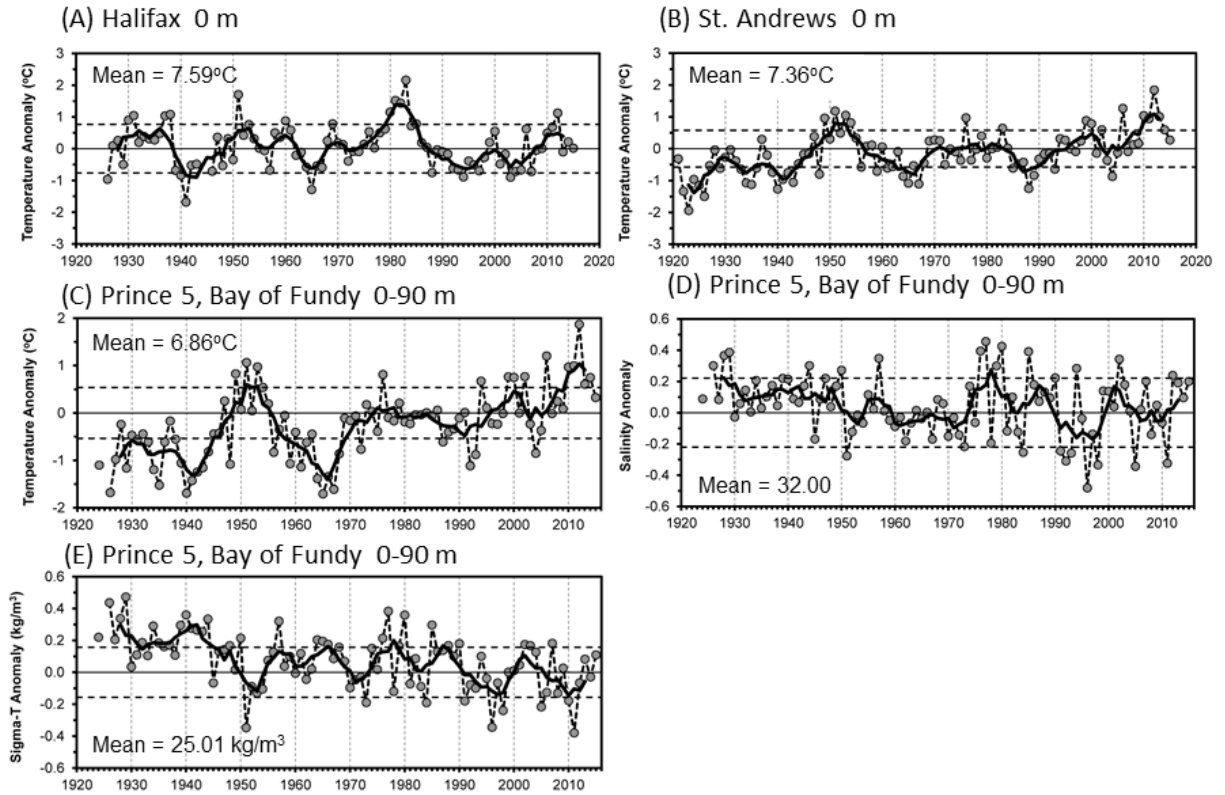
Fig. 8. The annual surface temperature anomalies (dotted line with circles) and their 5-year running means (heavy black line) for (A) Halifax Harbour and (B) St. Andrews; annual depth-averaged (0-90 m) (C) temperature, (D) salinity and (E) density anomalies for the Prince 5 monitoring station at the mouth of the Bay of Fundy. Horizontal dashed lines are mean plus and minus 1 SD.
