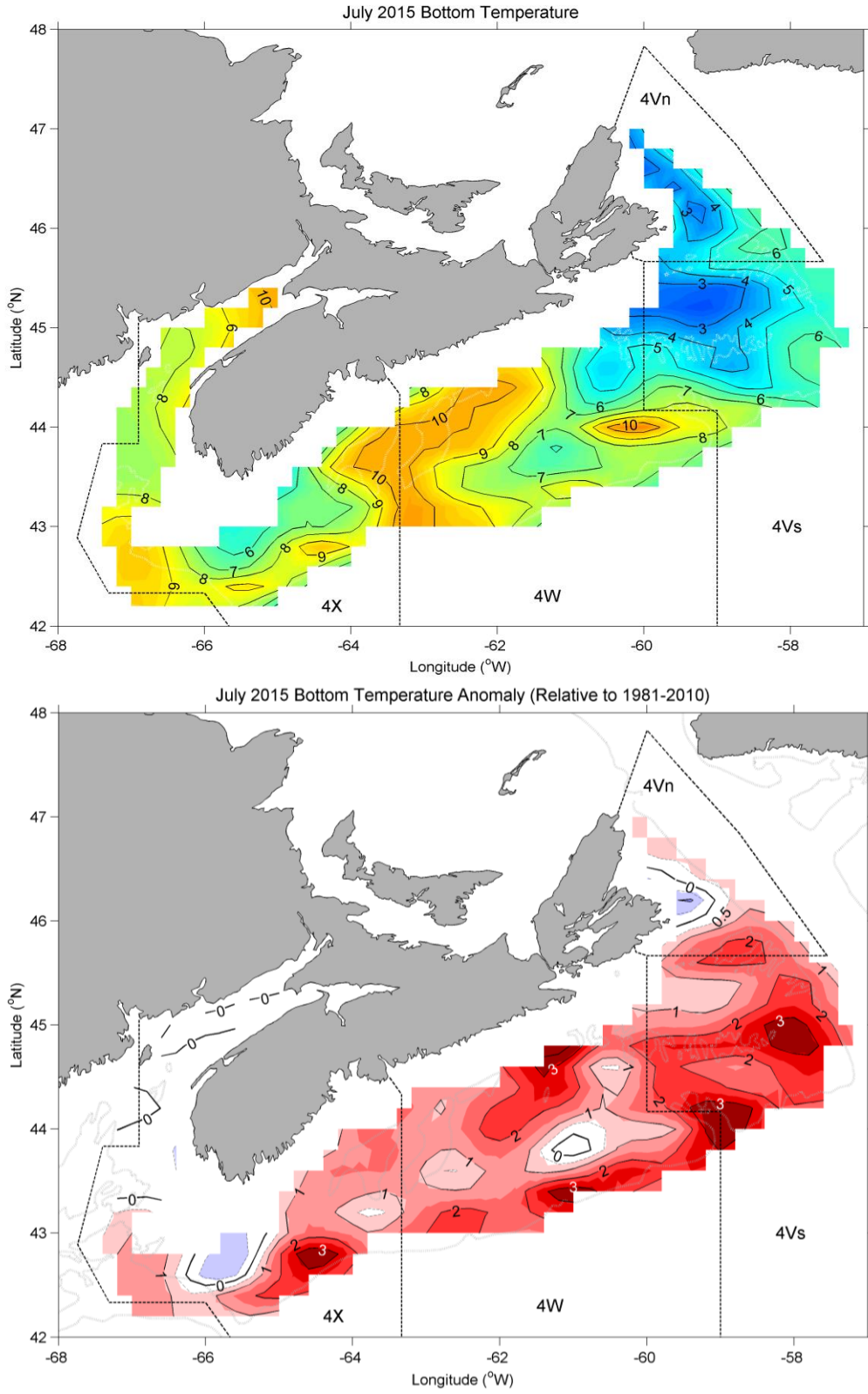
Fig. 11. July bottom temperature (upper panel) and anomaly (lower panel) maps for 2015. NAFO areas 4Vn, 4Vs, 4X and 4W are shown.
