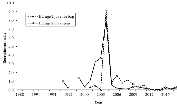
Fig. 5. Recruitment indices, abundances of age 2 in EU Survey from main gear and juvenile bag. Each series was standardized to its mean.
