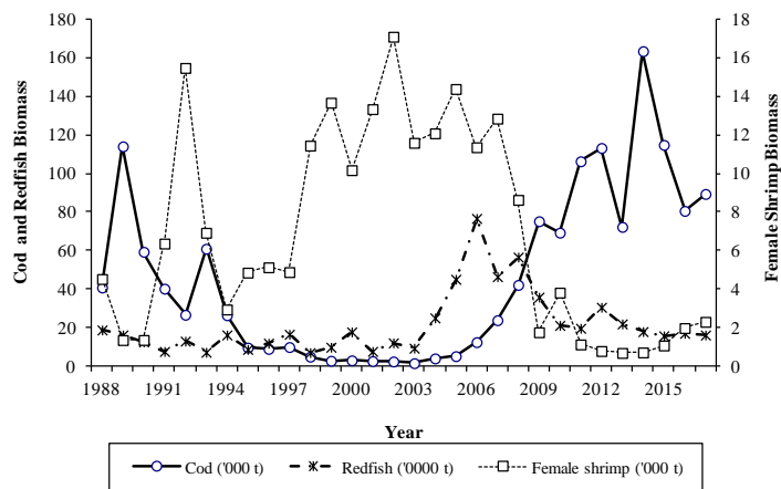
Fig.4. Cod, Redfish and Female shrimp biomass from EU trawl surveys, 1988-2017.
