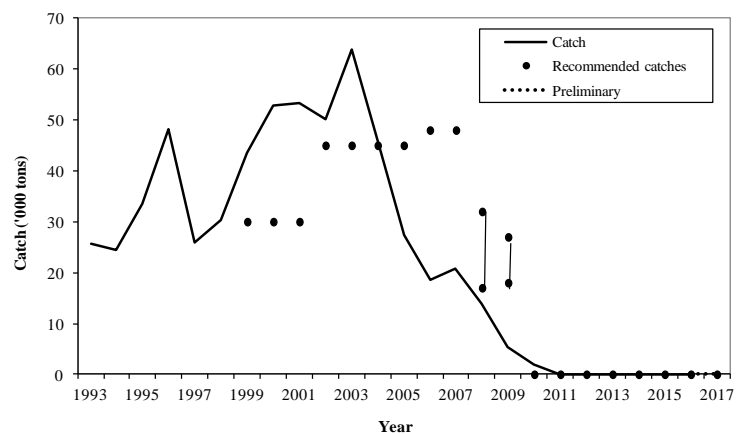
Fig.1. Catches (t) of shrimp on Flemish Cap and catches recommended in the period 1993-2017. Due to a moratorium, the shrimp catch is expected to be zero in 2017.
