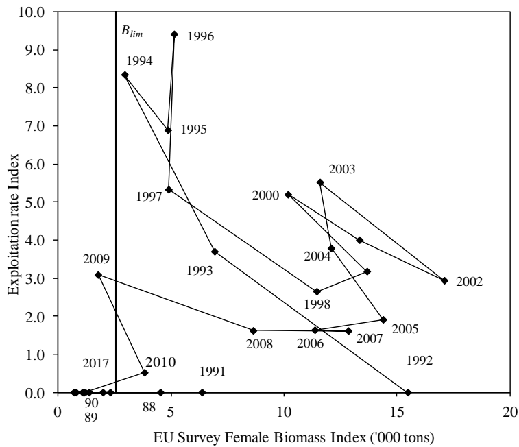
Fig. 6. Exploitation rate index plotted against female biomass index from EU survey. Line denoting B_{lim} is drawn where biomass is 15% of the maximum point in 2002. Due to the moratorium on shrimp fishing the expected catch in 2017 is 0 t.
