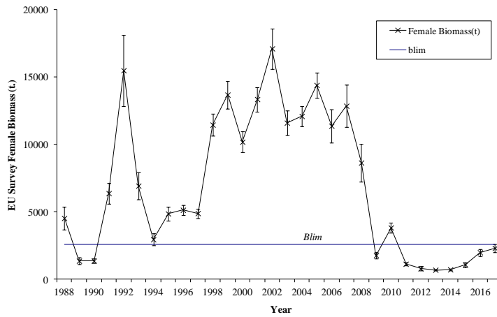
Fig. 3. Female biomass index from EU surveys, 1988-2017.
