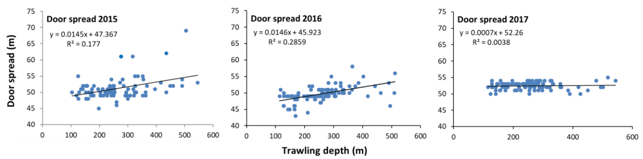
Fig. 6. Door spread (m) by trawling depth (m) for all valid trawl stations on the 2015-2017 Norwegian shrimp surveys in ICES Divs. IIIa and IVa east (Skagerrak and the Norwegian Deep).
