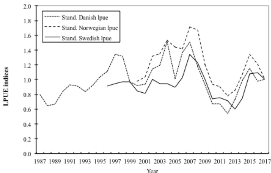
Fig. 5.3. Northern shrimp in Skagerrak and Norwegian Deep: Danish, Norwegian and Swedish standardized lpue until 2017. Each series is standardized to its final year.
