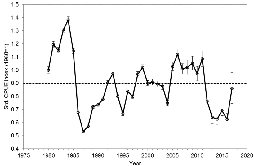
Fig. 6.6. Shrimp in ICES SA 1 and 2: Standardized CPUE based on Norwegian data. Error bars represent 1 SE; dotted line is the mean of the series.
