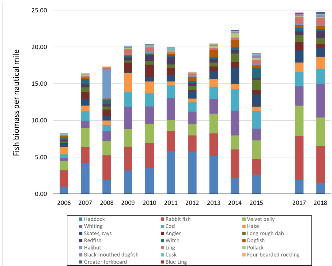
Fig. 5.2. Northern shrimp in Skagerrak and Norwegian Deep: Estimated indices of predator biomass (catch in kg per towed nautical mile) from the Norwegian shrimp survey in 2006–2018 excluding saithe, roundnose grenadier and blue whiting. The 2016 survey data have been omitted (see text for details).
