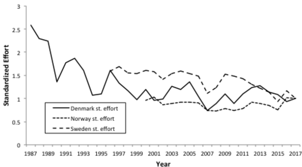
Fig. 5.4. Northern shrimp in Skagerrak and Norwegian Deep: Estimated standardized effort. Each series is standardized to its final year.
