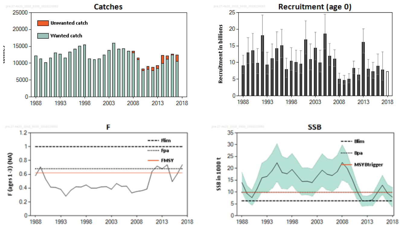
Fig.5.8. Northern shrimp in Skagerrak and Norwegian Deep: Summary assessment output. Total catch, including estimated discards since 2008 (tonnes) and F, SSB and R assessment results. SSB and R are depicted with 90% confidence intervals. The assumed recruitment value (geometric mean of the last ten years) for 2018 is unshaded.
