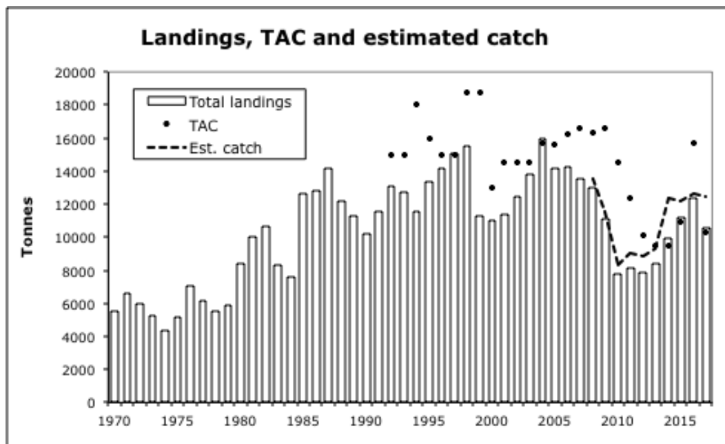
Fig. 5.1. Northern shrimp in Skagerrak and Norwegian Deep: TAC, total landings by all fleets, and total estimated catch including estimated Swedish discards for 2008–2017, and Norwegian and Danish discards for 2009–2017.
