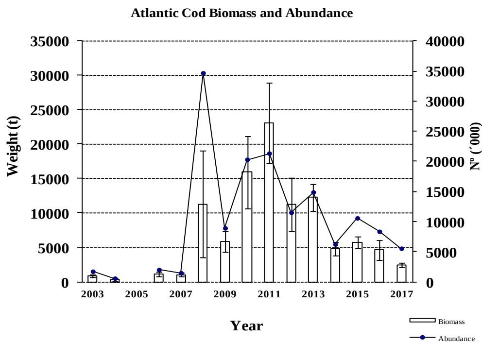
FIG. 2. Atlantic cod abundance ('000), biomass in tonnes and \pm SD by year. Spanish surveys in NAFO Division 3L: 2003 - 2017 (R/V “ Vizconde de Eza ”). In 2003, the data correspond to 69% of the total area prospected in 2006-2017.
