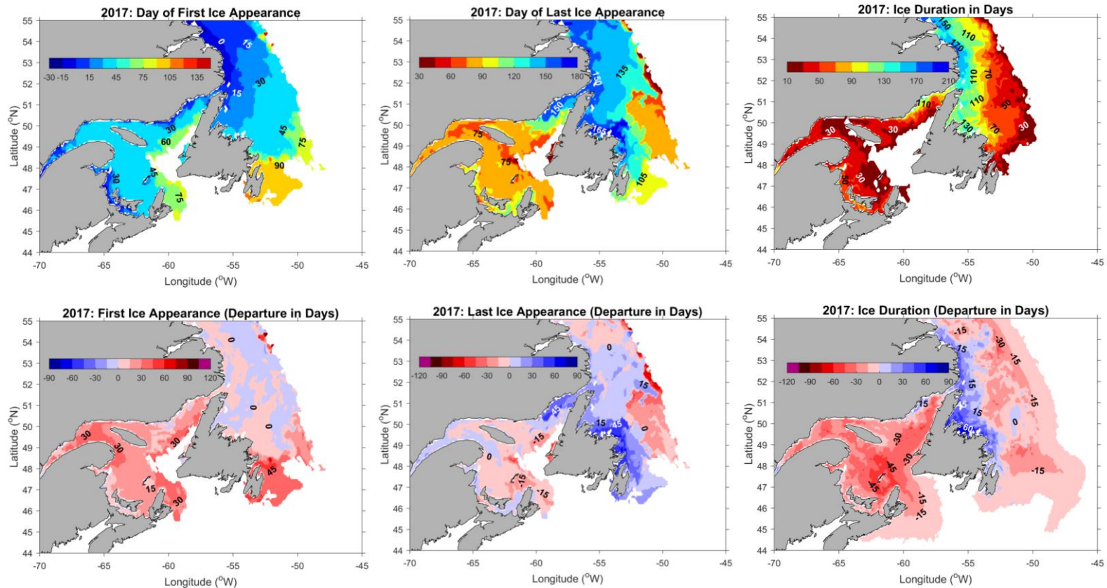
Fig. 4. The time when ice first appeared during 2017 in days from the beginning of the year (left, top panel) and its anomaly from the 1981-2010 mean in days (left, bottom panel). Negative (positive) anomalies indicate earlier (later) than normal appearance. The time when ice was last seen in 2017 in days from the beginning of the year (centre, top panel) and its anomaly from the 1981-2010 mean in days (centre, bottom panel). Positive (negative) anomalies indicate later (earlier) than normal disappearance. The duration of ice in days (right, top panel) during 2017 and the anomalies from the 1981-2010 mean in days (right, bottom panel). Positive (negative) anomalies indicate durations longer (shorter) than the mean.
