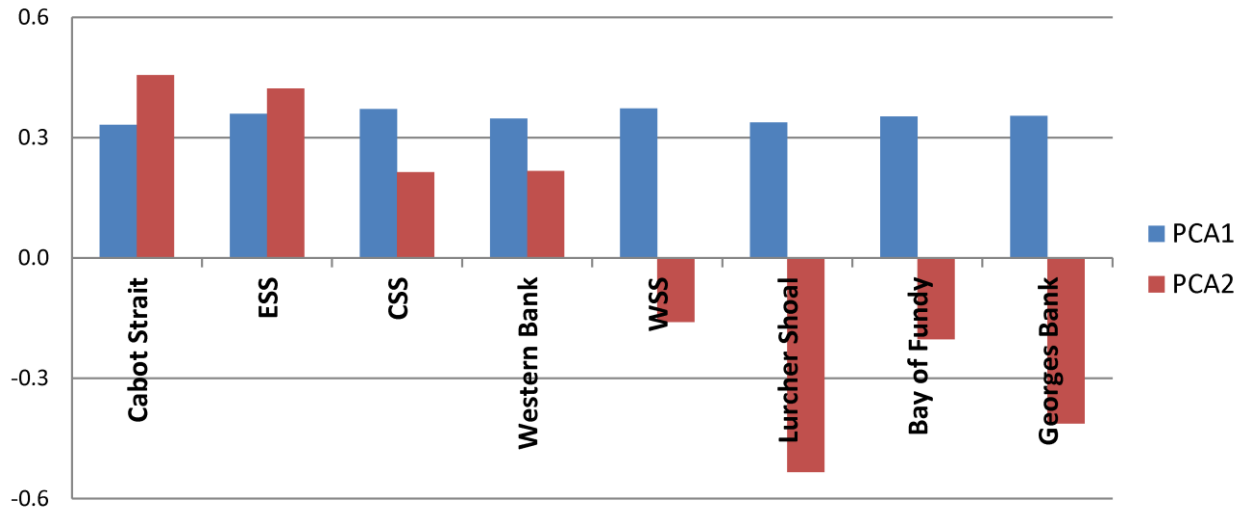
Fig. 7. First (PCA1: 83% of the variance) and second (PCA2: 6% of the variance) loadings from a principal components analysis of the annual mean temperature anomalies (Figure 6, lower panel) for the eight Scotian Shelf and Gulf of Maine regions (Cabot Strait, Eastern Scotian Shelf (EES), Western Bank, Central Scotian Shelf (CSS), Western Scotian Shelf (WSS), Georges Bank, Lurcher Shoals and Bay of Fundy -Figure 6, upper panel).
