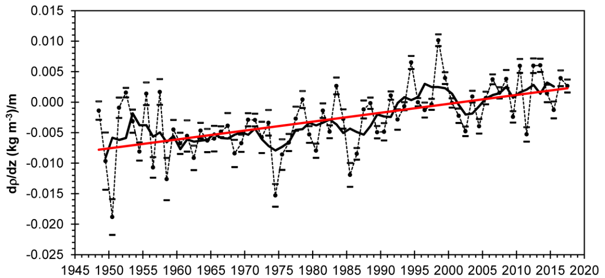
Fig. 13. The mean annual anomaly (dashed line with circles) and 5-yr running mean (heavy solid line) of the stratification index (0-50 m density gradient) averaged over the Scotian Shelf. Standard error estimates for each annual anomaly value are also shown. The linear trend (red line) shows a change in the 0-50 m density difference of 0.36 \text{ kg m}^{-3} over 50 years.
