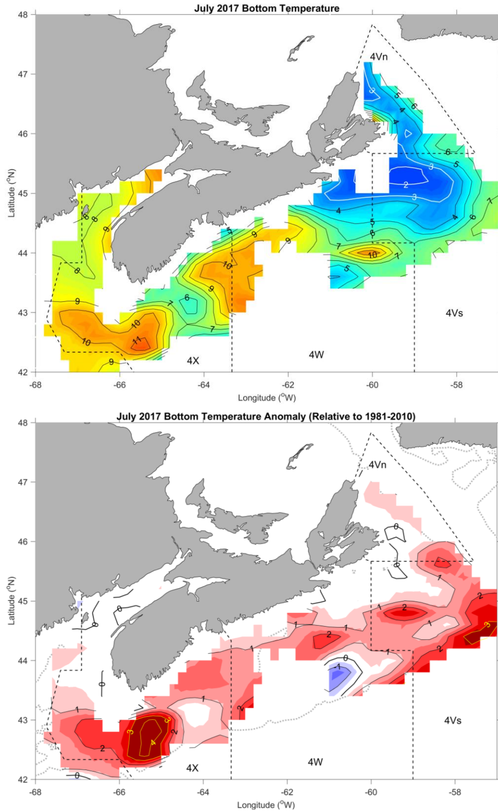
Fig. 11. July bottom temperature (upper panel) and anomaly (lower panel) maps for 2017. NAFO areas 4Vn, 4Vs, 4X and 4W are shown.
