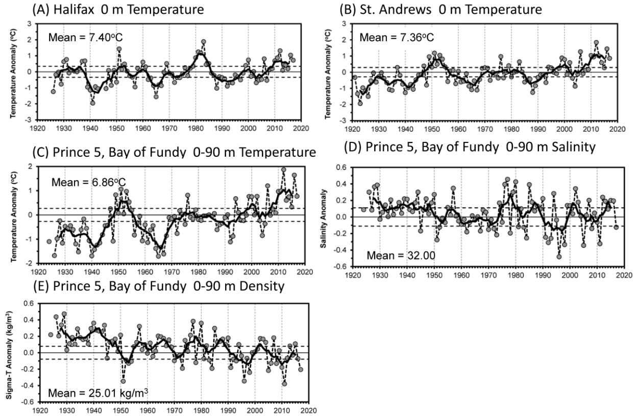
Fig. 8. The annual surface temperature anomalies (dotted line with circles) and their 5-year running means (heavy black line) for (A) Halifax Harbour and (B) St. Andrews; annual depth-averaged (0-90 m) (C) temperature, (D) salinity and (E) density anomalies for the Prince 5 monitoring station at the mouth of the Bay of Fundy. Horizontal dashed lines are mean plus and minus 0.5 SD.
