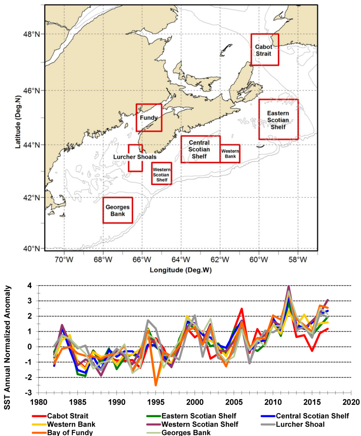
Fig. 6. Scotian Shelf-Gulf of Maine areas (Cabot Strait, Eastern Scotian Shelf (EES), Western Bank, Central Scotian Shelf (CSS), Western Scotian Shelf (WSS), Georges Bank, Lurcher Shoals and Bay of Fundy) used for extraction of sea surface temperature (upper panel). The annual sea surface temperature anomalies derived from satellite imagery compared to their long-term monthly means (lower panel).
