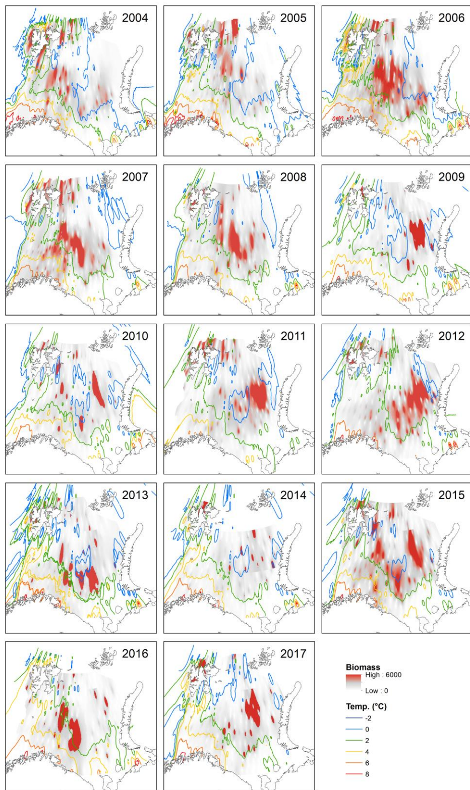
Fig. 13. Bottom temperature contour overlaid shrimp density distributions (see Fig. 7) from ecosystem surveys since 2004.
