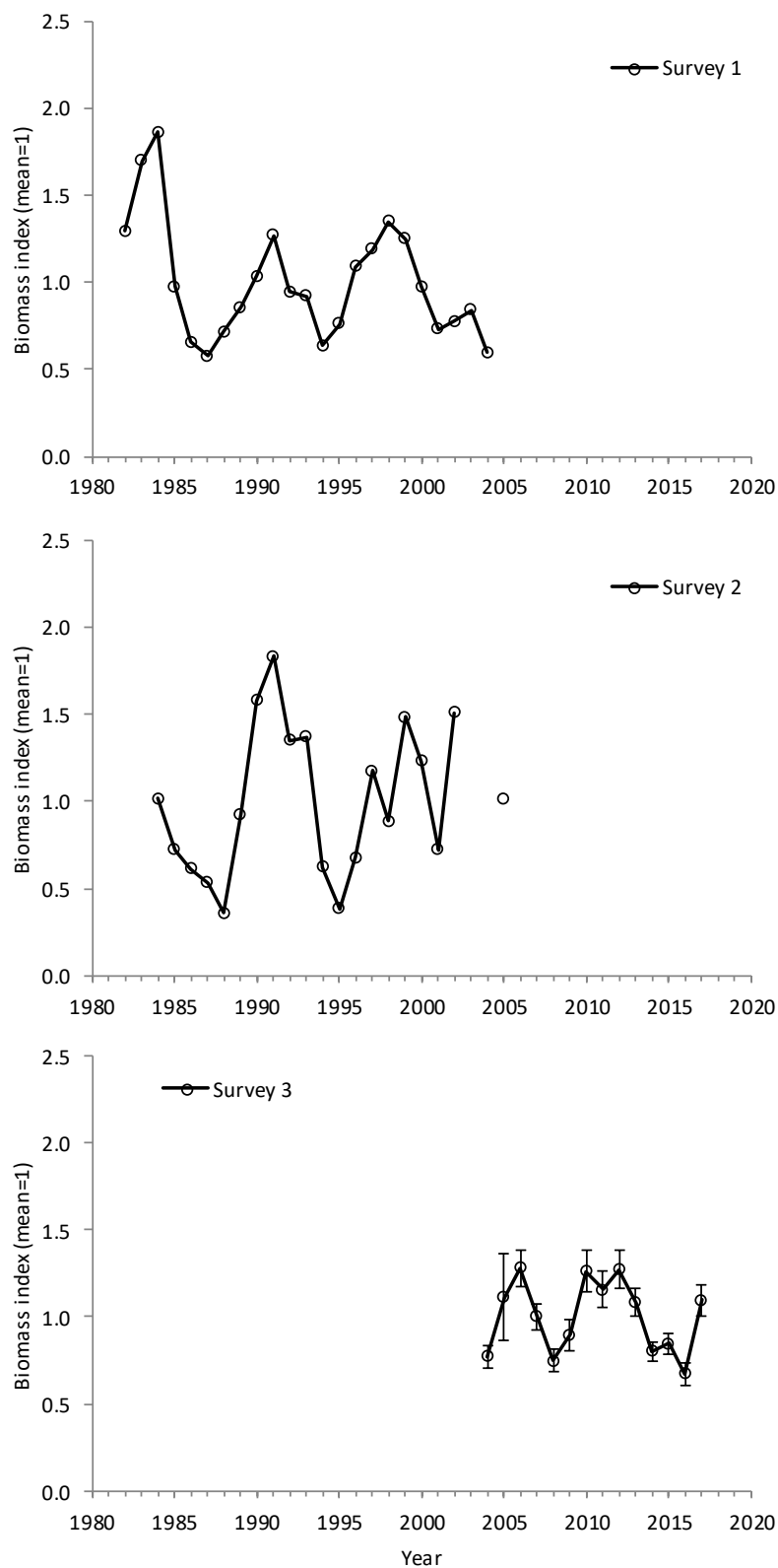
Fig. 5. Indices of annual mean biomass from survey 1: The Norwegian shrimp survey 1982-2004; survey 2: The Russian shrimp survey 1984-2002 and 2005; and survey 3: The joint Norwegian-Russian ecosystem survey since 2004.
