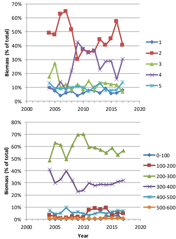
Fig. 7. Percentage of total biomass. Upper: by main strata (see fig 3). Bottom: by depth strata.
