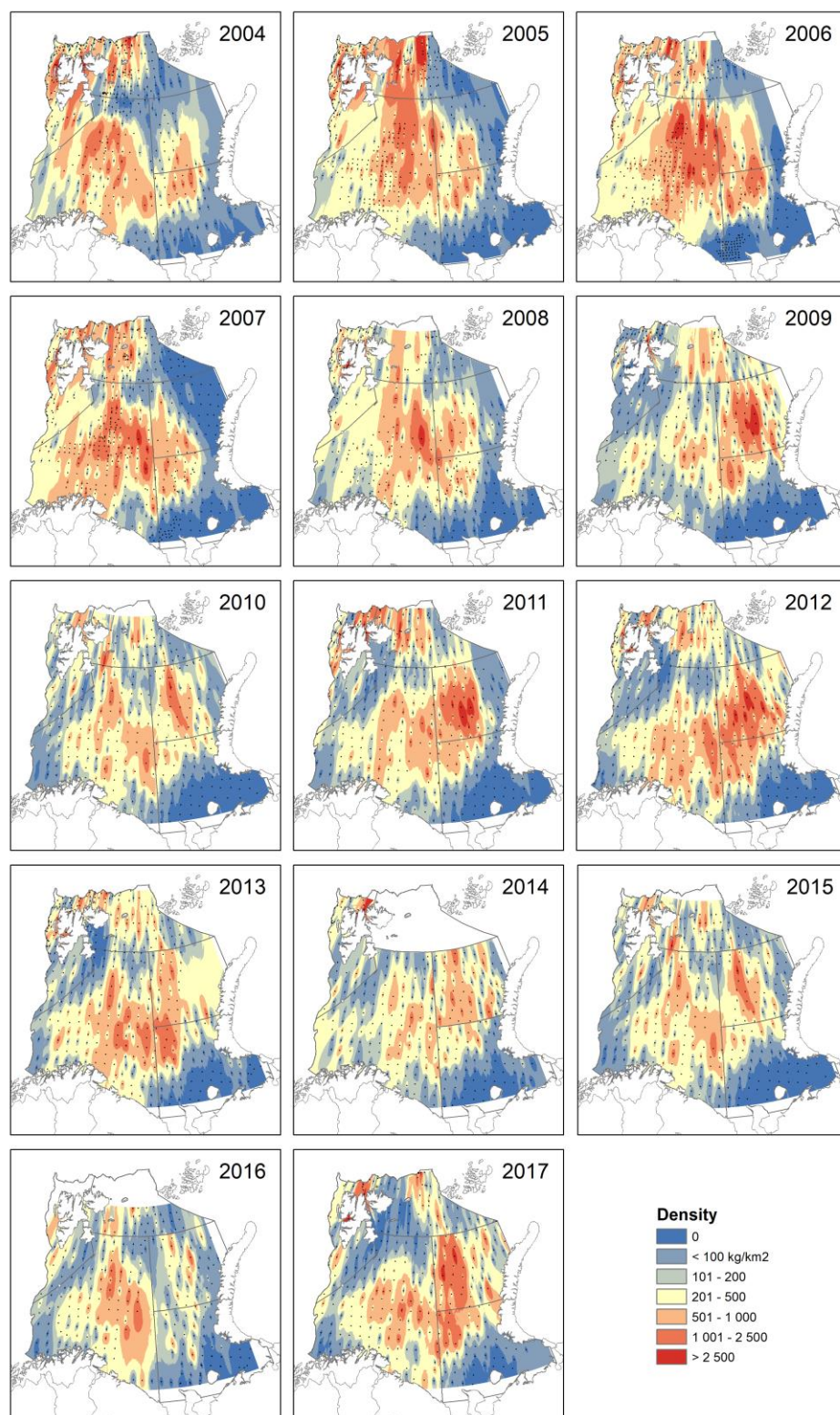
Fig. 10. Shrimp density by year from inverse distance weighted interpolation (e.g. Fisher et al. , 1987) between trawl stations (black dots) (Europe Albers Equal Area Conic projection).
