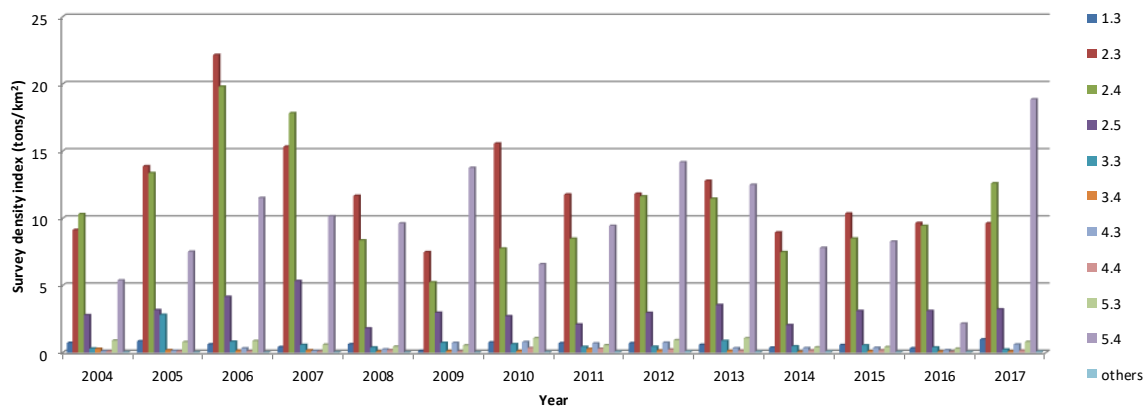
Fig. 8. Estimated mean biomass density by year and strata (code: see Table 1 and Fig. 3 for definition)
