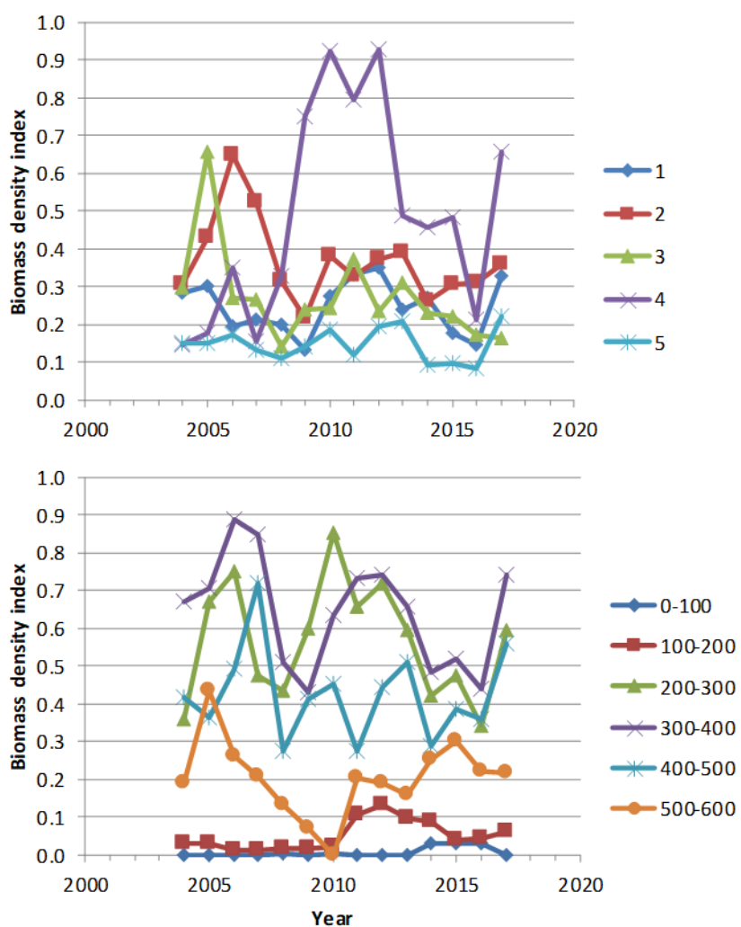
Fig. 9. Estimated mean biomass density index. Upper: by main strata (see fig 3). Bottom: by depth strata.
