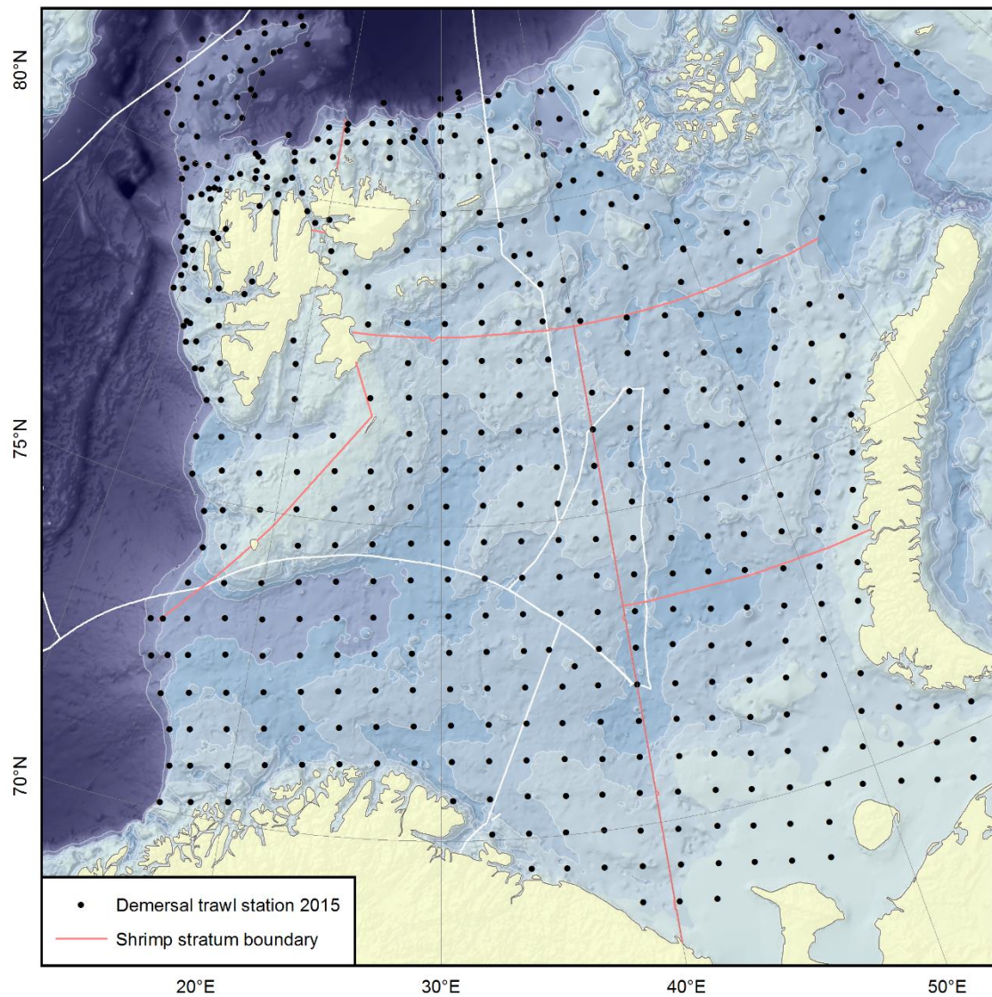
Fig. 1. Sampling locations of the 2016 Norwegian-Russian ecosystem survey in the Barents Sea.
