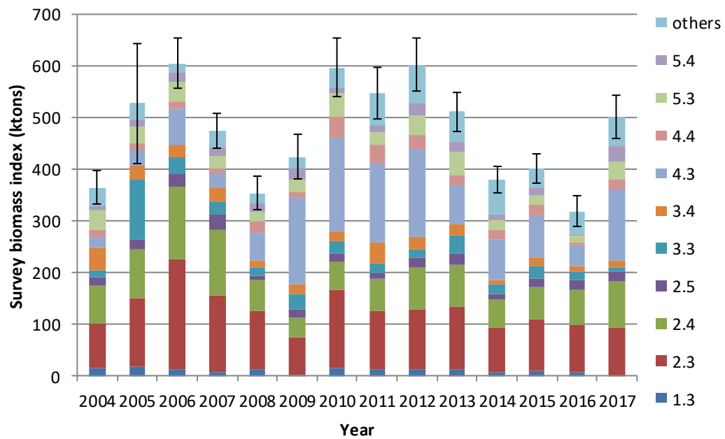
Fig. 6. Estimated mean index of biomass by year and sub-strata (code: see Table 1 and Fig. 3 for definition). Error bars indicate +/- one Standard Error of the overall estimate.
