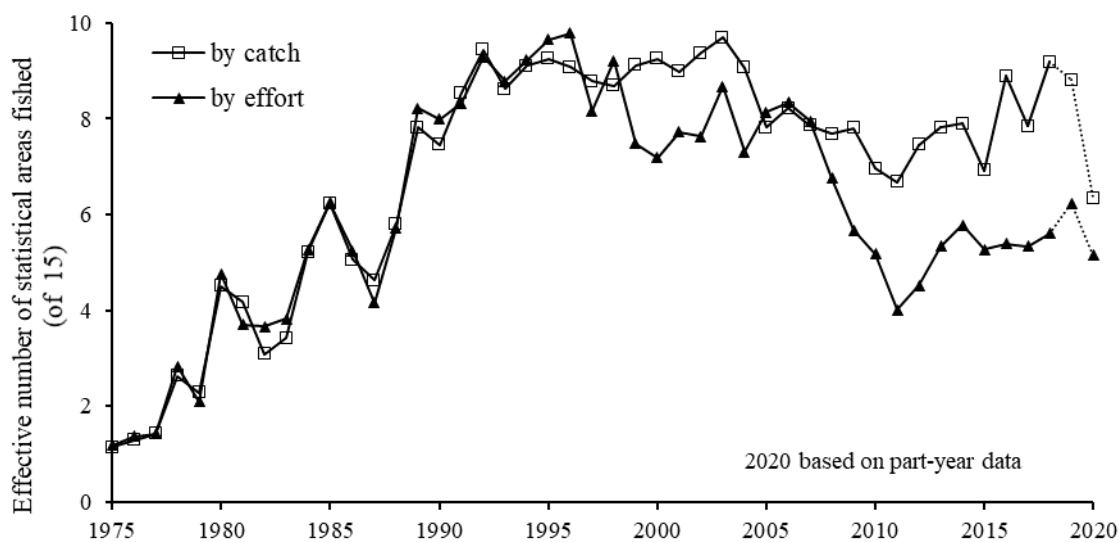
Figure 6a. P. borealis in W. Greenland: diversity indices for the distribution of logbook-recorded catch between statistical Areas in Greenland waters, 1975–2020. 2020 is on part-year's data.
